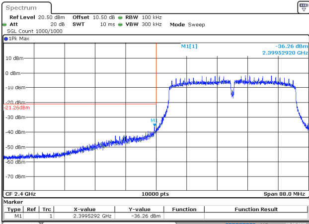
802.11n40_2422MHz
