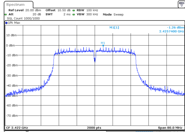
802.11n40_2422MHz
