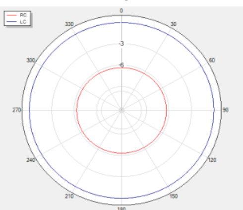
Theta=0 freq=2450MHz
