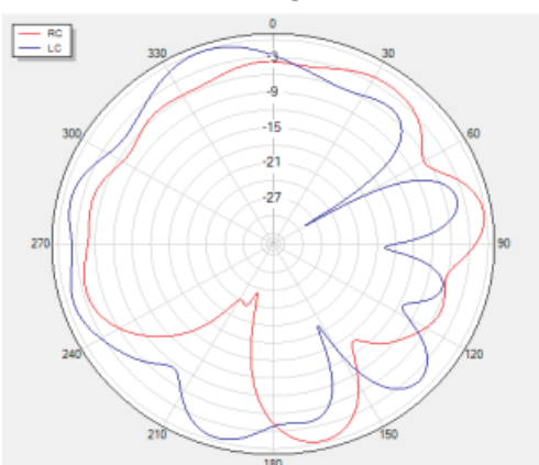
Theta=90 freq=2450MHz
