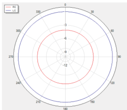
Theta=0 freq=2400MHz
