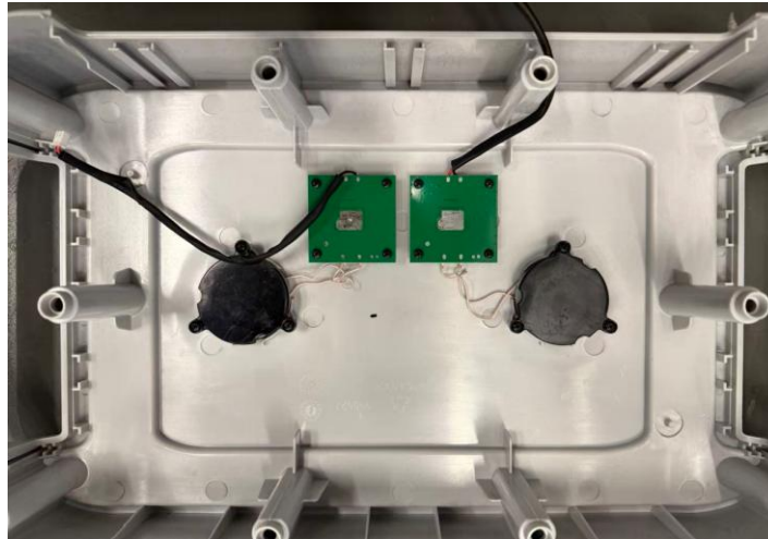
Wireless charging module
