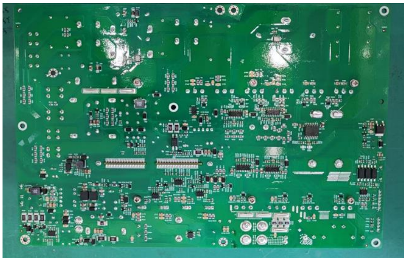
Bottom view of Inverter board
