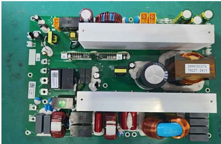
Top view of Inverter board
