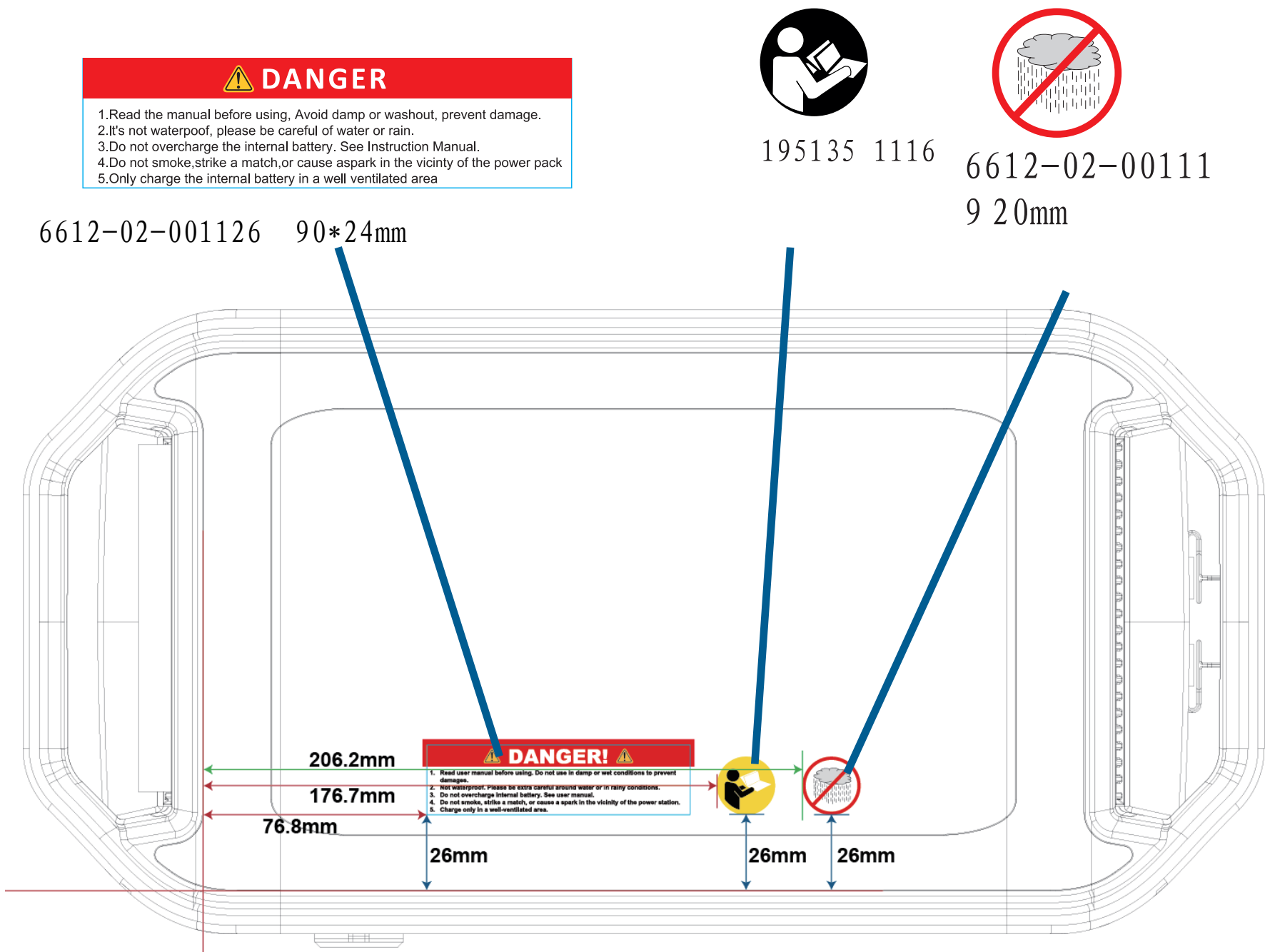
The top of the machine
