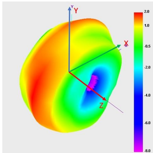
3D radiation
