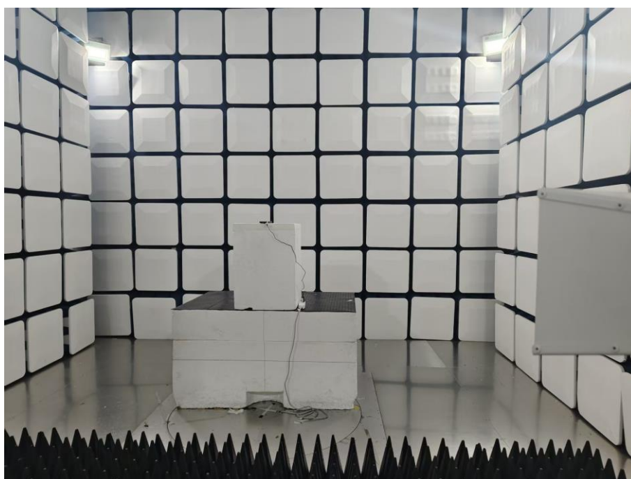
Above 1GHz-RFID
