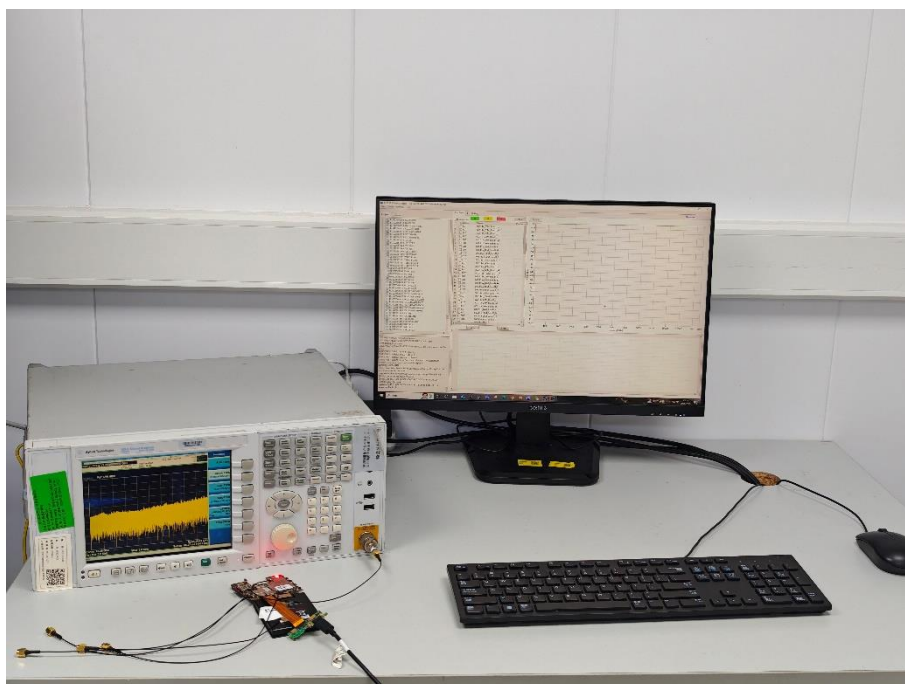
Conducted Test-BT/WIFI/RFID
