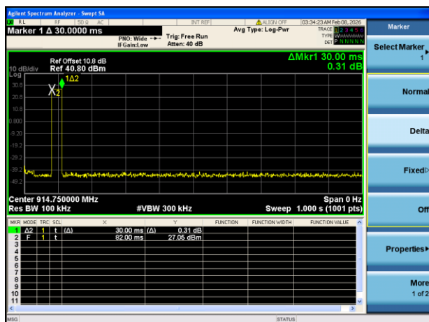
Pulse Width
