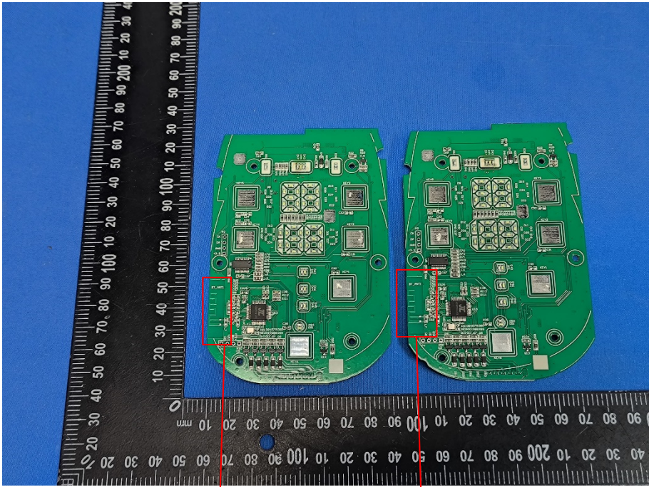
Bluetooth Antenna
