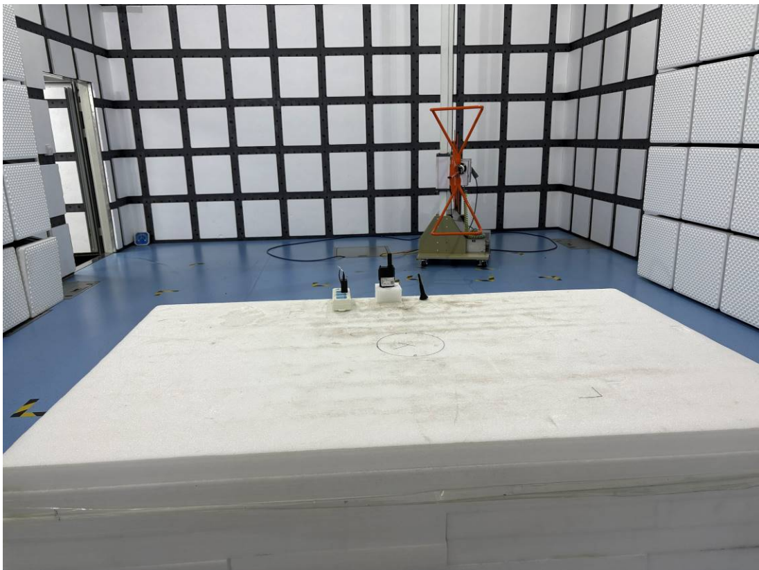
RE- Rear View (Below 1GHz)
