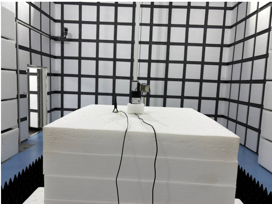
RE- Rear View (Above 1GHz)
