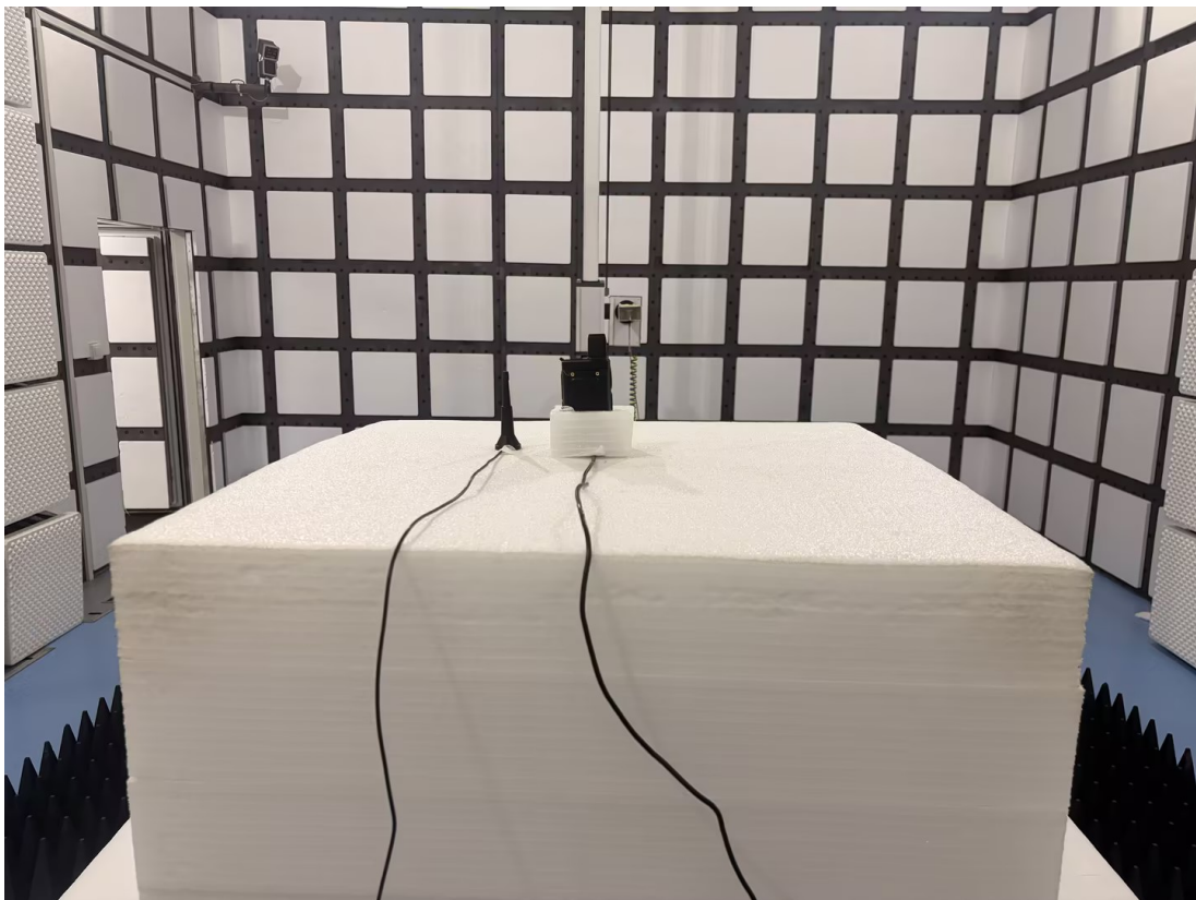
Radiation Emission - Back View (Above 18GHz)
