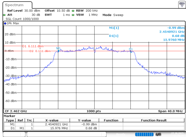
802.11n ht20_2462MHz_Chain 0
