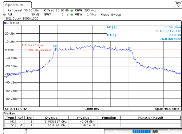
802.11n ht20_2412MHz_Chain 1
