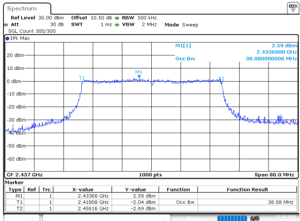
802.11ax he40_2437MHz_RU_Full_Chain 0
