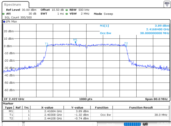
802.11ax he40_2422MHz_RU_Full_Chain 1
