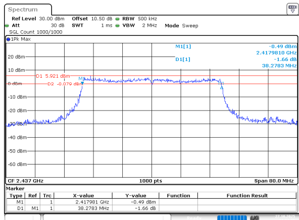
802.11ax he40_2437MHz_RU_Full_Chain 1
