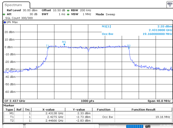
802.11ax he20_2437MHz_RU_Full_Chain 1
