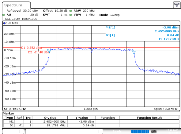
802.11ax he20_2462MHz_RU_Full_Chain 1
