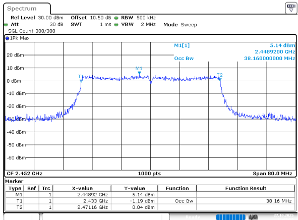
802.11ax he40_2452MHz_RU_Full_Chain 1
