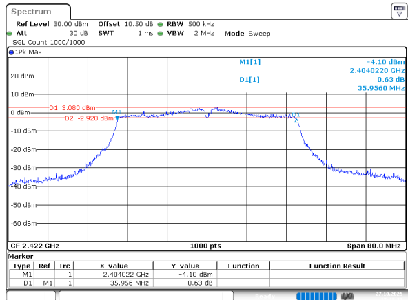
802.11n ht40_2422MHz_Chain 0
