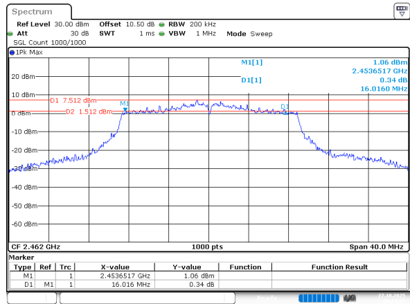
802.11n ht20_2462MHz_Chain 1
