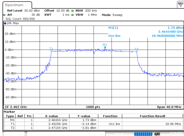
802.11ax he20_2462MHz_RU_Full_Chain 0
