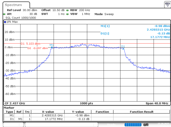
802.11n ht20_2437MHz_Chain 0
