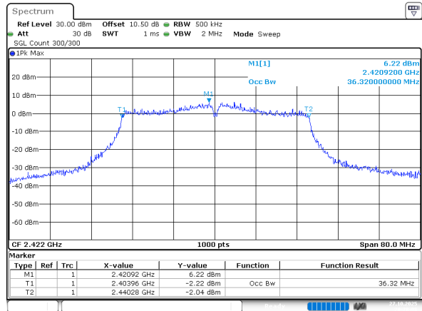
802.11n ht40_2422MHz_Chain 1
