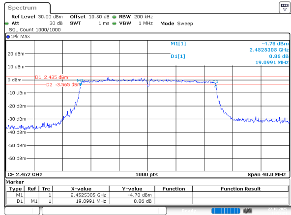
802.11ax he20_2462MHz_RU_Full_Chain 0
