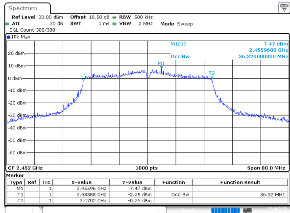
802.11n ht40_2452MHz_Chain 1
