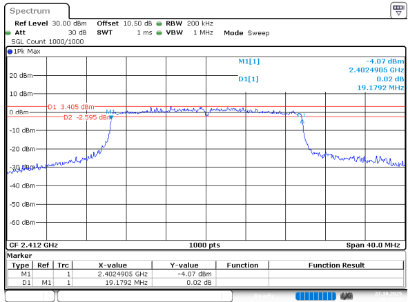
802.11ax he20_2412MHz_RU_Full_Chain 1
