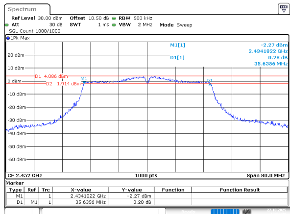
802.11n ht40_2452MHz_Chain 0
