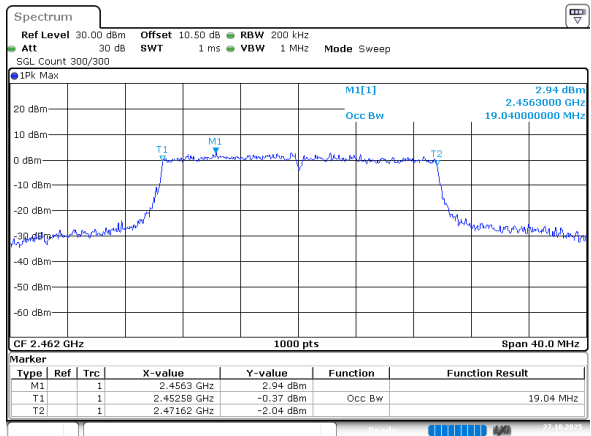
802.11ax he20_2462MHz_RU_Full_Chain 1
