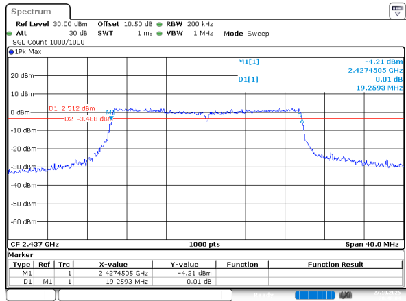
802.11ax he20_2437MHz_RU_Full_Chain 1
