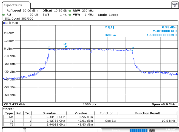
802.11ax he20_2437MHz_RU_Full_Chain 0
