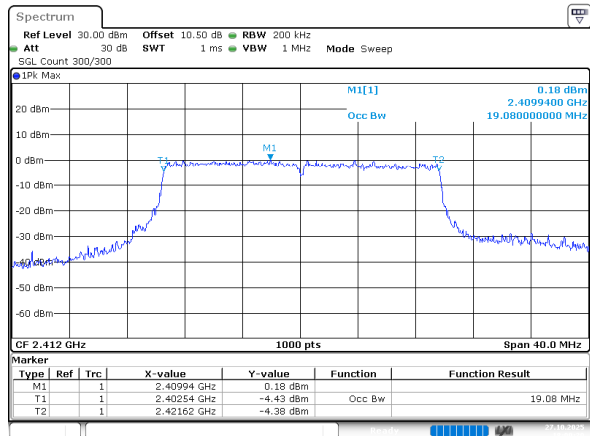
802.11ax he20_2412MHz_RU_Full_Chain 0
