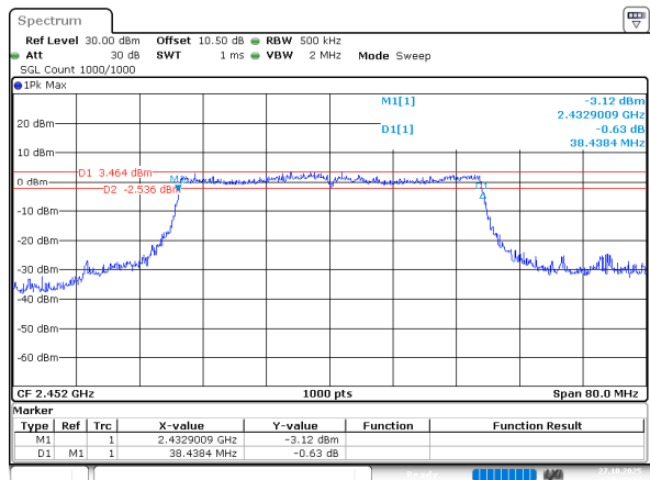
802.11ax he40_2452MHz_RU_Full_Chain 0
