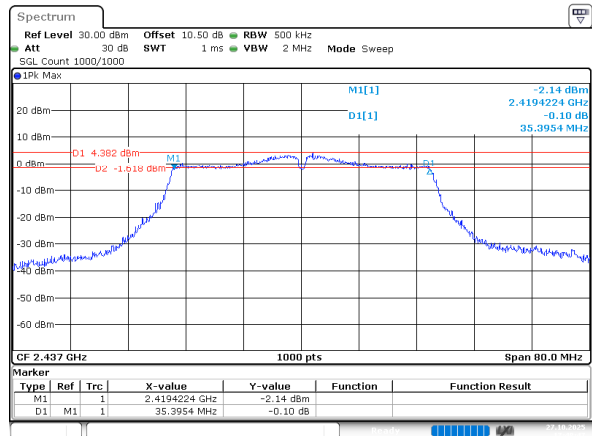
802.11n ht40_2437MHz_Chain 0
