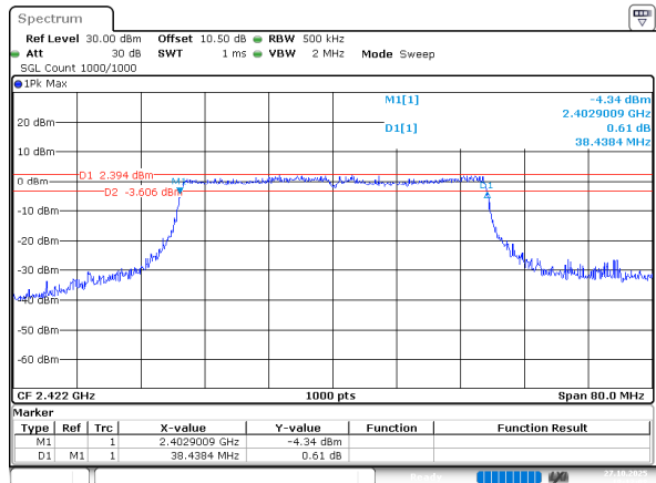
802.11ax he40_2422MHz_RU_Full_Chain 0
