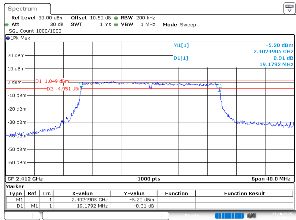
802.11ax he20_2412MHz_RU_Full_Chain 0
