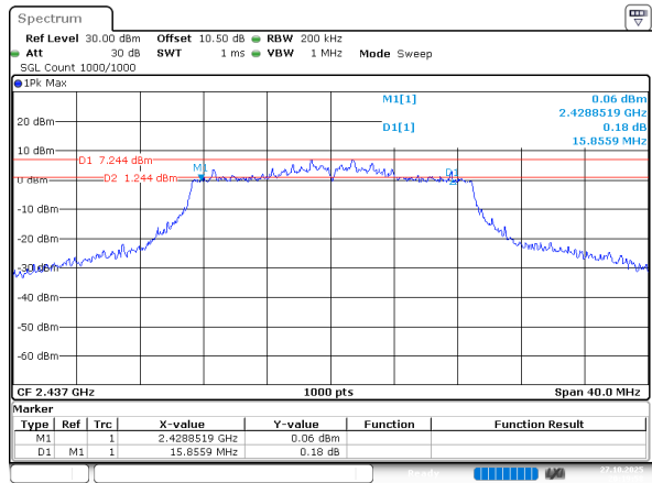
802.11n ht20_2437MHz_Chain 1
