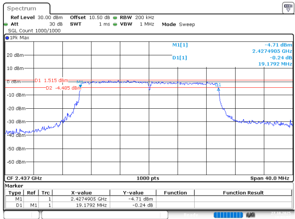
802.11ax he20_2437MHz_RU_Full_Chain 0
