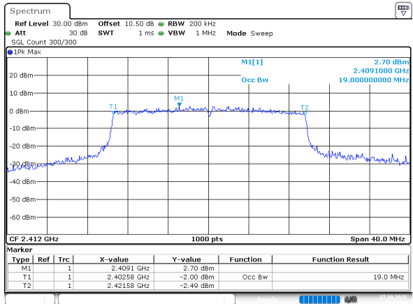
802.11ax he20_2412MHz_RU_Full_Chain 1
