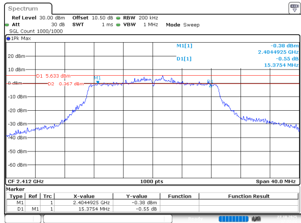
802.11n ht20_2412MHz_Chain 0
