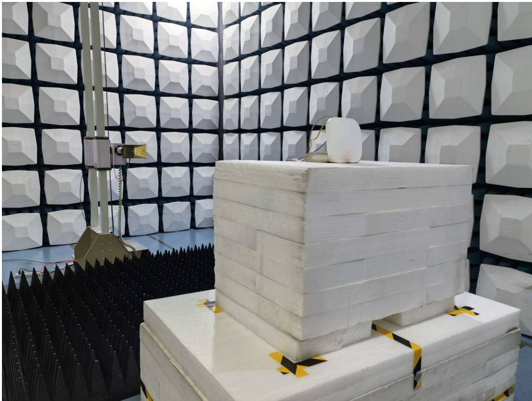
Radiated Emission 18GHz-25GHz View
