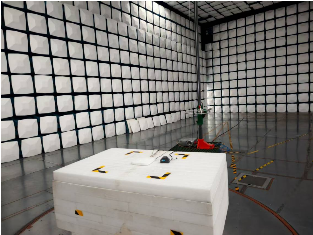
Radiated Emission 30MHz-1GHz View
