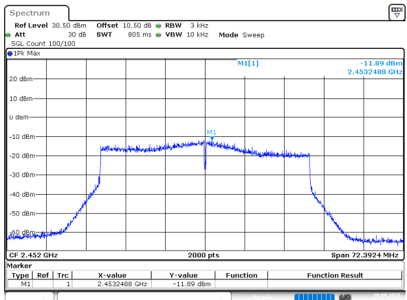
802.11ax40_2452MHz_Chain 1
