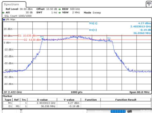
802.11ax40_2422MHz_Chain 0
