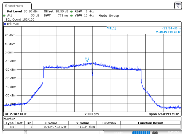
802.11ax40_2437MHz_Chain 1
