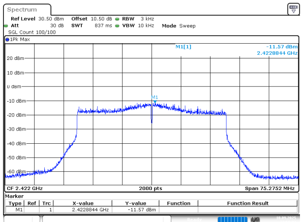
802.11ax40_2422MHz_Chain 1
