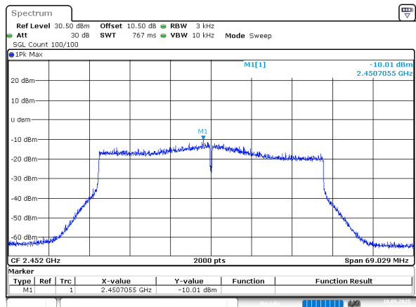
802.11ax40_2452MHz_Chain 0
