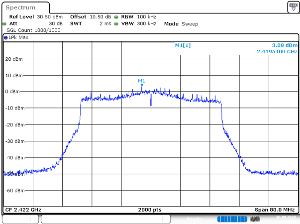
802.11ax40_2422MHz_Chain 0
