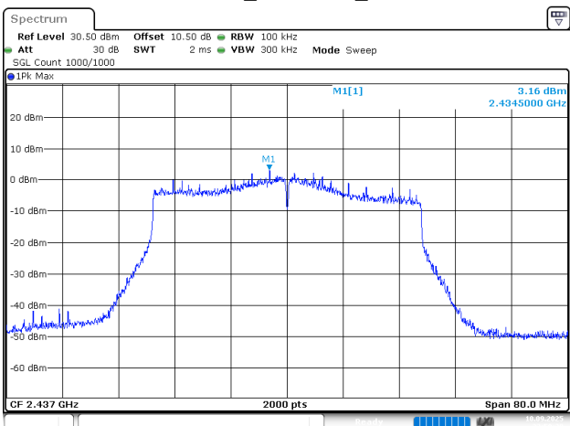
802.11ax40_2437MHz_Chain 1
