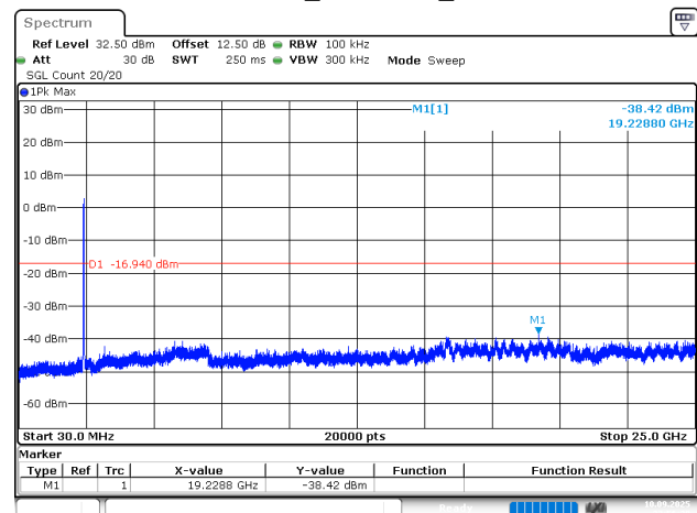
802.11ax40_2422MHz_Chain 1
