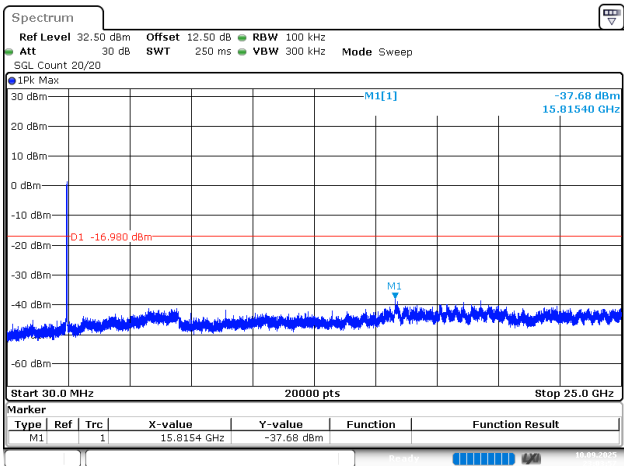
802.11ax40_2452MHz_Chain 1
