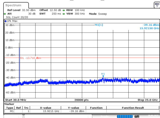
802.11ax20_2412MHz_Chain 0
