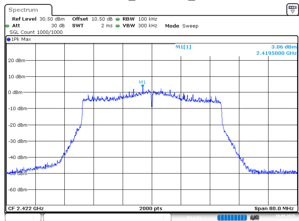
802.11ax40_2422MHz_Chain 1
