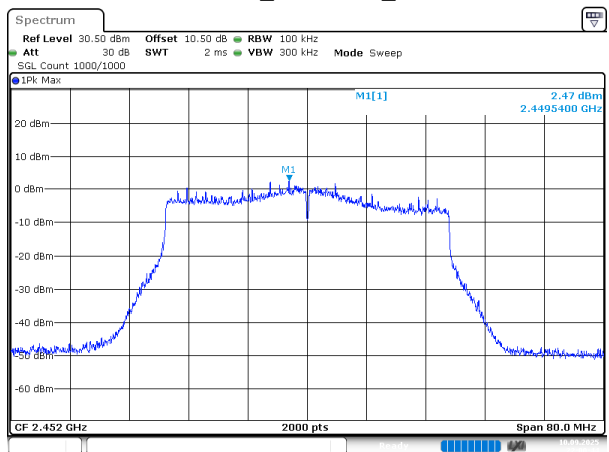
802.11ax40_2452MHz_Chain 0
