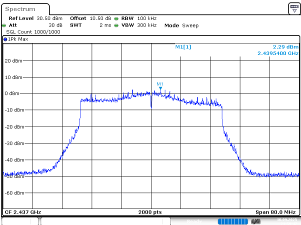
802.11ax40_2437MHz_Chain 0
