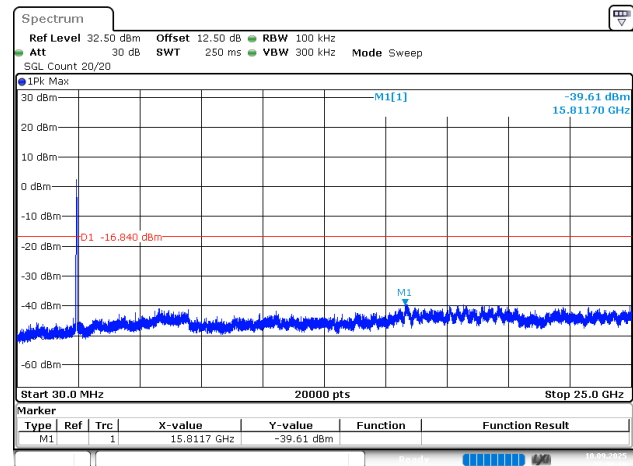
802.11ax40_2437MHz_Chain 1
