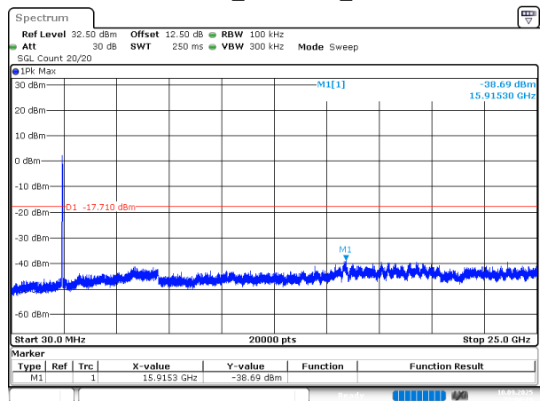
802.11ax40_2437MHz_Chain 0
