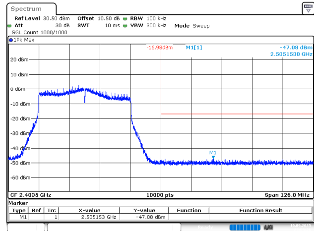
802.11ax40_2452MHz_Chain 1
