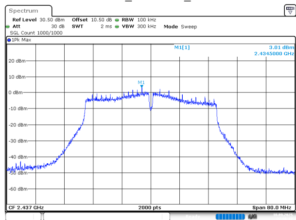
802.11n40_2437MHz_Chain 1
