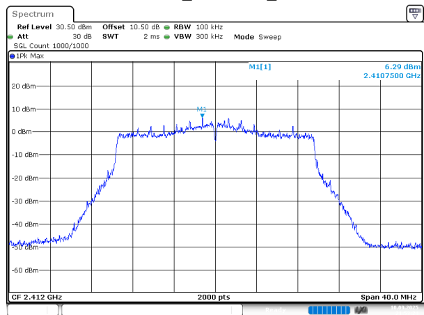
802.11ax20_2412MHz_Chain 0
