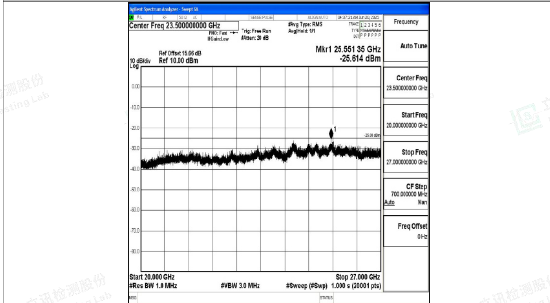
Band7_20MHz_QPSK_21100_1RB#0_20000~27000_20000~27000
