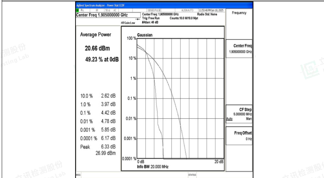
Band25-20MHz-16QAM-26590-1RB#0-PASS
