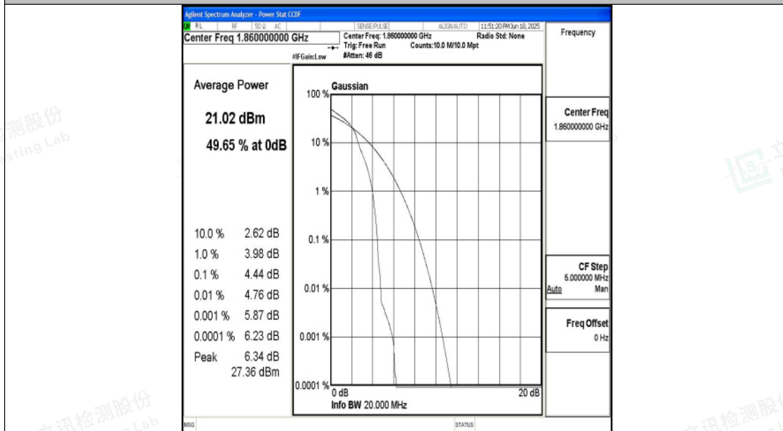
Band25-20MHz-16QAM-26140-1RB#0-PASS
