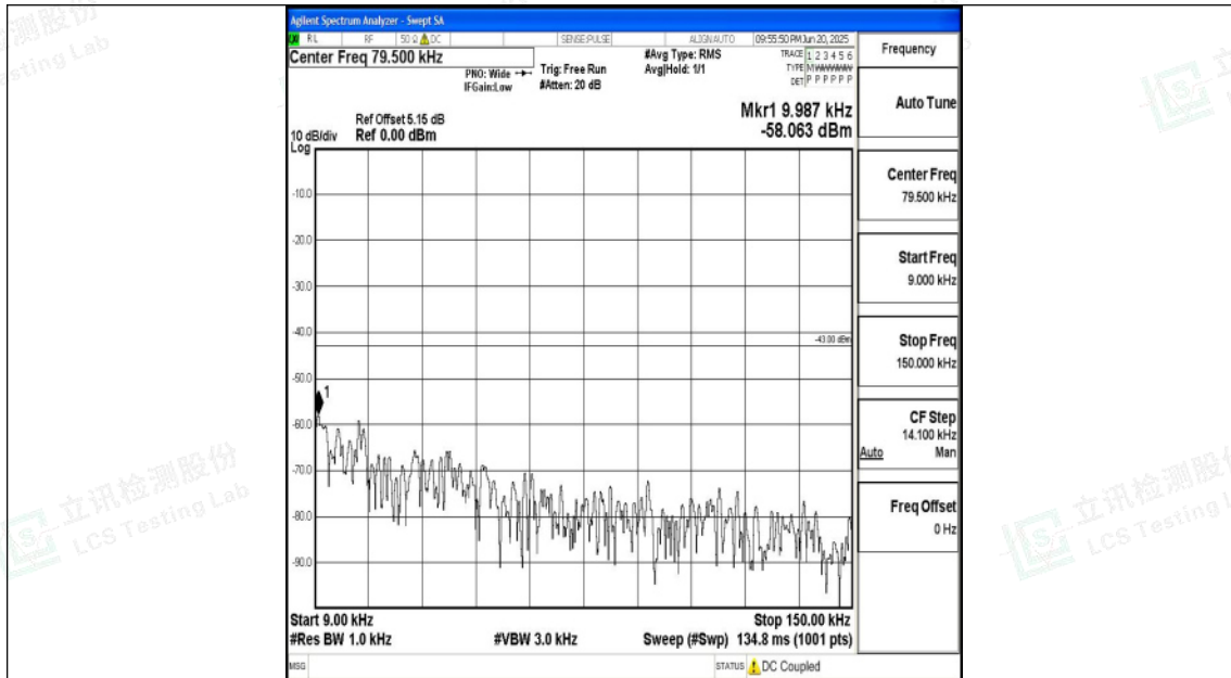
Band25_15MHz_QPSK_26365_1RB#0_0.009~0.15_0.009~0.15
