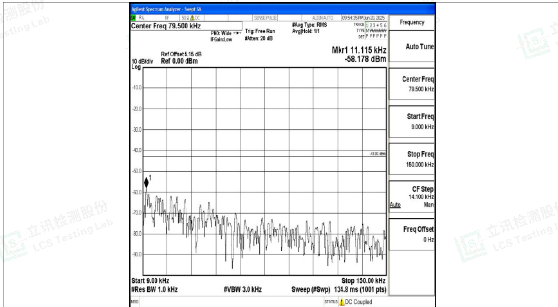
Band25_15MHz_QPSK_26115_1RB#0_0.009~0.15_0.009~0.15
