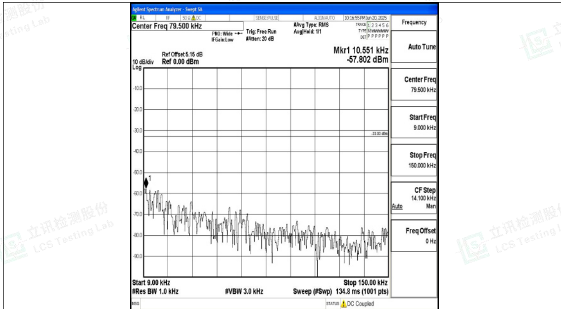
Band26_10MHz_QPSK_26740_1RB#0_0.009~0.15_0.009~0.15
