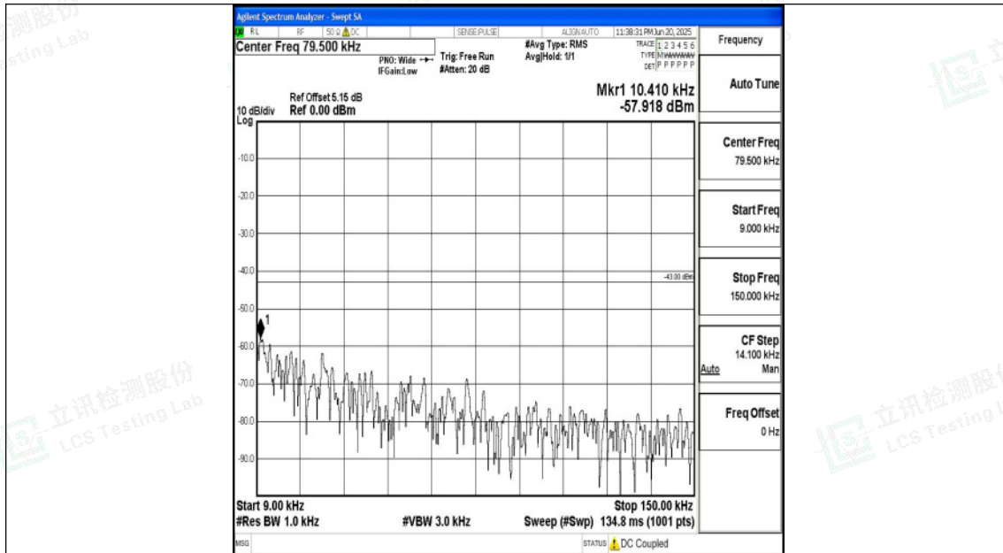
Band66_3MHz_QPSK_132657_1RB#0_0.009~0.15_0.009~0.15
