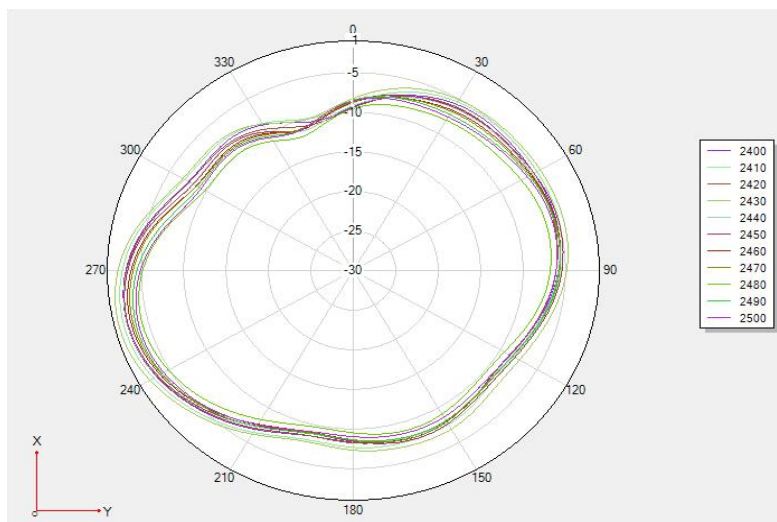
Theta 90 2D
