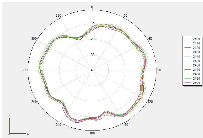
Phi 90 2D
