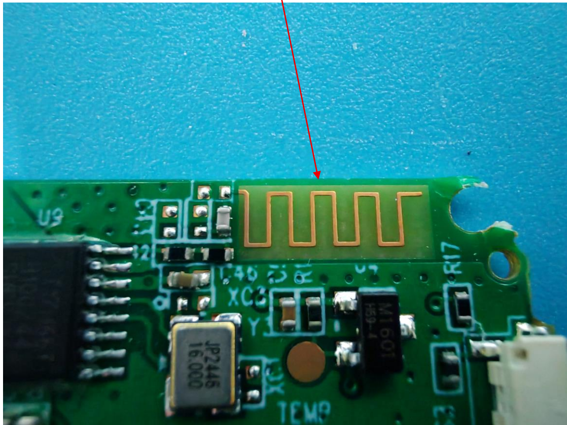
SRD Antenna (only RX)
