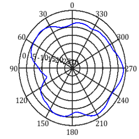
frequency=820MHz, X-Y Plane
