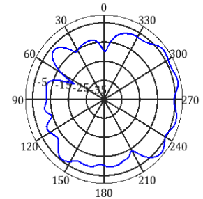
frequency=1990MHz, X-Y Plane
