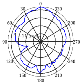
frequency=820MHz, X-Z Plane
