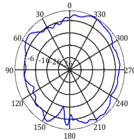
frequency=2600MHz, Y-Z Plane
