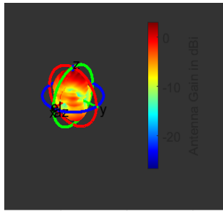
frequency=820MHz, X-Z Plane
