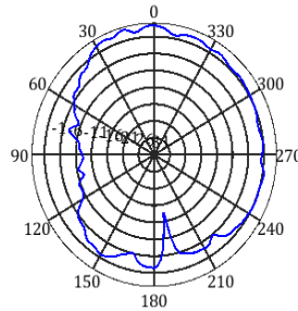
frequency=820MHz, Y-Z Plane
