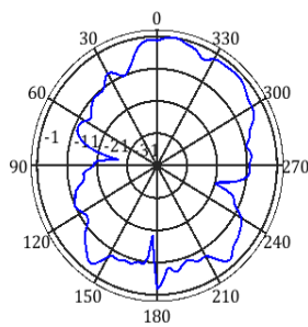
frequency=1990MHz, X-Z Plane
