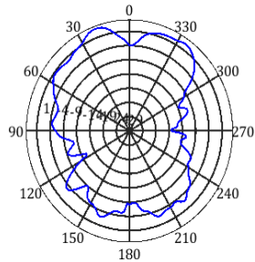
frequency=2600MHz, X-Z Plane
