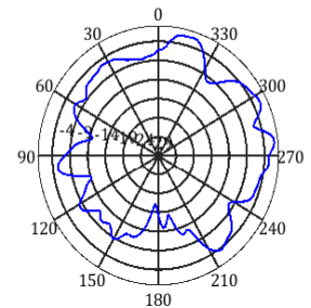
frequency=2600MHz, X-Y Plane
