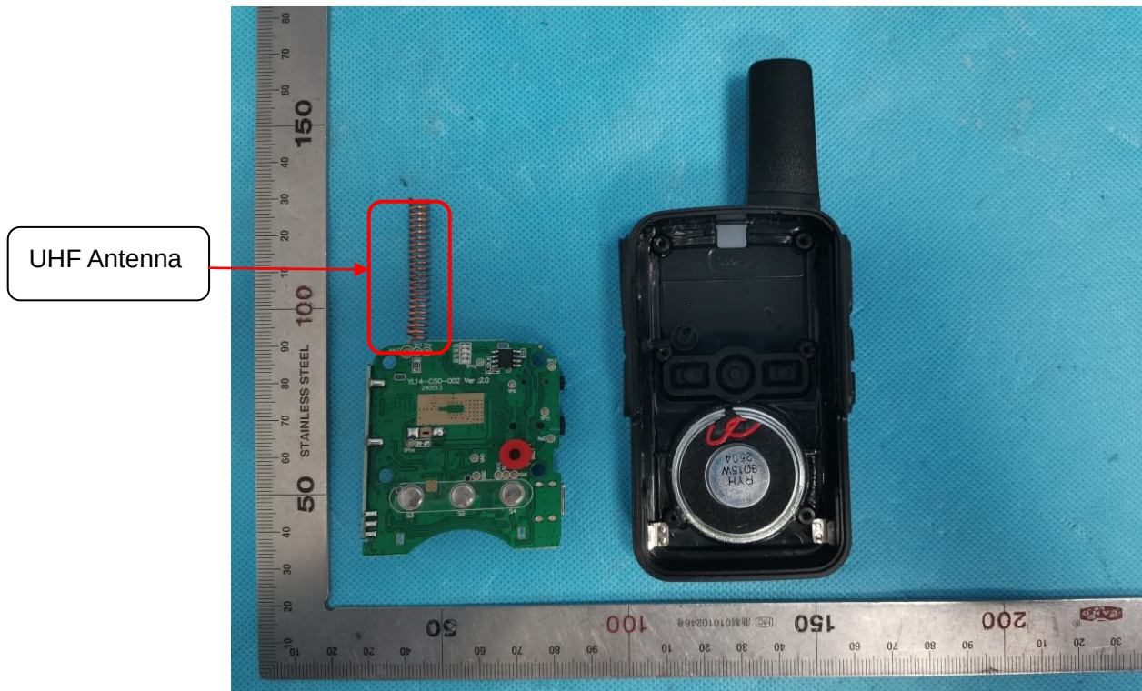
Internal View-3 of EUT
