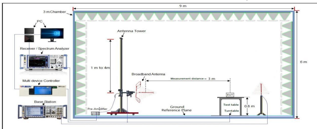
Radiated Emissions Above 1GHz Test setup
