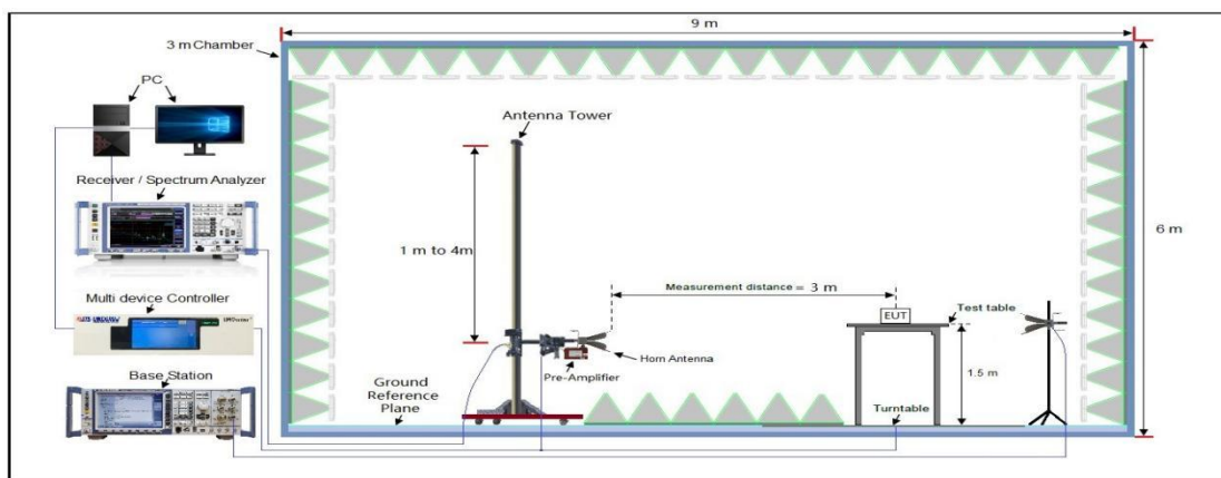
Radiated Emissions Above 1GHz Test setup
