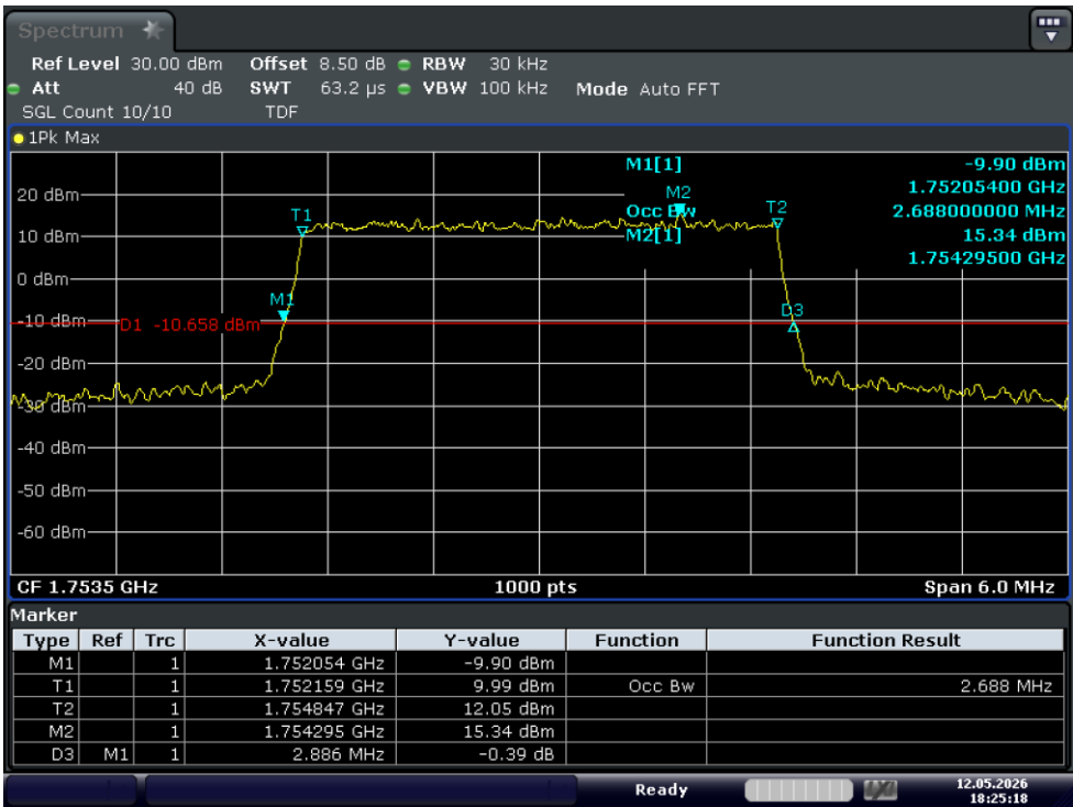
Test_Graph_band4_1753.5MHz_3M_16QAM_15RB#LOW_OBW&EBW
