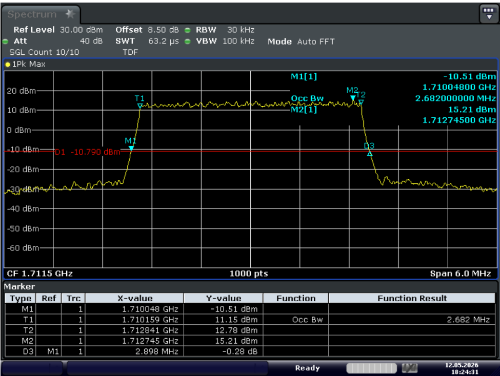
Test_Graph_band4_1711.5MHz_3M_16QAM_15RB#LOW_OBW&EBW
