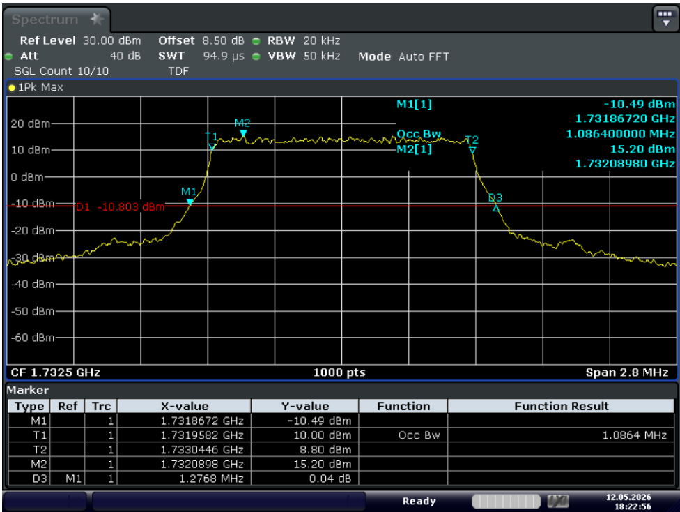
Test_Graph_band4_1732.5MHz_1.4M_16QAM_6RB#LOW_OBW&EBW
