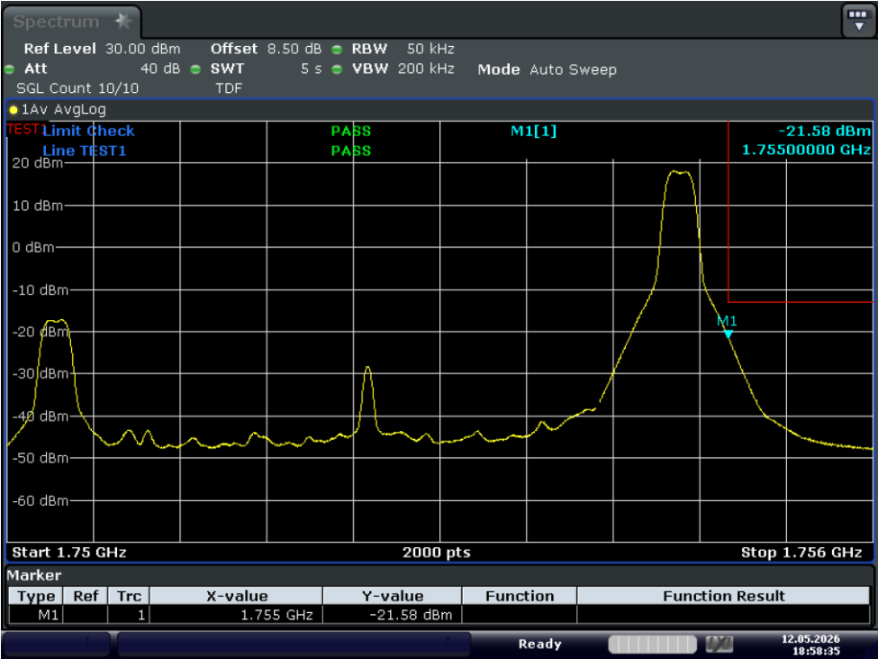
Test_Graph_band4_1752.5MHz_5M_QPSK_1RB#HIGH_Band edge
