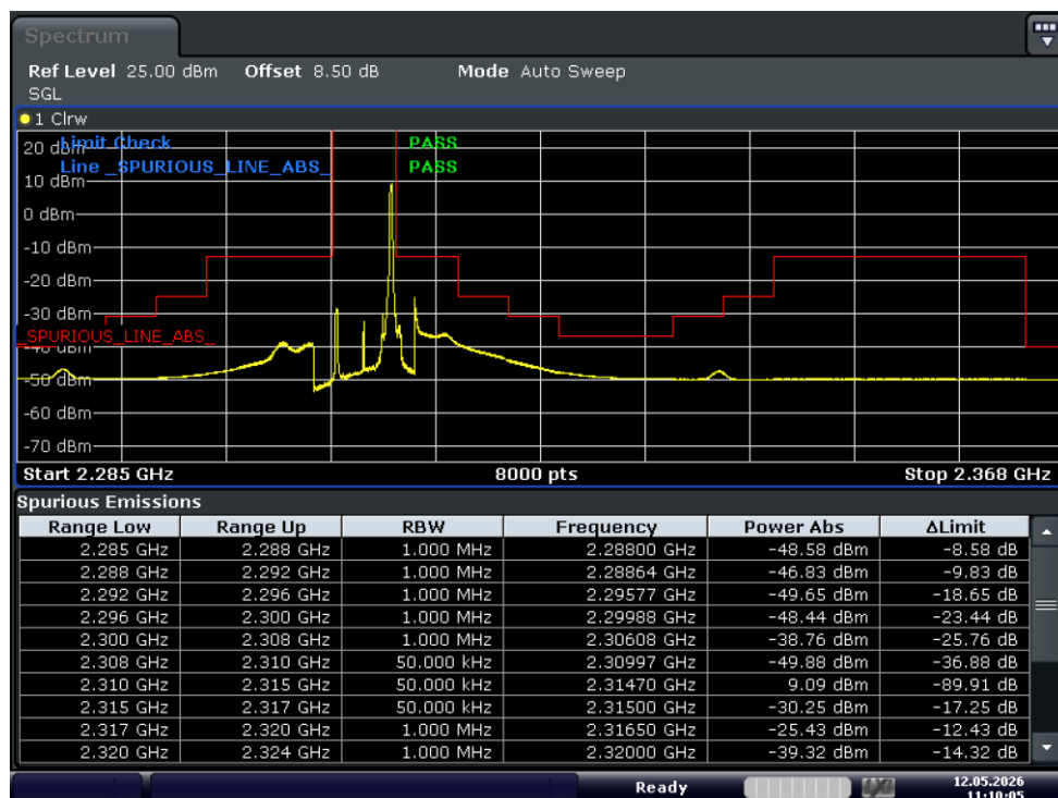
Test_Graph_band40(2305-2315)_2312.5MHz_5M_QPSK_1RB#HIGH_Band edge
