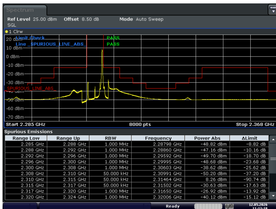
Test_Graph_band40(2305-2315)_2312.5MHz_5M_16QAM_1RB#HIGH_Band edge
