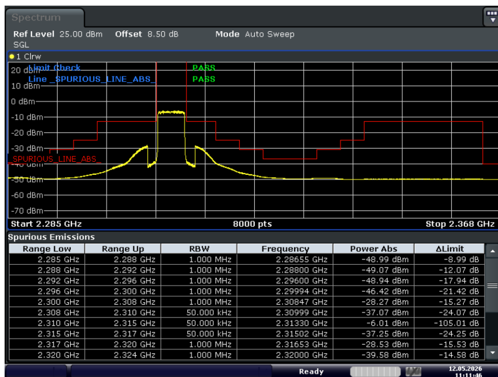
Test_Graph_band40(2305-2315)_2312.5MHz_5M_QPSK_1RB#HIGH_Band edge
