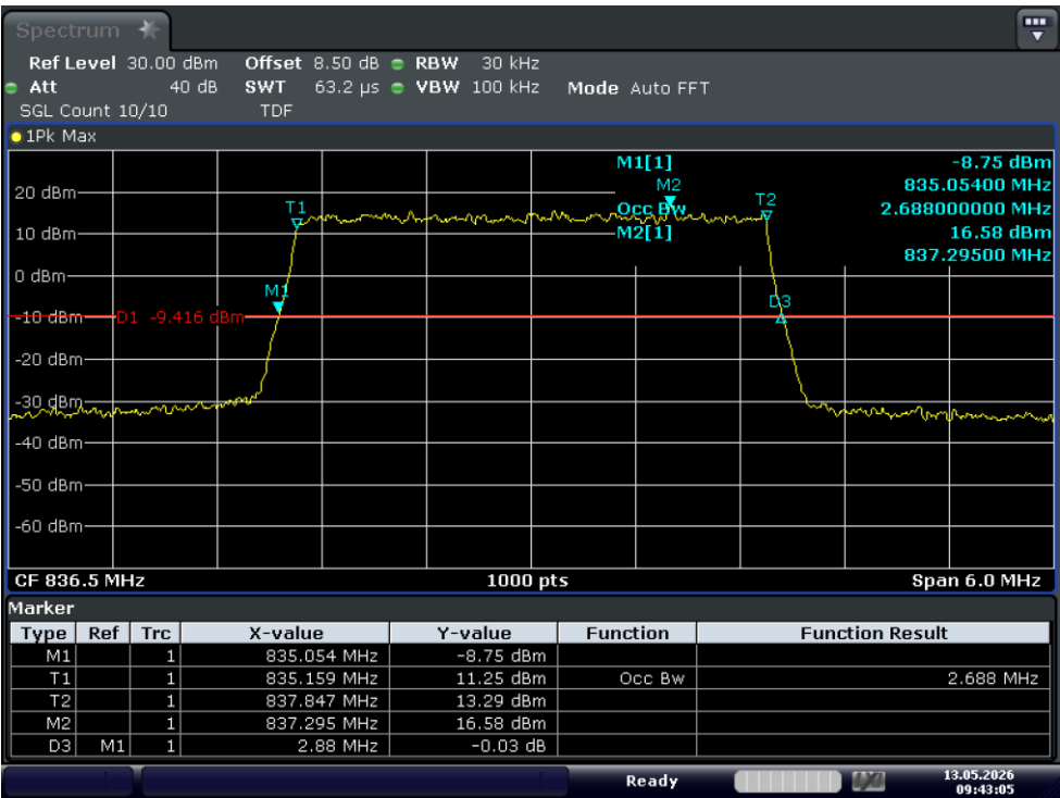
Test_Graph_band5_836.5MHz_3M_16QAM_15RB#LOW_OBW&EBW
