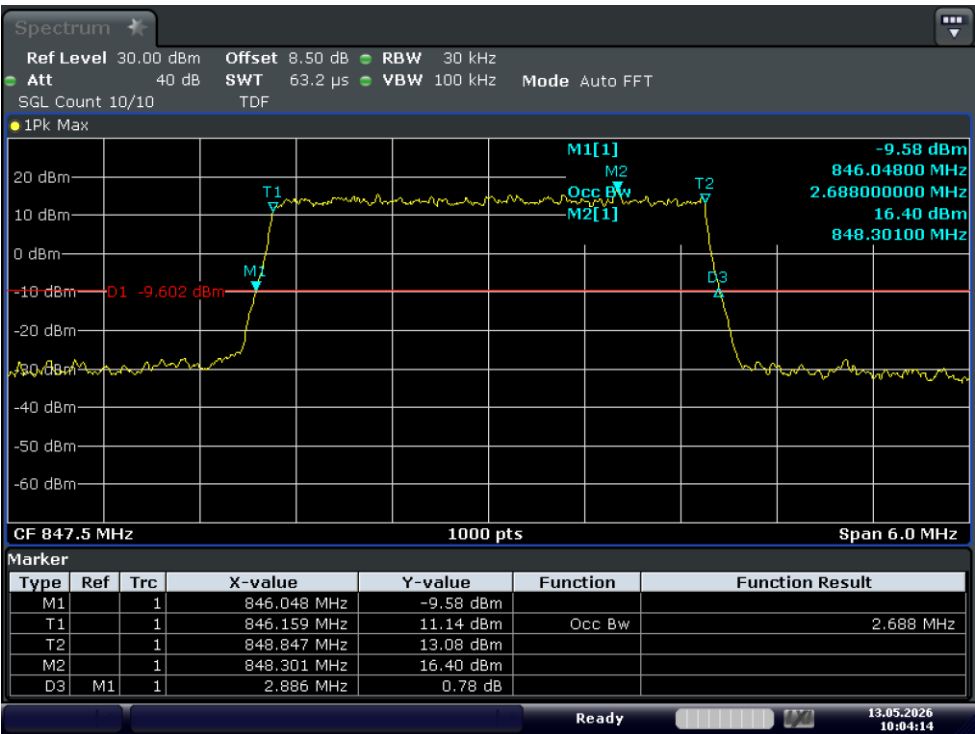
Test_Graph_band5_847.5MHz_3M_16QAM_15RB#LOW_OBW&EBW
