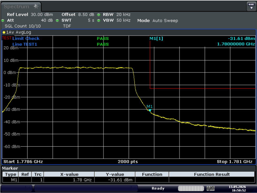
Test_Graph_band66_1779.3MHz_1.4M_16QAM_1RB#HIGH_Band edge
