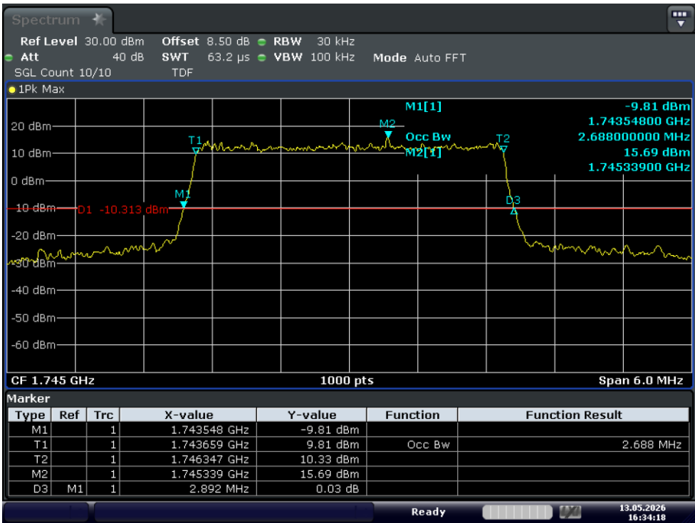
Test_Graph_band66_1745MHz_3M_16QAM_15RB#LOW_OBW&EBW
