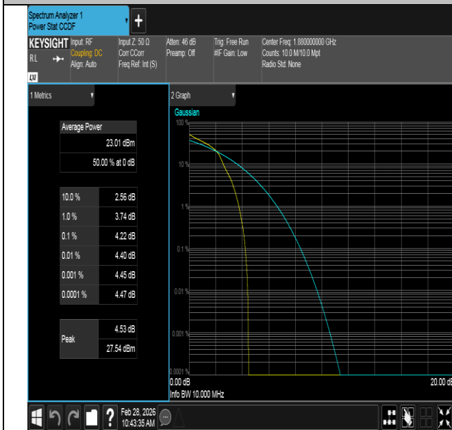
Band2-10MHz-16QAM-18900-1RB#0-PASS
