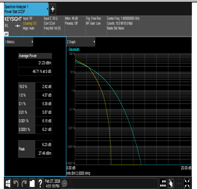
Band2-1.4MHz-16QAM-18900-6RB#0-PASS
