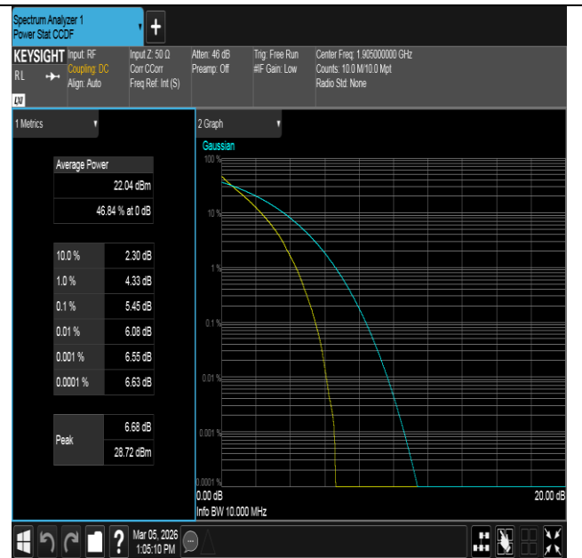
Band2-10MHz-QPSK-19150-50RB#0-PASS
