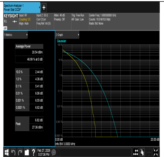
Band2-3MHz-QPSK-19185-15RB#0-PASS
