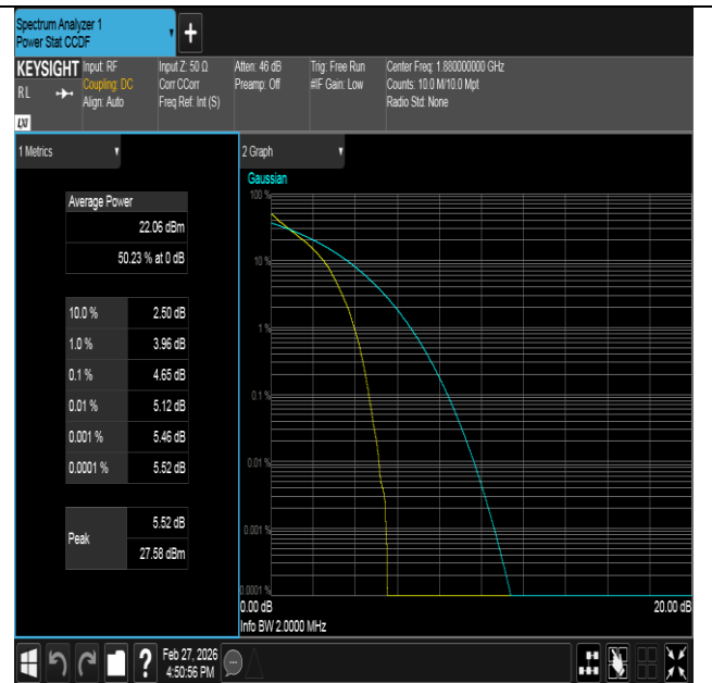
Band2-1.4MHz-QPSK-18900-6RB#0-PASS
