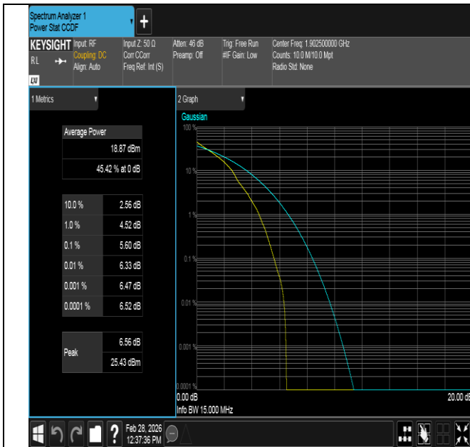
Band2-15MHz-QPSK-19125-1RB#0-PASS
