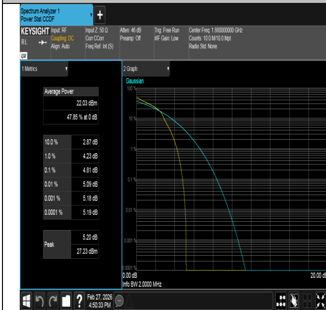
Band2-1.4MHz-16QAM-18900-1RB#0-PASS
