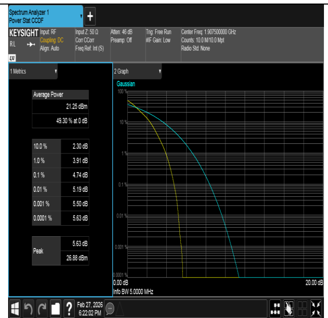
Band2-5MHz-QPSK-19175-25RB#0-PASS
