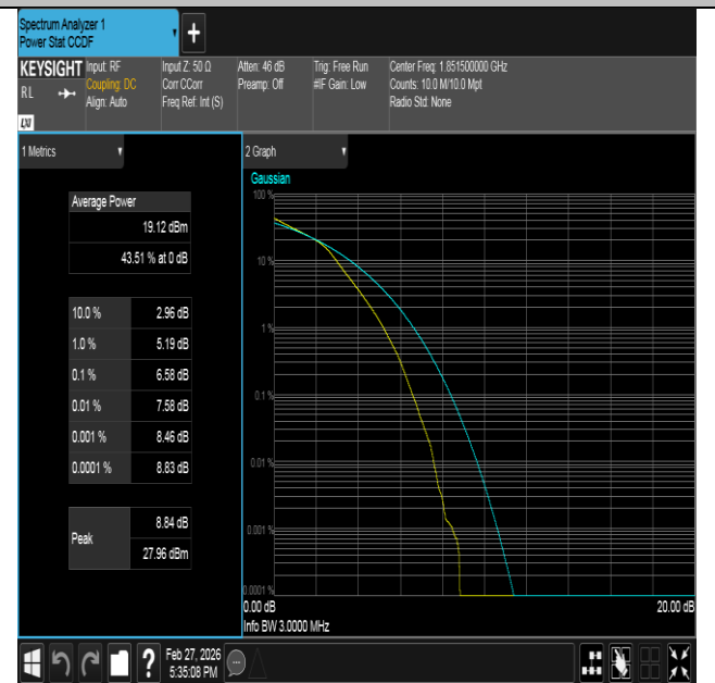
Band2-3MHz-16QAM-18615-15RB#0-PASS
