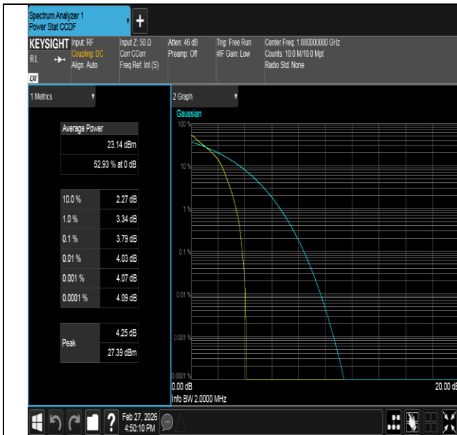
Band2-1.4MHz-QPSK-18900-1RB#0-PASS
