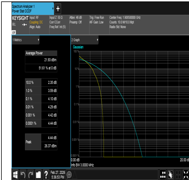
Band2-3MHz-QPSK-19185-1RB#0-PASS
