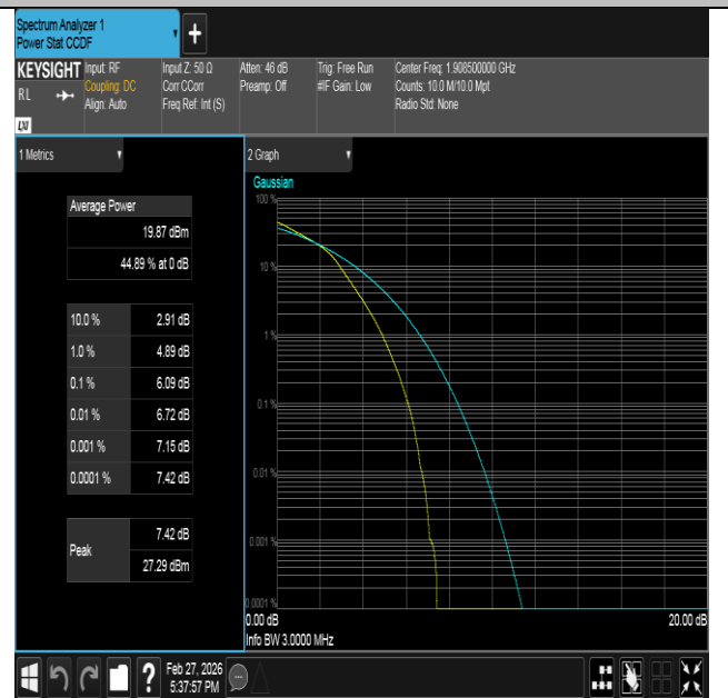
Band2-3MHz-16QAM-19185-15RB#0-PASS
