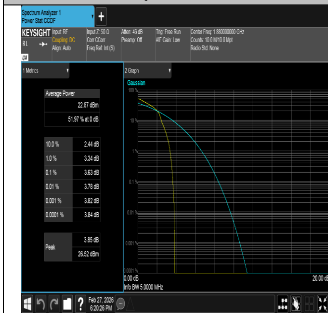
Band2-5MHz-16QAM-18900-1RB#0-PASS
