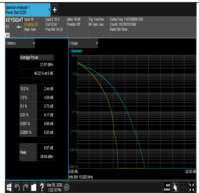
Band2-15MHz-QPSK-18675-75RB#0-PASS
