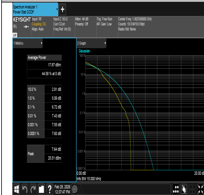
Band2-15MHz-16QAM-19125-1RB#0-PASS
