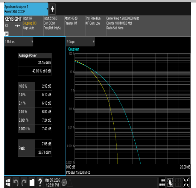
Band2-15MHz-16QAM-19125-75RB#0-PASS
