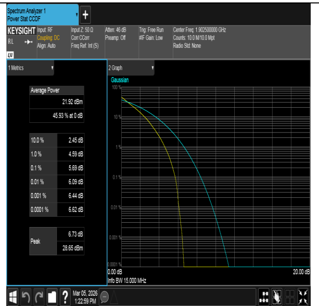
Band2-15MHz-QPSK-19125-75RB#0-PASS
