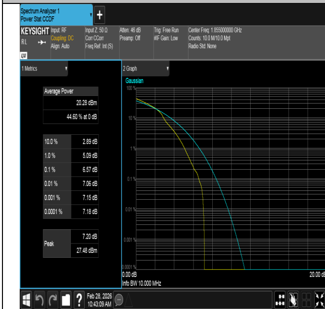
Band2-10MHz-16QAM-18650-1RB#0-PASS
