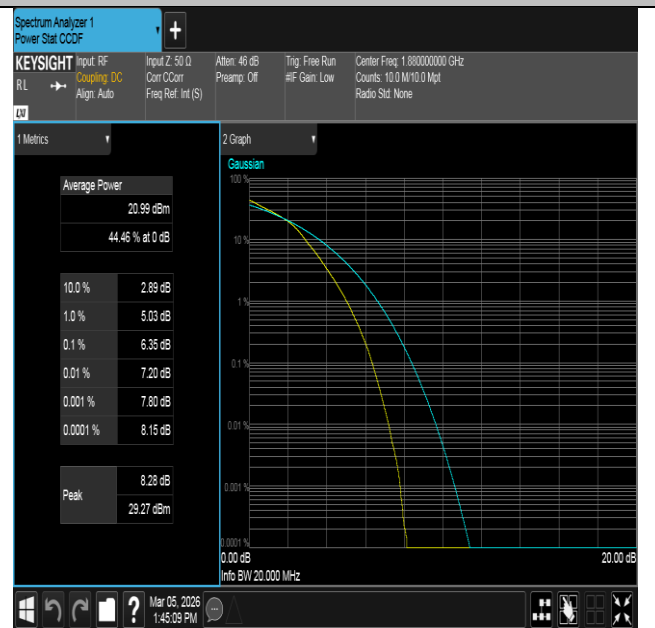
Band2-20MHz-16QAM-18900-100RB#0-PASS
