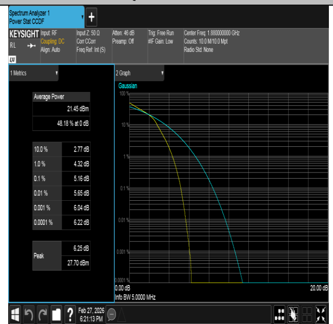
Band2-5MHz-16QAM-18900-25RB#0-PASS
