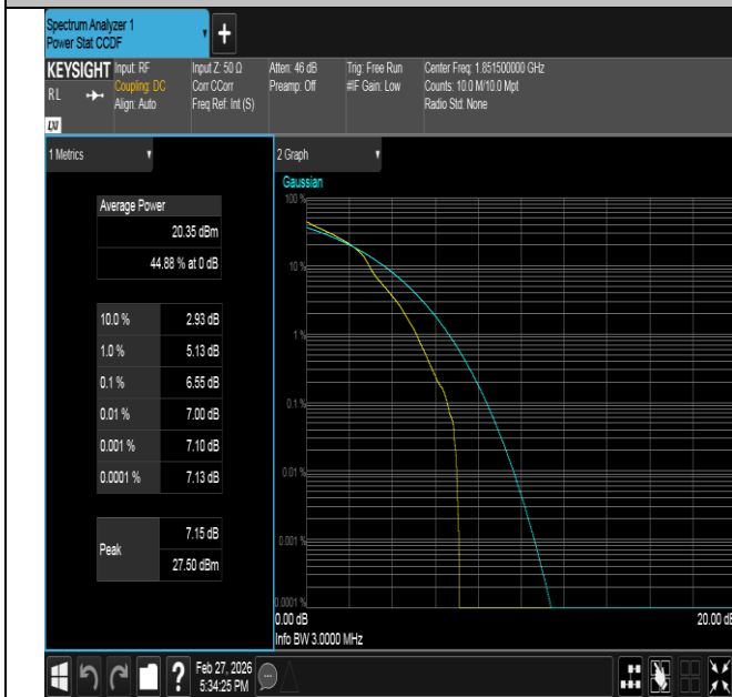
Band2-3MHz-16QAM-18615-1RB#0-PASS
