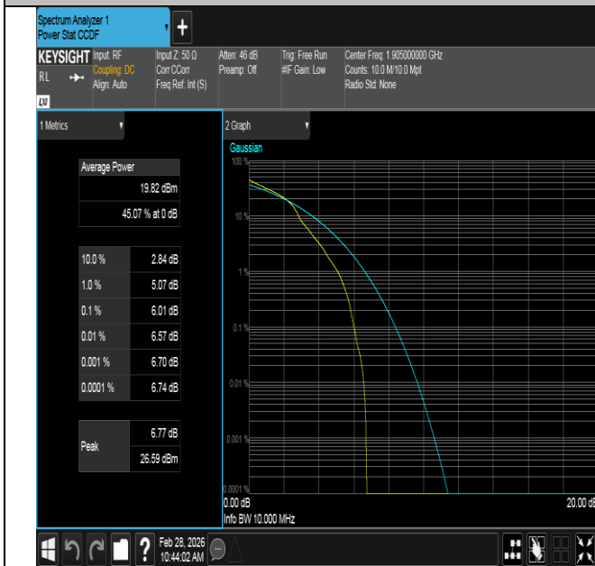
Band2-10MHz-16QAM-19150-1RB#0-PASS
