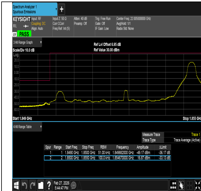
Band2-5MHz-16QAM-18625-1RB#24-PASS
