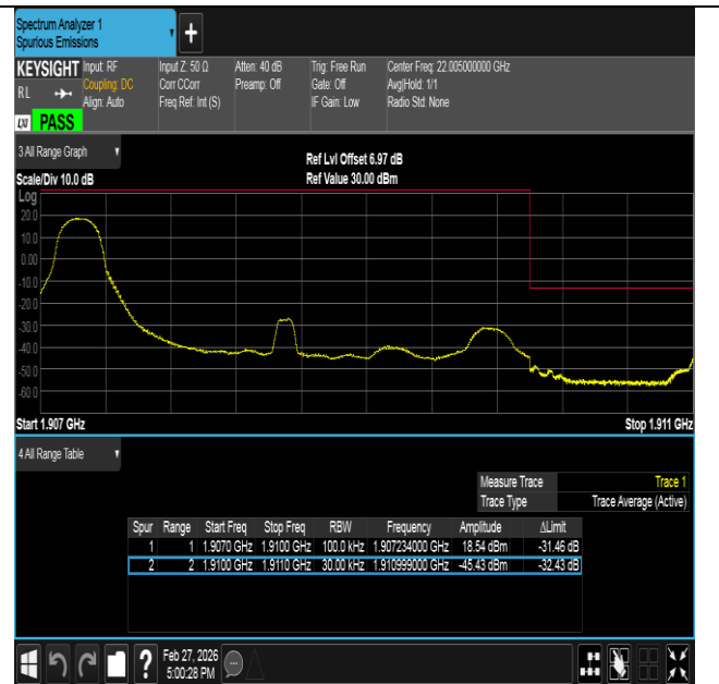
Band2-3MHz-16QAM-19185-1RB#0-PASS
