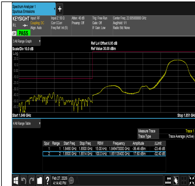
Band2-1.4MHz-16QAM-18607-1RB#5-PASS
