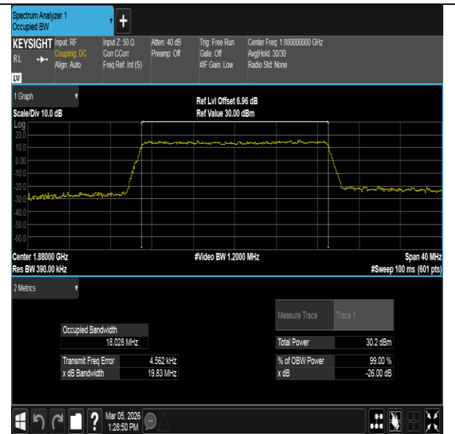
Band2-20MHz-16QAM-18900-100RB#0-PASS
