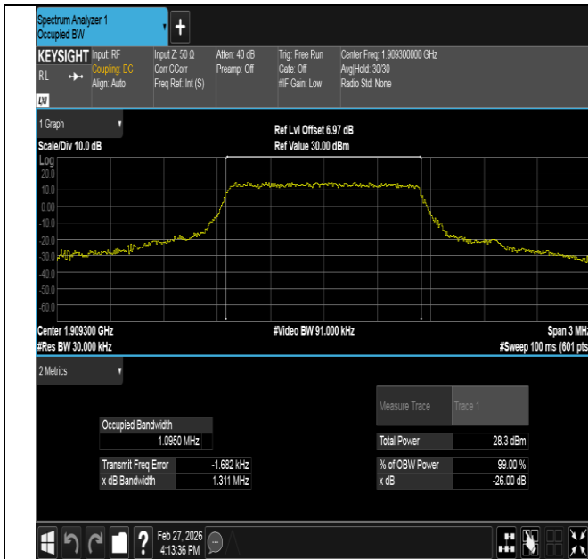
Band2-1.4MHz-QPSK-19193-6RB#0-PASS
