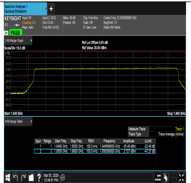
Band2-10MHz-16QAM-18650-50RB#0-PASS
