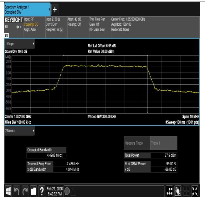
Band2-5MHz-16QAM-18625-25RB#0-PASS
