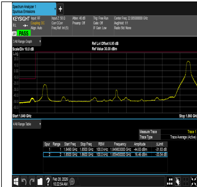
Band2-10MHz-16QAM-18650-1RB#49-PASS
