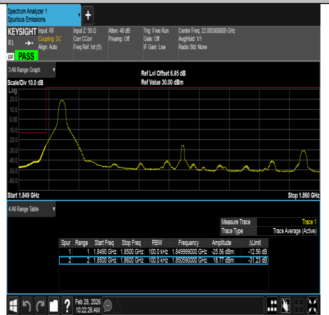
Band2-10MHz-16QAM-18650-1RB#0-PASS
