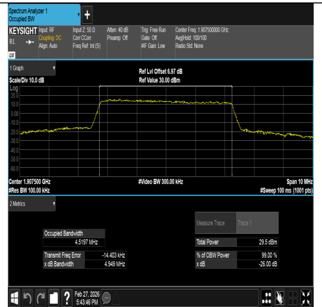
Band2-5MHz-16QAM-19175-25RB#0-PASS
