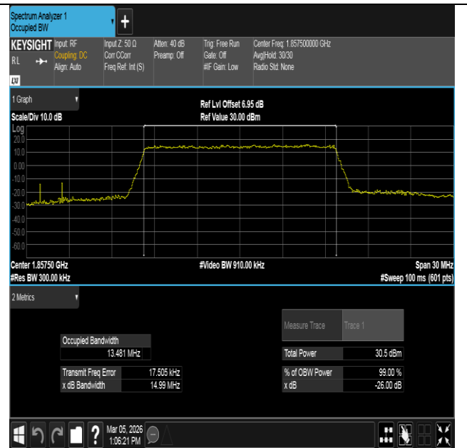
Band2-15MHz-16QAM-18675-75RB#0-PASS
