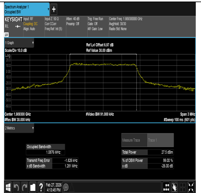
Band2-1.4MHz-16QAM-19193-6RB#0-PASS
