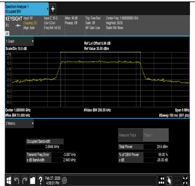
Band2-3MHz-16QAM-18900-15RB#0-PASS
