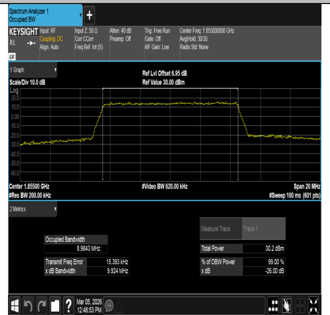
Band2-10MHz-16QAM-18650-50RB#0-PASS
