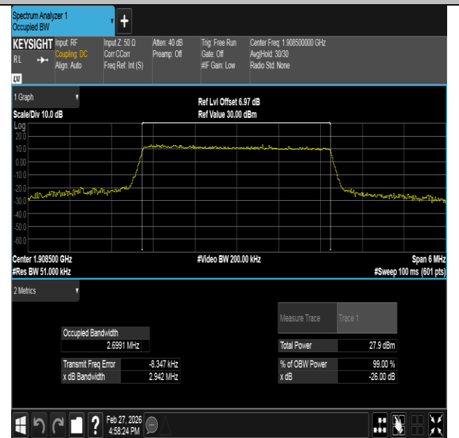
Band2-3MHz-16QAM-19185-15RB#0-PASS
