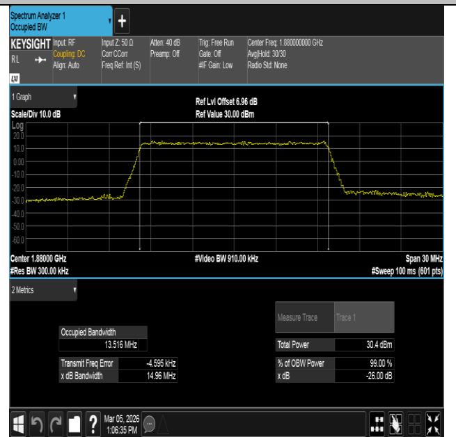
Band2-15MHz-16QAM-18900-75RB#0-PASS
