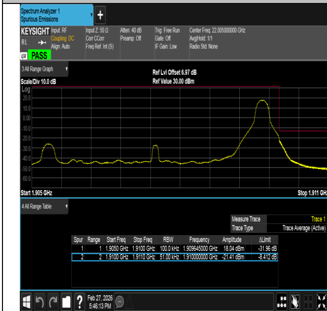
Band2-5MHz-16QAM-19175-1RB#24-PASS
