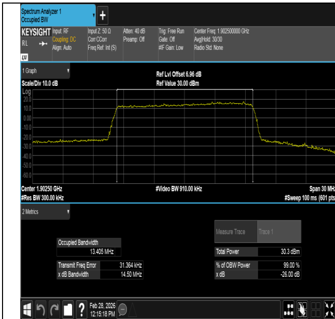
Band2-15MHz-QPSK-19125-75RB#0-PASS
