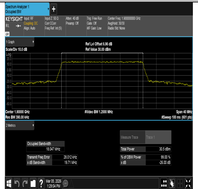
Band2-20MHz-16QAM-19100-100RB#0-PASS
