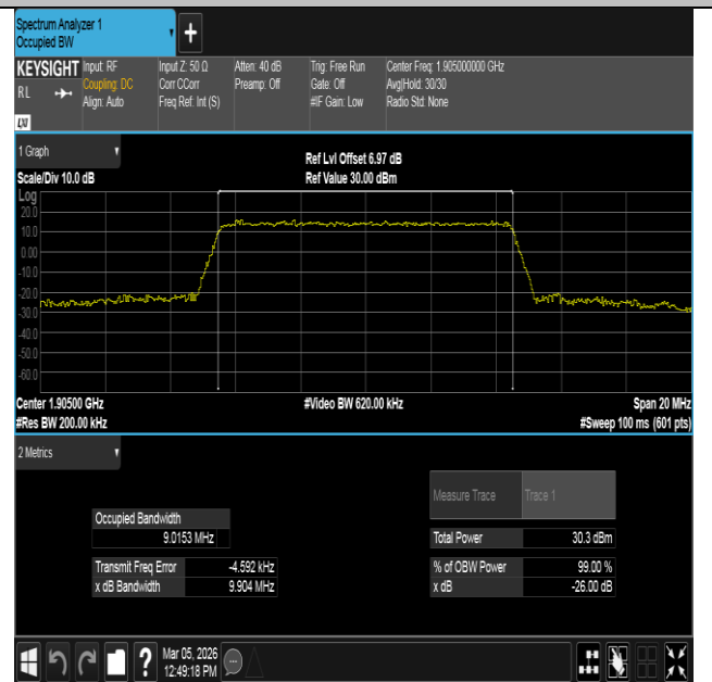
Band2-10MHz-16QAM-19150-50RB#0-PASS
