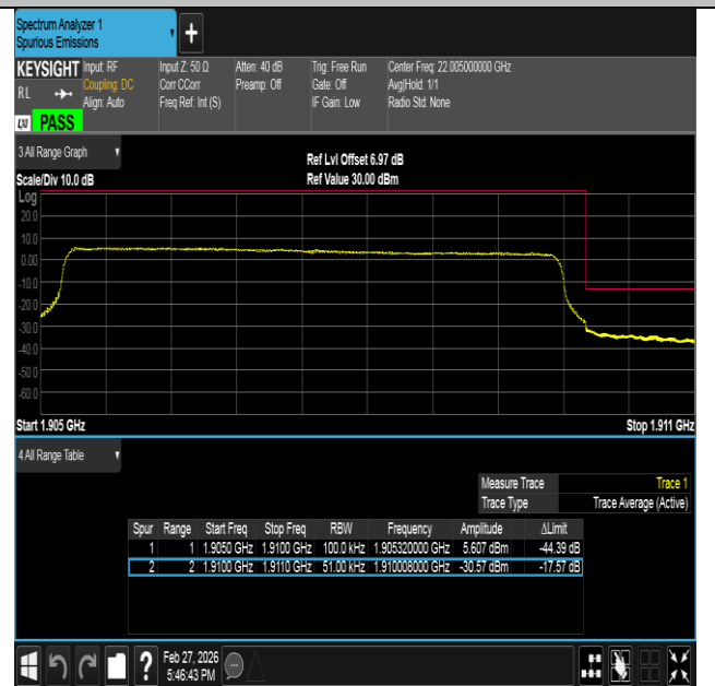
Band2-5MHz-16QAM-19175-25RB#0-PASS
