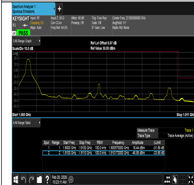
Band2-10MHz-QPSK-19150-1RB#0-PASS
