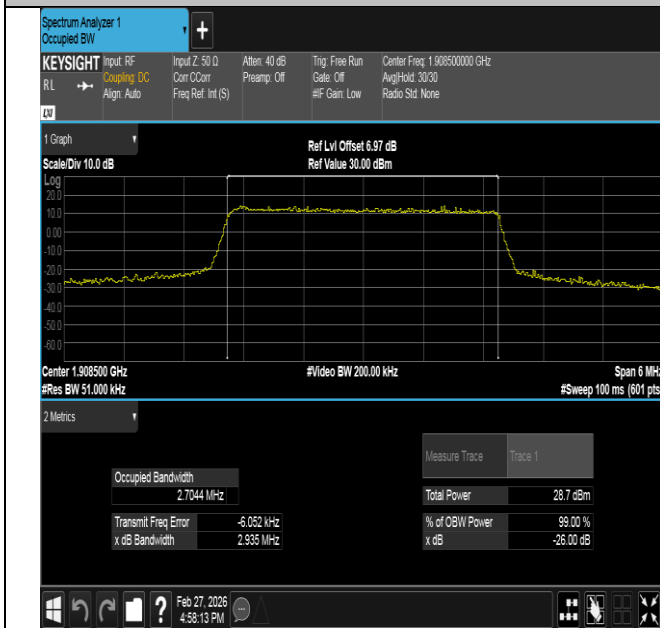
Band2-3MHz-QPSK-19185-15RB#0-PASS
