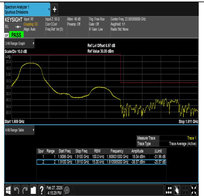
Band2-1.4MHz-16QAM-19193-1RB#0-PASS
