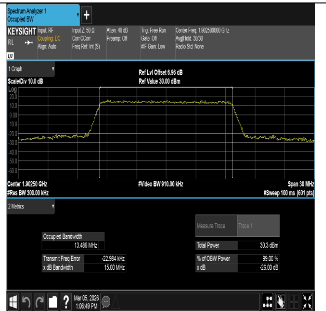
Band2-15MHz-16QAM-19125-75RB#0-PASS
