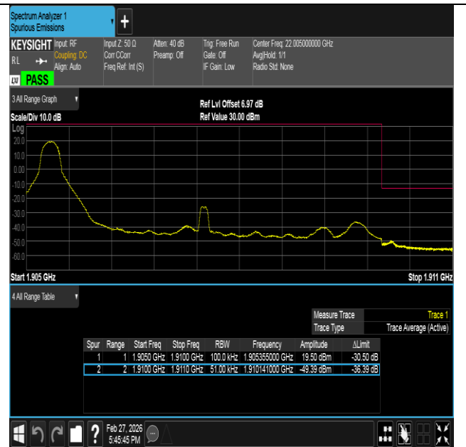
Band2-5MHz-16QAM-19175-1RB#0-PASS
