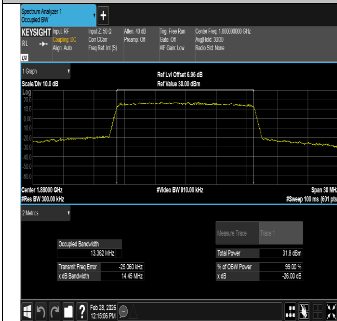
Band2-15MHz-QPSK-18900-75RB#0-PASS
