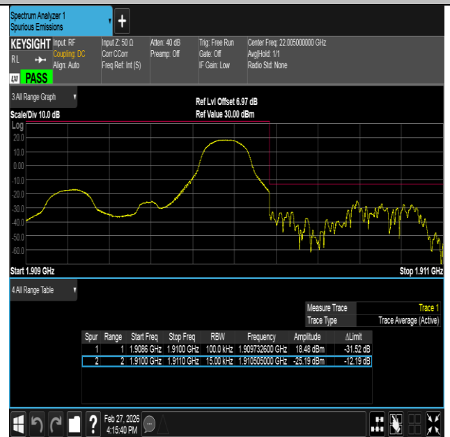
Band2-1.4MHz-QPSK-19193-1RB#5-PASS
