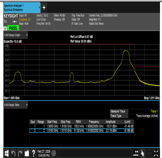
Band2-5MHz-QPSK-19175-1RB#24-PASS
