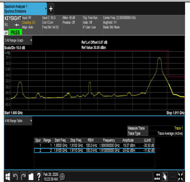
Band2-10MHz-QPSK-19150-1RB#49-PASS
