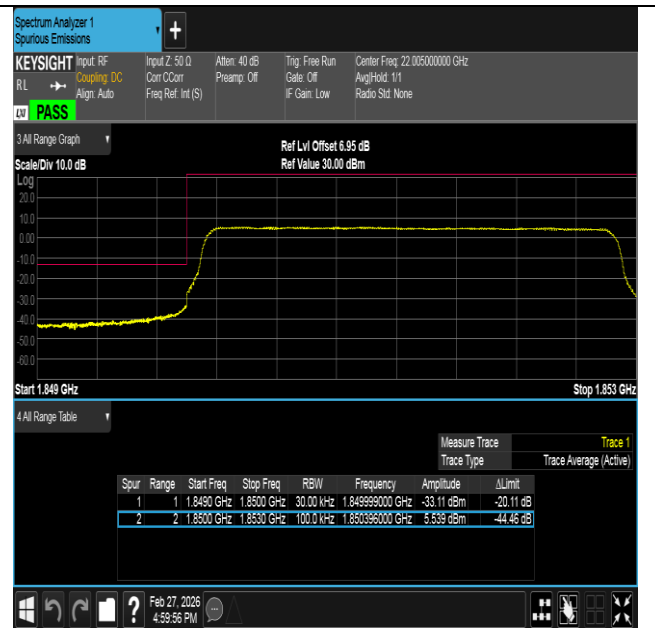
Band2-3MHz-16QAM-18615-15RB#0-PASS
