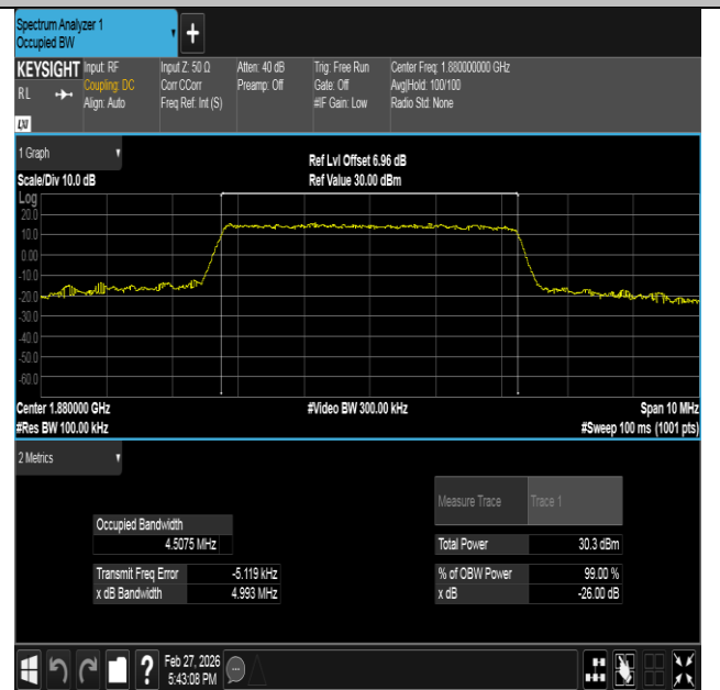
Band2-5MHz-16QAM-18900-25RB#0-PASS
