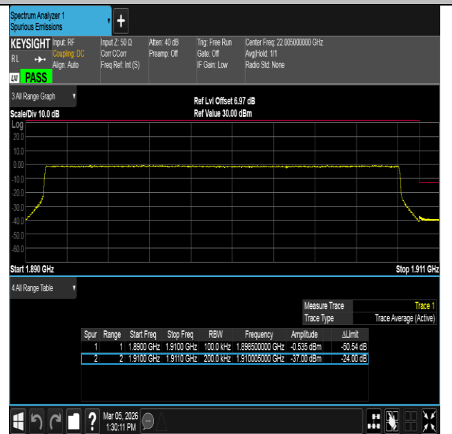
Band2-20MHz-16QAM-19100-100RB#0-PASS
