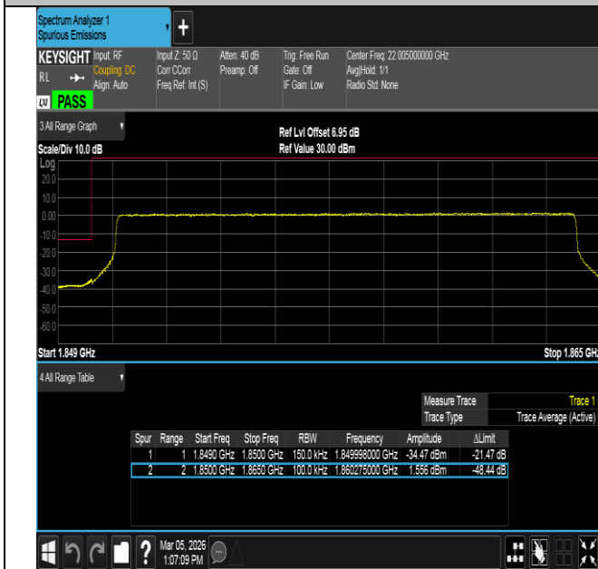
Band2-15MHz-QPSK-18675-75RB#0-PASS
