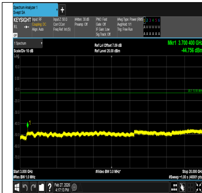
Band2-1.4MHz-QPSK-18607-1RB#0-3000~20000-PASS
