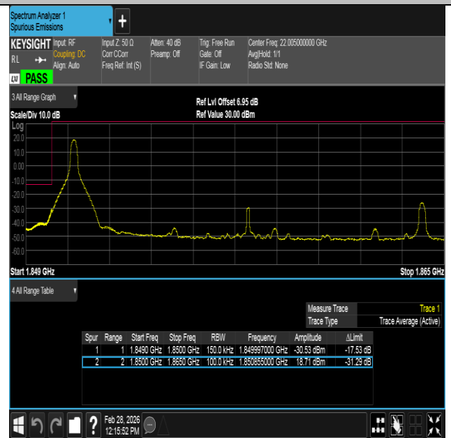
Band2-15MHz-16QAM-18675-1RB#0-PASS
