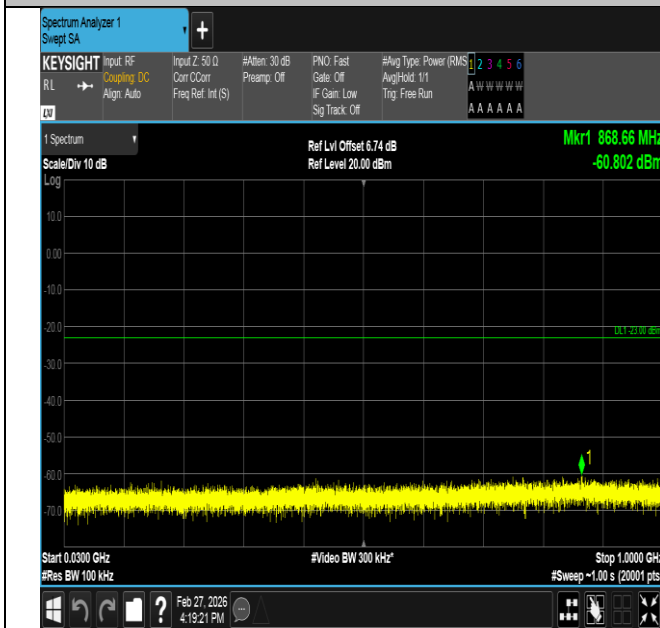
Band2-1.4MHz-16QAM-18607-1RB#5-30~1000-PASS
