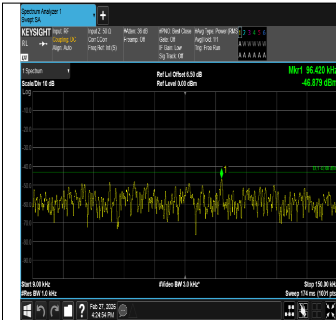
Band2-1.4MHz-QPSK-18900-6RB#0-0.009~0.15-PASS
