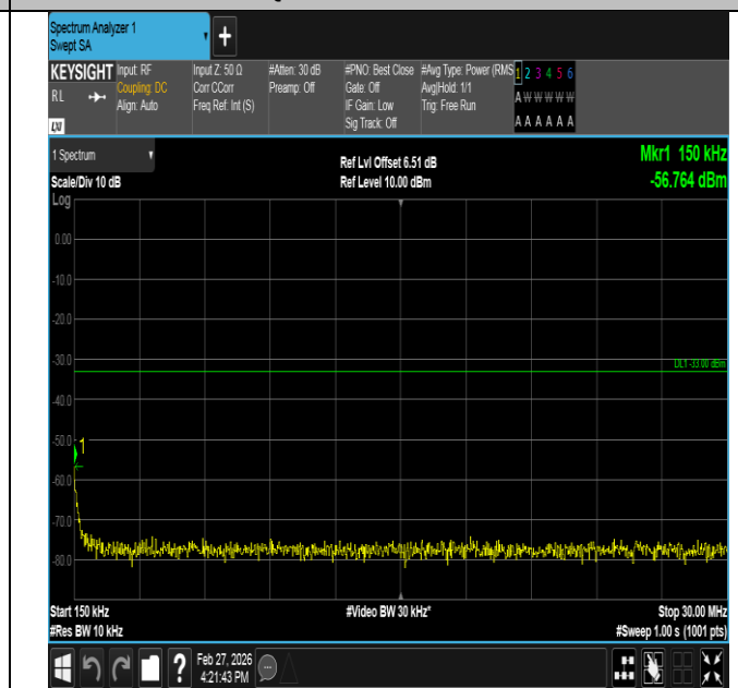
Band2-1.4MHz-QPSK-18900-1RB#0-0.15~30-PASS
