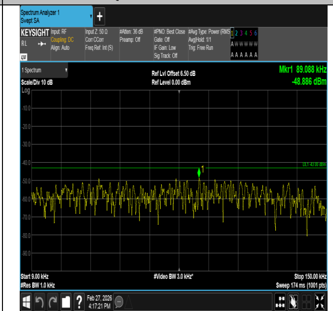
Band2-1.4MHz-16QAM-18607-1RB#0-0.009~0.15-PASS
