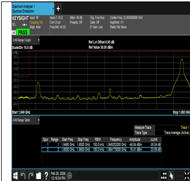
Band2-15MHz-16QAM-18675-1RB#74-PASS
