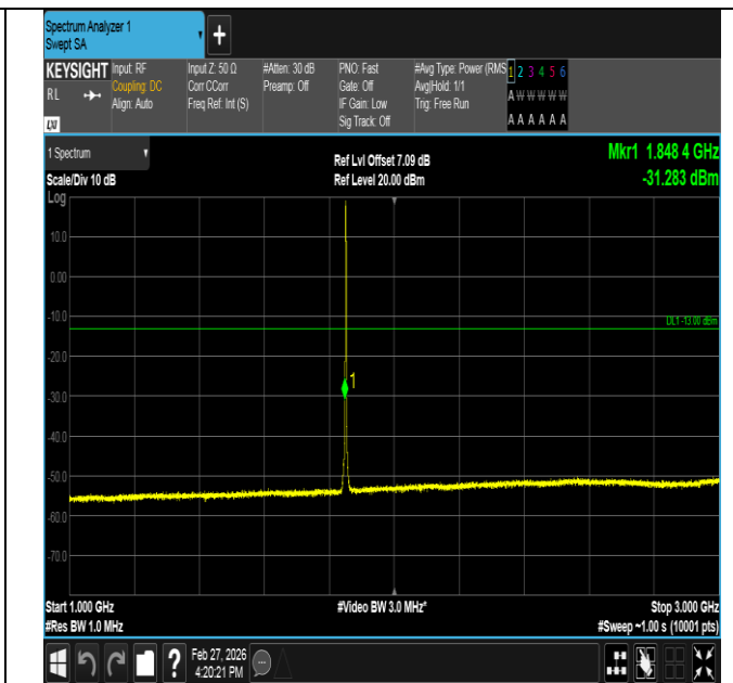
Band2-1.4MHz-QPSK-18607-6RB#0-1000~3000-PASS
