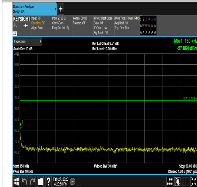
Band2-1.4MHz-16QAM-18607-6RB#0-0.15~30-PASS
