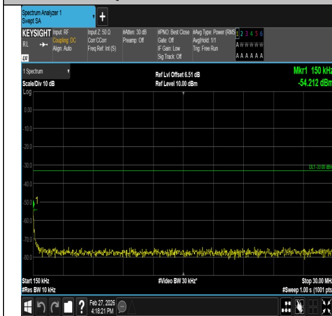
Band2-1.4MHz-QPSK-18607-1RB#5-0.15~30-PASS
