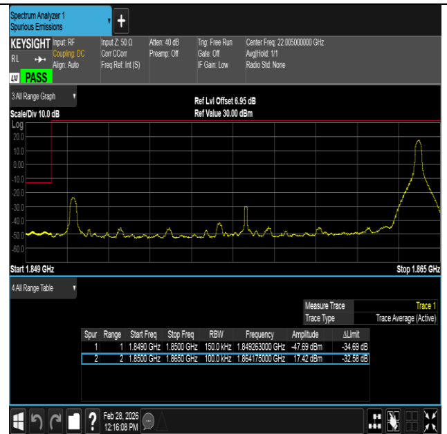
Band2-15MHz-QPSK-18675-1RB#74-PASS
