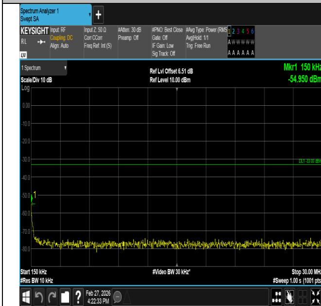
Band2-1.4MHz-16QAM-18900-1RB#0-0.15~30-PASS
