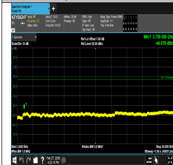
Band2-1.4MHz-QPSK-18900-1RB#0-3000~20000-PASS
