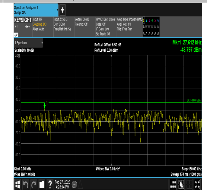
Band2-1.4MHz-QPSK-18900-1RB#5-0.009~0.15-PASS
