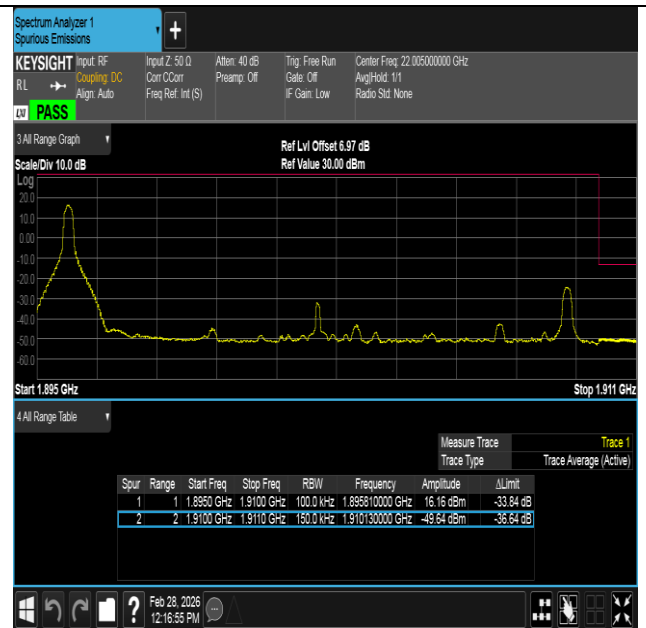
Band2-15MHz-16QAM-19125-1RB#0-PASS
