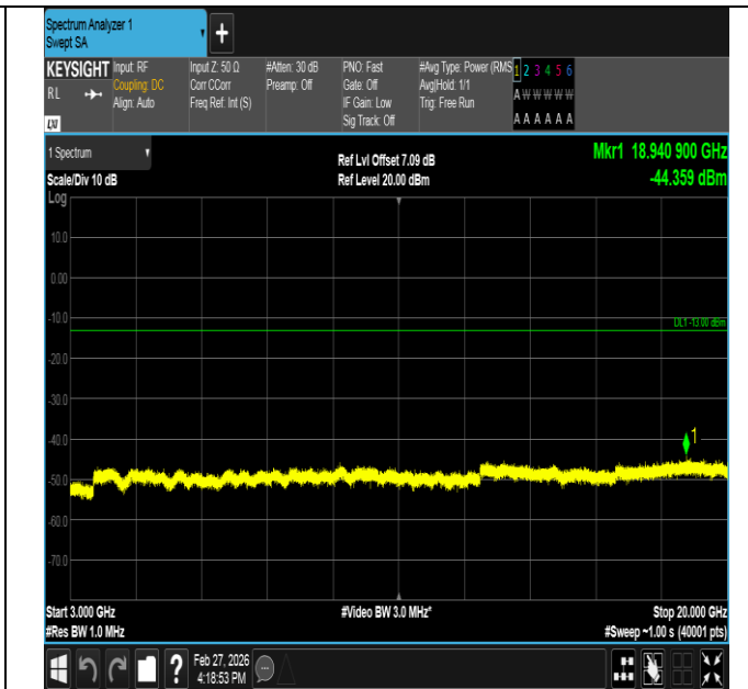
Band2-1.4MHz-QPSK-18607-1RB#5-3000~20000-PASS
