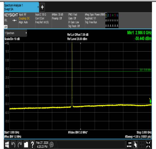
Band2-1.4MHz-QPSK-18900-6RB#0-1000~3000-PASS
