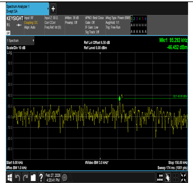
Band2-1.4MHz-16QAM-18607-6RB#0-0.009~0.15-PASS
