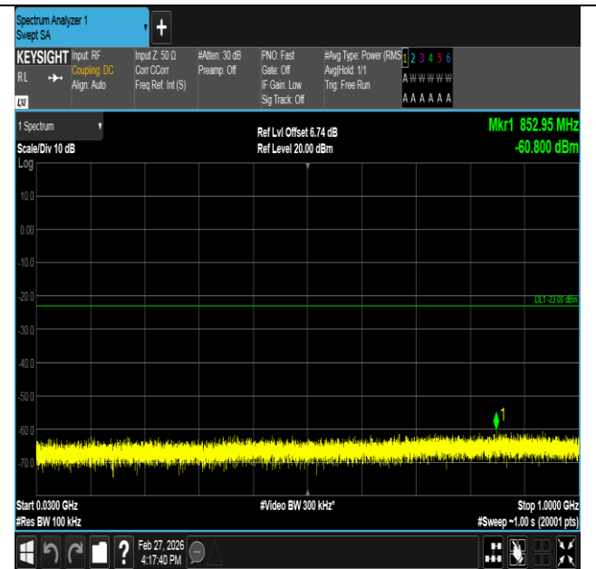
Band2-1.4MHz-16QAM-18607-1RB#0-30~1000-PASS
