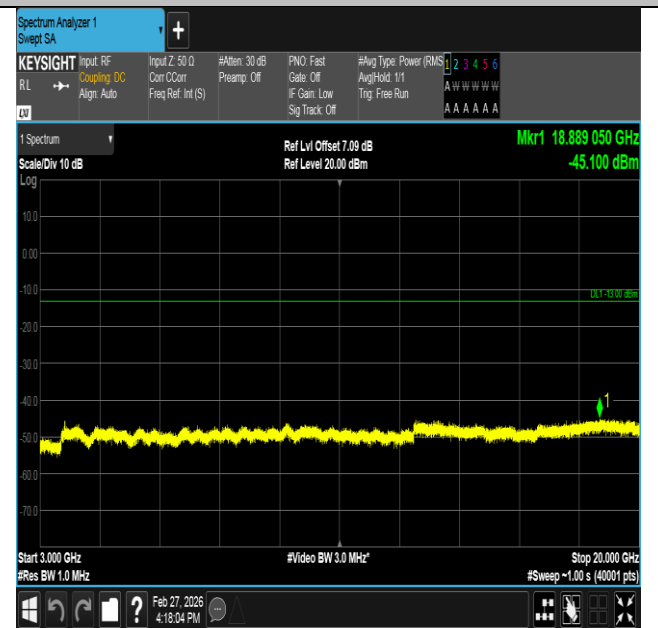
Band2-1.4MHz-16QAM-18607-1RB#0-3000~20000-PASS
