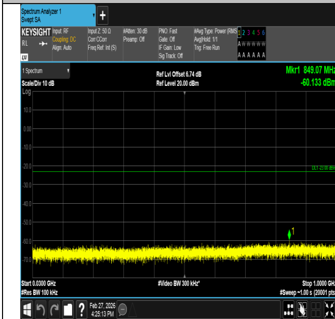
Band2-1.4MHz-QPSK-18900-6RB#0-30~1000-PASS
