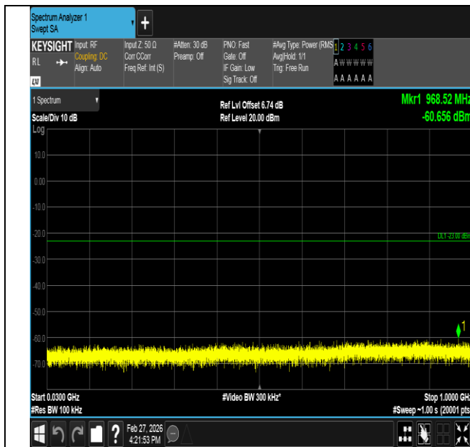
Band2-1.4MHz-QPSK-18900-1RB#0-30~1000-PASS
