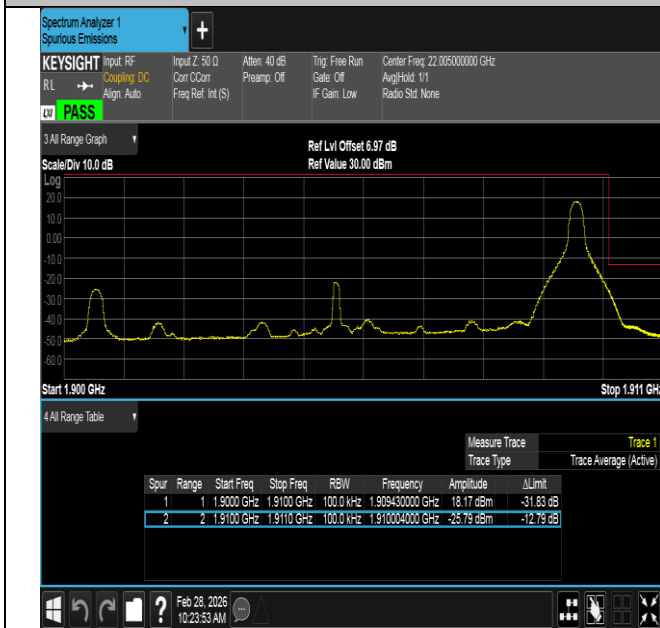
Band2-10MHz-16QAM-19150-1RB#49-PASS
