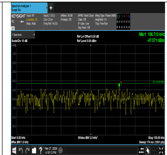
Band2-1.4MHz-QPSK-18607-1RB#5-0.009~0.15-PASS
