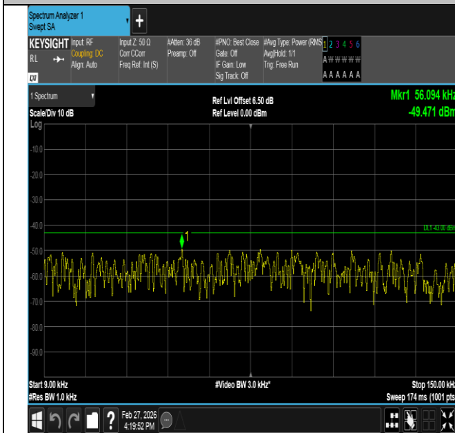
Band2-1.4MHz-QPSK-18607-6RB#0-0.009~0.15-PASS
