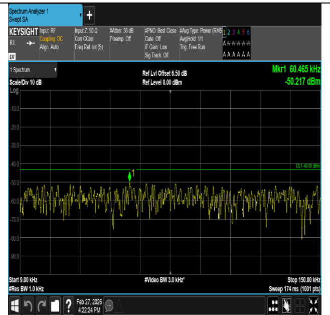
Band2-1.4MHz-16QAM-18900-1RB#0-0.009~0.15-PASS
