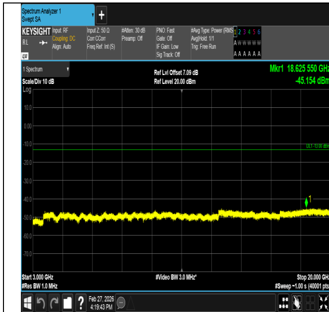
Band2-1.4MHz-16QAM-18607-1RB#5-3000~20000-PASS
