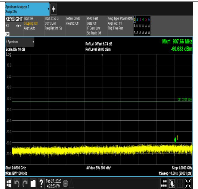
Band2-1.4MHz-QPSK-18900-1RB#5-30~1000-PASS
