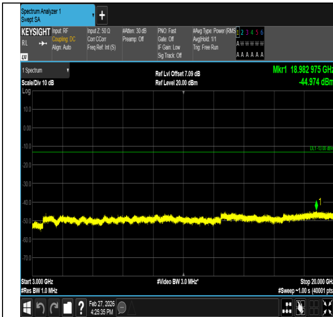
Band2-1.4MHz-QPSK-18900-6RB#0-3000~20000-PASS
