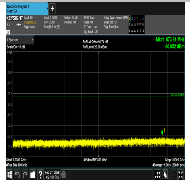
Band2-1.4MHz-16QAM-18607-6RB#0-30~1000-PASS
