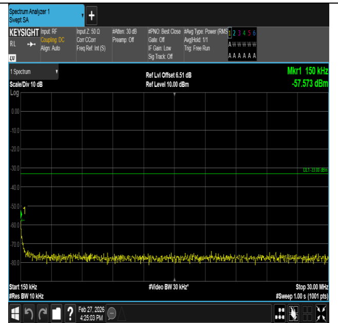
Band2-1.4MHz-QPSK-18900-6RB#0-0.15~30-PASS
