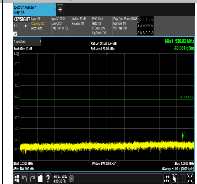
Band2-1.4MHz-QPSK-18607-1RB#5-30~1000-PASS
