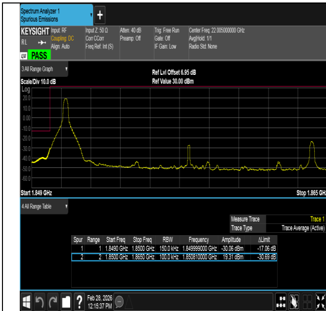
Band2-15MHz-QPSK-18675-1RB#0-PASS
