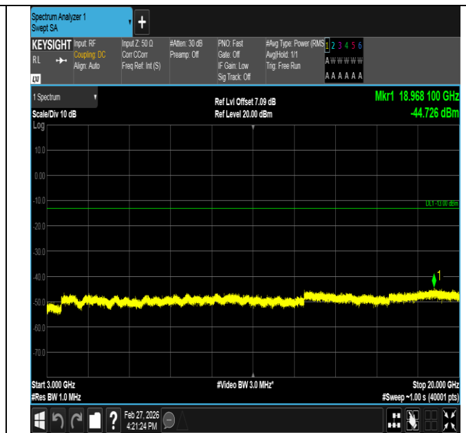
Band2-1.4MHz-16QAM-18607-6RB#0-3000~20000-PASS
