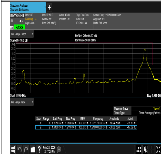
Band2-15MHz-16QAM-19125-1RB#74-PASS
