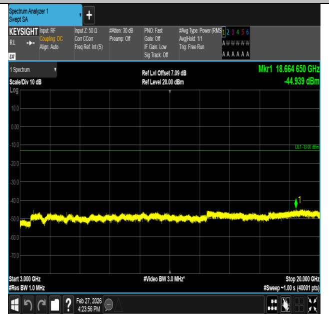
Band2-1.4MHz-QPSK-18900-1RB#5-3000~20000-PASS
