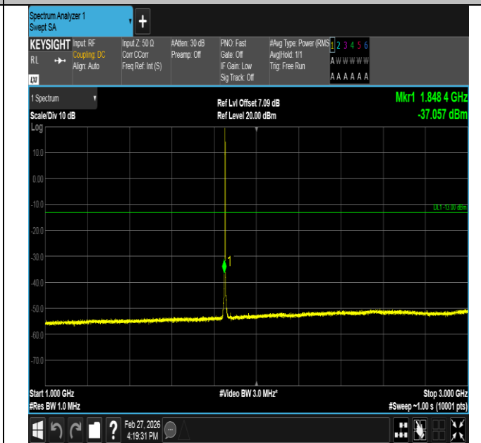
Band2-1.4MHz-16QAM-18607-1RB#5-1000~3000-PASS
