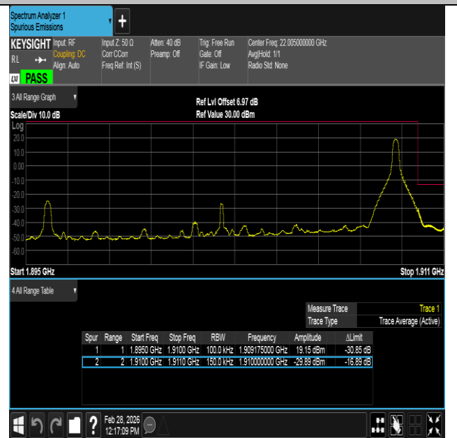
Band2-15MHz-QPSK-19125-1RB#74-PASS
