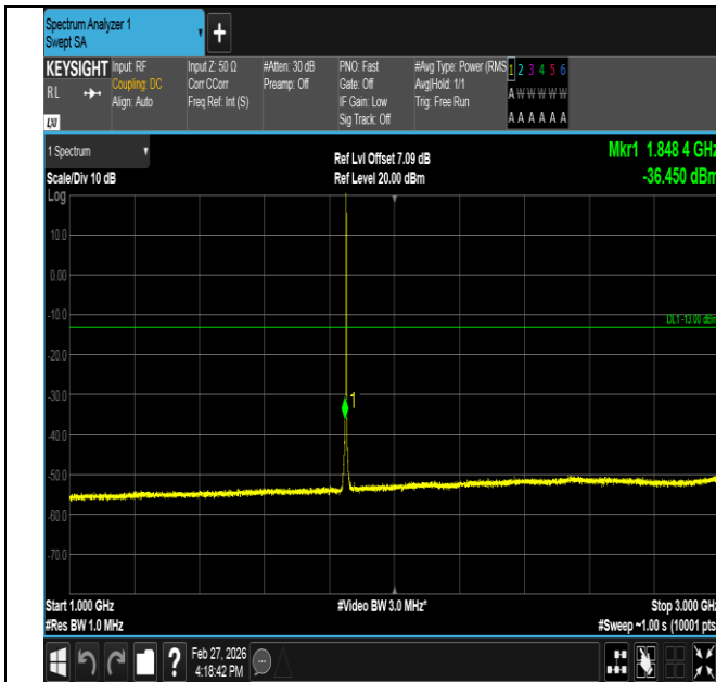
Band2-1.4MHz-QPSK-18607-1RB#5-1000~3000-PASS
