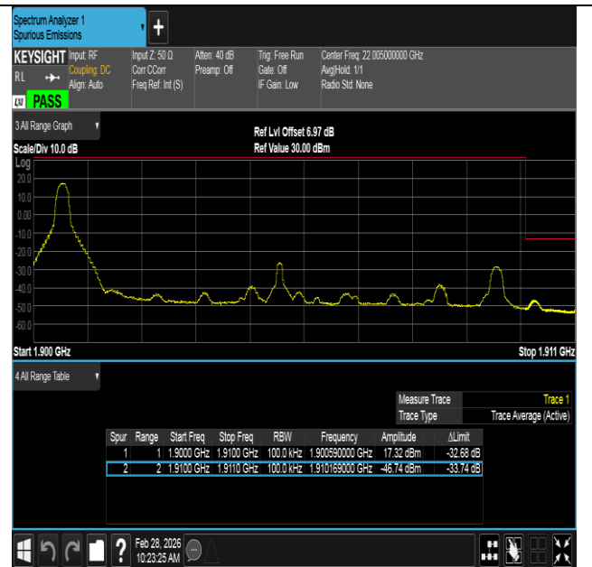
Band2-10MHz-16QAM-19150-1RB#0-PASS
