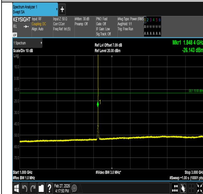
Band2-1.4MHz-16QAM-18607-1RB#0-1000~3000-PASS
