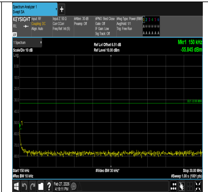
Band2-1.4MHz-16QAM-18607-1RB#5-0.15~30-PASS
