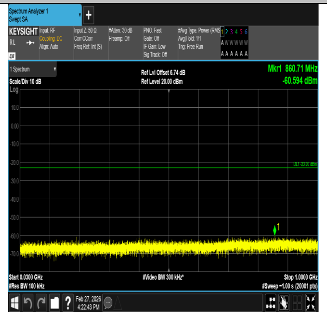
Band2-1.4MHz-16QAM-18900-1RB#0-30~1000-PASS
