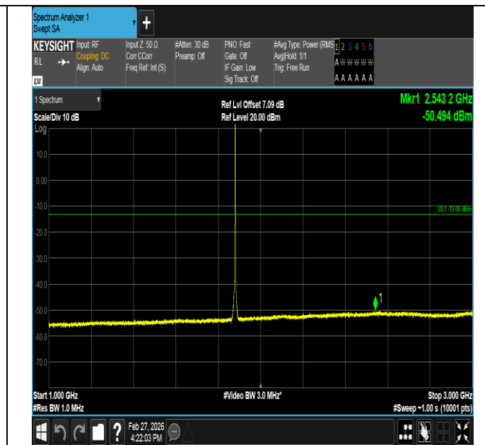
Band2-1.4MHz-QPSK-18900-1RB#0-1000~3000-PASS
