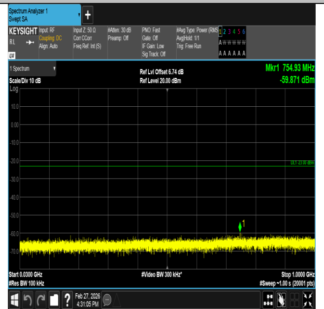
Band2-1.4MHz-16QAM-19193-6RB#0-30~1000-PASS
