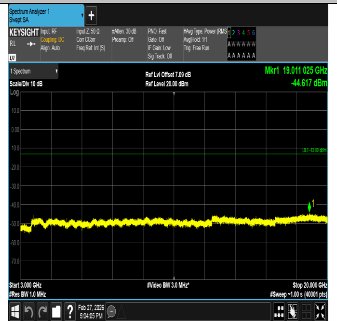
Band2-3MHz-QPSK-18615-1RB#14-3000~20000-PASS
