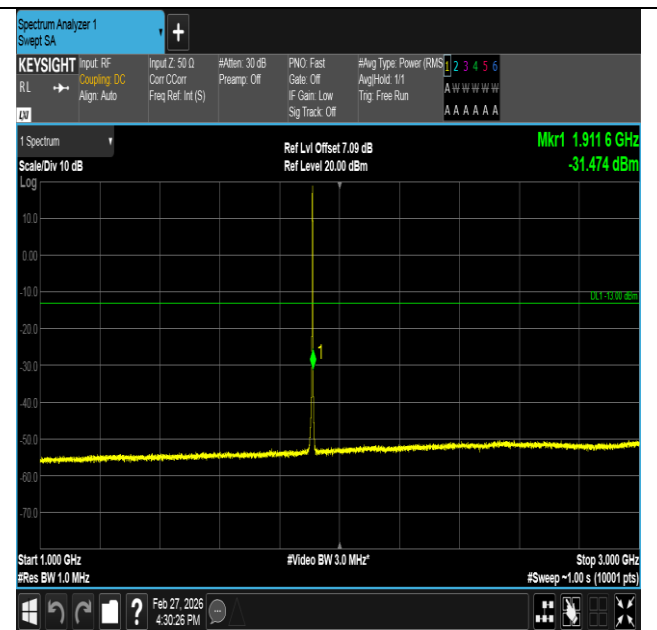
Band2-1.4MHz-QPSK-19193-6RB#0-1000~3000-PASS
