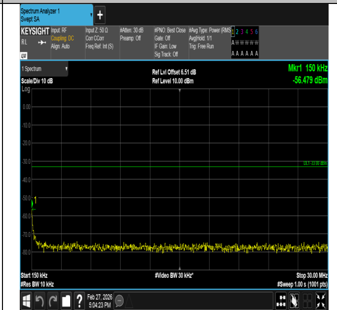
Band2-3MHz-16QAM-18615-1RB#14-0.15~30-PASS
