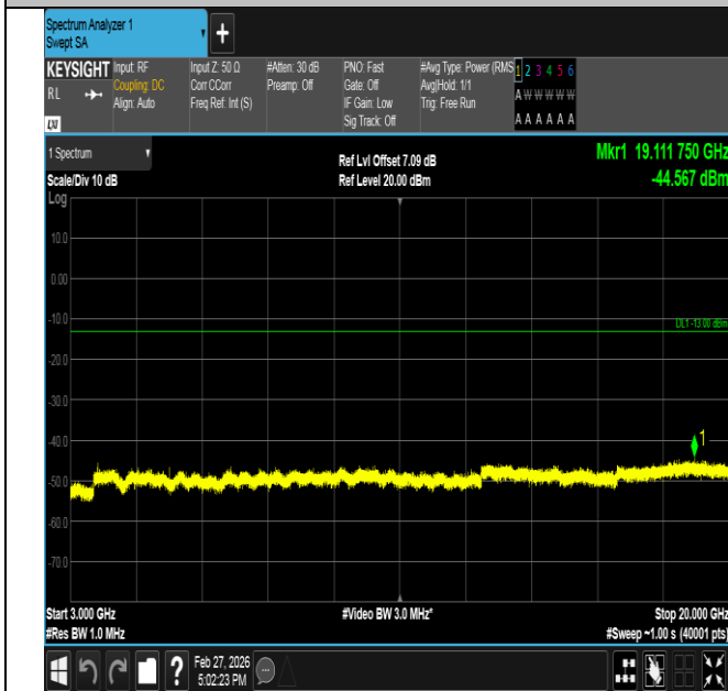
Band2-3MHz-QPSK-18615-1RB#0-3000~20000-PASS
