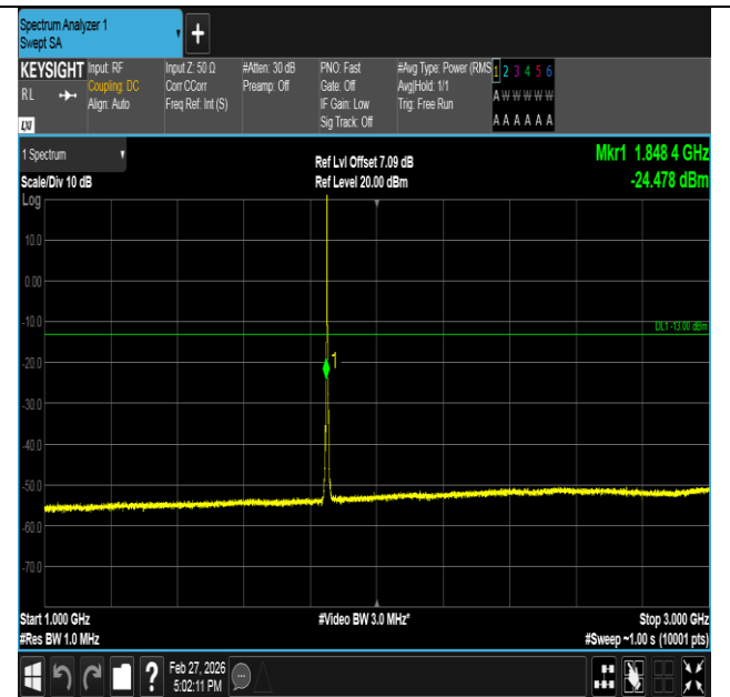
Band2-3MHz-QPSK-18615-1RB#0-1000~3000-PASS
