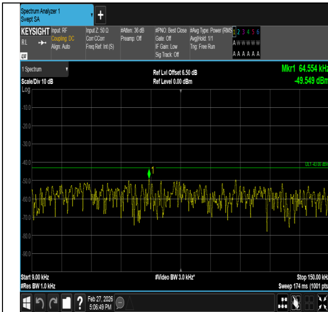
Band2-3MHz-QPSK-18900-1RB#0-0.009~0.15-PASS
