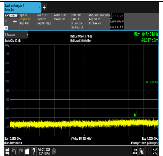
Band2-1.4MHz-16QAM-19193-1RB#0-30~1000-PASS
