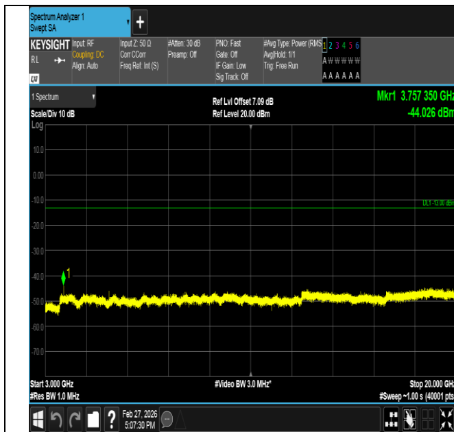
Band2-3MHz-QPSK-18900-1RB#0-3000~20000-PASS
