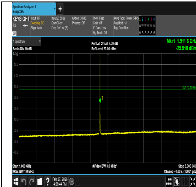
Band2-1.4MHz-QPSK-19193-1RB#5-1000~3000-PASS
