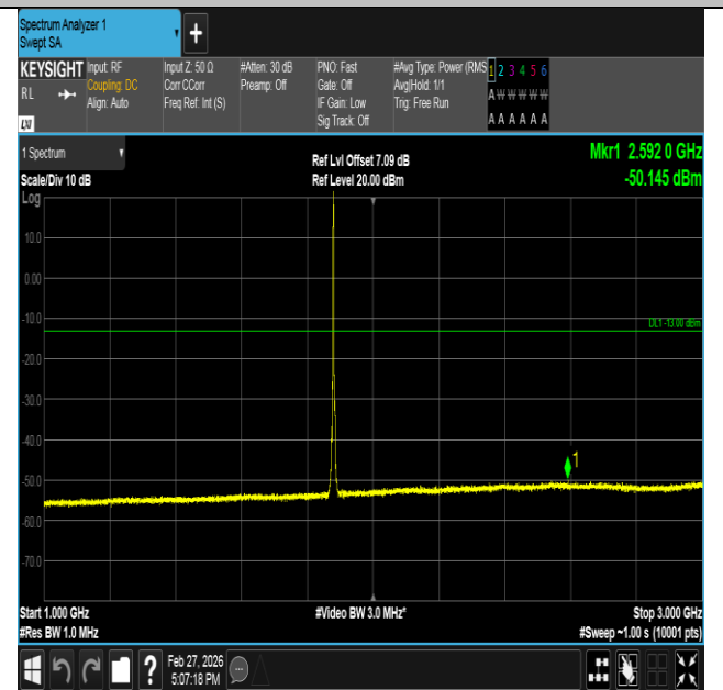
Band2-3MHz-QPSK-18900-1RB#0-1000~3000-PASS
