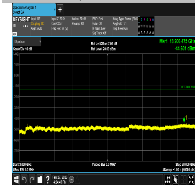
Band2-1.4MHz-16QAM-18900-1RB#5-3000~20000-PASS
