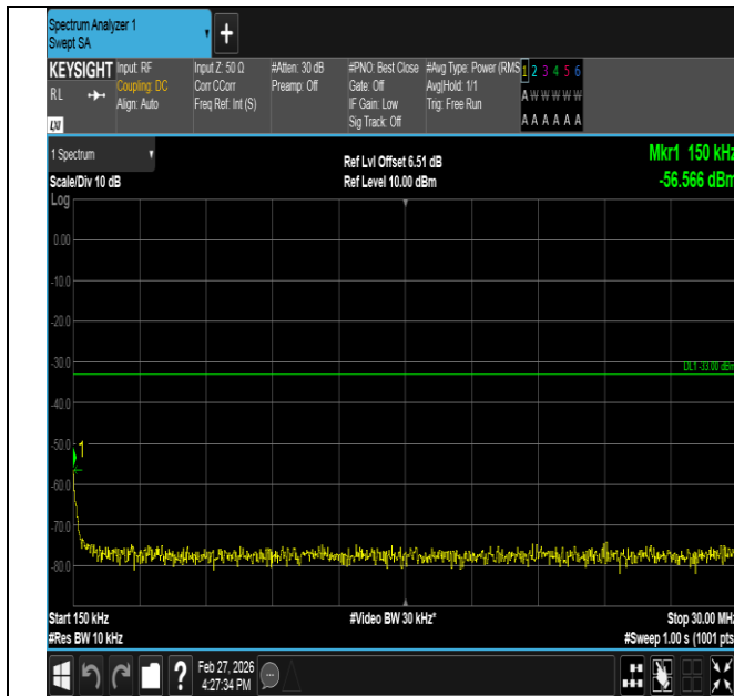
Band2-1.4MHz-16QAM-19193-1RB#0-0.15~30-PASS
