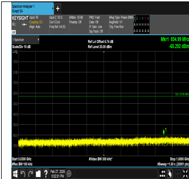
Band2-3MHz-QPSK-18615-1RB#0-30~1000-PASS
