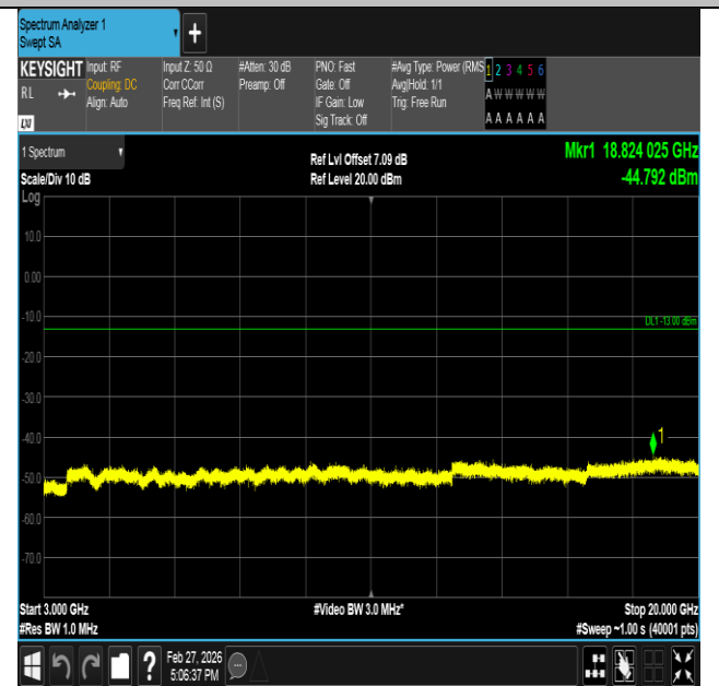
Band2-3MHz-16QAM-18615-15RB#0-3000~20000-PASS
