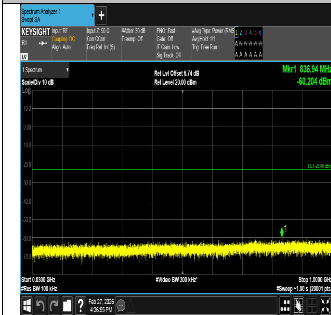
Band2-1.4MHz-QPSK-19193-1RB#0-30~1000-PASS
