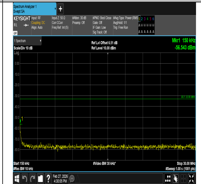
Band2-1.4MHz-QPSK-19193-6RB#0-0.15~30-PASS
