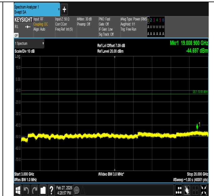
Band2-1.4MHz-QPSK-19193-1RB#5-3000~20000-PASS
