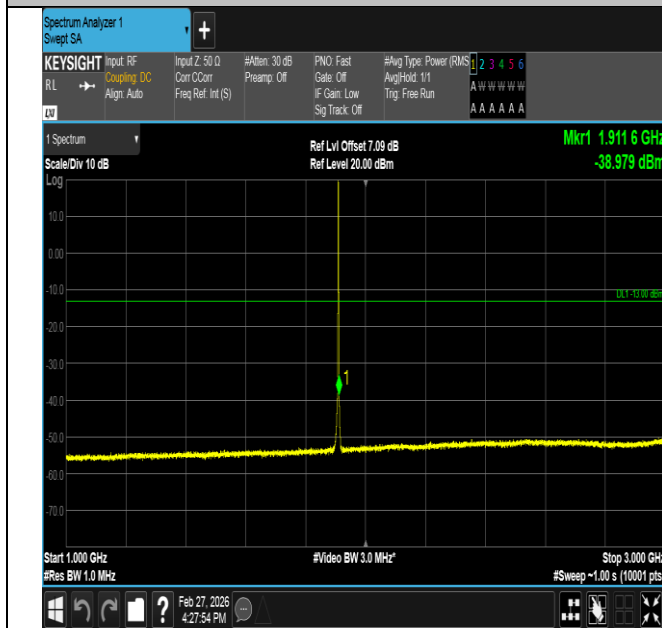
Band2-1.4MHz-16QAM-19193-1RB#0-1000~3000-PASS
