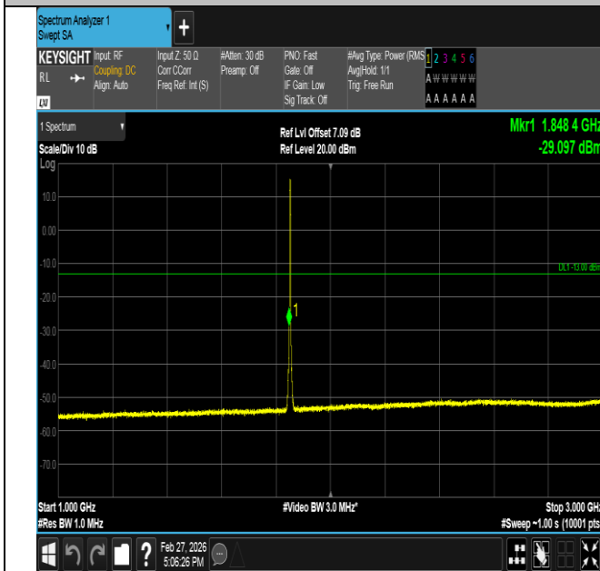
Band2-3MHz-16QAM-18615-15RB#0-1000~3000-PASS
