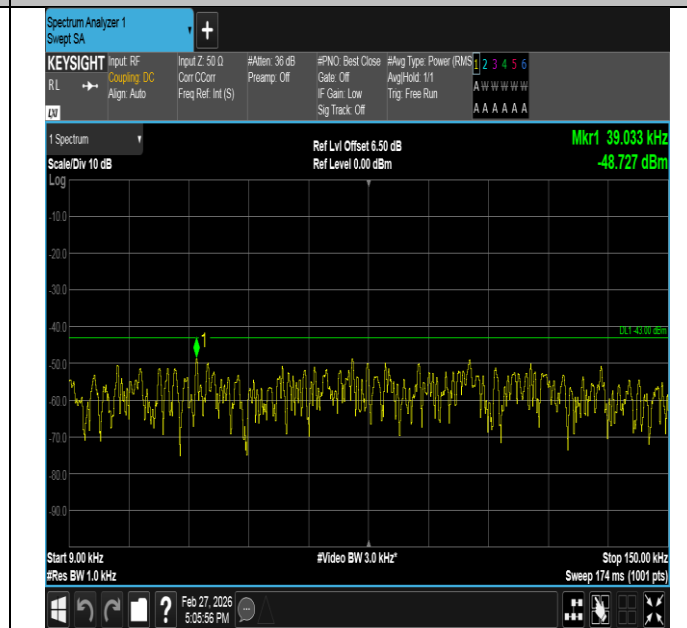
Band2-3MHz-16QAM-18615-15RB#0-0.009~0.15-PASS
