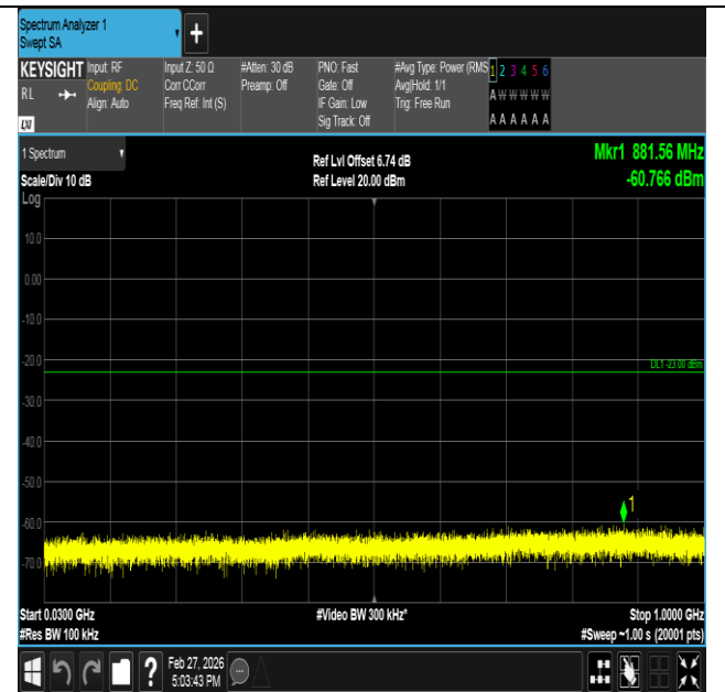
Band2-3MHz-QPSK-18615-1RB#14-30~1000-PASS
