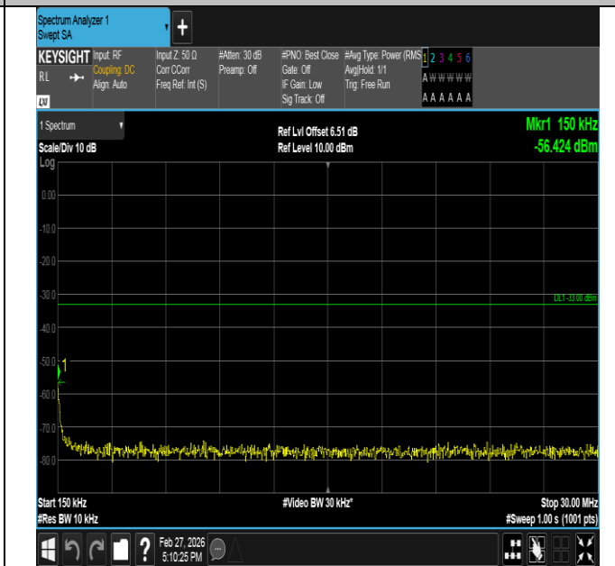
Band2-3MHz-QPSK-18900-15RB#0-0.15~30-PASS
