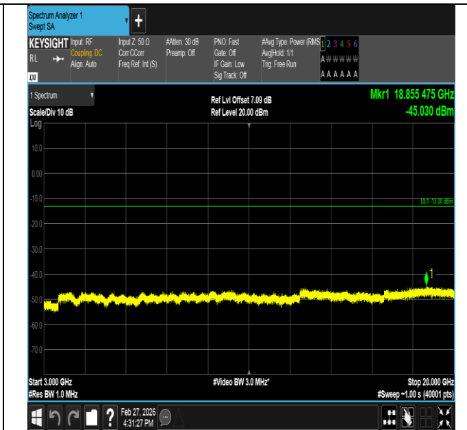
Band2-1.4MHz-16QAM-19193-6RB#0-3000~20000-PASS
