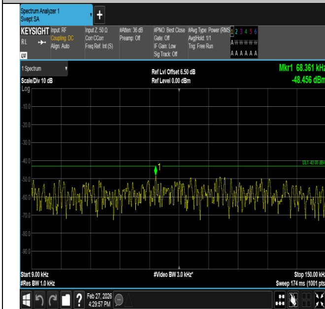
Band2-1.4MHz-QPSK-19193-6RB#0-0.009~0.15-PASS
