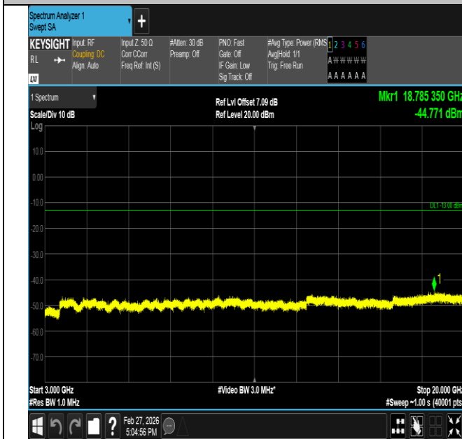
Band2-3MHz-16QAM-18615-1RB#14-3000~20000-PASS
