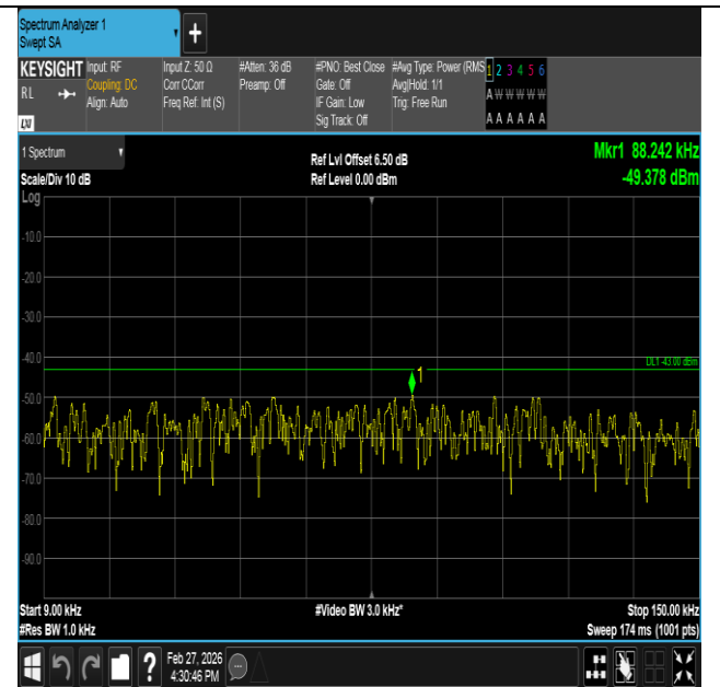
Band2-1.4MHz-16QAM-19193-6RB#0-0.009~0.15-PASS
