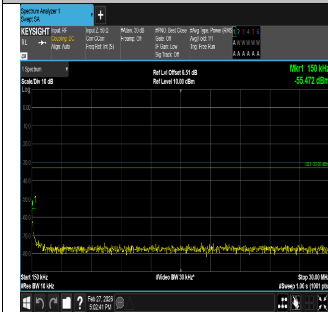
Band2-3MHz-16QAM-18615-1RB#0-0.15~30-PASS
