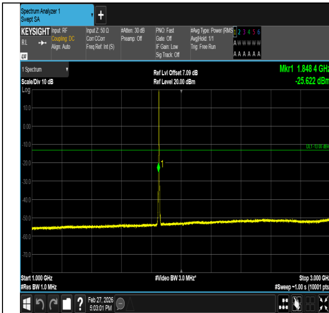
Band2-3MHz-16QAM-18615-1RB#0-1000~3000-PASS
