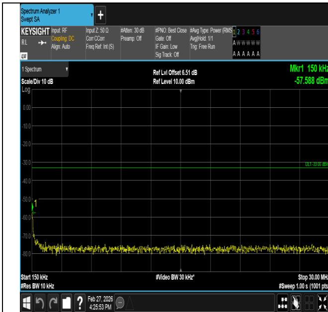
Band2-1.4MHz-16QAM-18900-6RB#0-0.15~30-PASS
