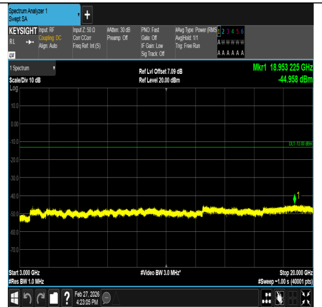
Band2-1.4MHz-16QAM-18900-1RB#0-3000~20000-PASS
