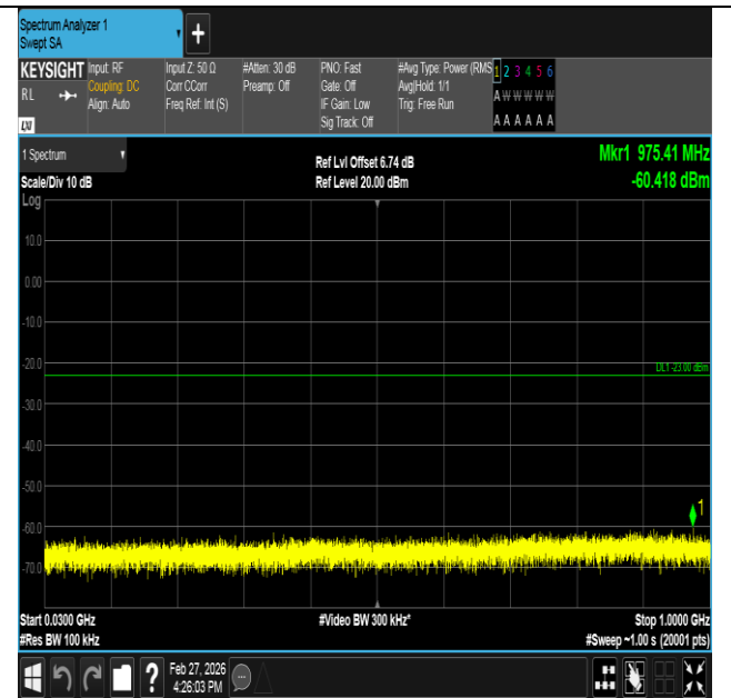
Band2-1.4MHz-16QAM-18900-6RB#0-30~1000-PASS
