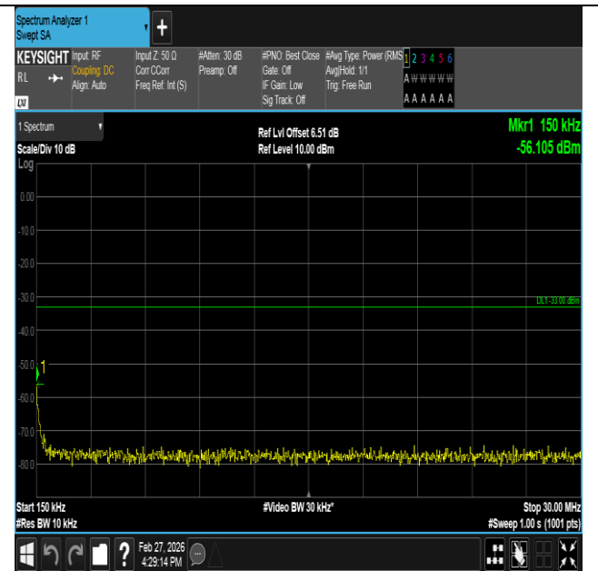
Band2-1.4MHz-16QAM-19193-1RB#5-0.15~30-PASS
