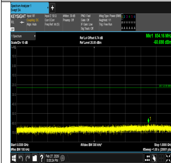
Band2-3MHz-QPSK-18615-15RB#0-30~1000-PASS
