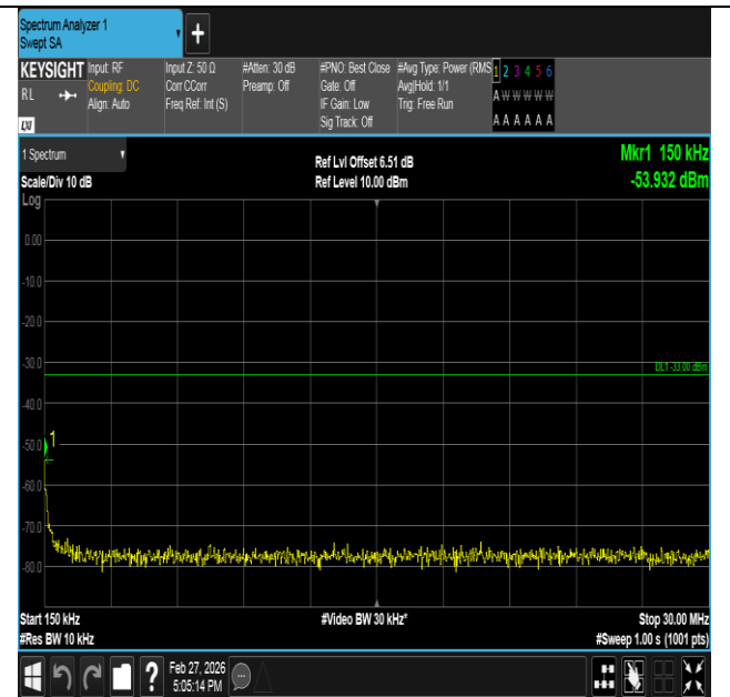
Band2-3MHz-QPSK-18615-15RB#0-0.15~30-PASS
