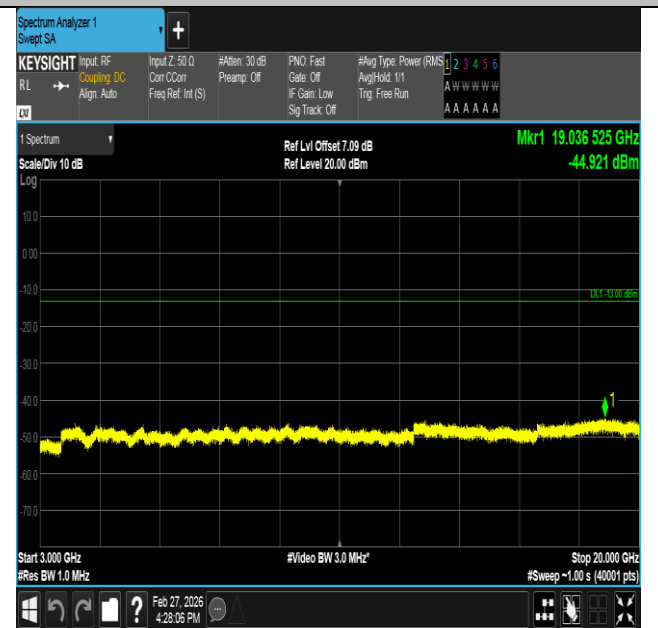
Band2-1.4MHz-16QAM-19193-1RB#0-3000~20000-PASS
