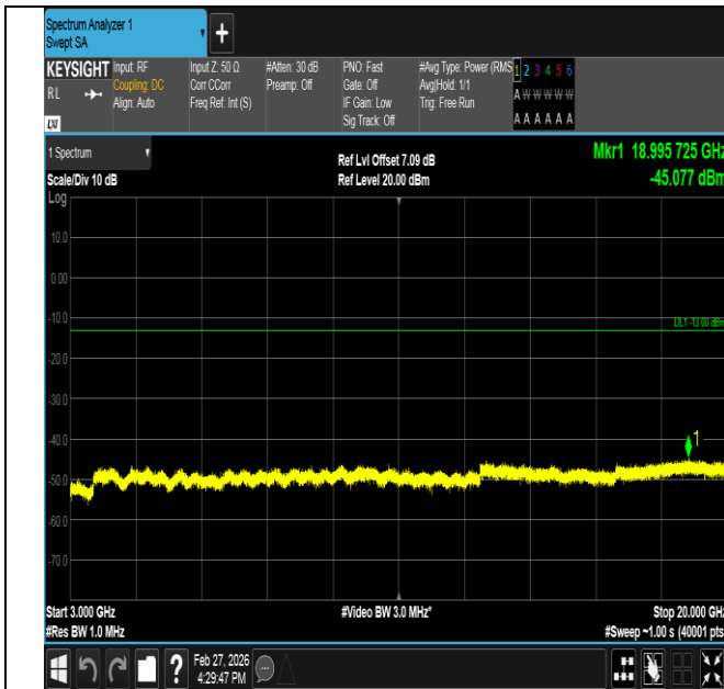
Band2-1.4MHz-16QAM-19193-1RB#5-3000~20000-PASS
