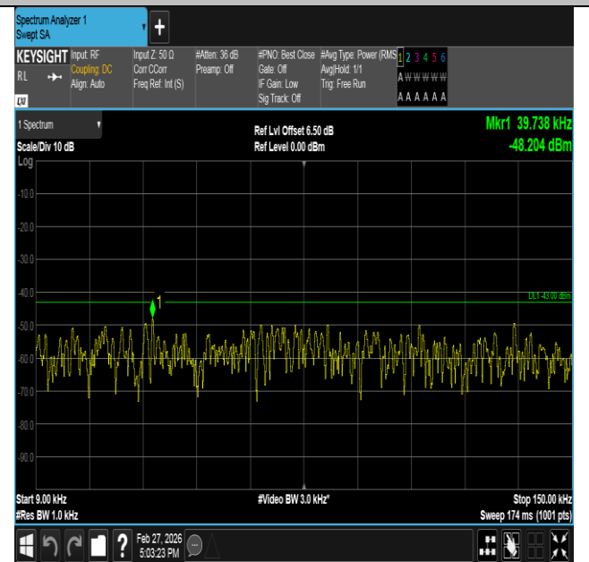
Band2-3MHz-QPSK-18615-1RB#14-0.009~0.15-PASS
