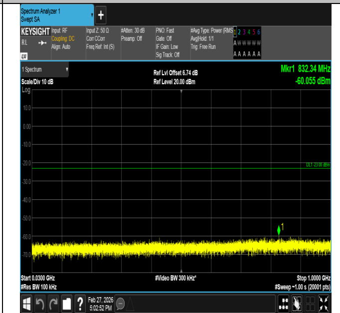
Band2-3MHz-16QAM-18615-1RB#0-30~1000-PASS
