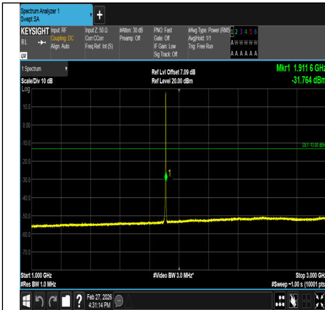
Band2-1.4MHz-16QAM-19193-6RB#0-1000~3000-PASS
