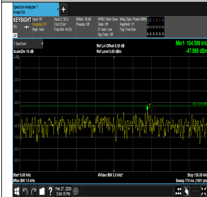
Band2-3MHz-16QAM-18615-1RB#14-0.009~0.15-PASS
