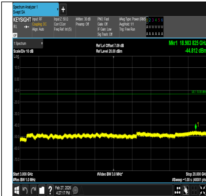
Band2-1.4MHz-QPSK-19193-1RB#0-3000~20000-PASS
