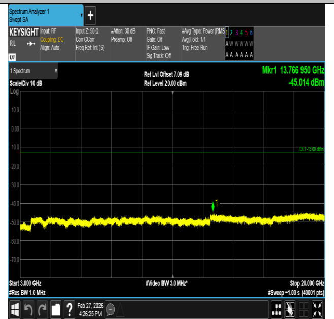
Band2-1.4MHz-16QAM-18900-6RB#0-3000~20000-PASS
