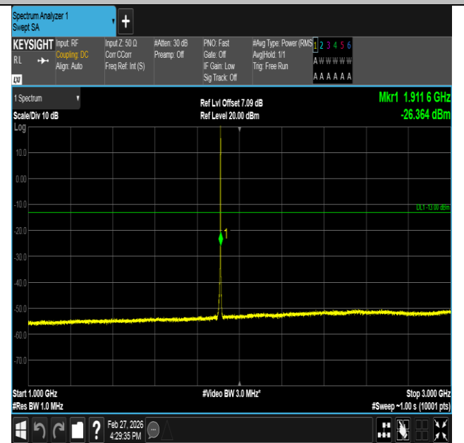
Band2-1.4MHz-16QAM-19193-1RB#5-1000~3000-PASS
