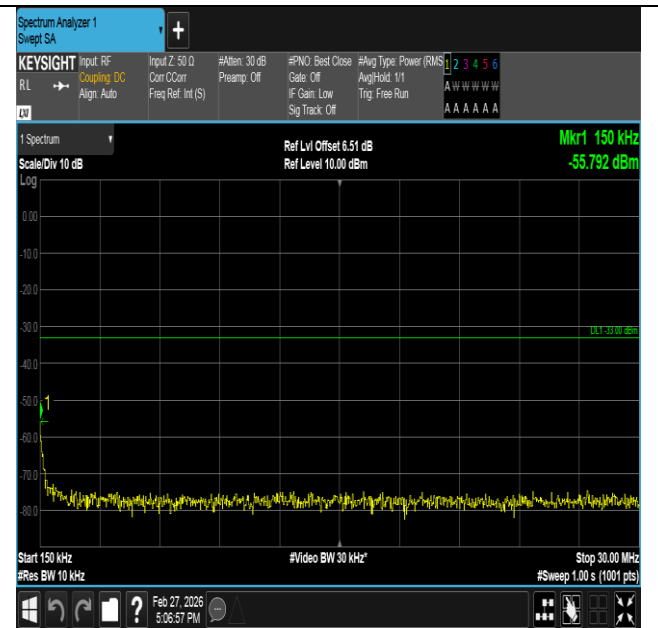
Band2-3MHz-QPSK-18900-1RB#0-0.15~30-PASS
