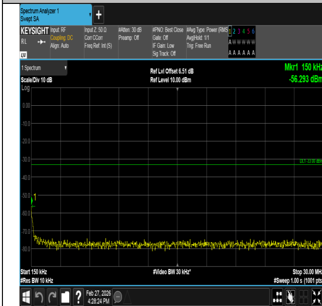
Band2-1.4MHz-QPSK-19193-1RB#5-0.15~30-PASS
