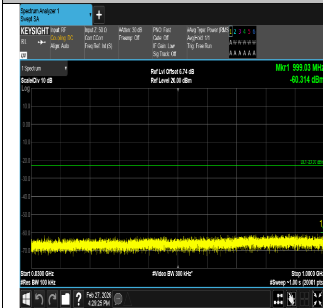
Band2-1.4MHz-16QAM-19193-1RB#5-30~1000-PASS
