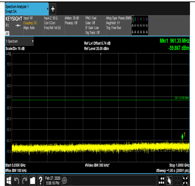
Band2-3MHz-16QAM-18615-15RB#0-30~1000-PASS
