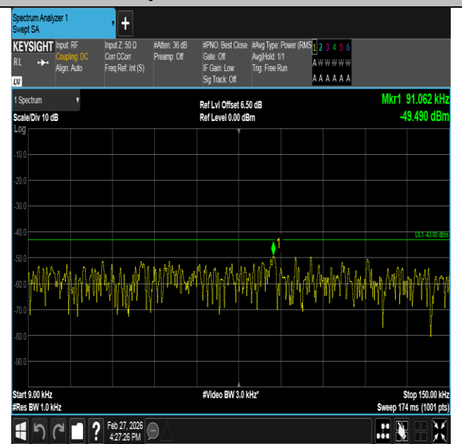
Band2-1.4MHz-16QAM-19193-1RB#0-0.009~0.15-PASS
