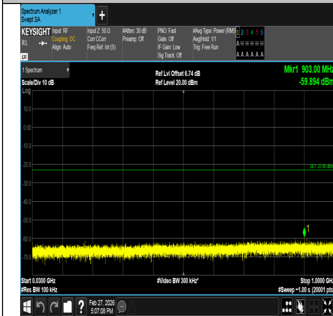
Band2-3MHz-QPSK-18900-1RB#0-30~1000-PASS
