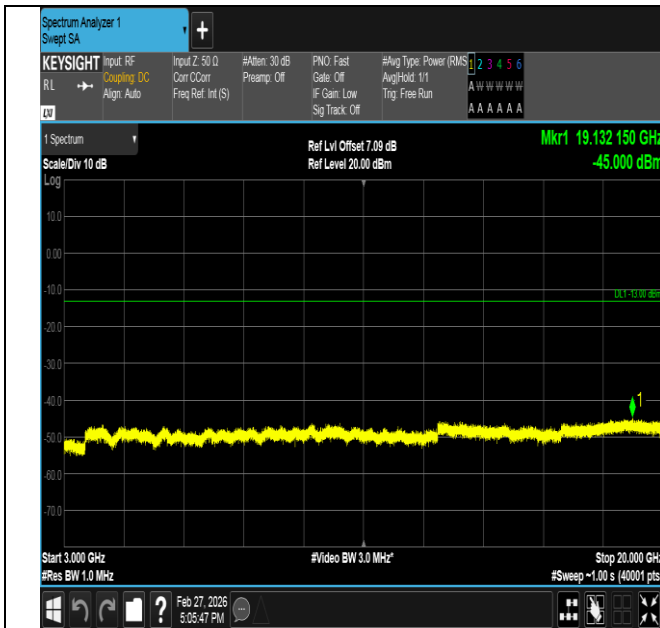
Band2-3MHz-QPSK-18615-15RB#0-3000~20000-PASS
