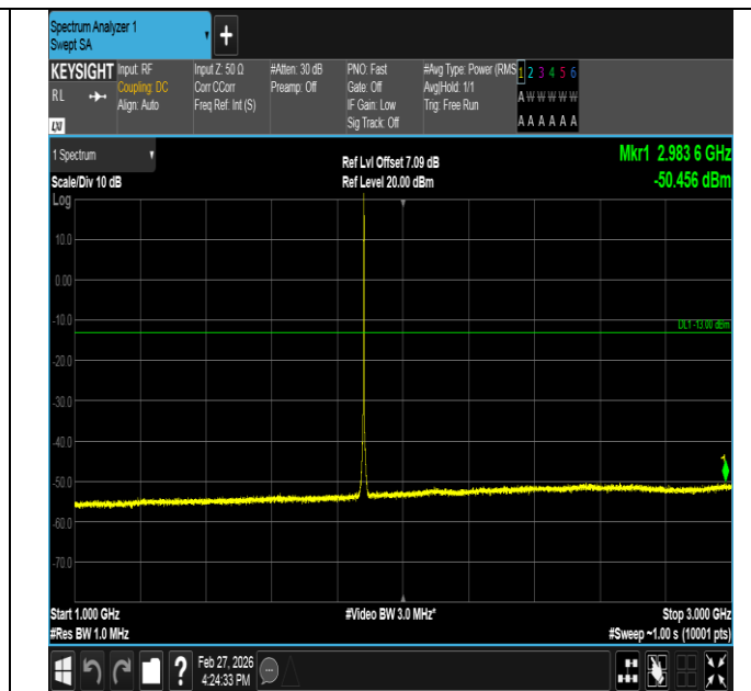
Band2-1.4MHz-16QAM-18900-1RB#5-1000~3000-PASS
