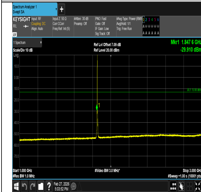
Band2-3MHz-QPSK-18615-1RB#14-1000~3000-PASS
