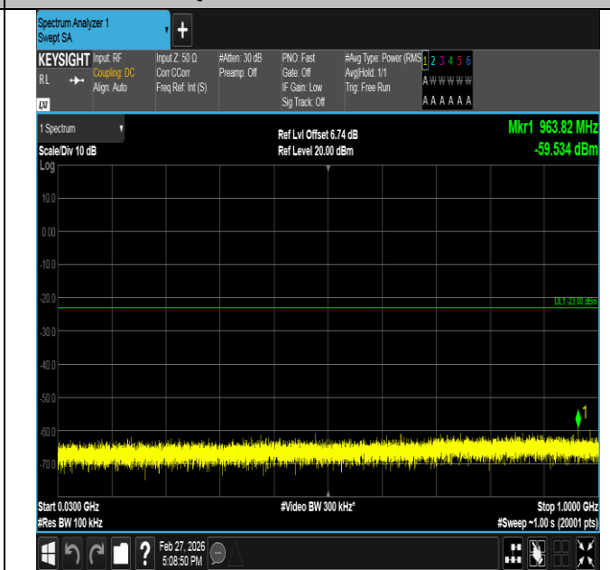
Band2-3MHz-QPSK-18900-1RB#14-30~1000-PASS
