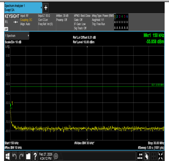
Band2-1.4MHz-16QAM-18900-1RB#5-0.15~30-PASS
