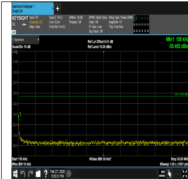
Band2-3MHz-QPSK-18615-1RB#14-0.15~30-PASS
