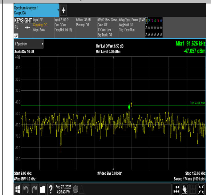
Band2-1.4MHz-16QAM-18900-6RB#0-0.009~0.15-PASS
