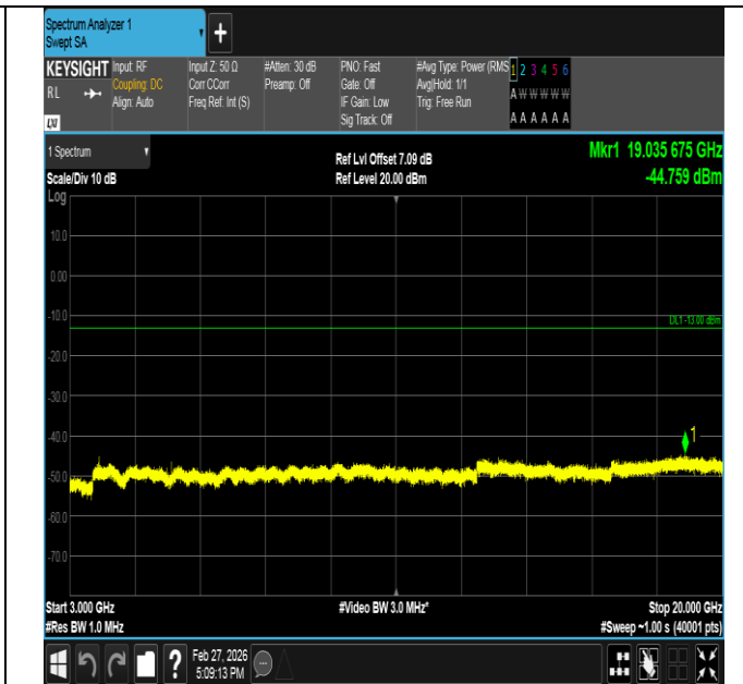
Band2-3MHz-QPSK-18900-1RB#14-3000~20000-PASS
