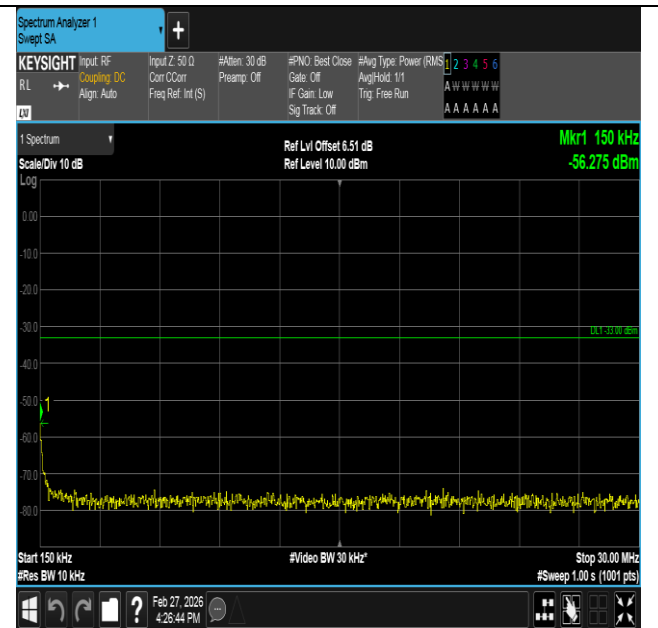
Band2-1.4MHz-QPSK-19193-1RB#0-0.15~30-PASS
