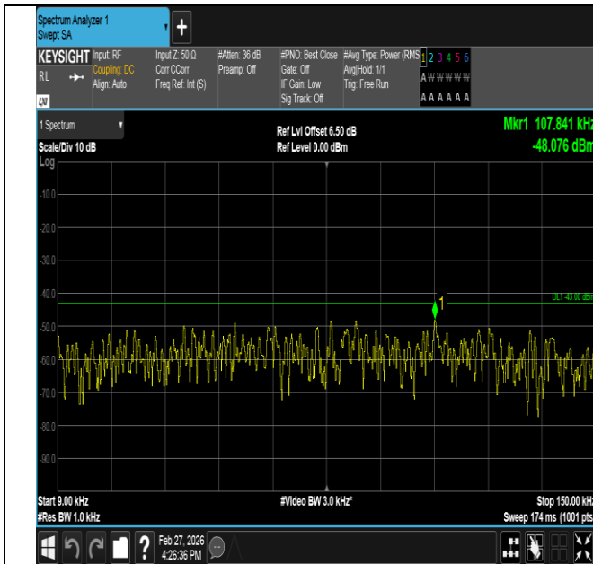
Band2-1.4MHz-QPSK-19193-1RB#0-0.009~0.15-PASS
