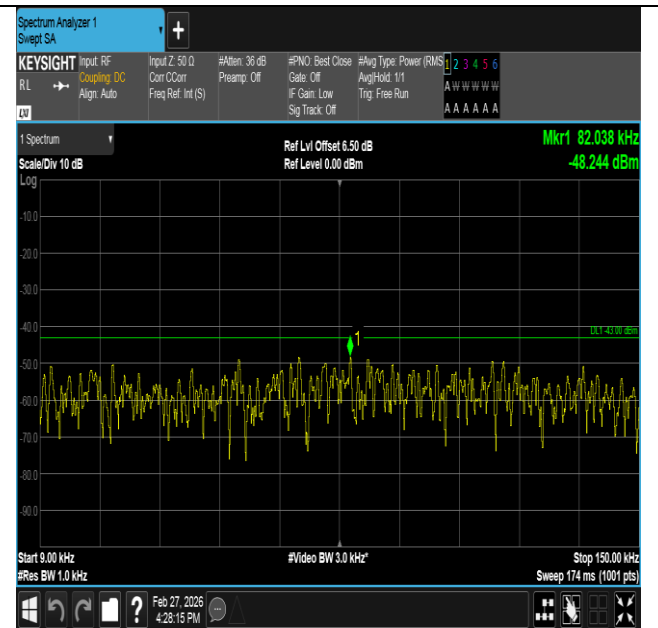
Band2-1.4MHz-QPSK-19193-1RB#5-0.009~0.15-PASS
