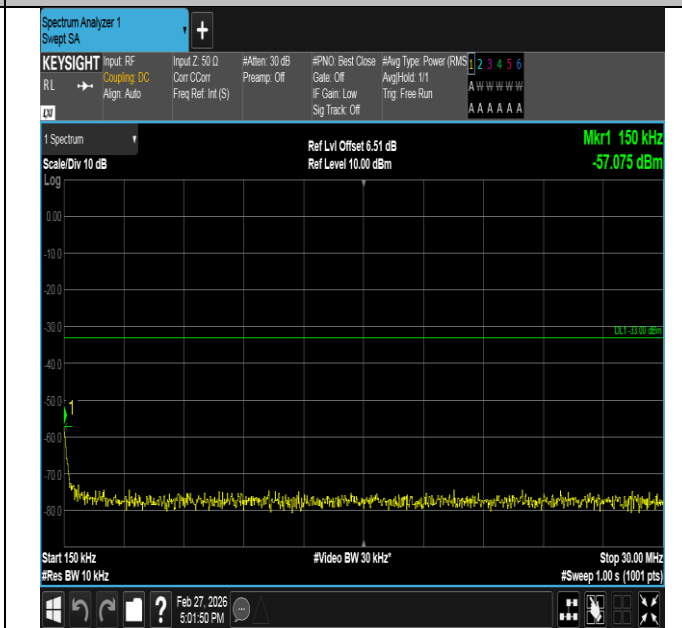
Band2-3MHz-QPSK-18615-1RB#0-0.15~30-PASS
