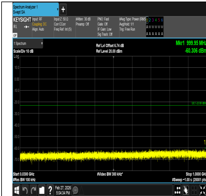
Band2-3MHz-16QAM-18615-1RB#14-30~1000-PASS
