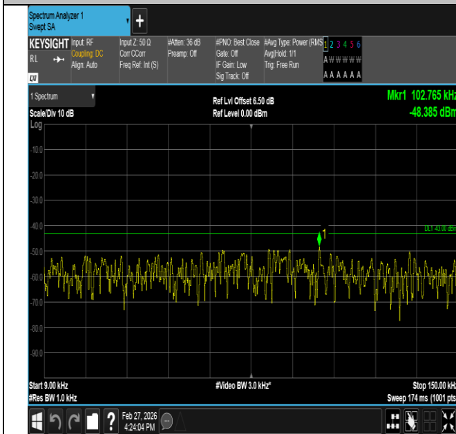
Band2-1.4MHz-16QAM-18900-1RB#5-0.009~0.15-PASS
