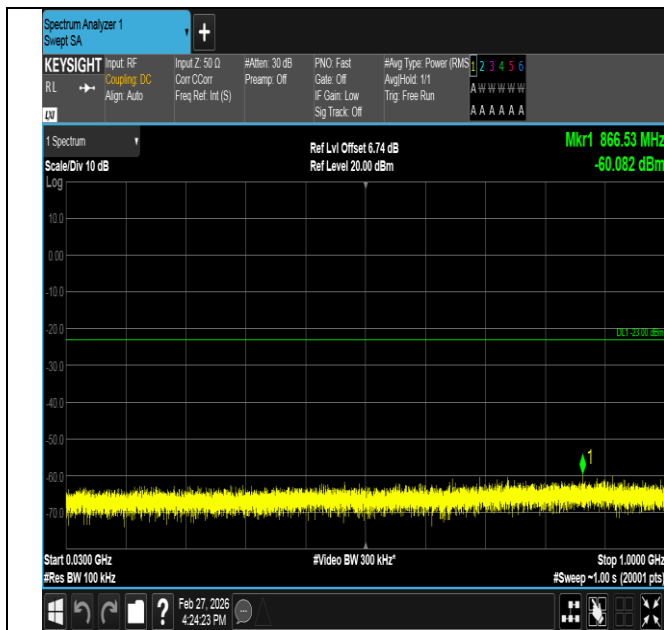
Band2-1.4MHz-16QAM-18900-1RB#5-30~1000-PASS
