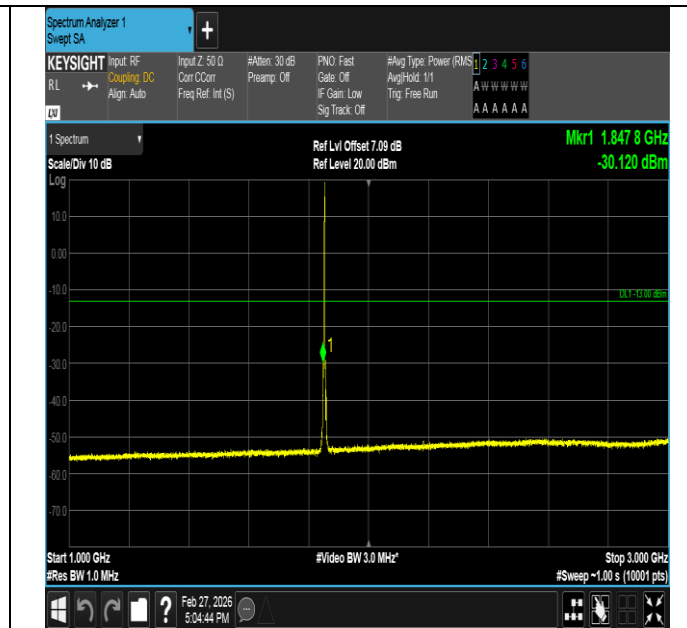
Band2-3MHz-16QAM-18615-1RB#14-1000~3000-PASS
