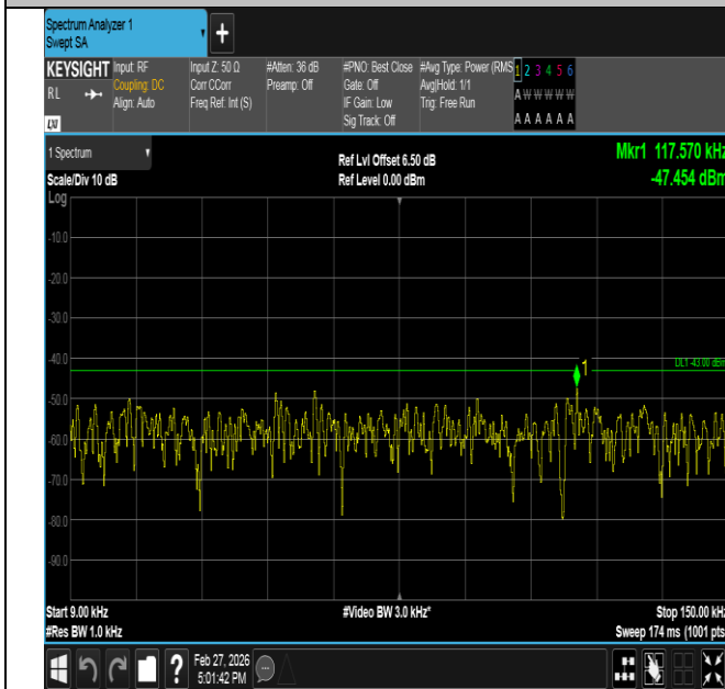
Band2-3MHz-QPSK-18615-1RB#0-0.009~0.15-PASS
