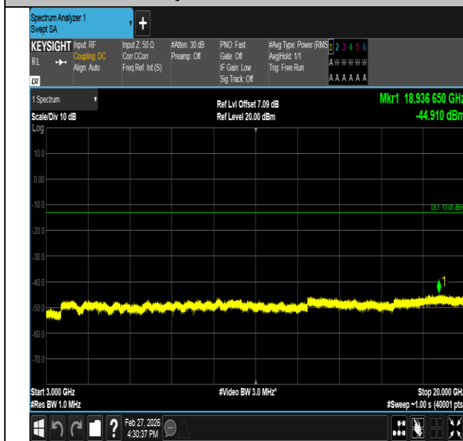
Band2-1.4MHz-QPSK-19193-6RB#0-3000~20000-PASS
