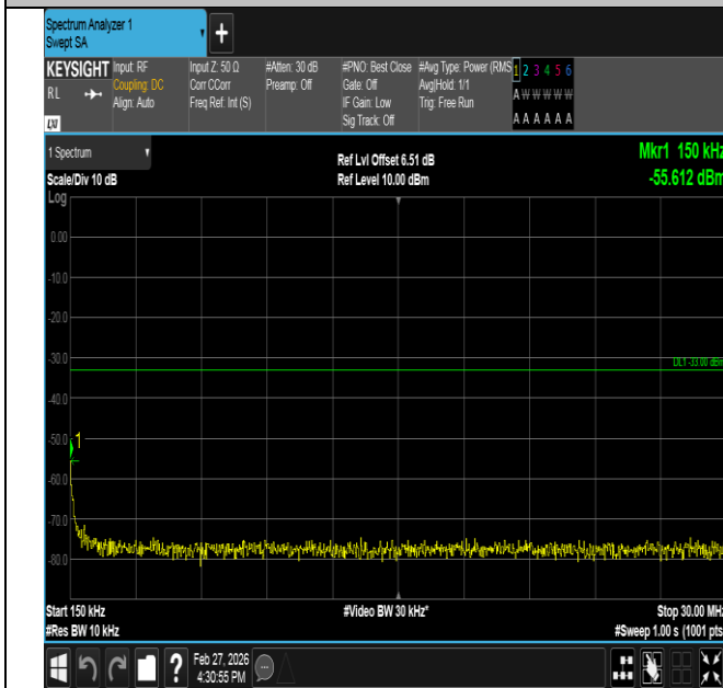
Band2-1.4MHz-16QAM-19193-6RB#0-0.15~30-PASS
