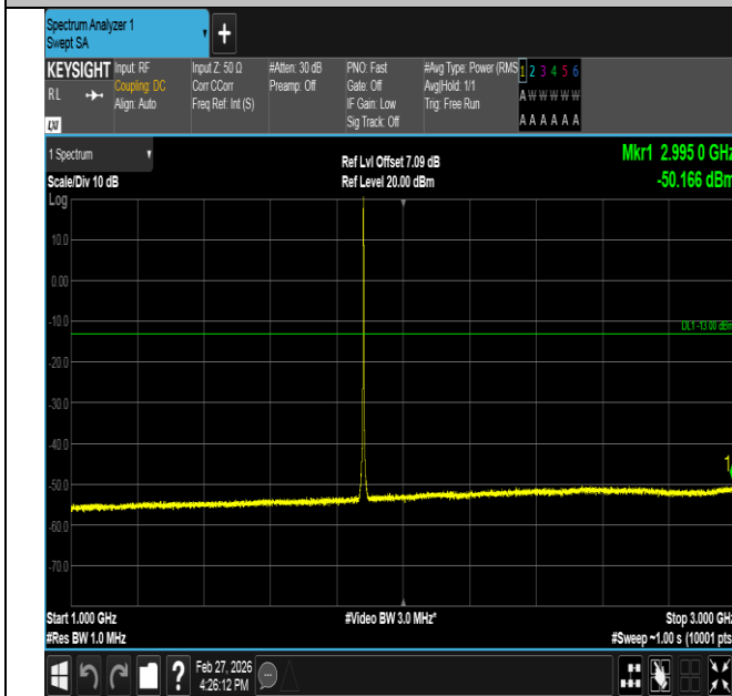
Band2-1.4MHz-16QAM-18900-6RB#0-1000~3000-PASS
