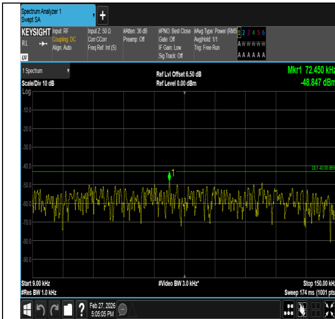
Band2-3MHz-QPSK-18615-15RB#0-0.009~0.15-PASS
