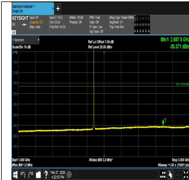
Band2-1.4MHz-16QAM-18900-1RB#0-1000~3000-PASS
