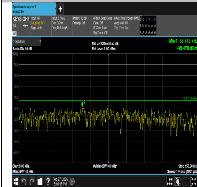
Band2-3MHz-QPSK-18900-15RB#0-0.009~0.15-PASS
