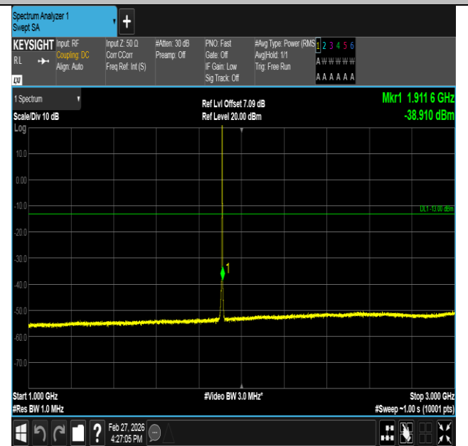
Band2-1.4MHz-QPSK-19193-1RB#0-1000~3000-PASS
