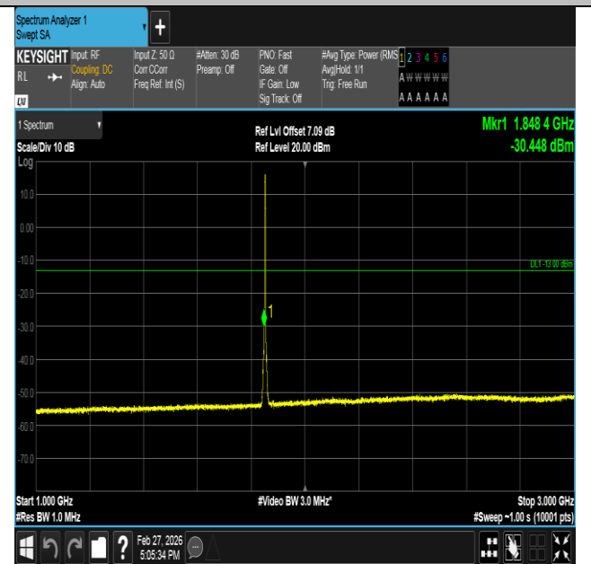
Band2-3MHz-QPSK-18615-15RB#0-1000~3000-PASS
