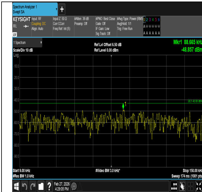
Band2-1.4MHz-16QAM-19193-1RB#5-0.009~0.15-PASS
