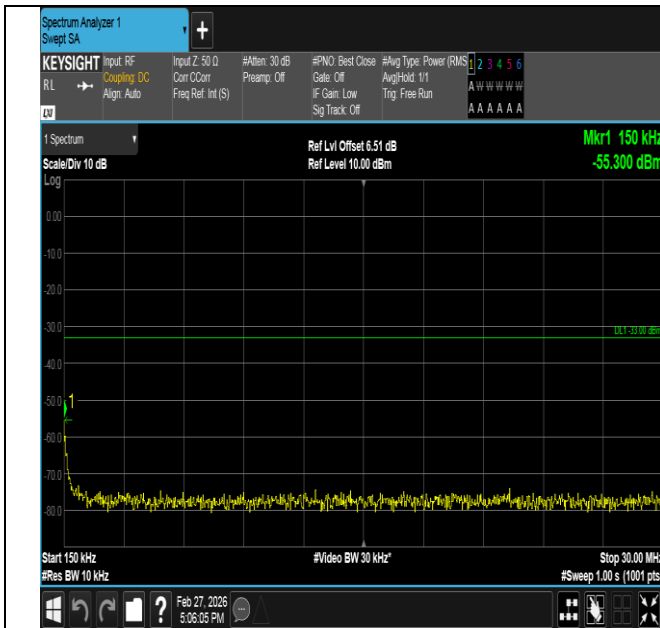
Band2-3MHz-16QAM-18615-15RB#0-0.15~30-PASS
