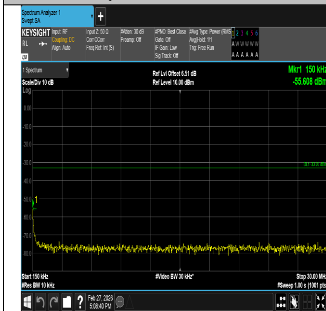
Band2-3MHz-QPSK-18900-1RB#14-0.15~30-PASS
