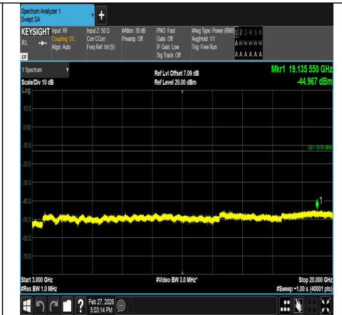
Band2-3MHz-16QAM-18615-1RB#0-3000~20000-PASS
