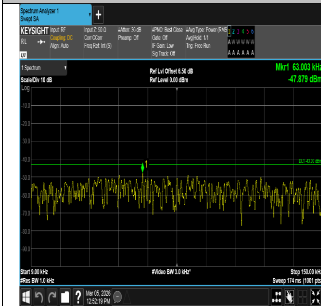
Band2-10MHz-QPSK-18900-50RB#0-0.009~0.15-PASS
