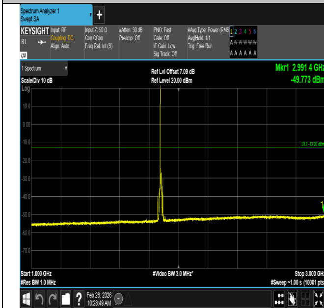
Band2-10MHz-16QAM-18900-1RB#0-1000~3000-PASS
