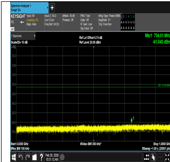
Band2-10MHz-QPSK-19150-1RB#0-30~1000-PASS
