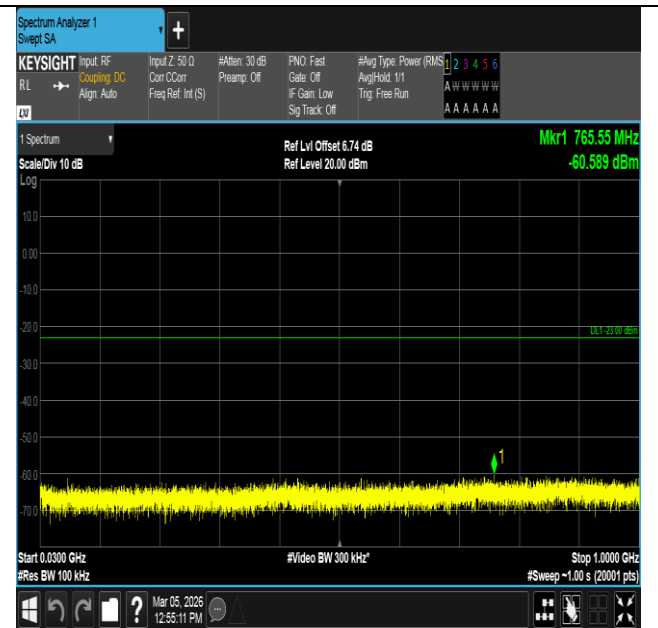
Band2-10MHz-16QAM-19150-50RB#0-30~1000-PASS
