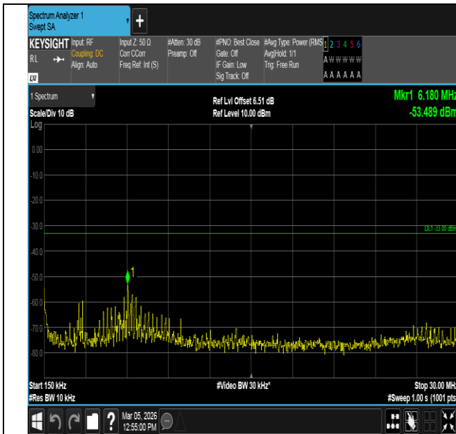
Band2-10MHz-16QAM-19150-50RB#0-0.15~30-PASS
