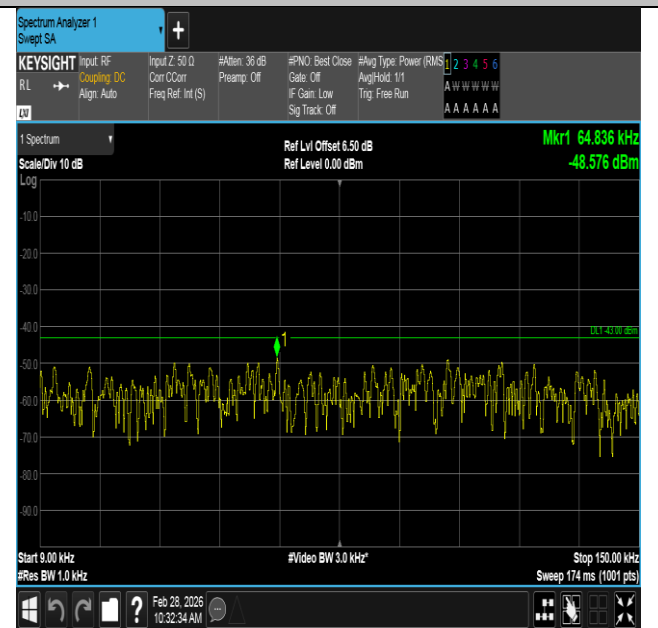
Band2-10MHz-QPSK-19150-1RB#49-0.009~0.15-PASS
