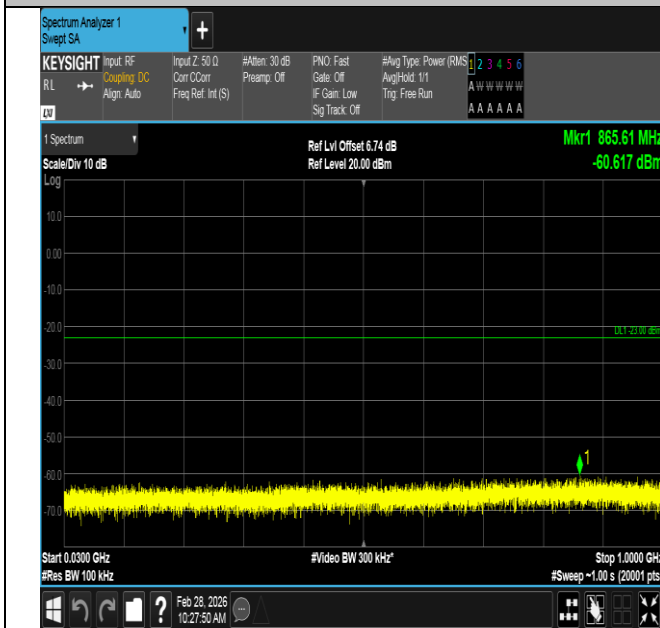
Band2-10MHz-QPSK-18900-1RB#0-30~1000-PASS
