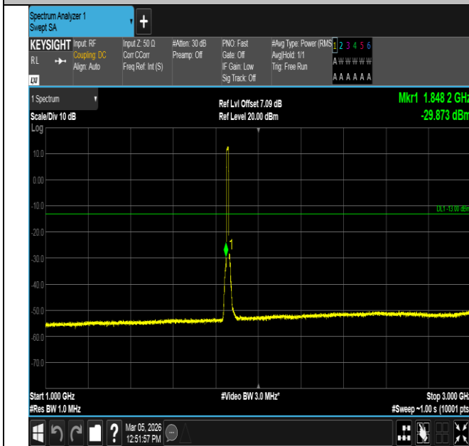
Band2-10MHz-16QAM-18650-50RB#0-1000~3000-PASS
