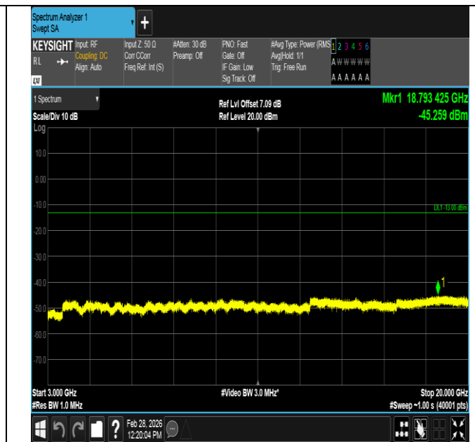
Band2-15MHz-QPSK-18675-1RB#74-3000~20000-PASS
