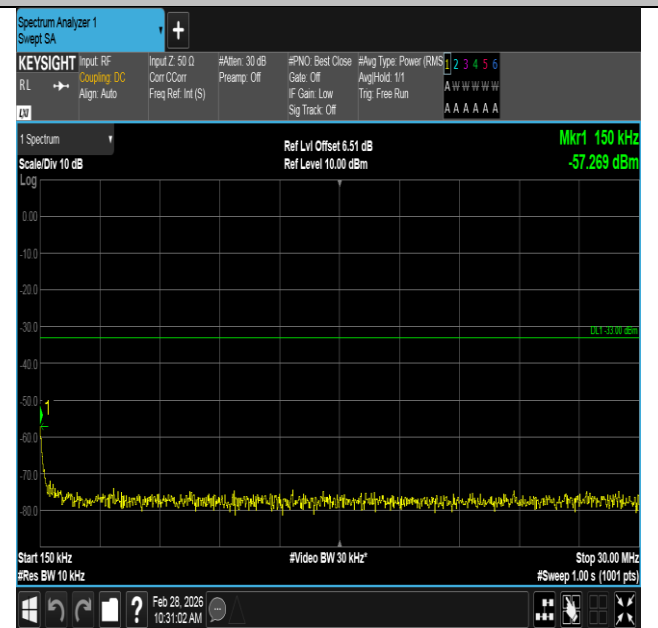
Band2-10MHz-QPSK-19150-1RB#0-0.15~30-PASS
