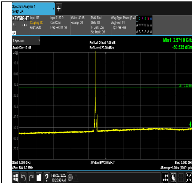
Band2-10MHz-QPSK-18900-1RB#49-1000~3000-PASS
