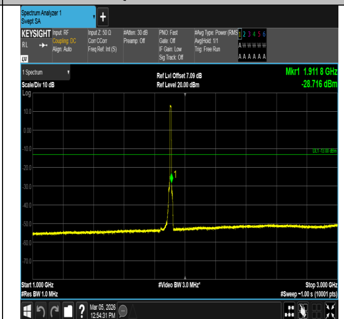
Band2-10MHz-QPSK-19150-50RB#0-1000~3000-PASS
