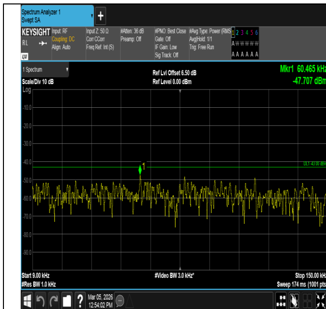
Band2-10MHz-QPSK-19150-50RB#0-0.009~0.15-PASS
