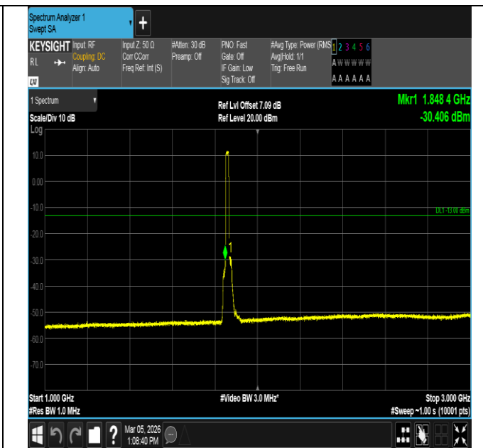
Band2-15MHz-QPSK-18675-75RB#0-1000~3000-PASS
