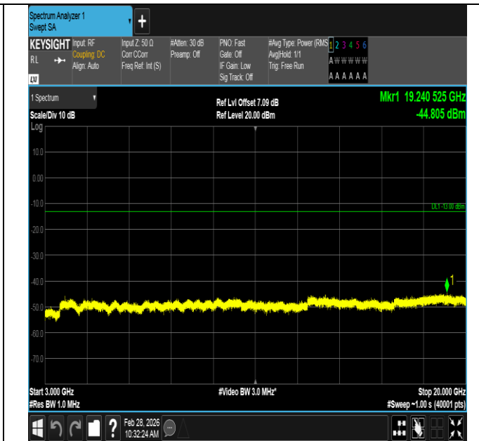
Band2-10MHz-16QAM-19150-1RB#0-3000~20000-PASS
