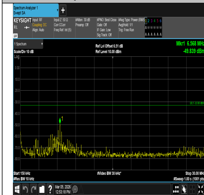
Band2-10MHz-16QAM-18900-50RB#0-0.15~30-PASS
