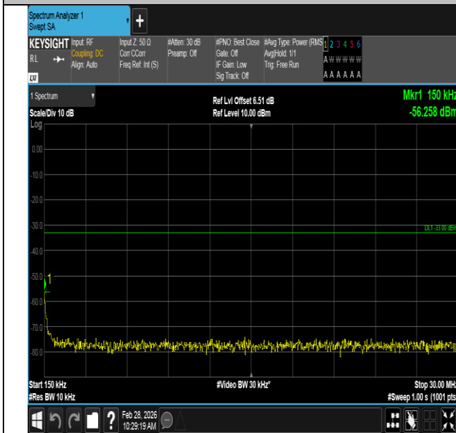
Band2-10MHz-QPSK-18900-1RB#49-0.15~30-PASS
