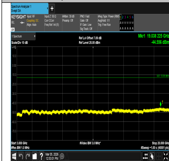
Band2-10MHz-QPSK-18900-50RB#0-3000~20000-PASS
