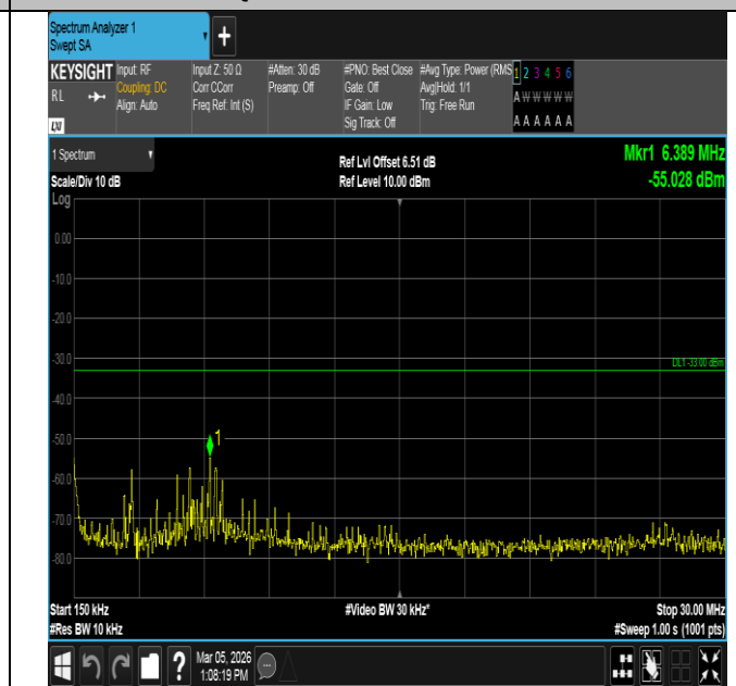
Band2-15MHz-QPSK-18675-75RB#0-0.15~30-PASS
