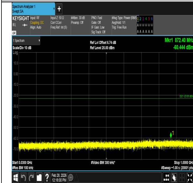
Band2-15MHz-QPSK-18675-1RB#0-30~1000-PASS
