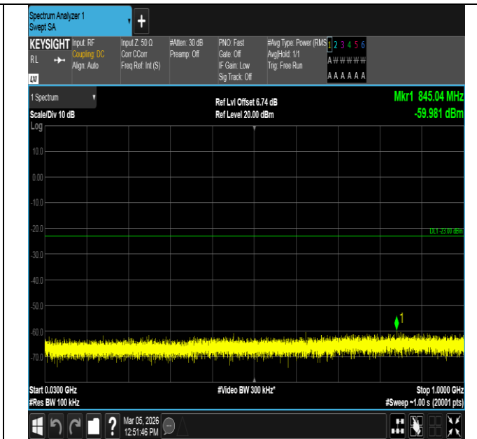
Band2-10MHz-16QAM-18650-50RB#0-30~1000-PASS
