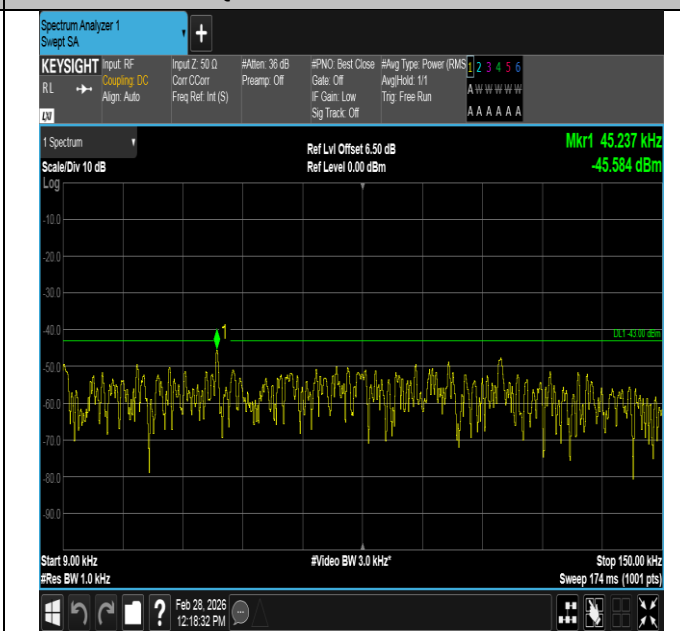
Band2-15MHz-16QAM-18675-1RB#0-0.009~0.15-PASS
