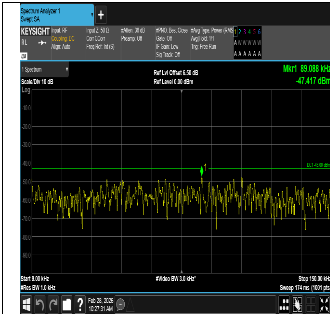
Band2-10MHz-QPSK-18900-1RB#0-0.009~0.15-PASS
