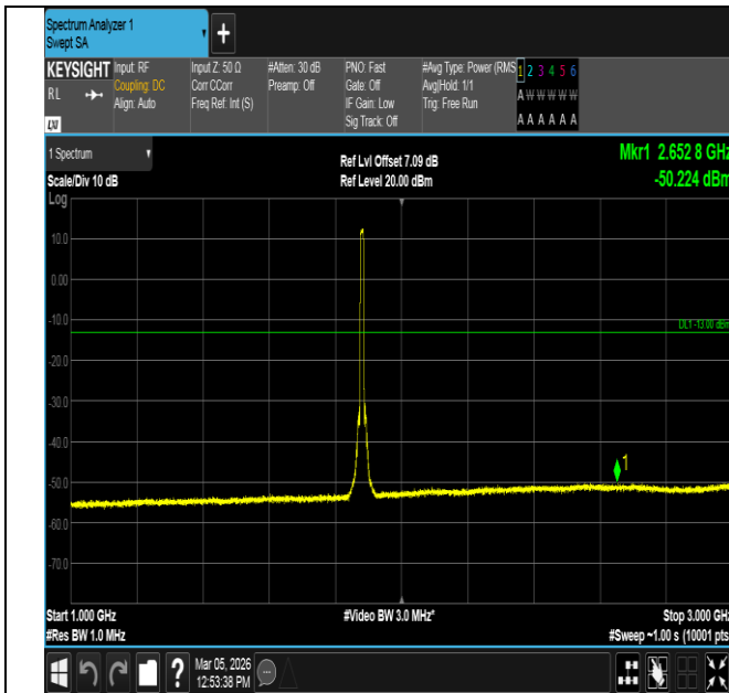
Band2-10MHz-16QAM-18900-50RB#0-1000~3000-PASS
