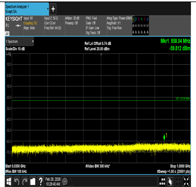
Band2-10MHz-16QAM-18900-1RB#0-30~1000-PASS
