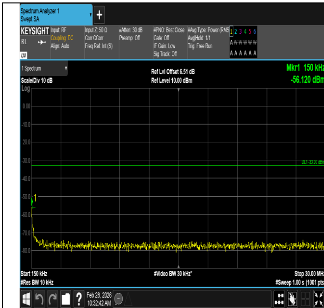
Band2-10MHz-QPSK-19150-1RB#49-0.15~30-PASS
