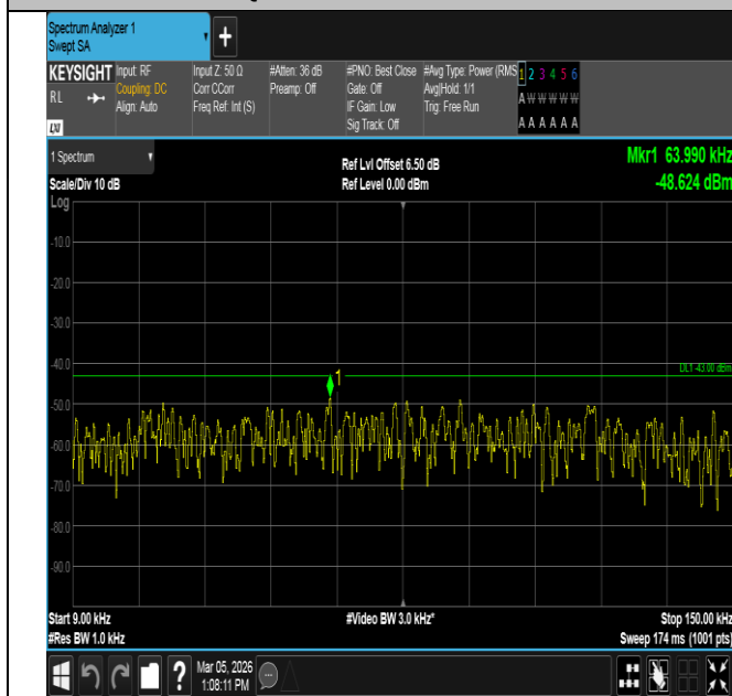
Band2-15MHz-QPSK-18675-75RB#0-0.009~0.15-PASS
