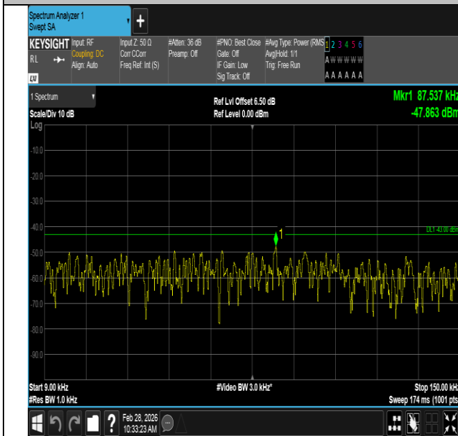
Band2-10MHz-16QAM-19150-1RB#49-0.009~0.15-PASS
