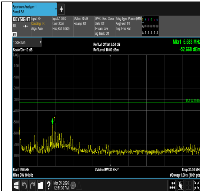
Band2-10MHz-16QAM-18650-50RB#0-0.15~30-PASS
