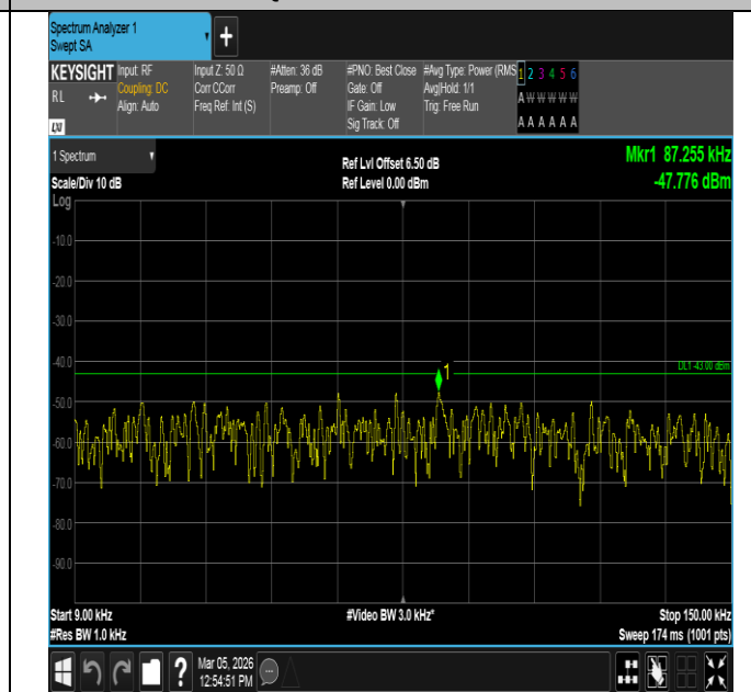
Band2-10MHz-16QAM-19150-50RB#0-0.009~0.15-PASS
