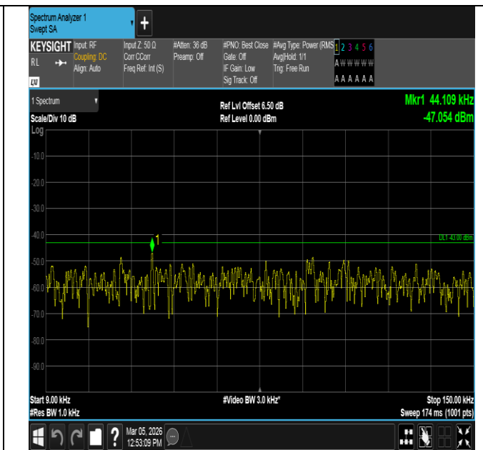
Band2-10MHz-16QAM-18900-50RB#0-0.009~0.15-PASS
