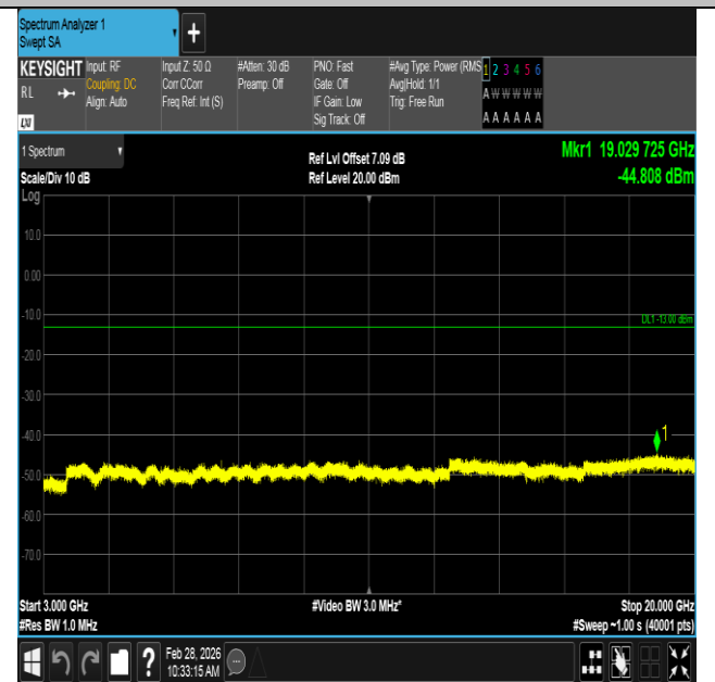
Band2-10MHz-QPSK-19150-1RB#49-3000~20000-PASS
