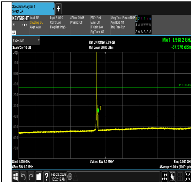
Band2-10MHz-16QAM-19150-1RB#0-1000~3000-PASS
