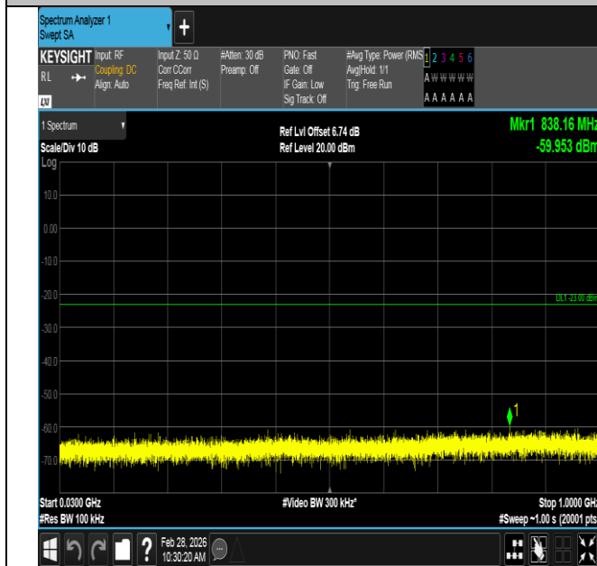
Band2-10MHz-16QAM-18900-1RB#49-30~1000-PASS
