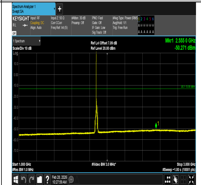
Band2-10MHz-QPSK-18900-1RB#0-1000~3000-PASS
