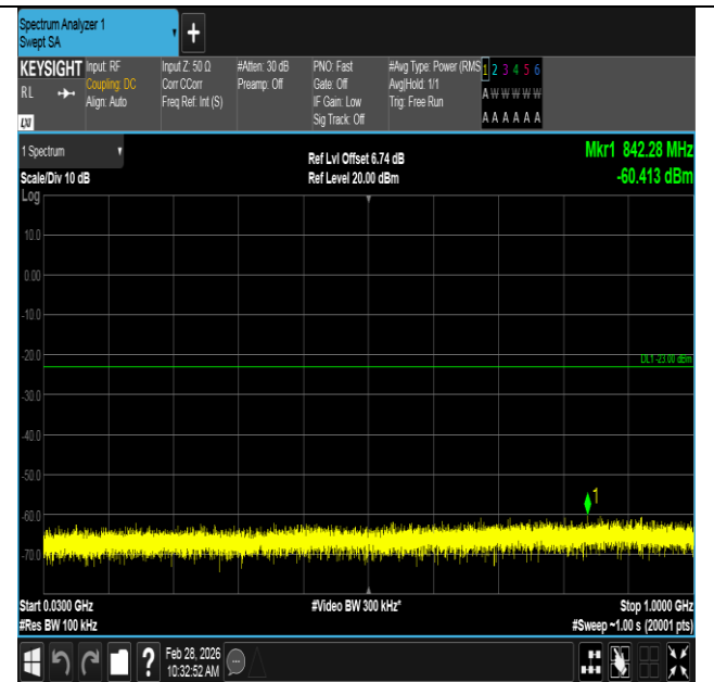
Band2-10MHz-QPSK-19150-1RB#49-30~1000-PASS
