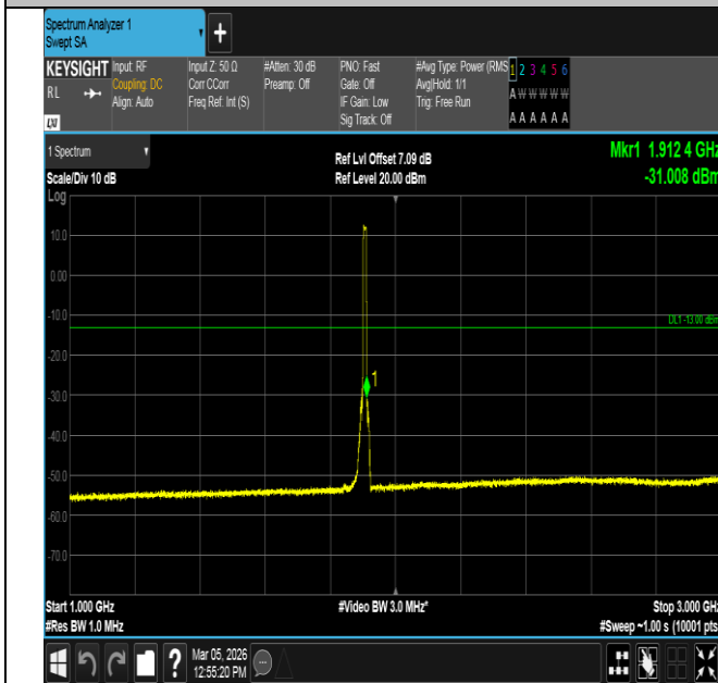
Band2-10MHz-16QAM-19150-50RB#0-1000~3000-PASS
