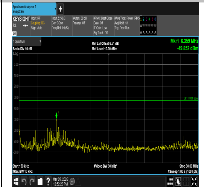
Band2-10MHz-QPSK-18900-50RB#0-0.15~30-PASS
