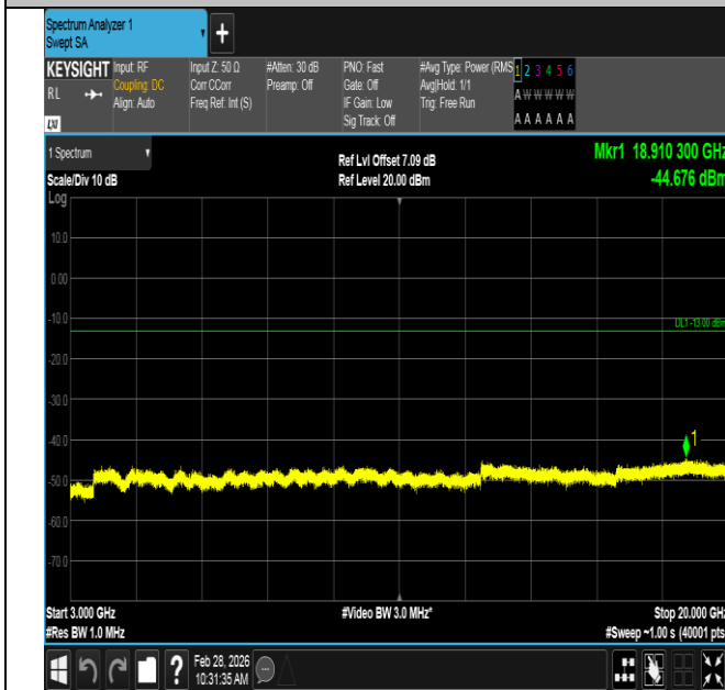
Band2-10MHz-QPSK-19150-1RB#0-3000~20000-PASS
