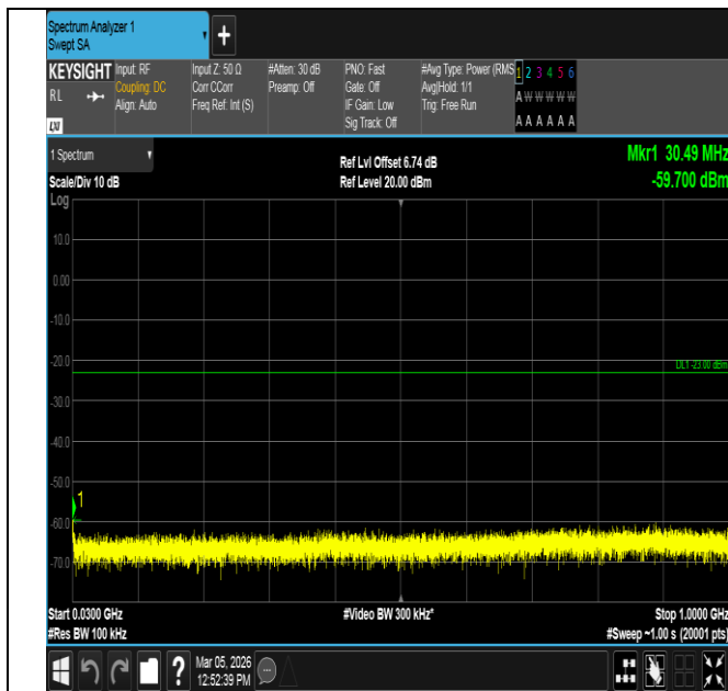
Band2-10MHz-QPSK-18900-50RB#0-30~1000-PASS
