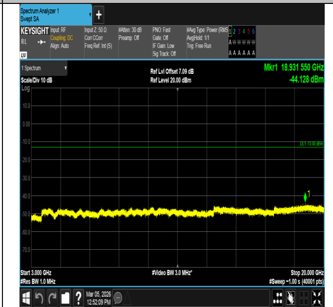
Band2-10MHz-16QAM-18650-50RB#0-3000~20000-PASS
