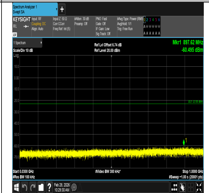
Band2-10MHz-QPSK-18900-1RB#49-30~1000-PASS
