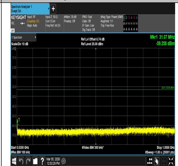
Band2-10MHz-16QAM-18900-50RB#0-30~1000-PASS
