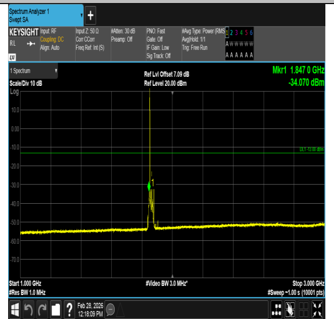
Band2-15MHz-QPSK-18675-1RB#0-1000~3000-PASS
