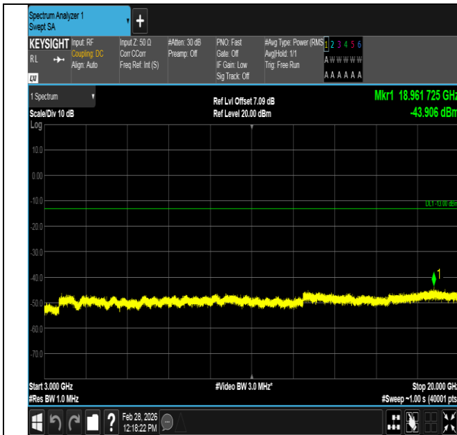
Band2-15MHz-QPSK-18675-1RB#0-3000~20000-PASS
