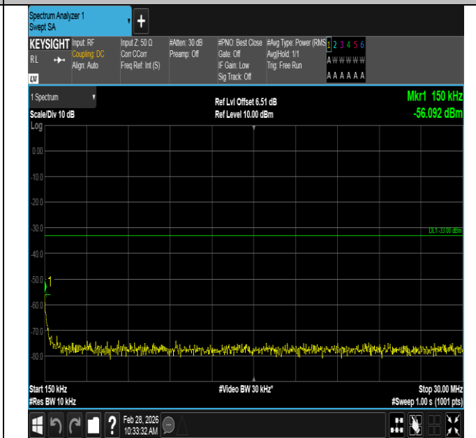
Band2-10MHz-16QAM-19150-1RB#49-0.15~30-PASS
