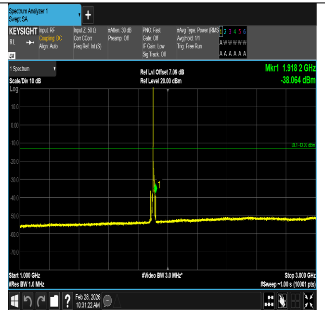
Band2-10MHz-QPSK-19150-1RB#0-1000~3000-PASS
