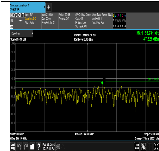
Band2-15MHz-QPSK-18675-1RB#0-0.009~0.15-PASS
