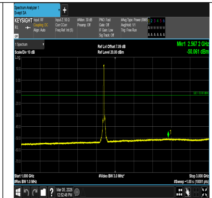
Band2-10MHz-QPSK-18900-50RB#0-1000~3000-PASS
