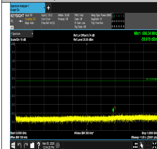
Band2-10MHz-QPSK-19150-50RB#0-30~1000-PASS
