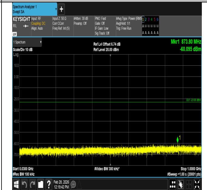
Band2-15MHz-QPSK-18675-1RB#74-30~1000-PASS
