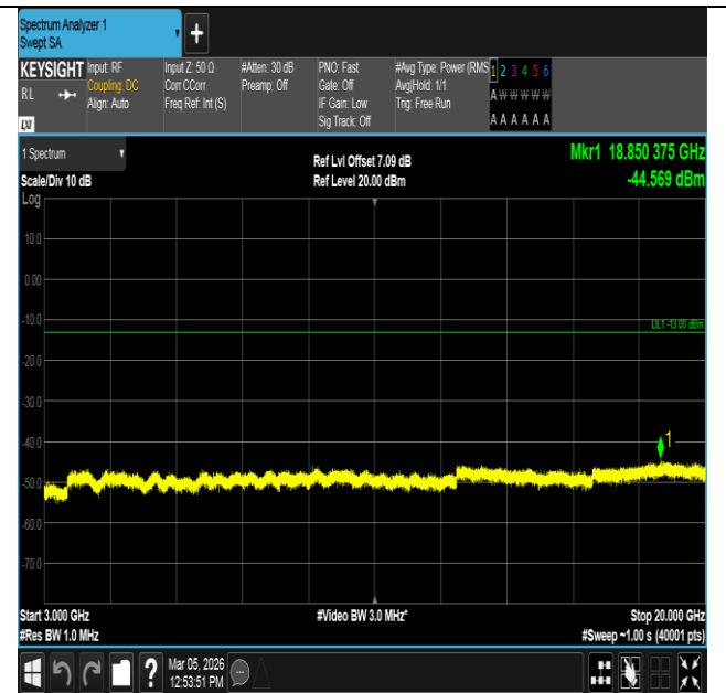
Band2-10MHz-16QAM-18900-50RB#0-3000~20000-PASS
