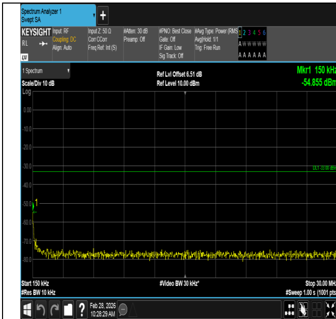
Band2-10MHz-16QAM-18900-1RB#0-0.15~30-PASS
