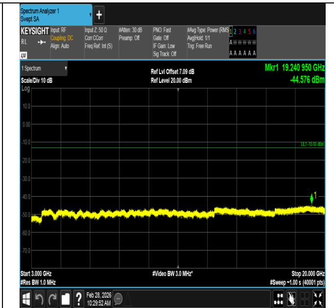
Band2-10MHz-QPSK-18900-1RB#49-3000~20000-PASS
