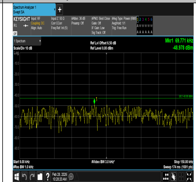
Band2-10MHz-16QAM-18900-1RB#0-0.009~0.15-PASS
