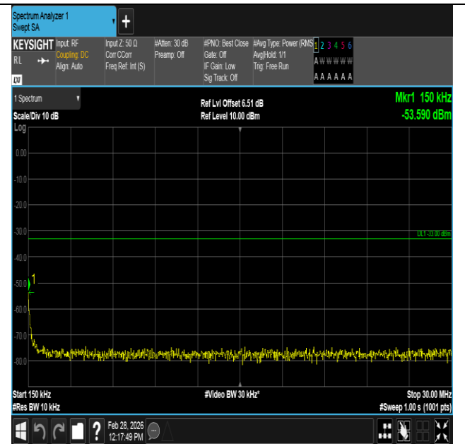
Band2-15MHz-QPSK-18675-1RB#0-0.15~30-PASS
