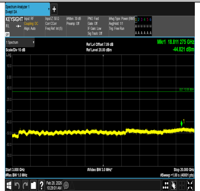
Band2-10MHz-16QAM-18900-1RB#0-3000~20000-PASS
