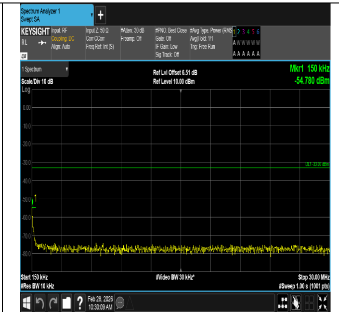
Band2-10MHz-16QAM-18900-1RB#49-0.15~30-PASS
