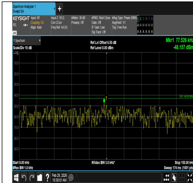
Band2-10MHz-16QAM-18900-1RB#49-0.009~0.15-PASS
