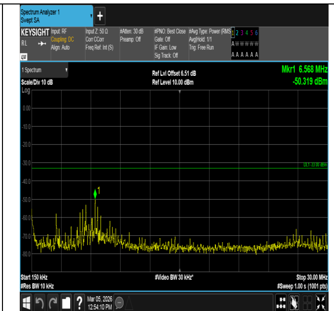
Band2-10MHz-QPSK-19150-50RB#0-0.15~30-PASS
