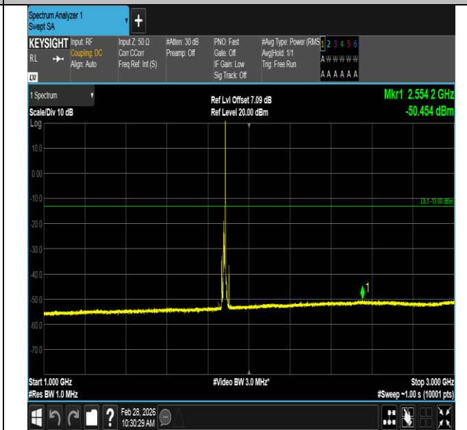
Band2-10MHz-16QAM-18900-1RB#49-1000~3000-PASS
