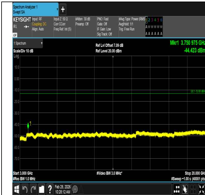
Band2-10MHz-QPSK-18900-1RB#0-3000~20000-PASS
