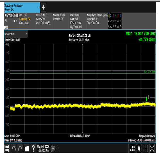
Band2-10MHz-16QAM-19150-50RB#0-3000~20000-PASS
