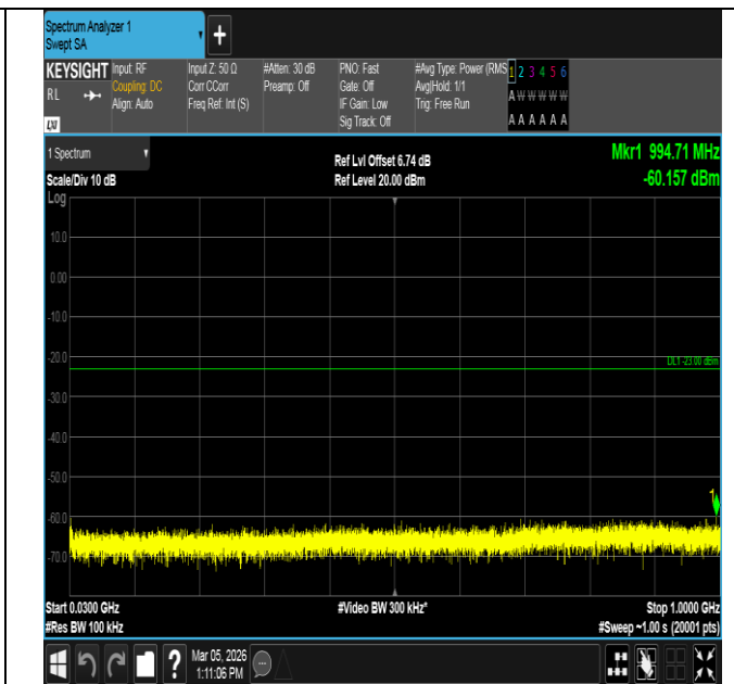
Band2-15MHz-16QAM-18900-75RB#0-30~1000-PASS
