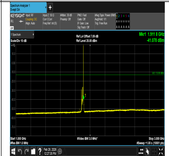
Band2-15MHz-16QAM-19125-1RB#74-1000~3000-PASS
