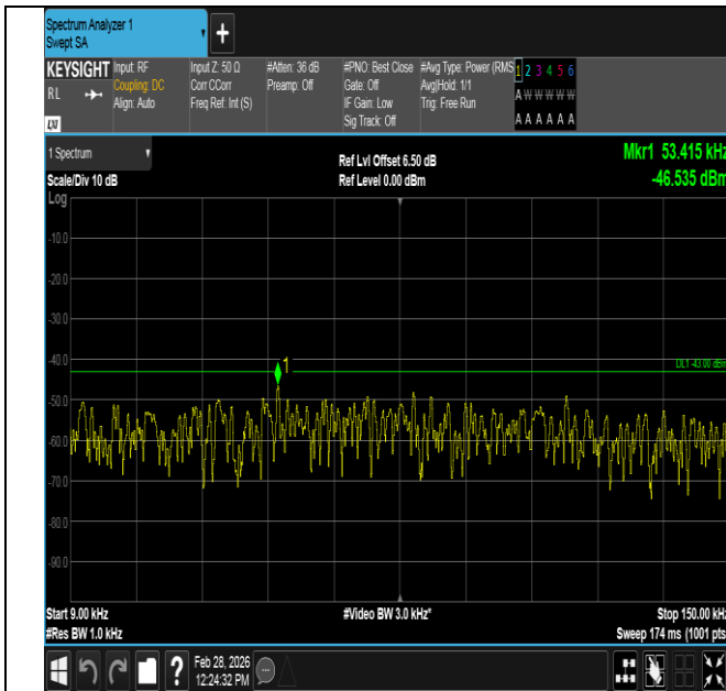
Band2-15MHz-QPSK-19125-1RB#0-0.009~0.15-PASS
