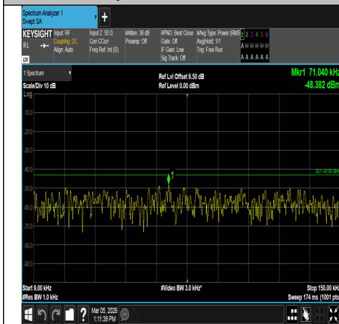
Band2-15MHz-QPSK-19125-75RB#0-0.009~0.15-PASS
