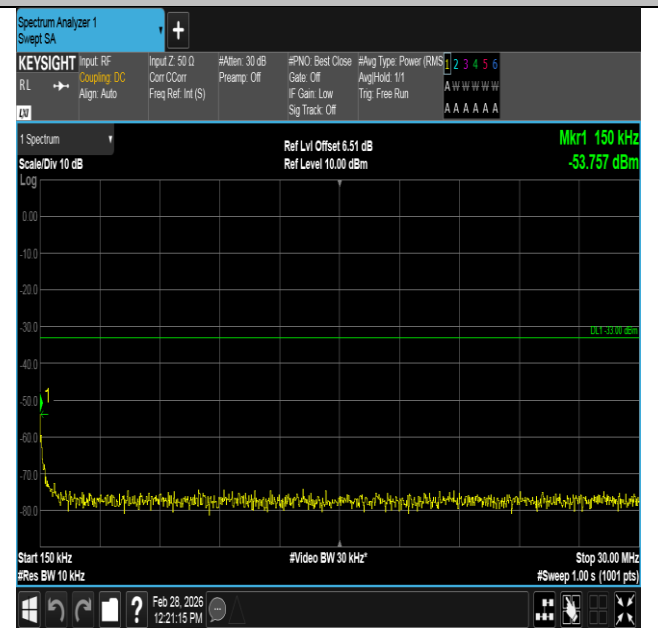
Band2-15MHz-QPSK-18900-1RB#0-0.15~30-PASS
