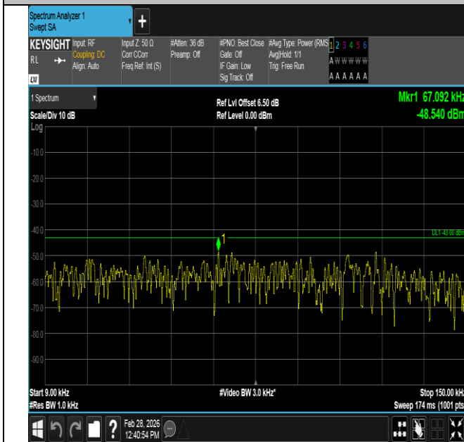
Band2-20MHz-QPSK-18700-1RB#0-0.009~0.15-PASS
