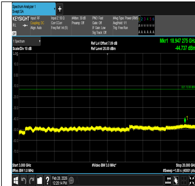
Band2-15MHz-QPSK-19125-1RB#0-3000~20000-PASS
