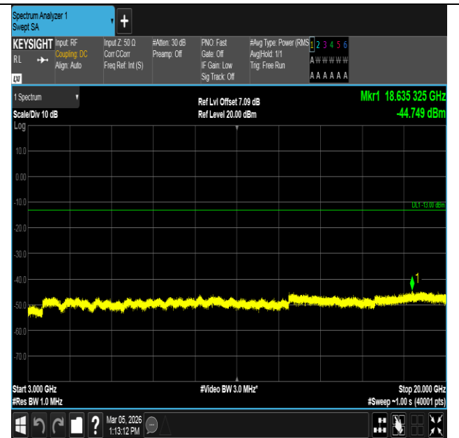
Band2-15MHz-16QAM-19125-75RB#0-3000~20000-PASS
