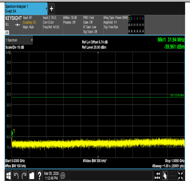
Band2-15MHz-16QAM-19125-75RB#0-30~1000-PASS
