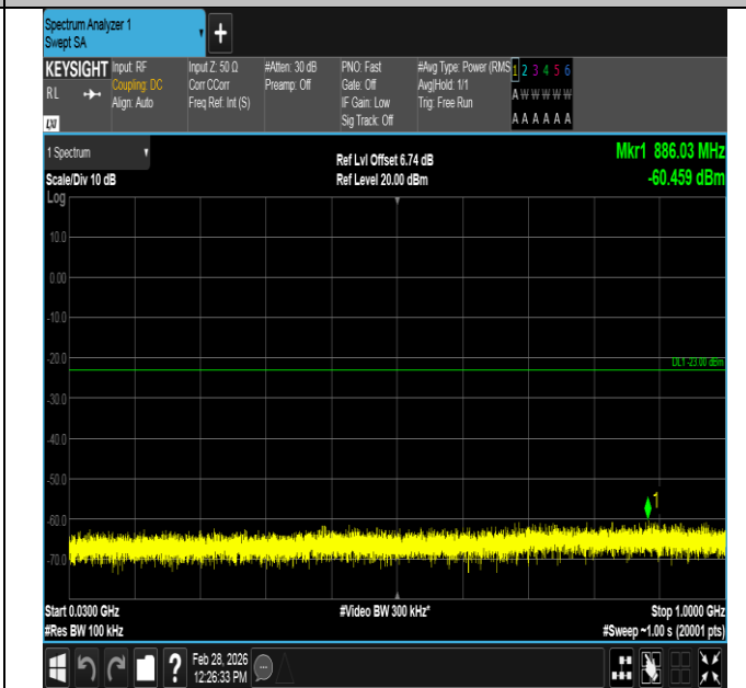
Band2-15MHz-QPSK-19125-1RB#74-30~1000-PASS
