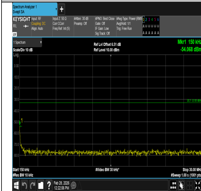
Band2-15MHz-16QAM-18900-1RB#0-0.15~30-PASS
