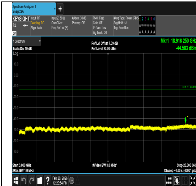
Band2-15MHz-16QAM-18675-1RB#74-3000~20000-PASS
