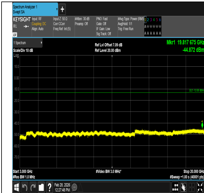
Band2-15MHz-16QAM-19125-1RB#74-3000~20000-PASS
