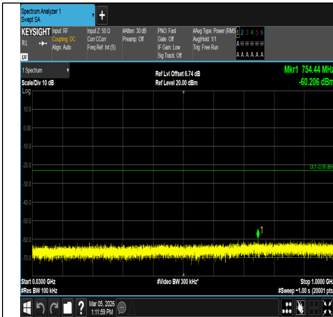
Band2-15MHz-QPSK-19125-75RB#0-30~1000-PASS
