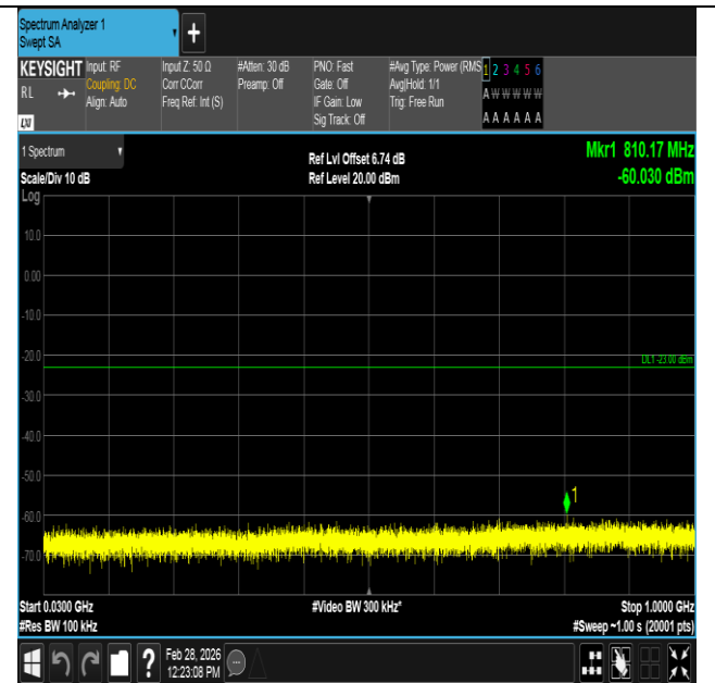
Band2-15MHz-QPSK-18900-1RB#74-30~1000-PASS
