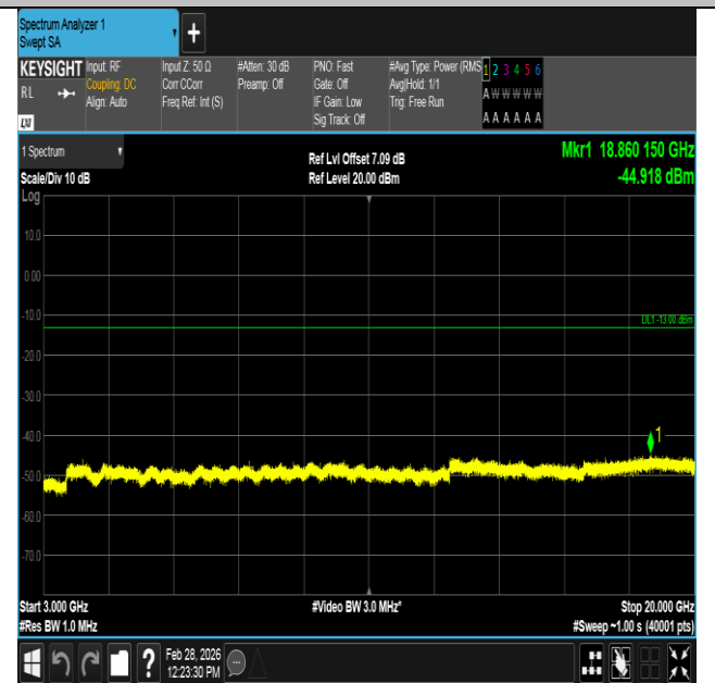
Band2-15MHz-QPSK-18900-1RB#74-3000~20000-PASS
