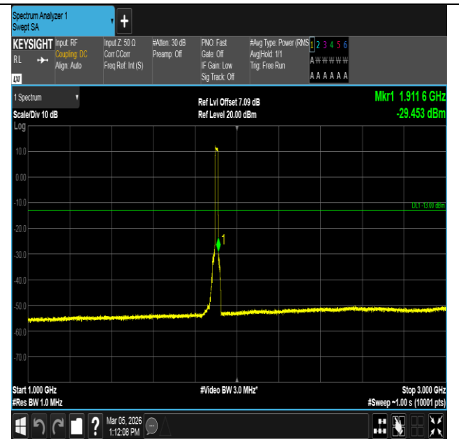
Band2-15MHz-QPSK-19125-75RB#0-1000~3000-PASS
