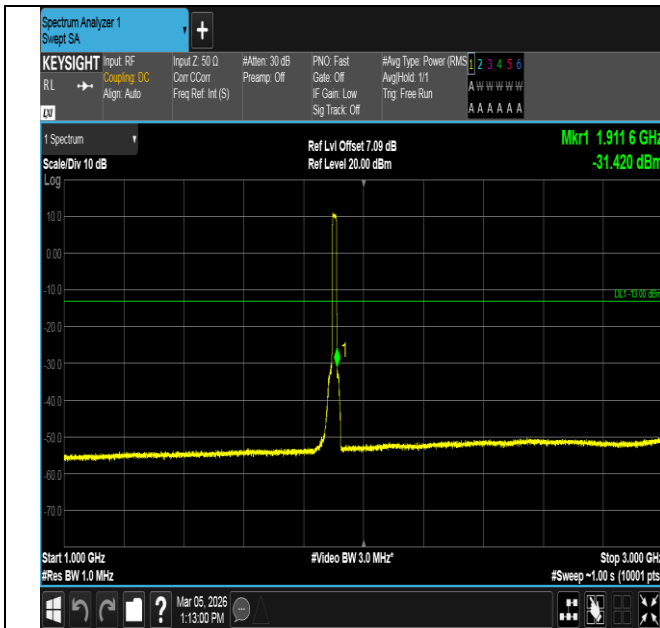
Band2-15MHz-16QAM-19125-75RB#0-1000~3000-PASS
