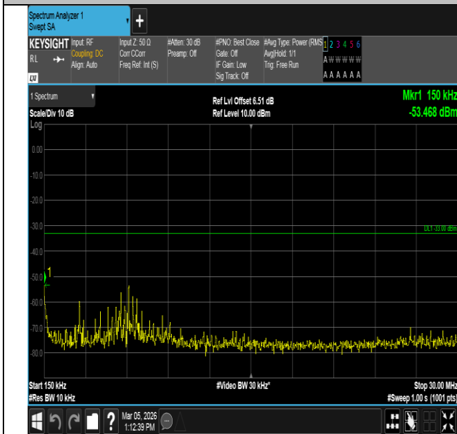
Band2-15MHz-16QAM-19125-75RB#0-0.15~30-PASS
