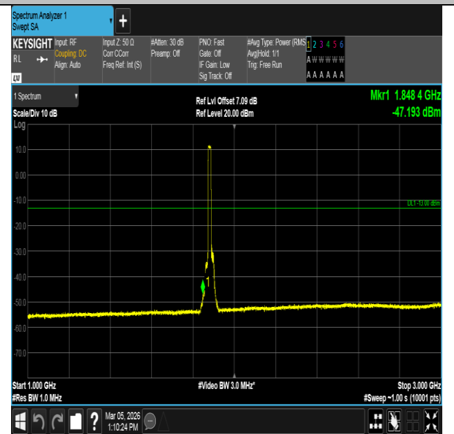
Band2-15MHz-QPSK-18900-75RB#0-1000~3000-PASS
