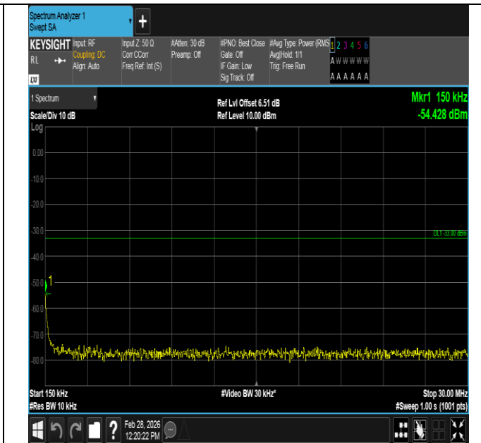
Band2-15MHz-16QAM-18675-1RB#74-0.15~30-PASS
