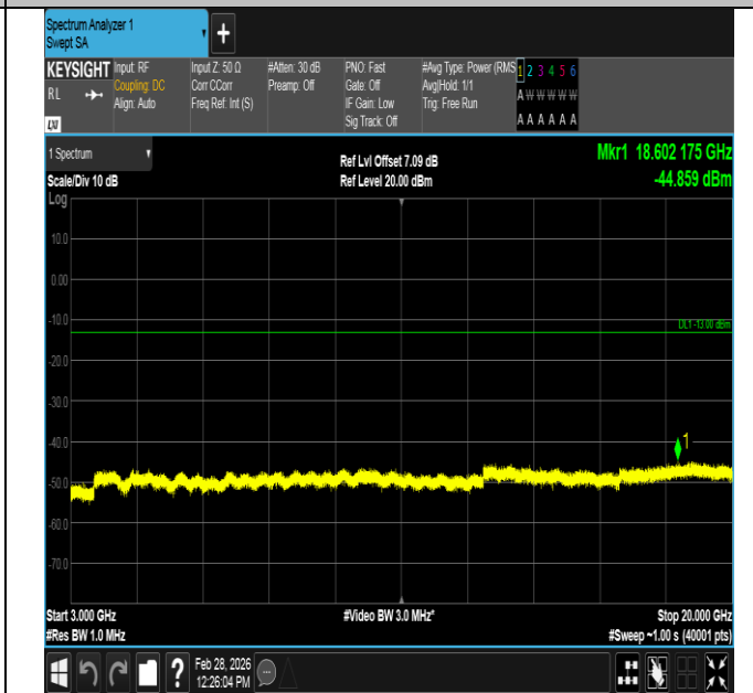
Band2-15MHz-16QAM-19125-1RB#0-3000~20000-PASS
