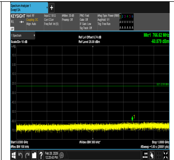
Band2-15MHz-16QAM-19125-1RB#0-30~1000-PASS
