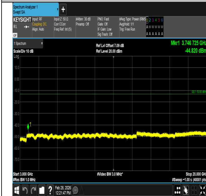
Band2-15MHz-QPSK-18900-1RB#0-3000~20000-PASS
