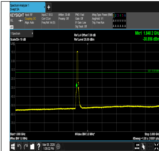
Band2-15MHz-16QAM-18675-75RB#0-1000~3000-PASS
