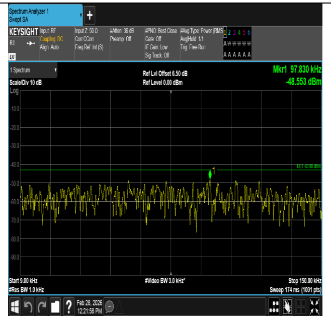
Band2-15MHz-16QAM-18900-1RB#0-0.009~0.15-PASS
