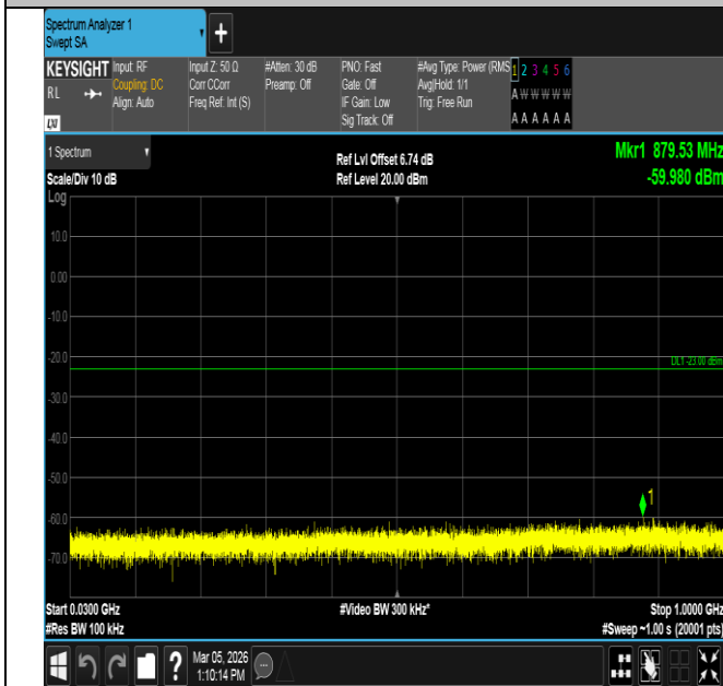
Band2-15MHz-QPSK-18900-75RB#0-30~1000-PASS
