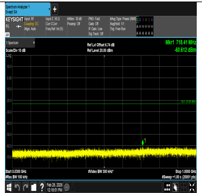
Band2-15MHz-16QAM-18675-1RB#0-30~1000-PASS
