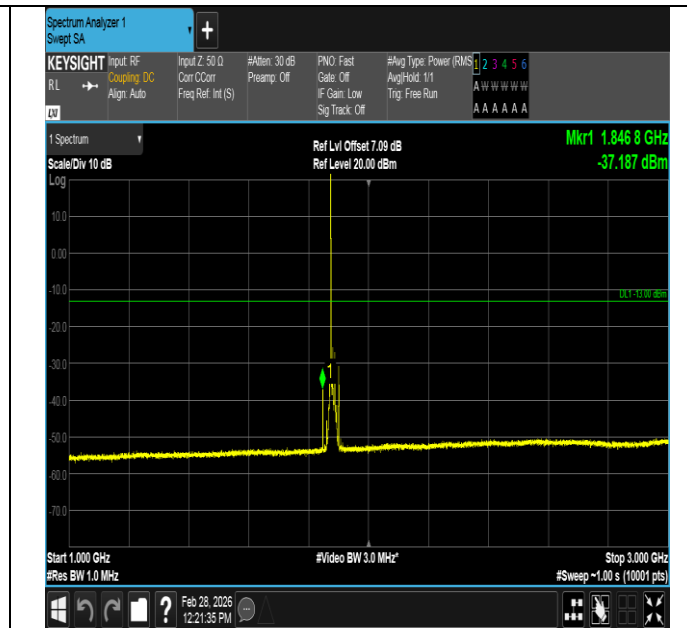
Band2-15MHz-QPSK-18900-1RB#0-1000~3000-PASS
