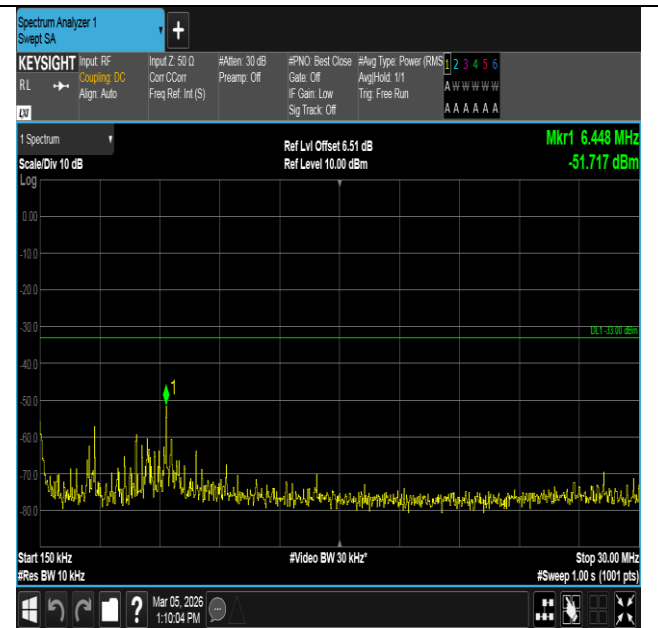
Band2-15MHz-QPSK-18900-75RB#0-0.15~30-PASS
