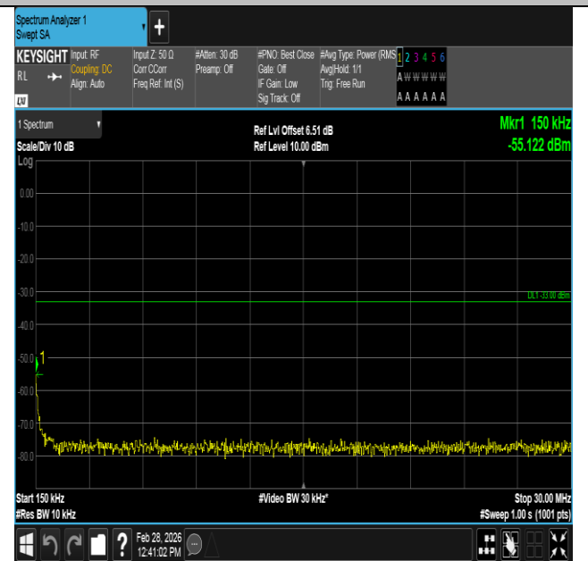
Band2-20MHz-QPSK-18700-1RB#0-0.15~30-PASS
