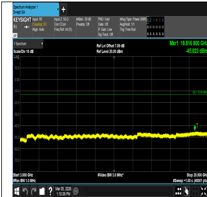
Band2-15MHz-QPSK-18900-75RB#0-3000~20000-PASS
