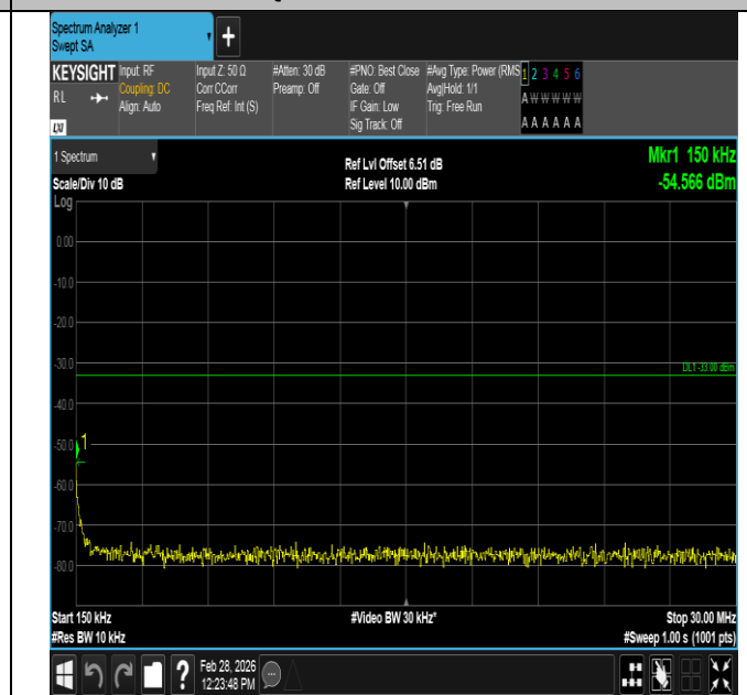
Band2-15MHz-16QAM-18900-1RB#74-0.15~30-PASS
