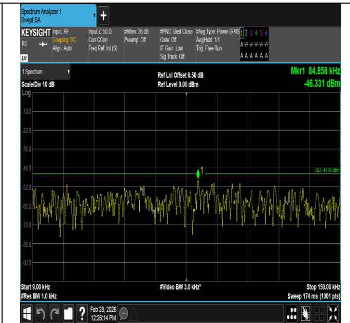
Band2-15MHz-QPSK-19125-1RB#74-0.009~0.15-PASS
