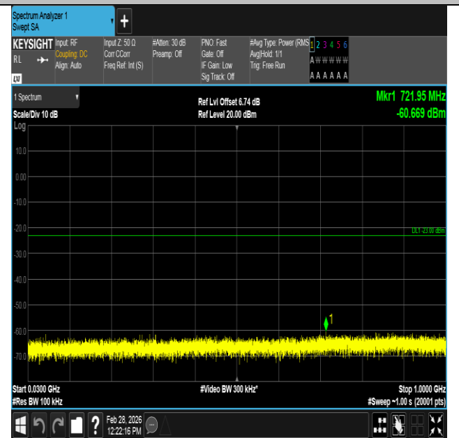
Band2-15MHz-16QAM-18900-1RB#0-30~1000-PASS
