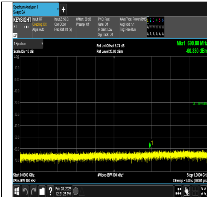
Band2-15MHz-QPSK-18900-1RB#0-30~1000-PASS
