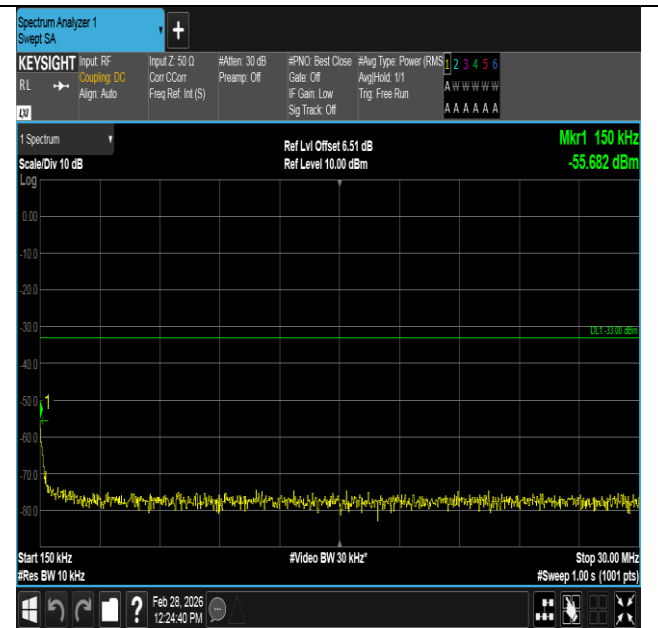
Band2-15MHz-QPSK-19125-1RB#0-0.15~30-PASS
