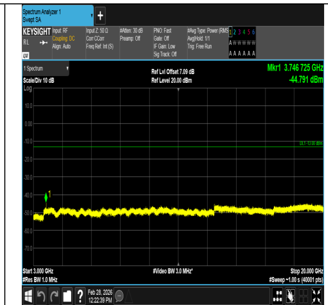
Band2-15MHz-16QAM-18900-1RB#0-3000~20000-PASS
