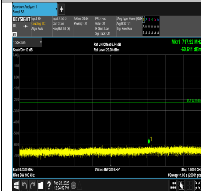
Band2-15MHz-QPSK-19125-1RB#0-30~1000-PASS
