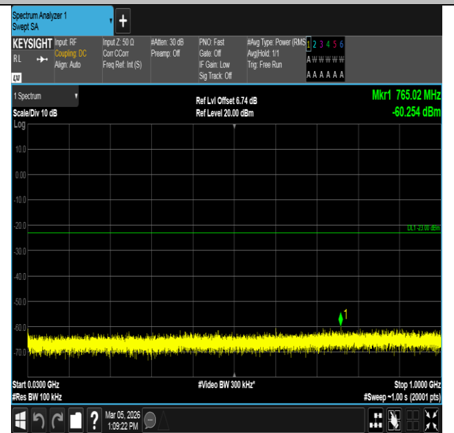
Band2-15MHz-16QAM-18675-75RB#0-30~1000-PASS
