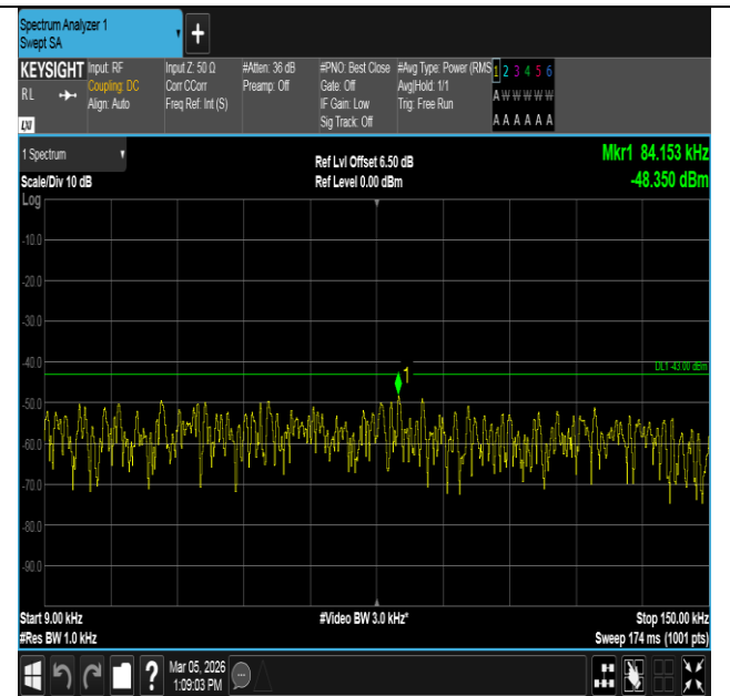
Band2-15MHz-16QAM-18675-75RB#0-0.009~0.15-PASS
