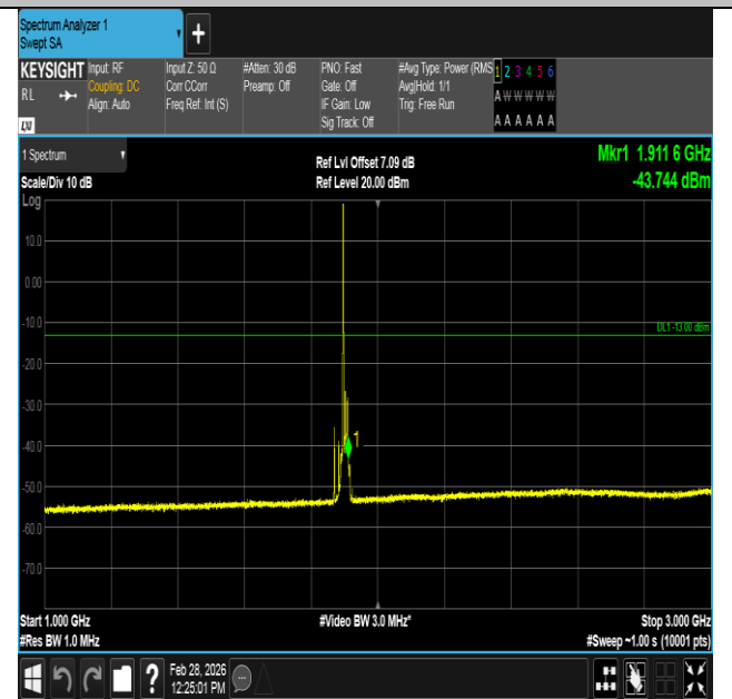
Band2-15MHz-QPSK-19125-1RB#0-1000~3000-PASS
