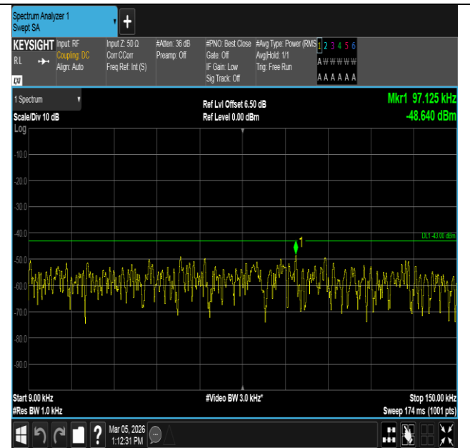
Band2-15MHz-16QAM-19125-75RB#0-0.009~0.15-PASS
