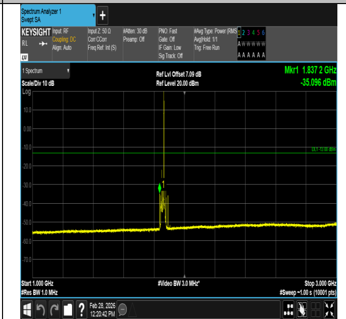
Band2-15MHz-16QAM-18675-1RB#74-1000~3000-PASS
