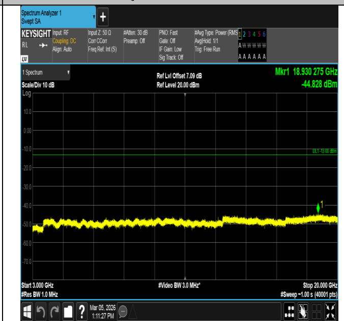
Band2-15MHz-16QAM-18900-75RB#0-3000~20000-PASS
