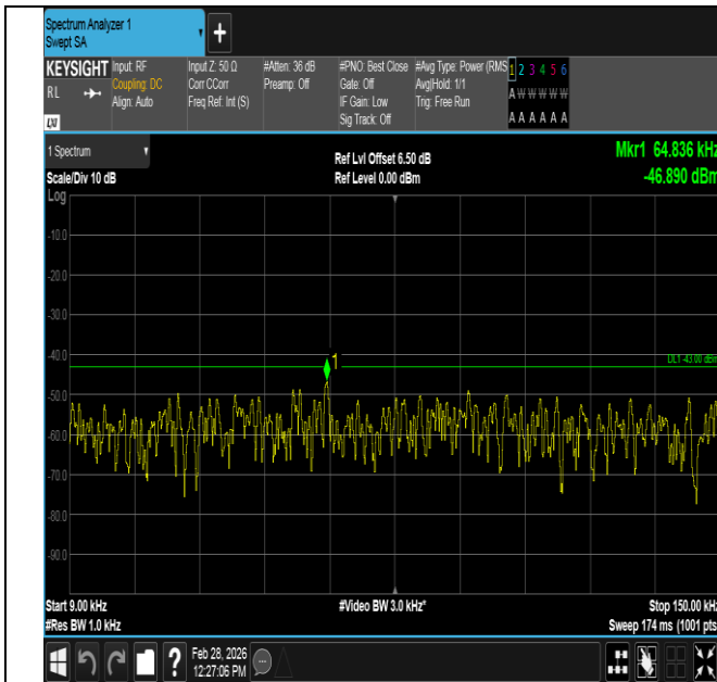
Band2-15MHz-16QAM-19125-1RB#74-0.009~0.15-PASS
