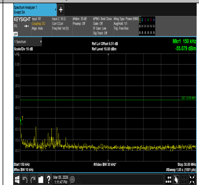
Band2-15MHz-QPSK-19125-75RB#0-0.15~30-PASS
