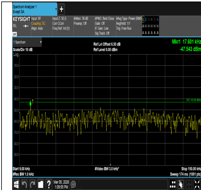
Band2-15MHz-QPSK-18900-75RB#0-0.009~0.15-PASS
