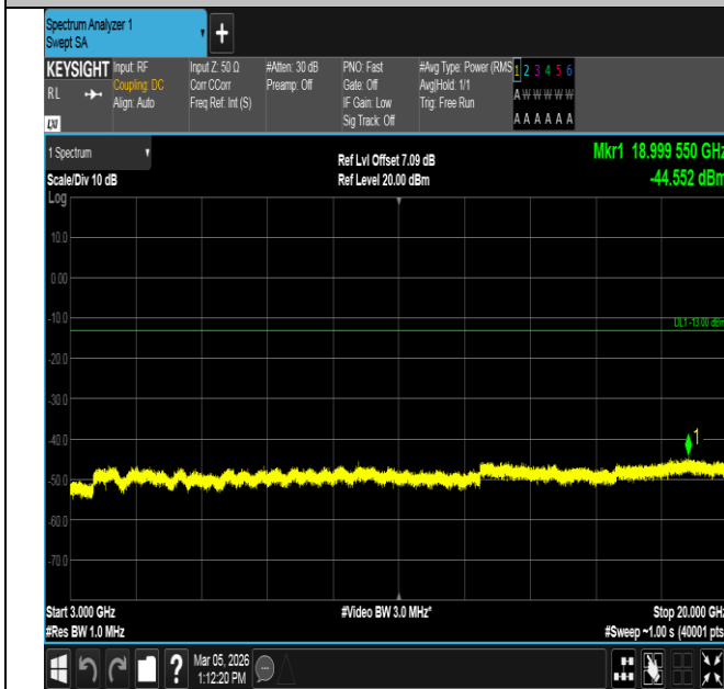
Band2-15MHz-QPSK-19125-75RB#0-3000~20000-PASS
