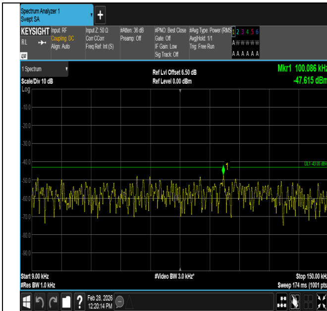
Band2-15MHz-16QAM-18675-1RB#74-0.009~0.15-PASS
