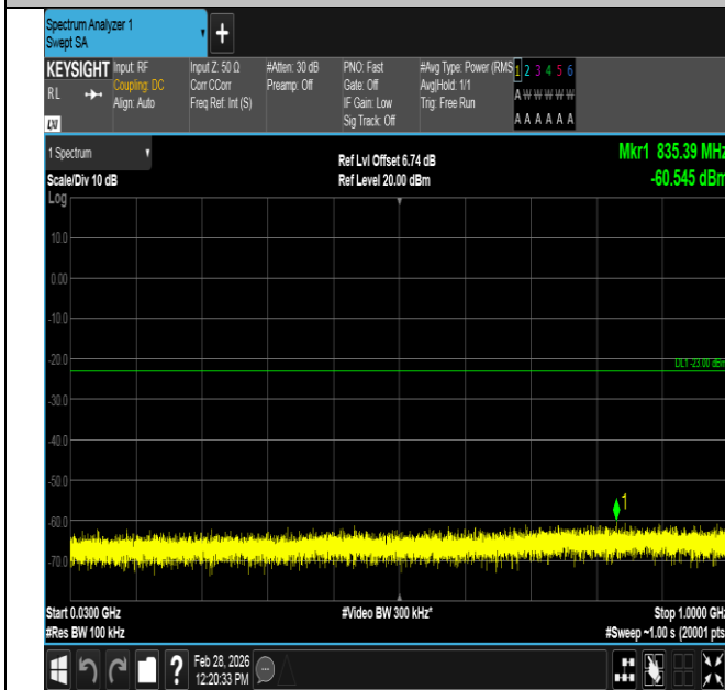
Band2-15MHz-16QAM-18675-1RB#74-30~1000-PASS
