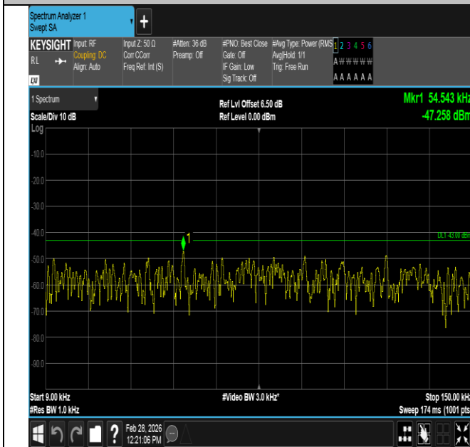
Band2-15MHz-QPSK-18900-1RB#0-0.009~0.15-PASS
