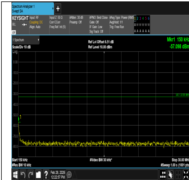
Band2-15MHz-QPSK-18900-1RB#74-0.15~30-PASS
