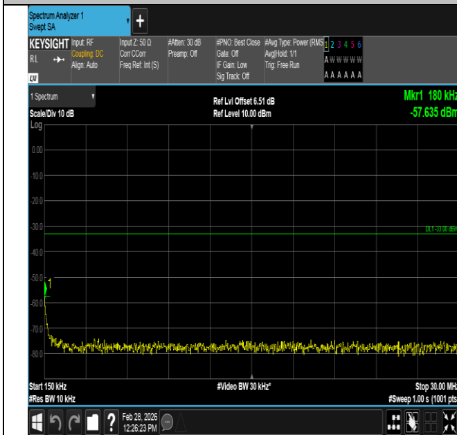
Band2-15MHz-QPSK-19125-1RB#74-0.15~30-PASS
