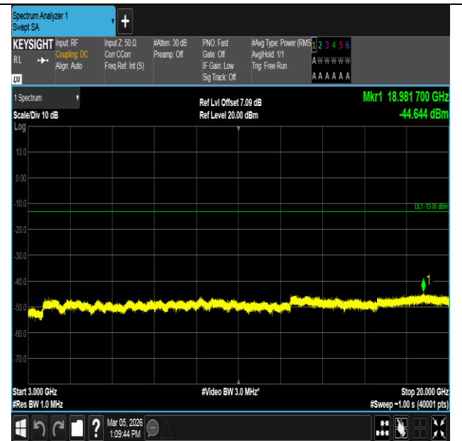
Band2-15MHz-16QAM-18675-75RB#0-3000~20000-PASS
