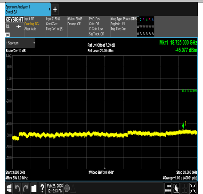
Band2-15MHz-16QAM-18675-1RB#0-3000~20000-PASS
