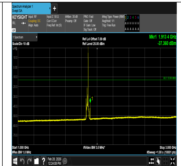
Band2-15MHz-16QAM-18900-1RB#74-1000~3000-PASS
