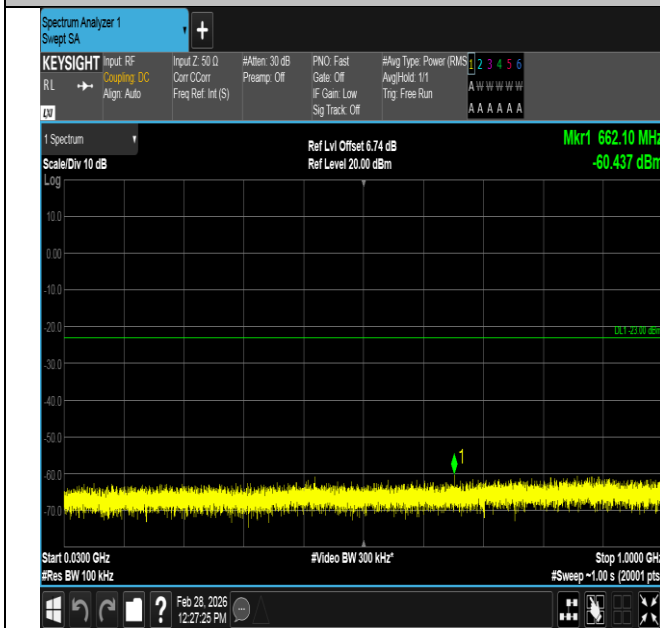
Band2-15MHz-16QAM-19125-1RB#74-30~1000-PASS
