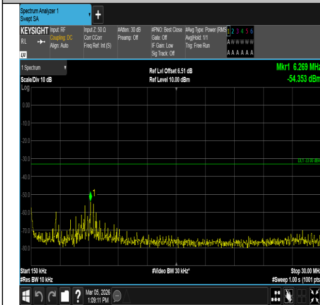
Band2-15MHz-16QAM-18675-75RB#0-0.15~30-PASS
