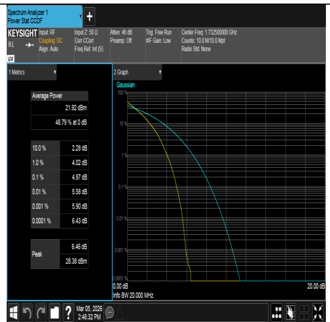
Band4-20MHz-QPSK-20175-100RB#0-PASS
