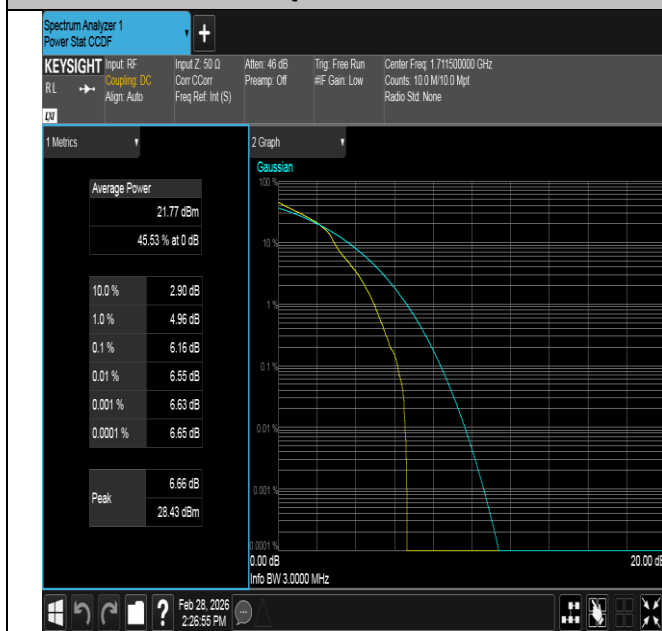
Band4-3MHz-16QAM-19965-1RB#0-PASS
