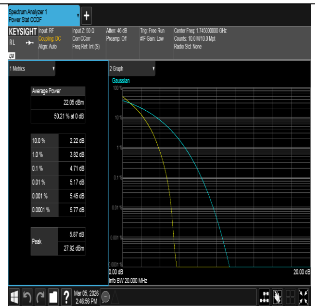
Band4-20MHz-QPSK-20300-100RB#0-PASS
