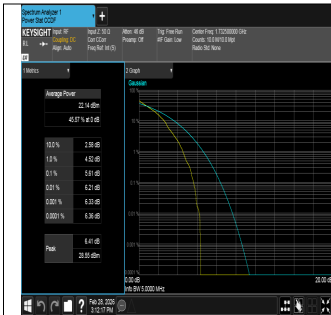
Band4-5MHz-QPSK-20175-1RB#0-PASS
