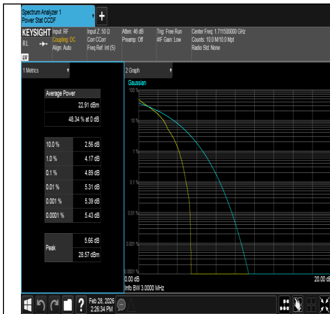
Band4-3MHz-QPSK-19965-1RB#0-PASS
