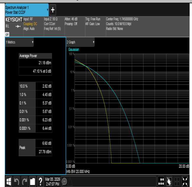
Band4-20MHz-16QAM-20300-100RB#0-PASS
