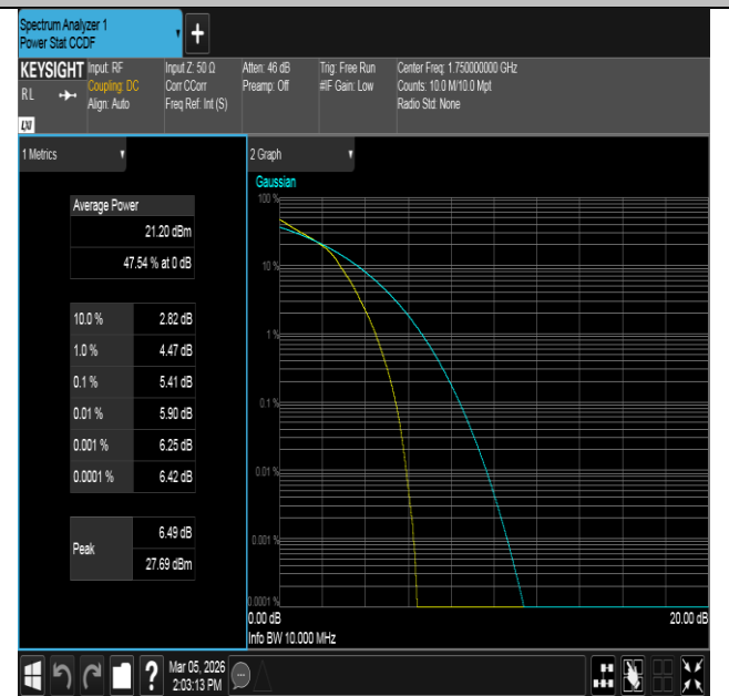
Band4-10MHz-16QAM-20350-50RB#0-PASS
