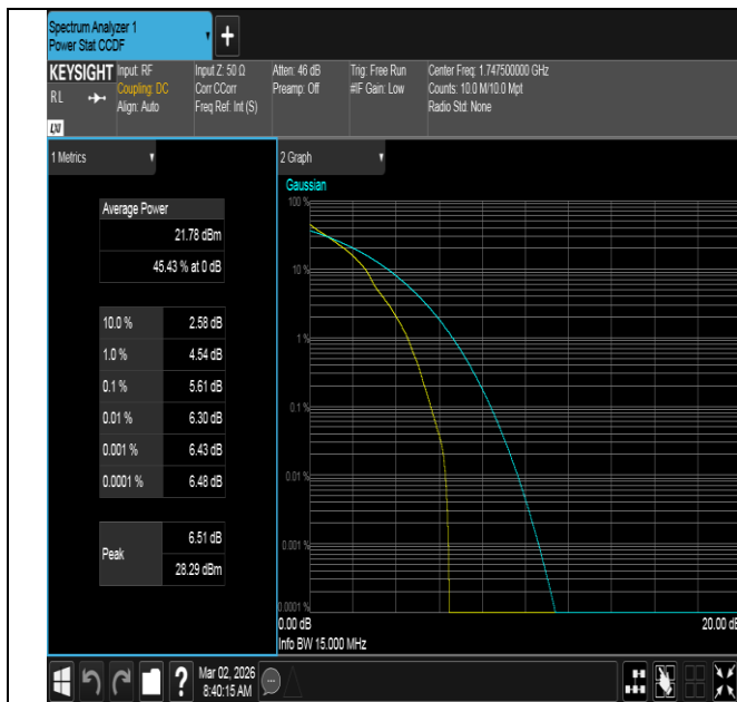
Band4-15MHz-QPSK-20325-1RB#0-PASS
