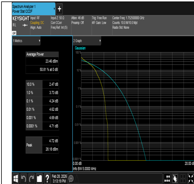
Band4-5MHz-QPSK-20375-1RB#0-PASS
