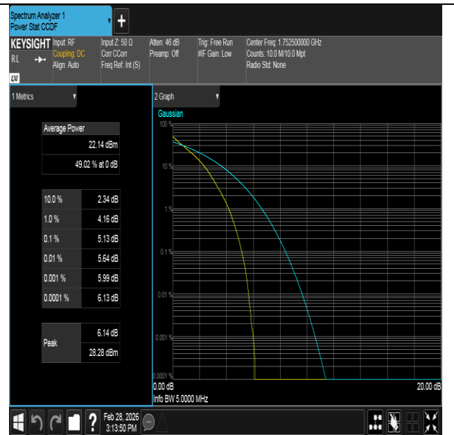
Band4-5MHz-QPSK-20375-25RB#0-PASS
