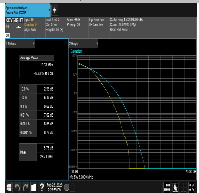
Band4-3MHz-16QAM-20175-15RB#0-PASS
