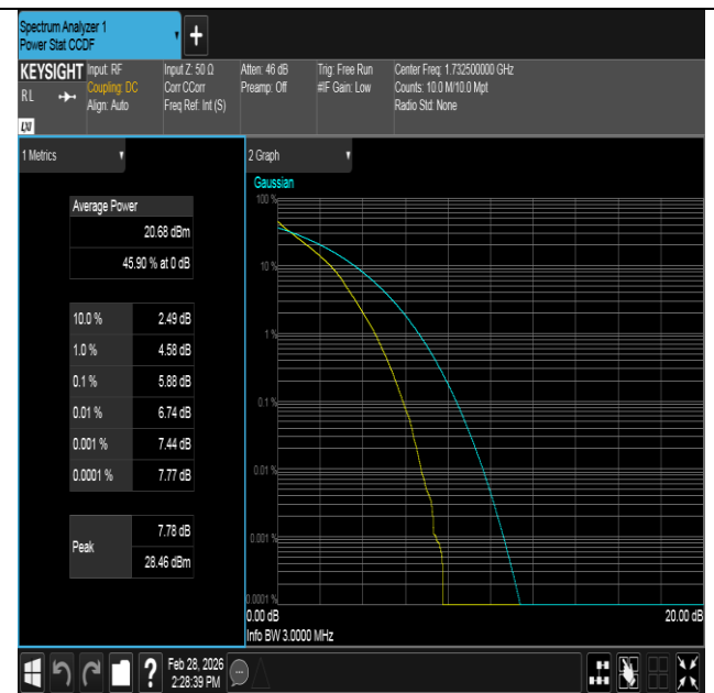
Band4-3MHz-QPSK-20175-15RB#0-PASS
