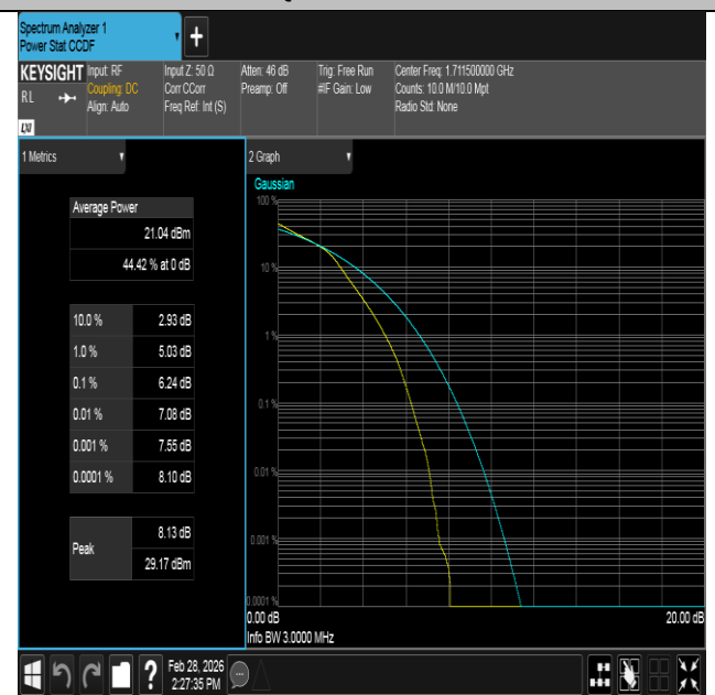
Band4-3MHz-16QAM-19965-15RB#0-PASS
