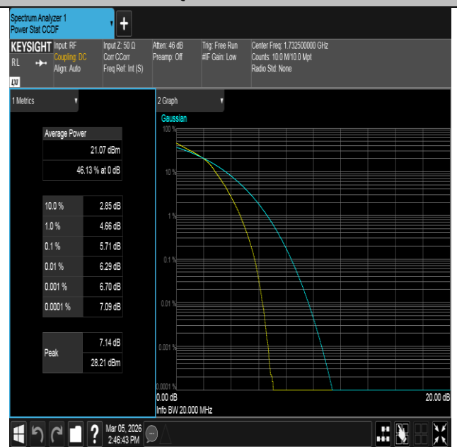
Band4-20MHz-16QAM-20175-100RB#0-PASS
