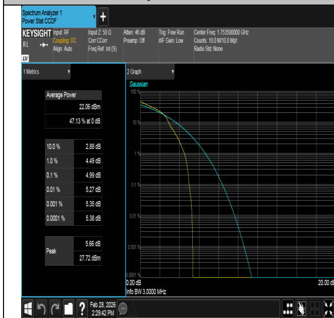
Band4-3MHz-16QAM-20385-1RB#0-PASS
