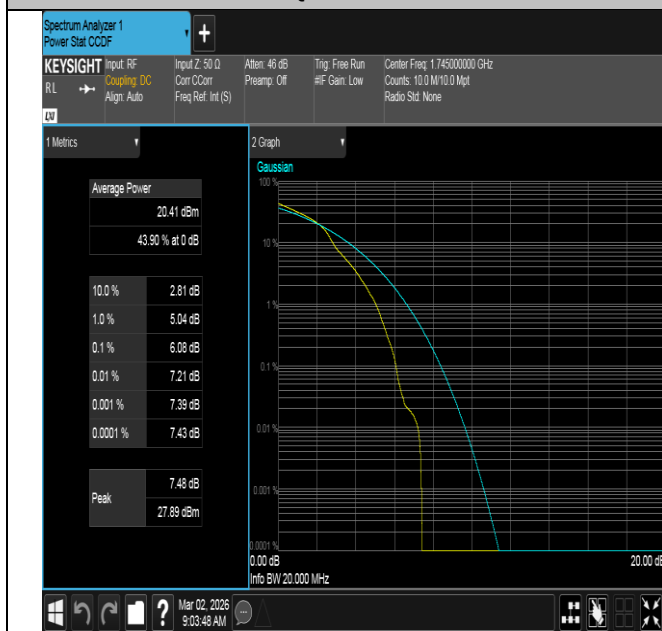
Band4-20MHz-16QAM-20300-1RB#0-PASS
