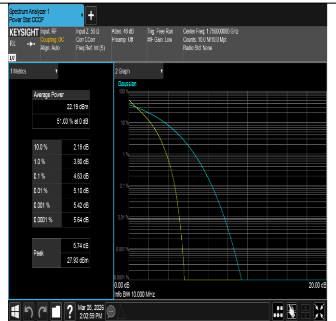
Band4-10MHz-QPSK-20350-50RB#0-PASS
