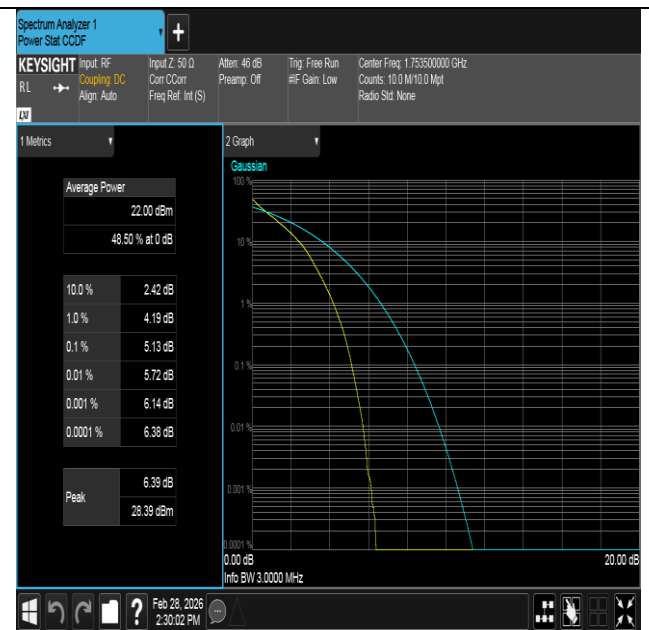
Band4-3MHz-QPSK-20385-15RB#0-PASS
