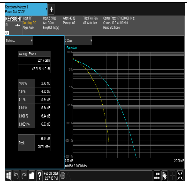
Band4-3MHz-QPSK-19965-15RB#0-PASS
