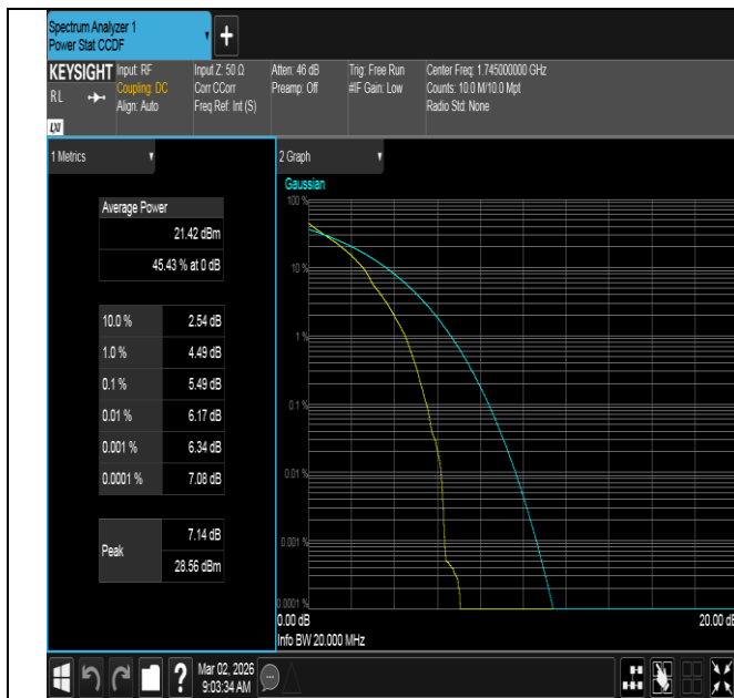
Band4-20MHz-QPSK-20300-1RB#0-PASS
