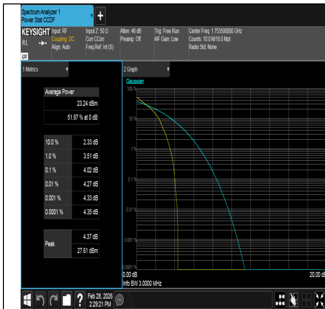
Band4-3MHz-QPSK-20385-1RB#0-PASS
