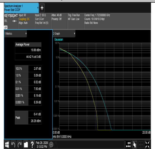
Band4-5MHz-16QAM-20175-25RB#0-PASS
