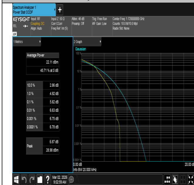
Band4-20MHz-16QAM-20050-1RB#0-PASS
