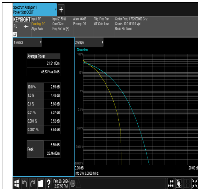
Band4-3MHz-QPSK-20175-1RB#0-PASS
