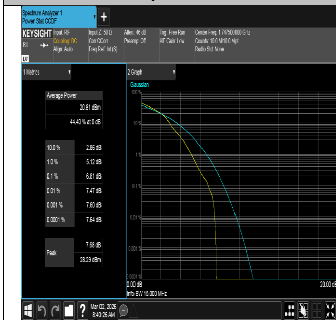
Band4-15MHz-16QAM-20325-1RB#0-PASS
