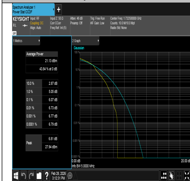
Band4-5MHz-16QAM-20175-1RB#0-PASS
