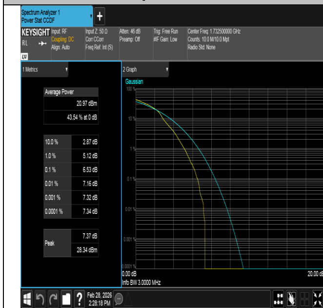
Band4-3MHz-16QAM-20175-1RB#0-PASS
