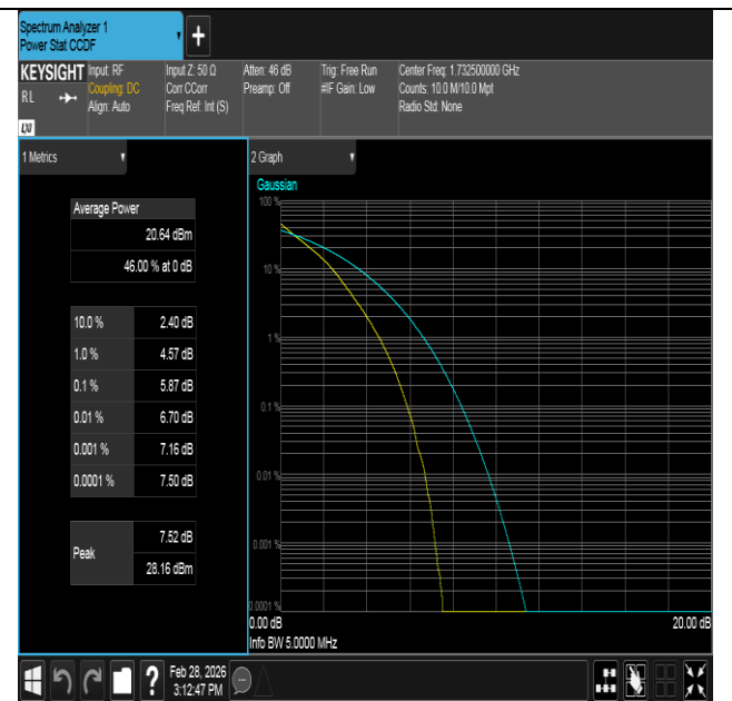
Band4-5MHz-QPSK-20175-25RB#0-PASS
