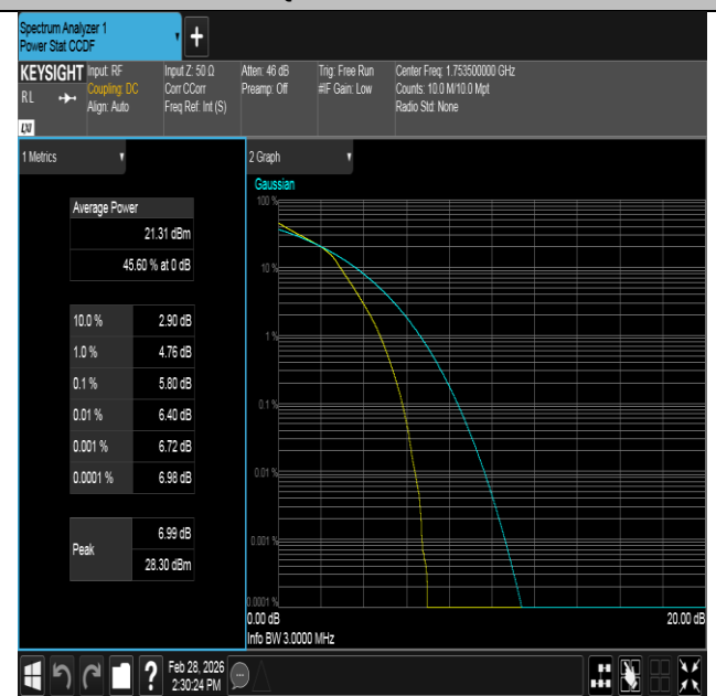
Band4-3MHz-16QAM-20385-15RB#0-PASS
