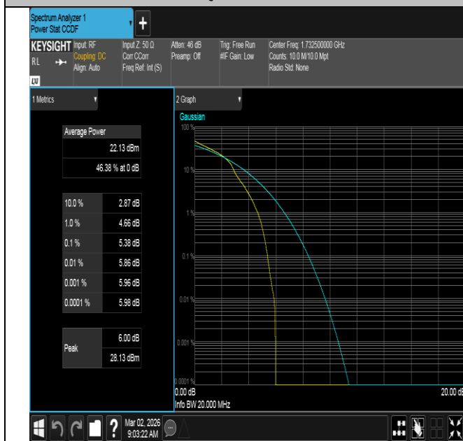
Band4-20MHz-16QAM-20175-1RB#0-PASS
