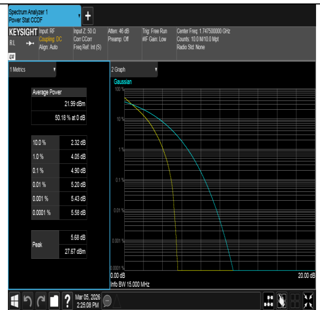
Band4-15MHz-QPSK-20325-75RB#0-PASS
