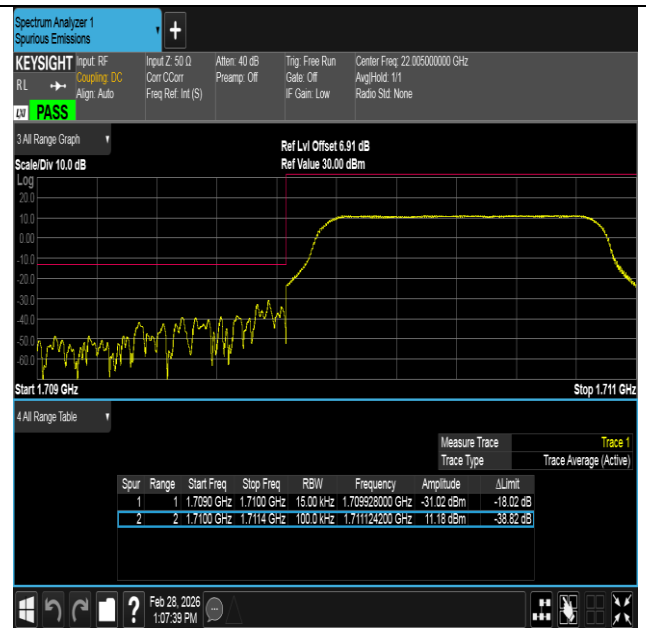
Band4-1.4MHz-16QAM-19957-6RB#0-PASS
