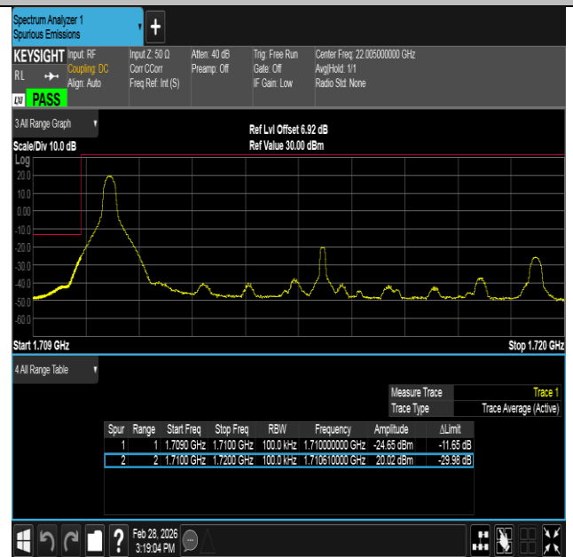
Band4-10MHz-16QAM-20000-1RB#0-PASS
