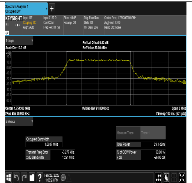
Band4-1.4MHz-16QAM-20393-6RB#0-PASS
