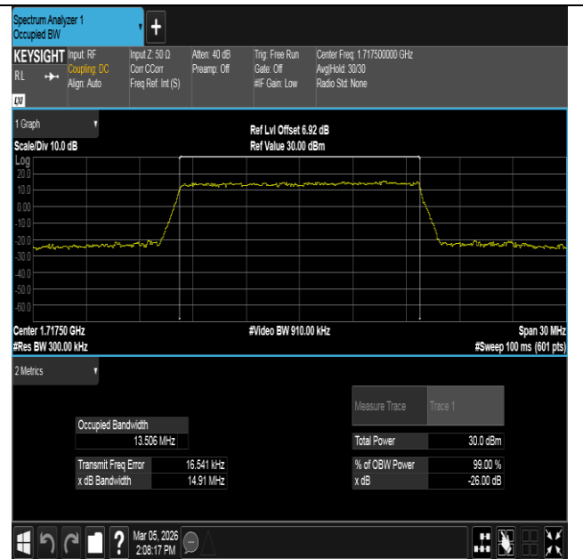
Band4-15MHz-16QAM-20025-75RB#0-PASS
