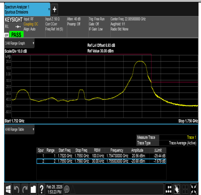
Band4-3MHz-QPSK-20385-1RB#14-PASS
