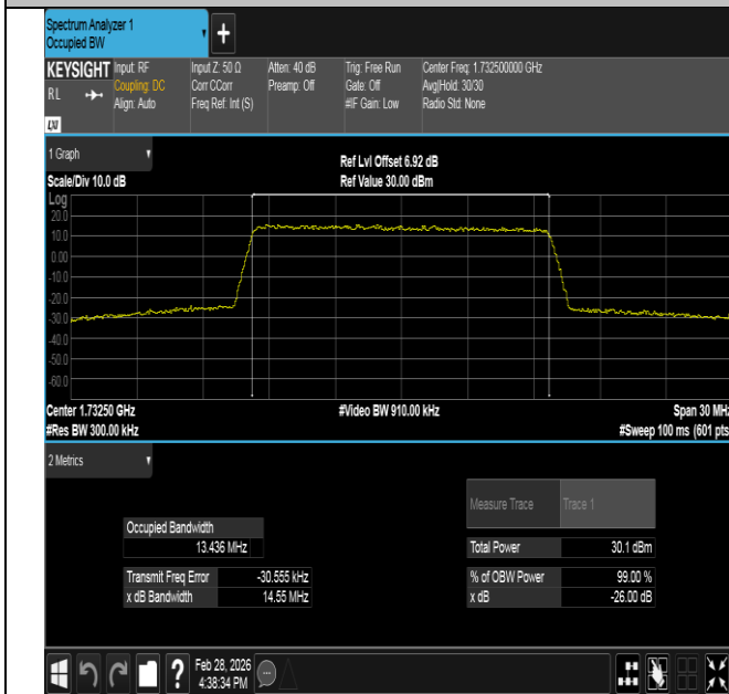
Band4-15MHz-QPSK-20175-75RB#0-PASS
