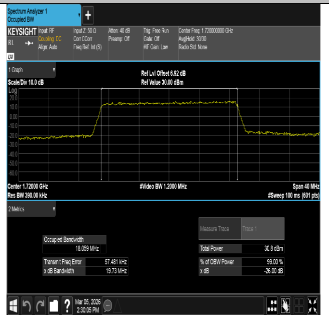
Band4-20MHz-16QAM-20050-100RB#0-PASS
