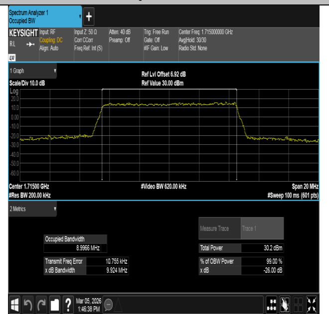
Band4-10MHz-16QAM-20000-50RB#0-PASS
