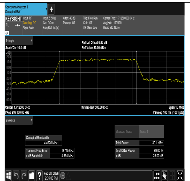
Band4-5MHz-16QAM-19975-25RB#0-PASS
