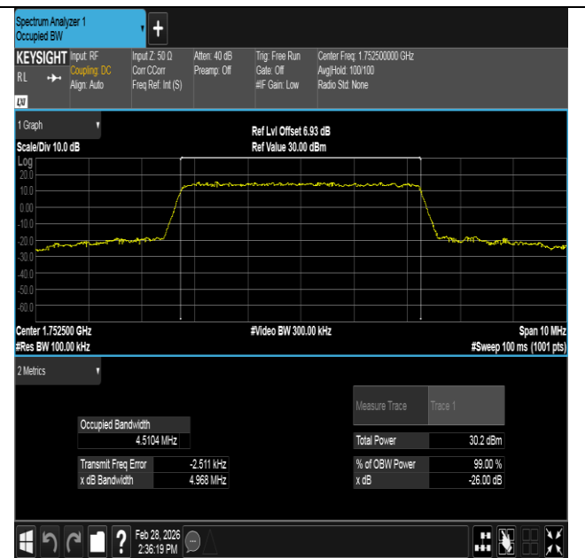
Band4-5MHz-16QAM-20375-25RB#0-PASS
