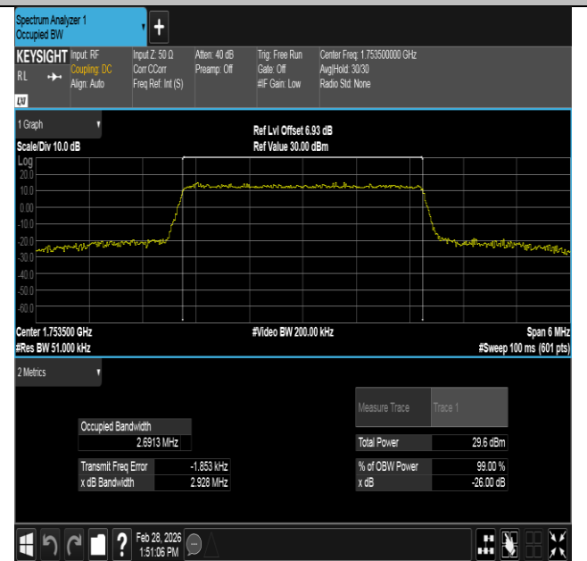
Band4-3MHz-16QAM-20385-15RB#0-PASS
