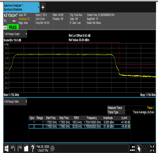
Band4-3MHz-16QAM-20385-15RB#0-PASS
