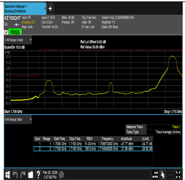
Band4-5MHz-QPSK-19975-1RB#24-PASS
