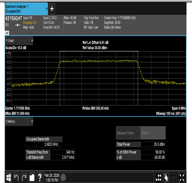
Band4-3MHz-16QAM-19965-15RB#0-PASS
