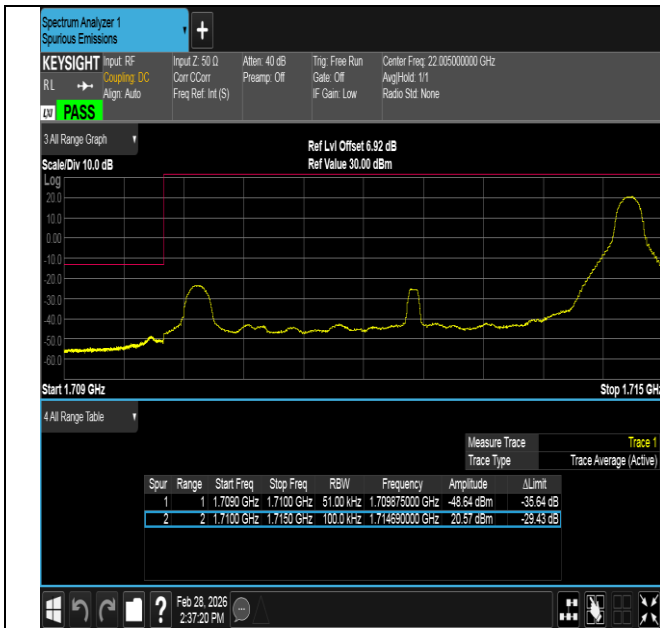
Band4-5MHz-16QAM-19975-1RB#24-PASS
