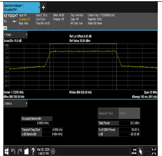
Band4-10MHz-16QAM-20175-50RB#0-PASS
