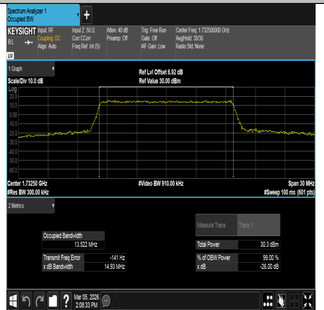
Band4-15MHz-16QAM-20175-75RB#0-PASS
