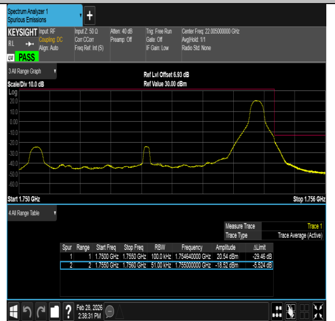
Band4-5MHz-QPSK-20375-1RB#24-PASS
