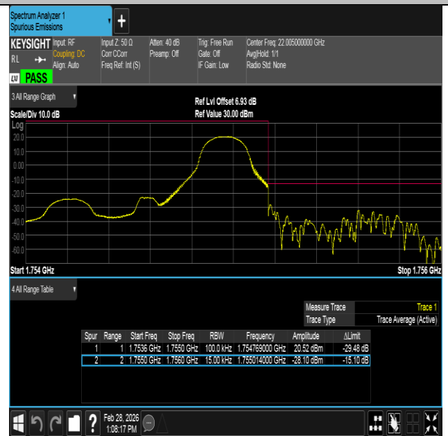
Band4-1.4MHz-QPSK-20393-1RB#5-PASS
