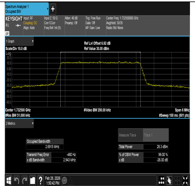
Band4-3MHz-16QAM-20175-15RB#0-PASS
