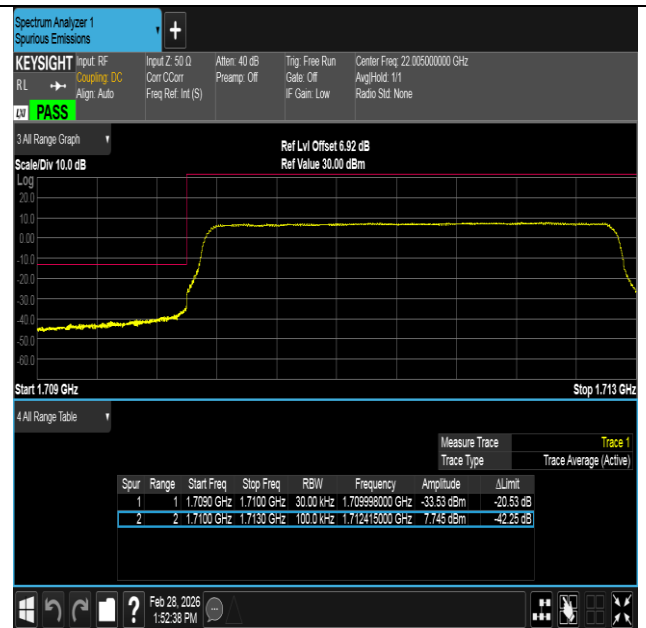
Band4-3MHz-16QAM-19965-15RB#0-PASS
