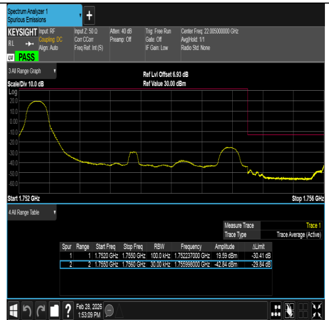
Band4-3MHz-16QAM-20385-1RB#0-PASS
