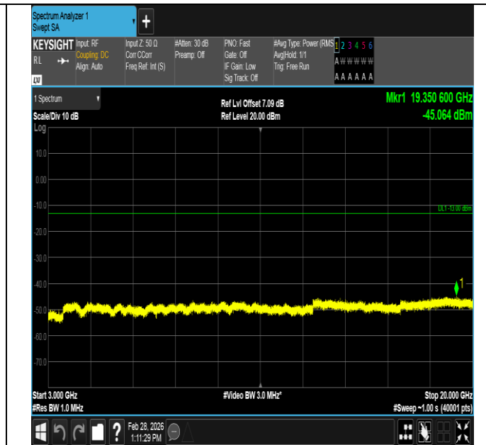
Band4-1.4MHz-QPSK-19957-1RB#5-3000~20000-PASS
