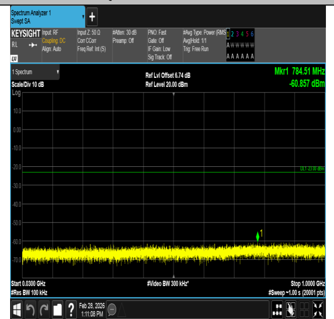
Band4-1.4MHz-QPSK-19957-1RB#5-30~1000-PASS
