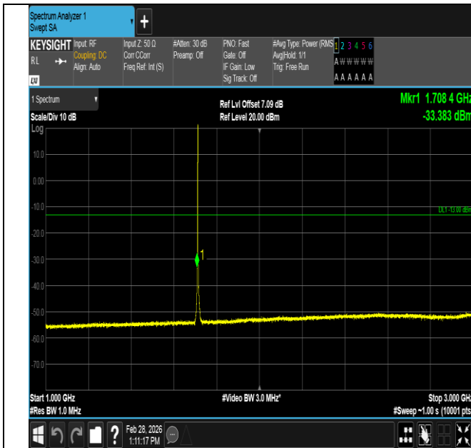
Band4-1.4MHz-QPSK-19957-1RB#5-1000~3000-PASS
