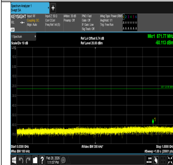
Band4-1.4MHz-16QAM-19957-1RB#5-30~1000-PASS
