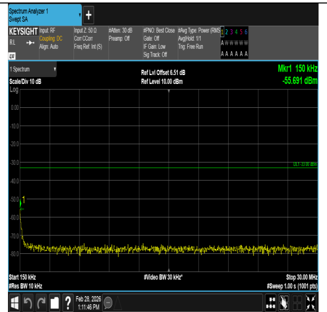
Band4-1.4MHz-16QAM-19957-1RB#5-0.15~30-PASS
