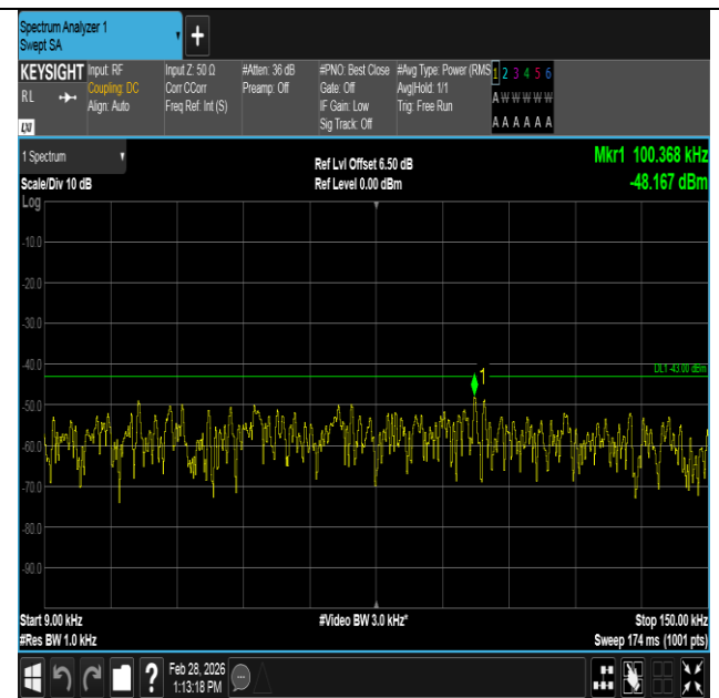
Band4-1.4MHz-16QAM-19957-6RB#0-0.009~0.15-PASS
