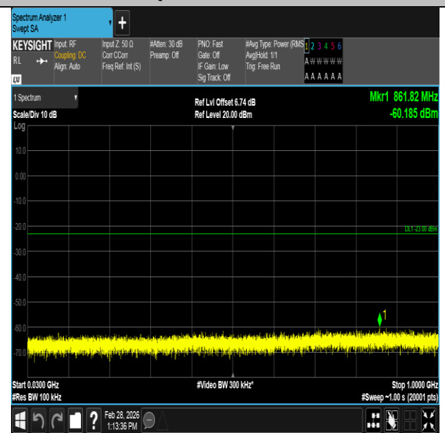
Band4-1.4MHz-16QAM-19957-6RB#0-30~1000-PASS
