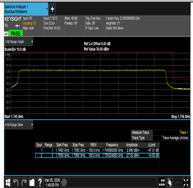
Band4-10MHz-16QAM-20350-50RB#0-PASS
