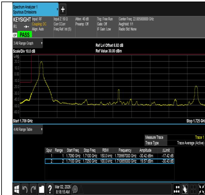
Band4-15MHz-QPSK-20025-1RB#0-PASS
