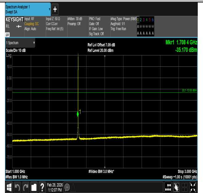
Band4-1.4MHz-16QAM-19957-1RB#5-1000~3000-PASS
