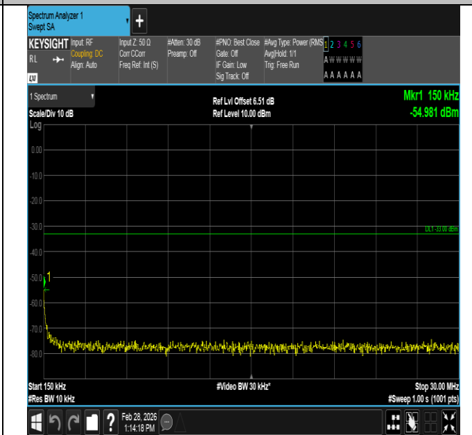
Band4-1.4MHz-QPSK-20175-1RB#0-0.15~30-PASS
