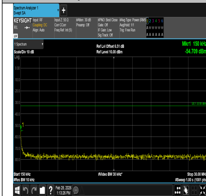
Band4-1.4MHz-16QAM-19957-6RB#0-0.15~30-PASS
