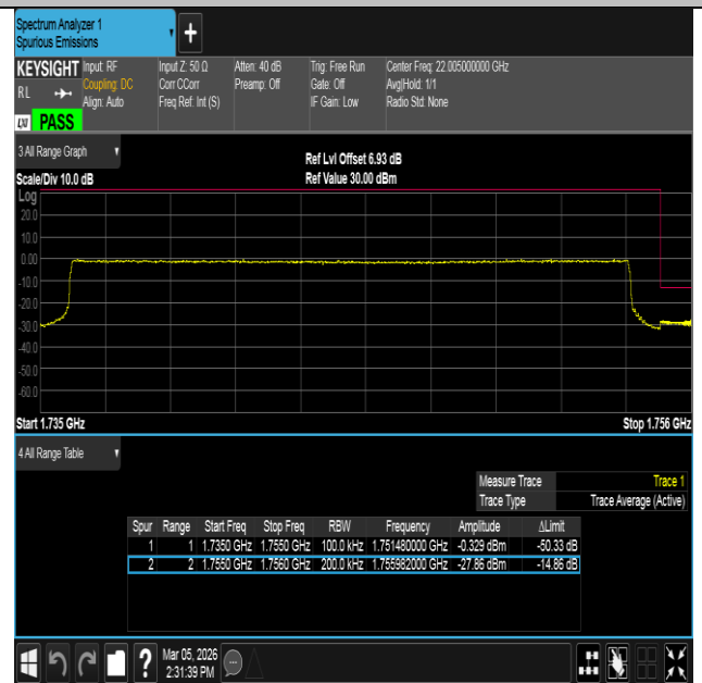
Band4-20MHz-16QAM-20300-100RB#0-PASS
