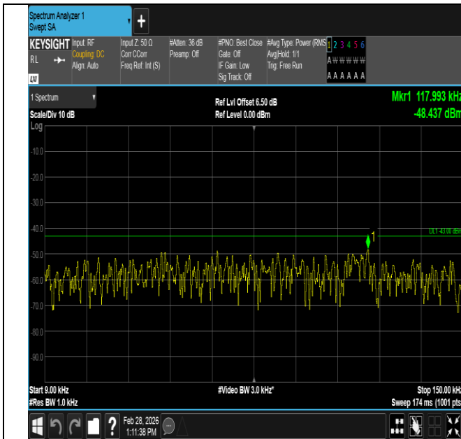
Band4-1.4MHz-16QAM-19957-1RB#5-0.009~0.15-PASS
