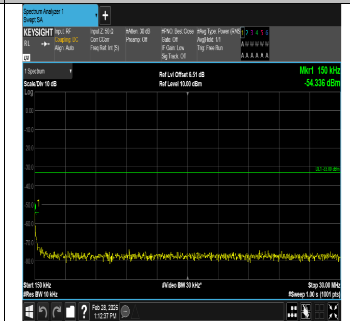
Band4-1.4MHz-QPSK-19957-6RB#0-0.15~30-PASS
