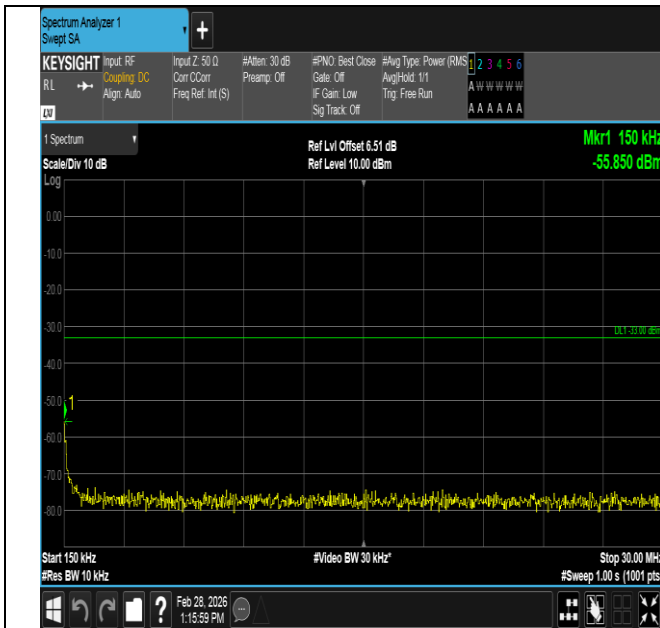
Band4-1.4MHz-QPSK-20175-1RB#5-0.15~30-PASS
