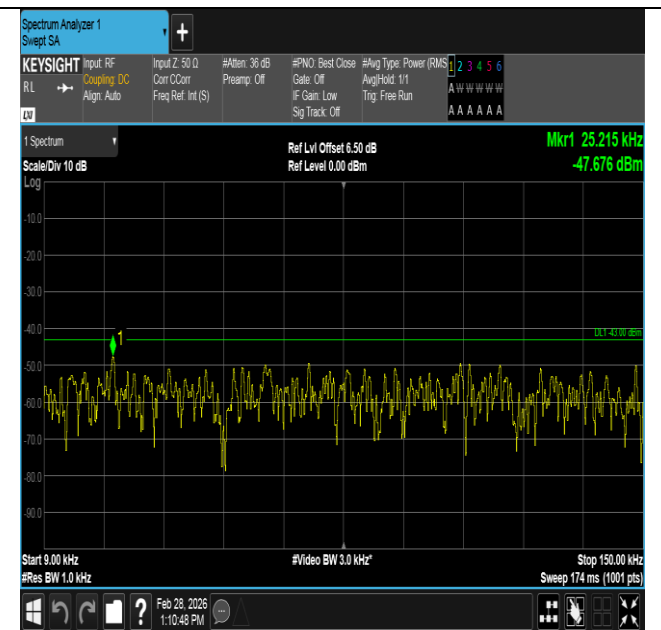
Band4-1.4MHz-QPSK-19957-1RB#5-0.009~0.15-PASS
