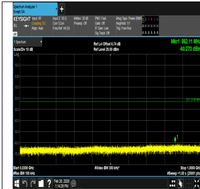
Band4-1.4MHz-QPSK-20175-1RB#0-30~1000-PASS
