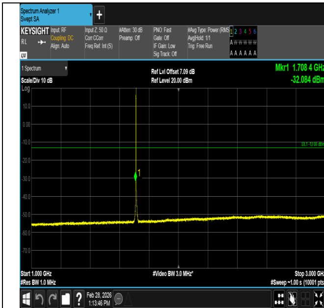
Band4-1.4MHz-16QAM-19957-6RB#0-1000~3000-PASS
