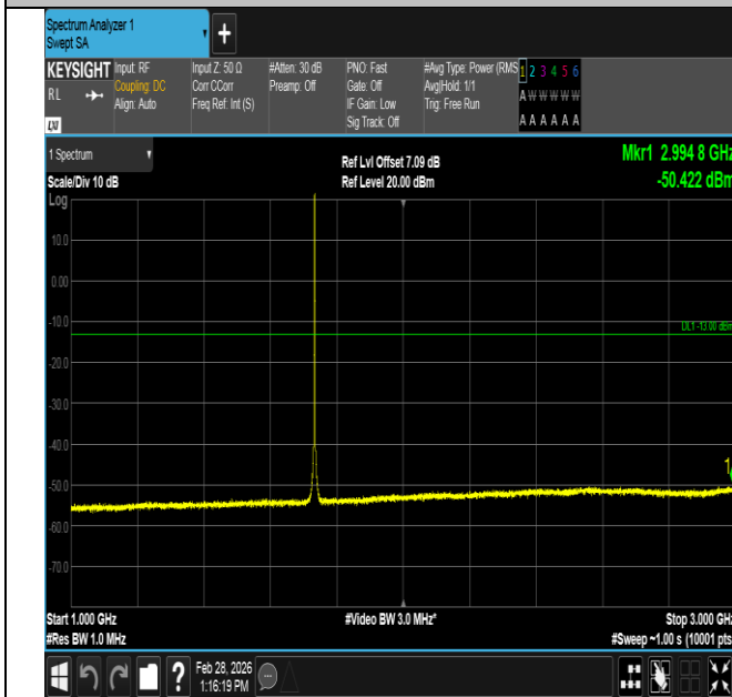
Band4-1.4MHz-QPSK-20175-1RB#5-1000~3000-PASS
