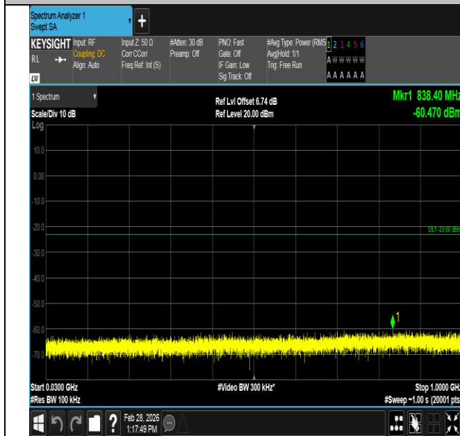
Band4-1.4MHz-QPSK-20175-6RB#0-30~1000-PASS
