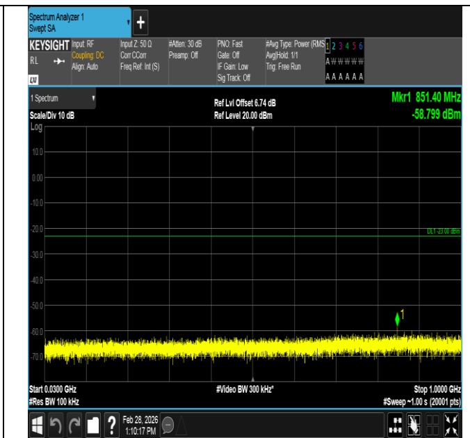
Band4-1.4MHz-16QAM-19957-1RB#0-30~1000-PASS
