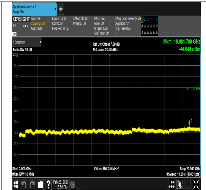
Band4-1.4MHz-16QAM-19957-6RB#0-3000~20000-PASS
