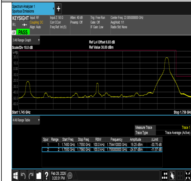
Band4-10MHz-16QAM-20350-1RB#49-PASS
