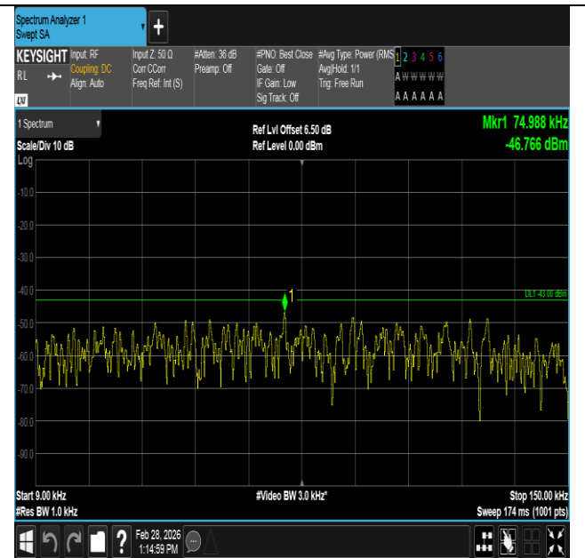
Band4-1.4MHz-16QAM-20175-1RB#0-0.009~0.15-PASS
