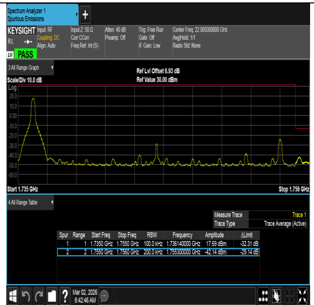
Band4-20MHz-16QAM-20300-1RB#0-PASS
