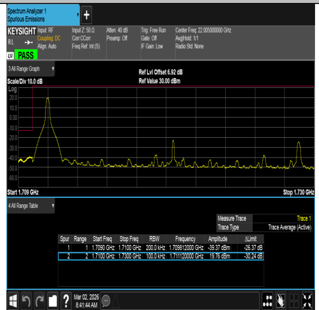
Band4-20MHz-16QAM-20050-1RB#0-PASS
