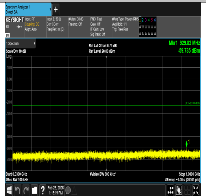
Band4-1.4MHz-16QAM-20175-1RB#0-30~1000-PASS
