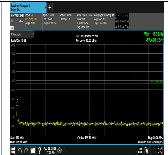
Band4-1.4MHz-QPSK-20175-6RB#0-0.15~30-PASS
