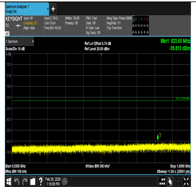
Band4-1.4MHz-QPSK-20175-1RB#5-30~1000-PASS
