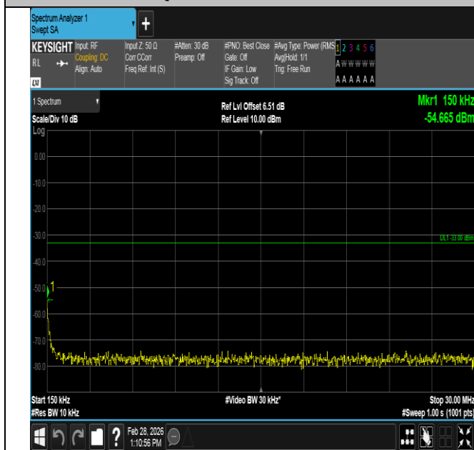
Band4-1.4MHz-QPSK-19957-1RB#5-0.15~30-PASS
