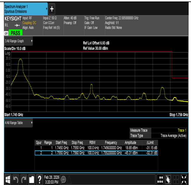
Band4-10MHz-16QAM-20350-1RB#0-PASS
