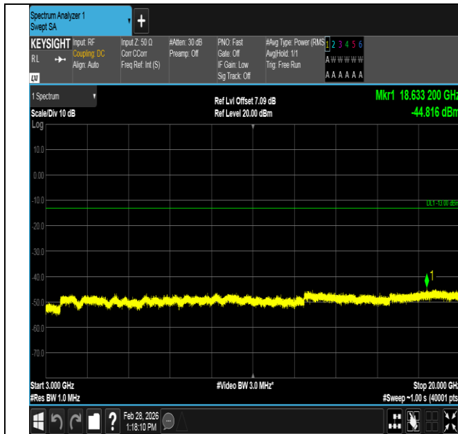
Band4-1.4MHz-QPSK-20175-6RB#0-3000~20000-PASS
