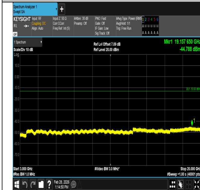
Band4-1.4MHz-QPSK-20175-1RB#0-3000~20000-PASS
