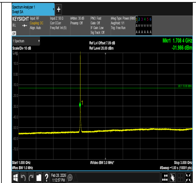
Band4-1.4MHz-QPSK-19957-6RB#0-1000~3000-PASS
