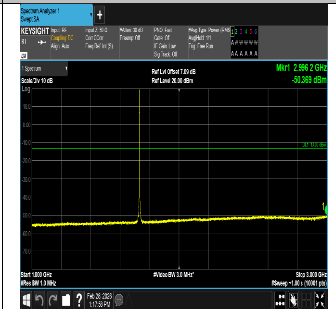
Band4-1.4MHz-QPSK-20175-6RB#0-1000~3000-PASS
