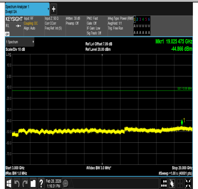
Band4-1.4MHz-QPSK-20175-1RB#5-3000~20000-PASS
