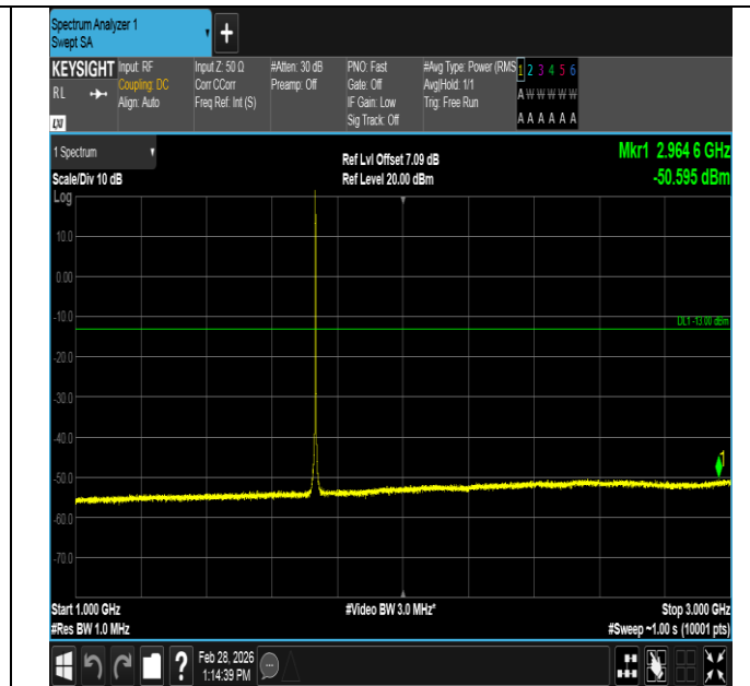
Band4-1.4MHz-QPSK-20175-1RB#0-1000~3000-PASS
