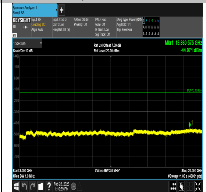
Band4-1.4MHz-16QAM-19957-1RB#0-3000~20000-PASS
