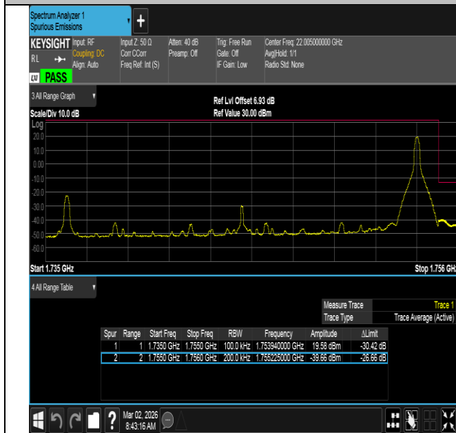
Band4-20MHz-16QAM-20300-1RB#99-PASS
