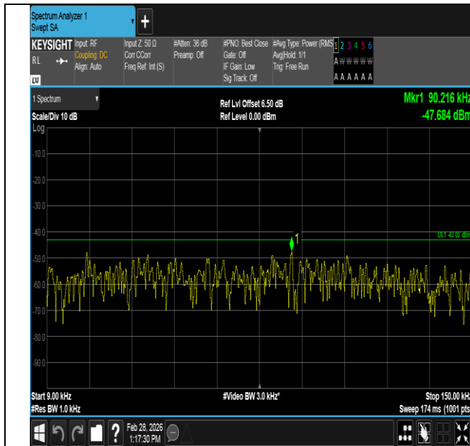
Band4-1.4MHz-QPSK-20175-6RB#0-0.009~0.15-PASS
