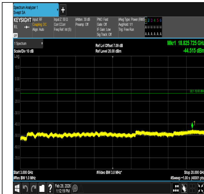
Band4-1.4MHz-16QAM-19957-1RB#5-3000~20000-PASS
