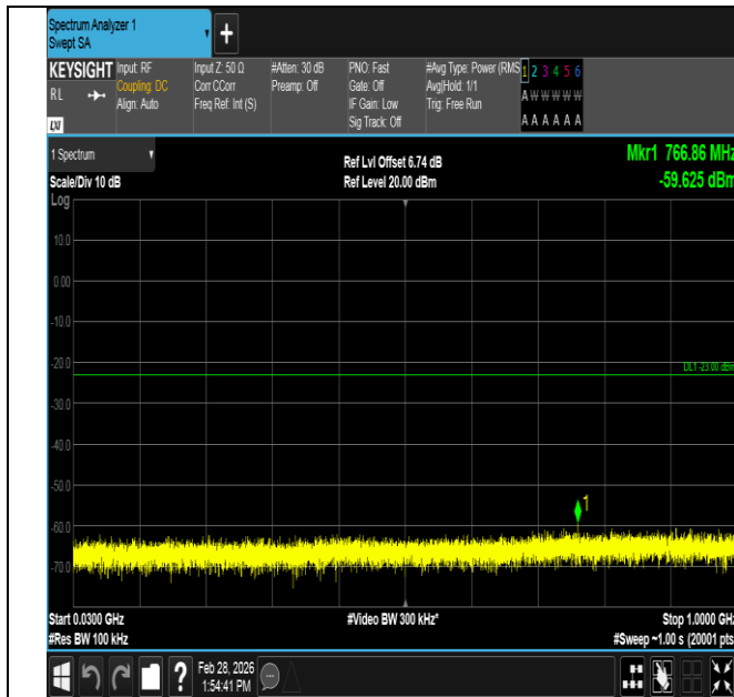
Band4-3MHz-QPSK-19965-1RB#0-30~1000-PASS
