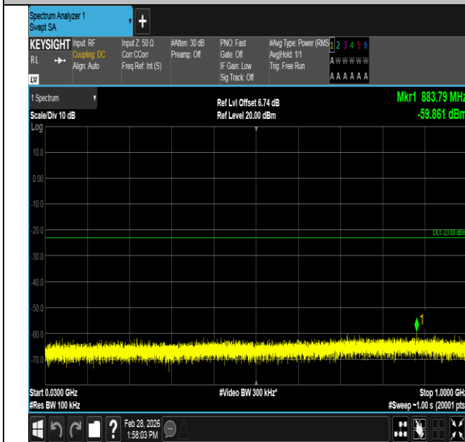
Band4-3MHz-QPSK-19965-15RB#0-30~1000-PASS
