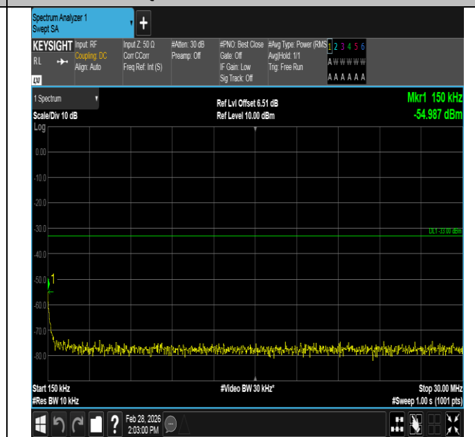
Band4-3MHz-QPSK-20175-15RB#0-0.15~30-PASS
