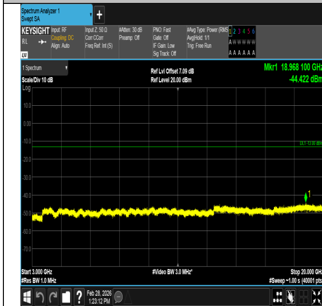
Band4-1.4MHz-QPSK-20393-6RB#0-3000~20000-PASS
