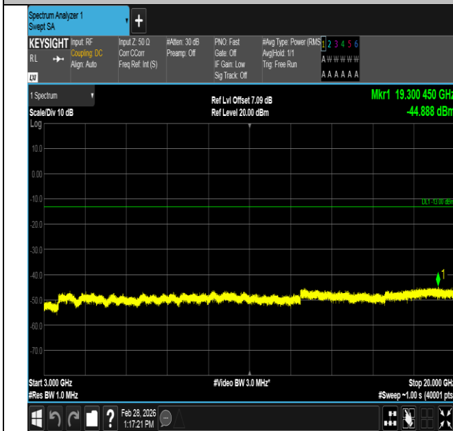
Band4-1.4MHz-16QAM-20175-1RB#5-3000~20000-PASS
