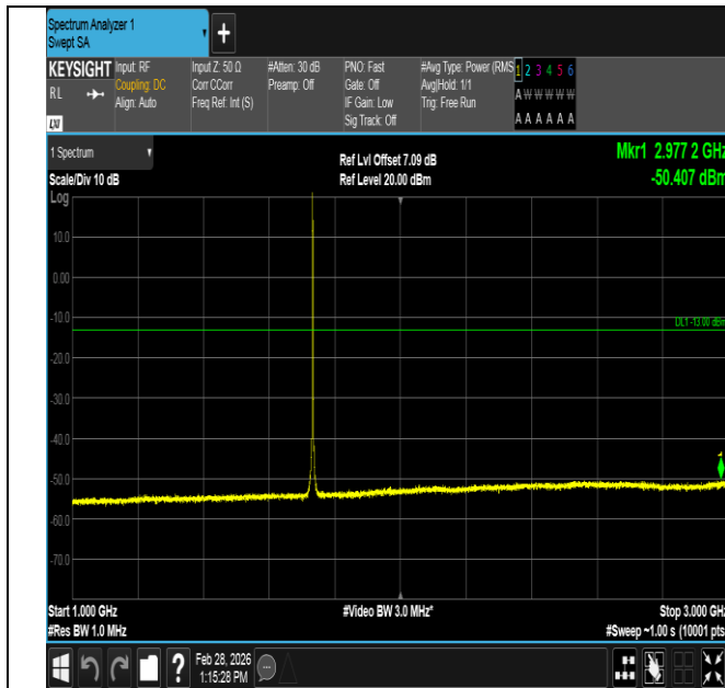
Band4-1.4MHz-16QAM-20175-1RB#0-1000~3000-PASS
