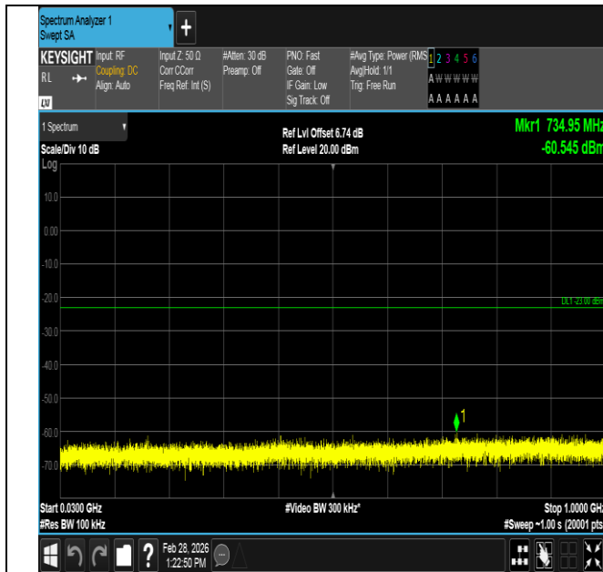
Band4-1.4MHz-QPSK-20393-6RB#0-30~1000-PASS
