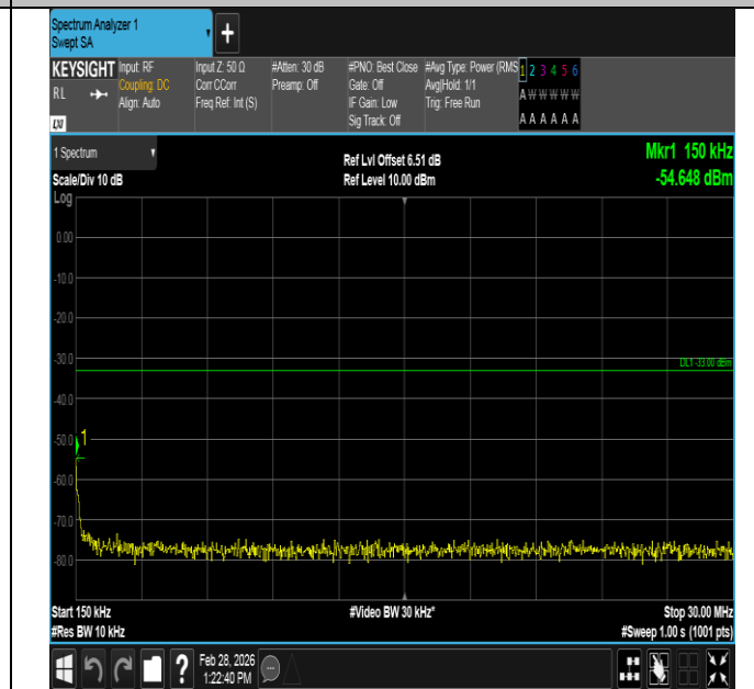
Band4-1.4MHz-QPSK-20393-6RB#0-0.15~30-PASS
