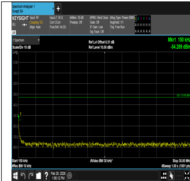
Band4-3MHz-QPSK-19965-1RB#14-0.15~30-PASS
