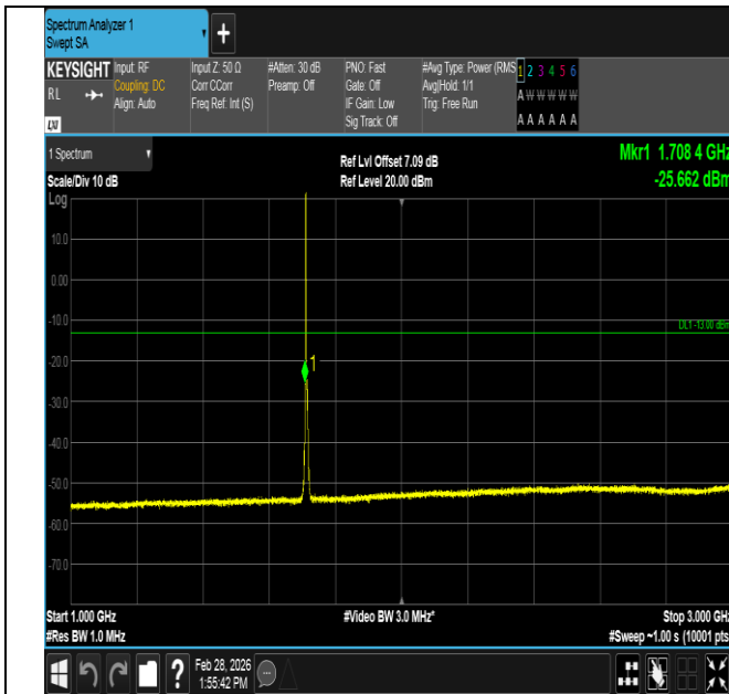
Band4-3MHz-16QAM-19965-1RB#0-1000~3000-PASS
