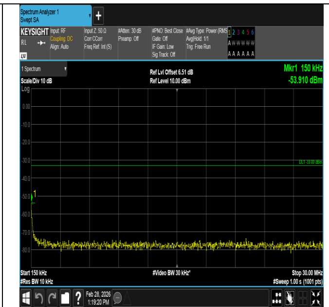
Band4-1.4MHz-QPSK-20393-1RB#0-0.15~30-PASS
