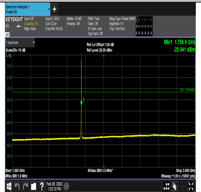
Band4-1.4MHz-16QAM-20393-1RB#5-1000~3000-PASS
