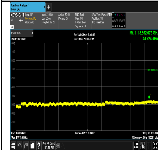
Band4-3MHz-16QAM-19965-1RB#14-3000~20000-PASS
