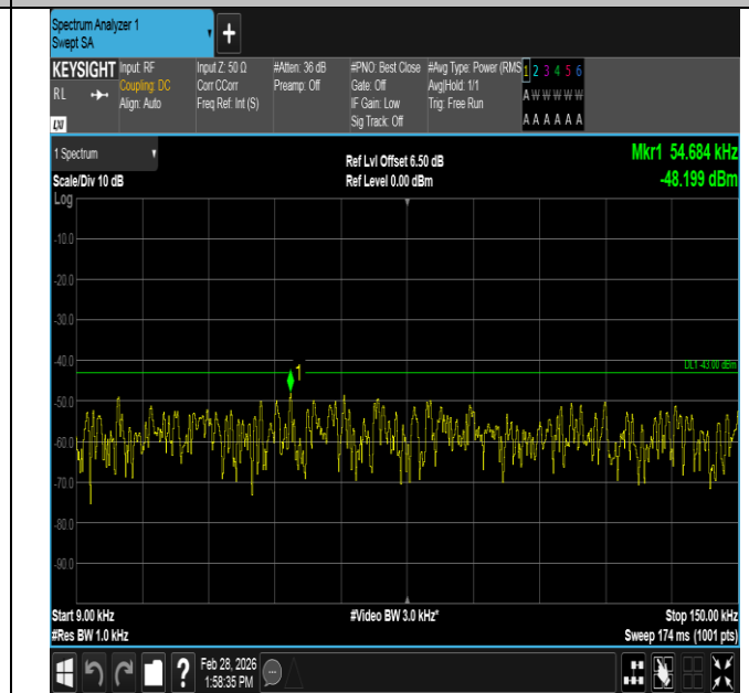
Band4-3MHz-16QAM-19965-15RB#0-0.009~0.15-PASS
