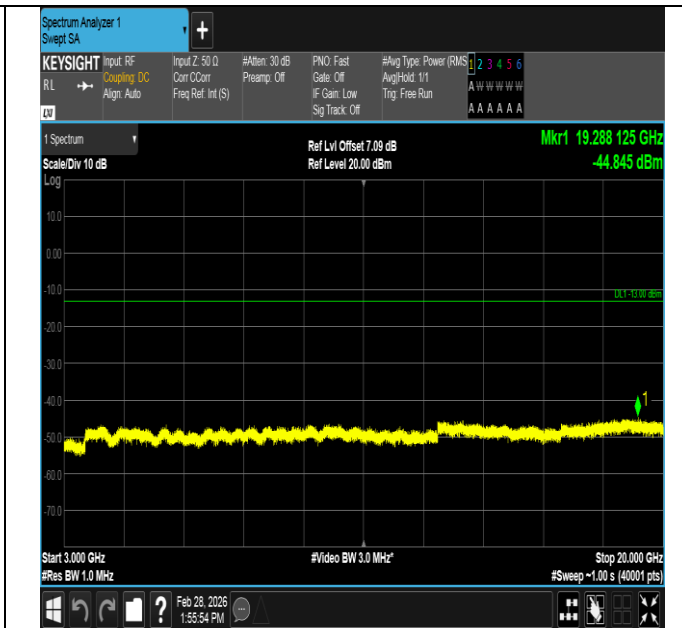
Band4-3MHz-16QAM-19965-1RB#0-3000~20000-PASS
