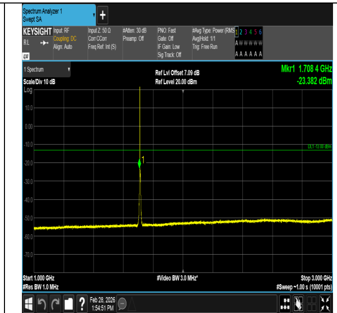
Band4-3MHz-QPSK-19965-1RB#0-1000~3000-PASS
