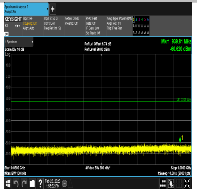
Band4-3MHz-16QAM-19965-1RB#0-30~1000-PASS
