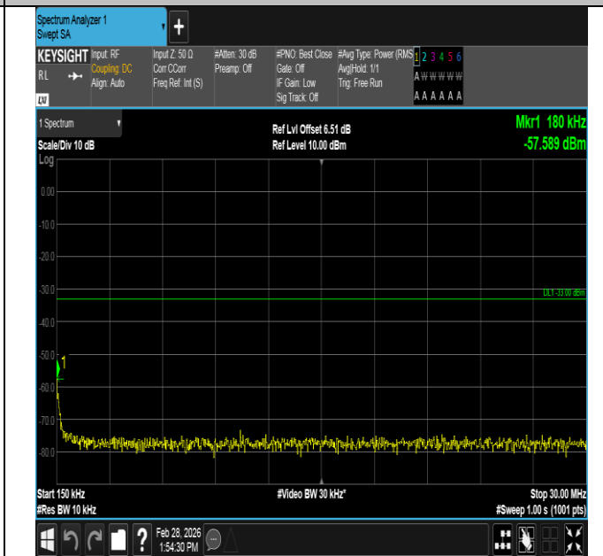
Band4-3MHz-QPSK-19965-1RB#0-0.15~30-PASS
