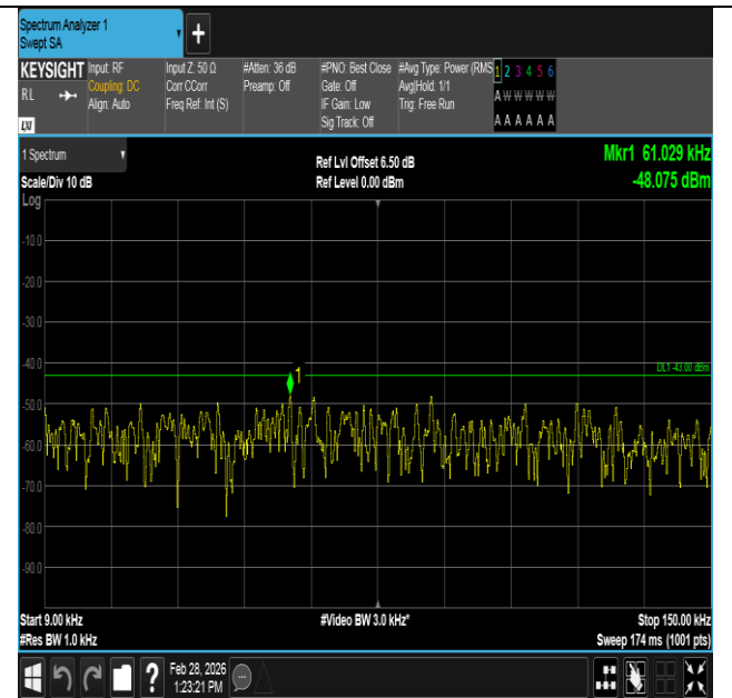
Band4-1.4MHz-16QAM-20393-6RB#0-0.009~0.15-PASS
