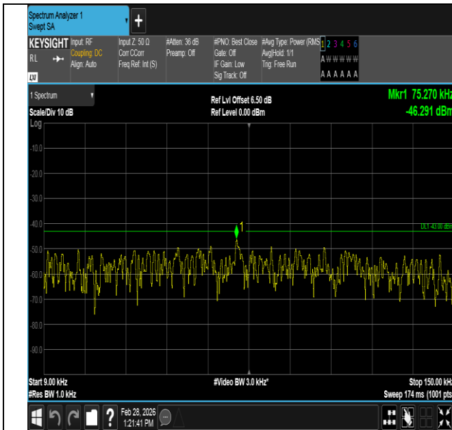
Band4-1.4MHz-16QAM-20393-1RB#5-0.009~0.15-PASS
