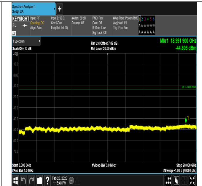
Band4-1.4MHz-16QAM-20175-1RB#0-3000~20000-PASS
