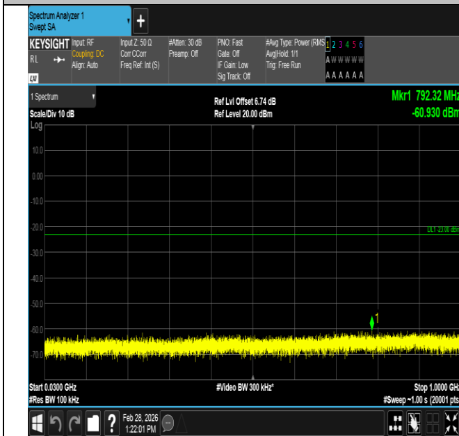
Band4-1.4MHz-16QAM-20393-1RB#5-30~1000-PASS
