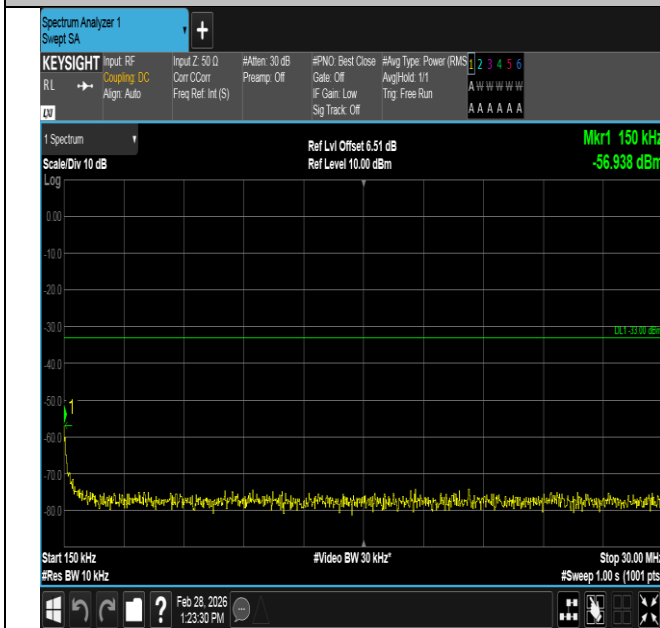
Band4-1.4MHz-16QAM-20393-6RB#0-0.15~30-PASS
