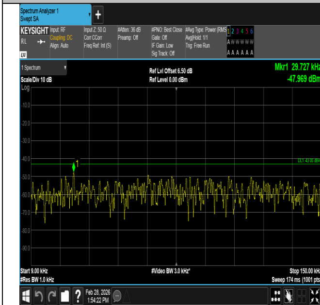
Band4-3MHz-QPSK-19965-1RB#0-0.009~0.15-PASS
