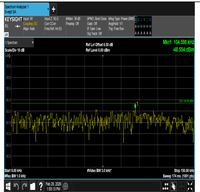
Band4-3MHz-16QAM-19965-1RB#0-0.009~0.15-PASS
