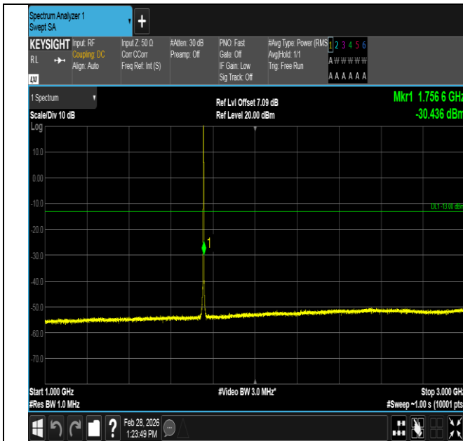
Band4-1.4MHz-16QAM-20393-6RB#0-1000~3000-PASS
