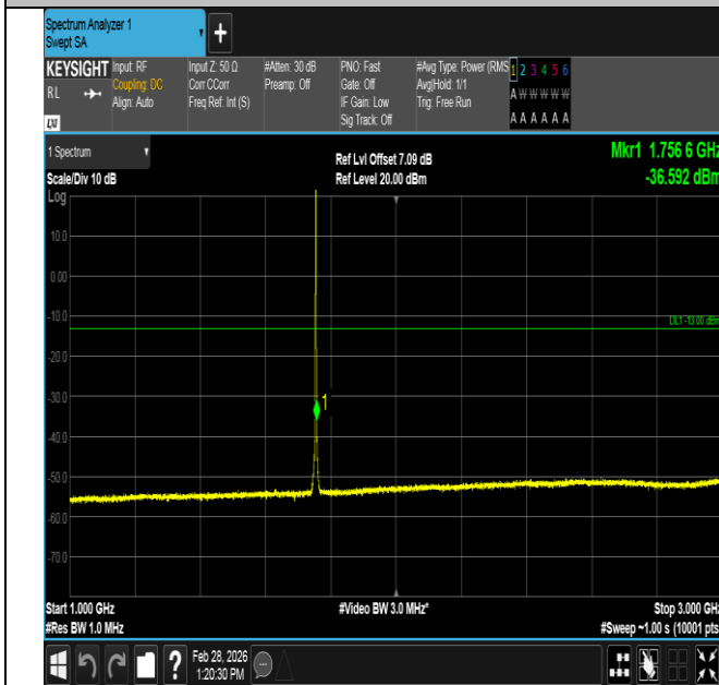
Band4-1.4MHz-16QAM-20393-1RB#0-1000~3000-PASS
