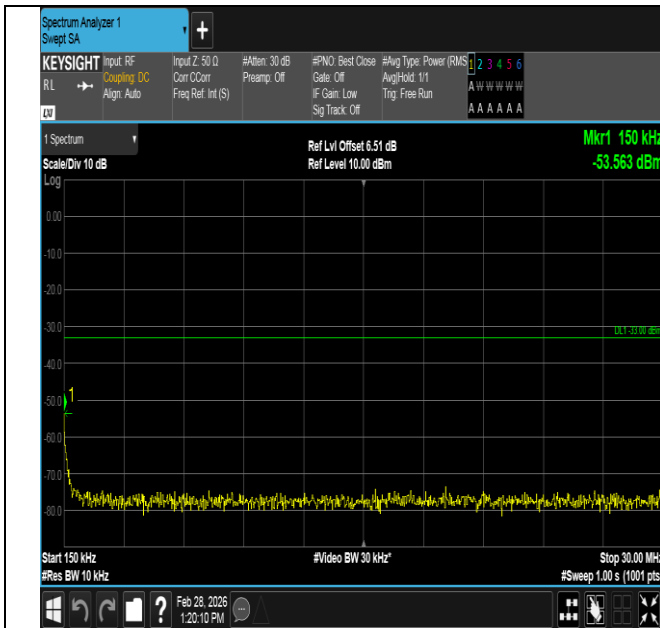
Band4-1.4MHz-16QAM-20393-1RB#0-0.15~30-PASS
