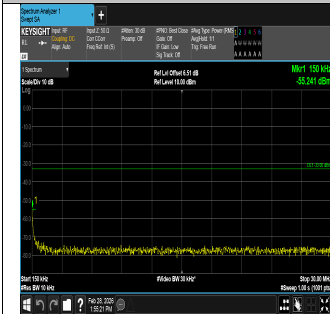
Band4-3MHz-16QAM-19965-1RB#0-0.15~30-PASS
