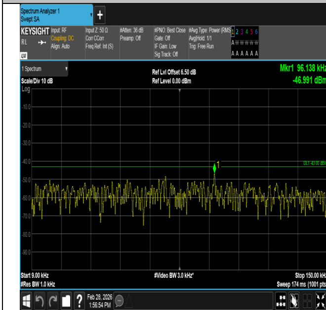
Band4-3MHz-16QAM-19965-1RB#14-0.009~0.15-PASS
