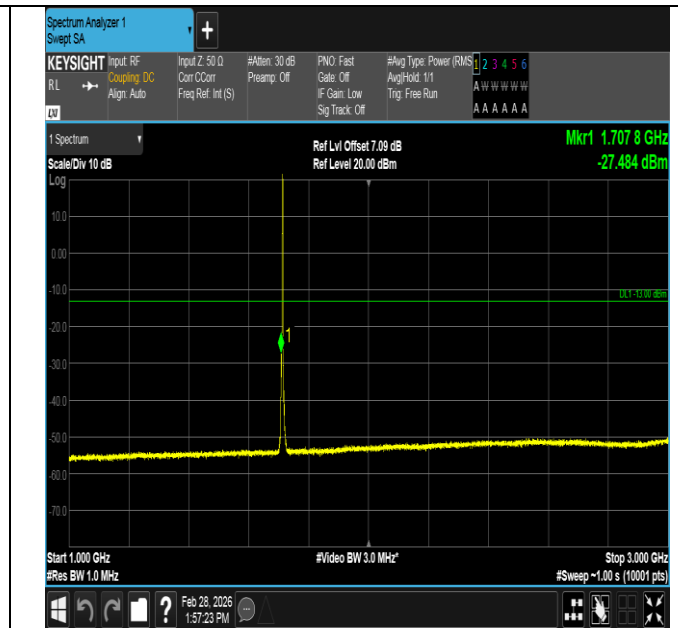
Band4-3MHz-16QAM-19965-1RB#14-1000~3000-PASS
