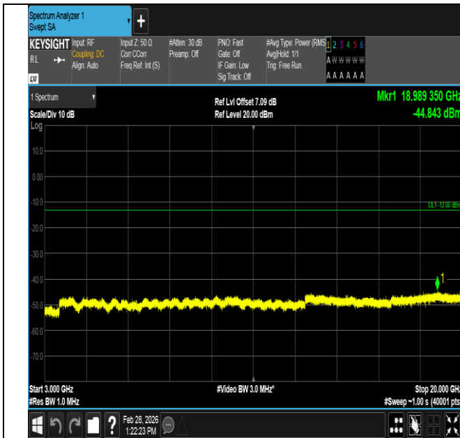
Band4-1.4MHz-16QAM-20393-1RB#5-3000~20000-PASS
