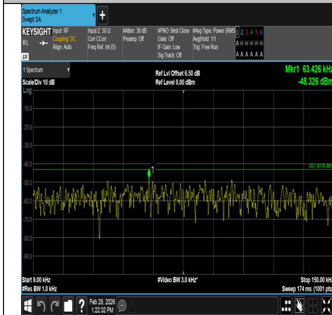
Band4-1.4MHz-QPSK-20393-6RB#0-0.009~0.15-PASS
