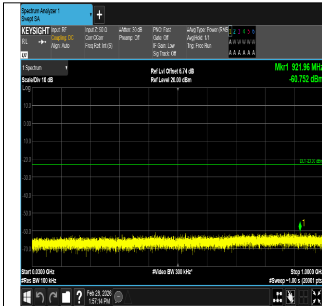
Band4-3MHz-16QAM-19965-1RB#14-30~1000-PASS
