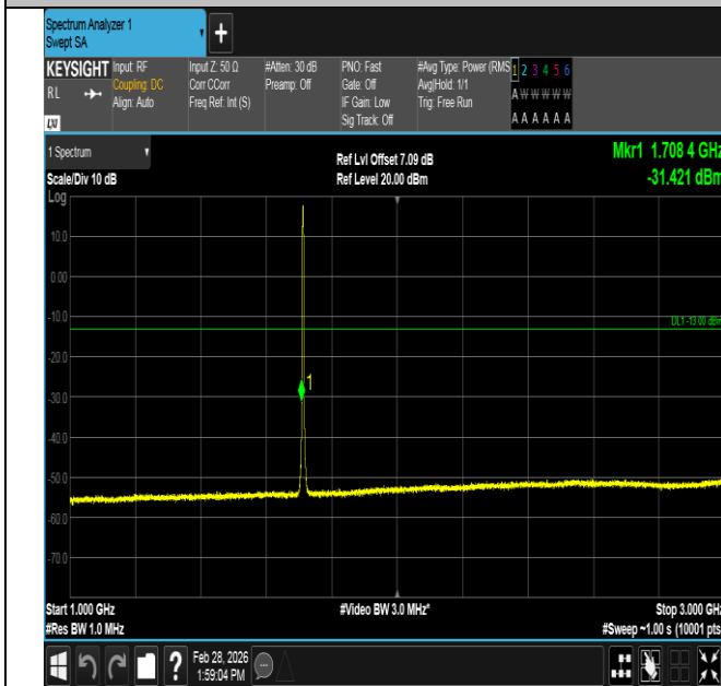
Band4-3MHz-16QAM-19965-15RB#0-1000~3000-PASS
