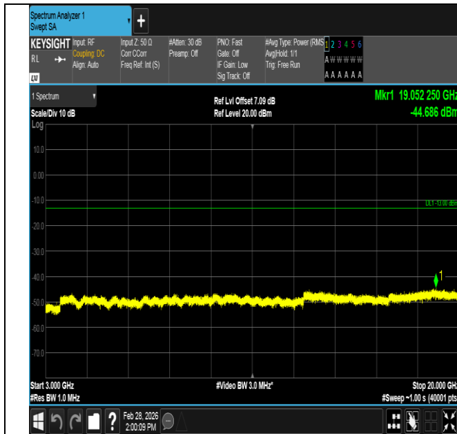
Band4-3MHz-QPSK-20175-1RB#0-3000~20000-PASS
