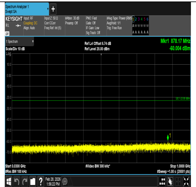
Band4-3MHz-QPSK-19965-1RB#14-30~1000-PASS
