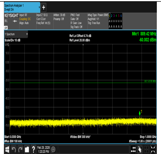
Band4-1.4MHz-16QAM-20393-1RB#0-30~1000-PASS
