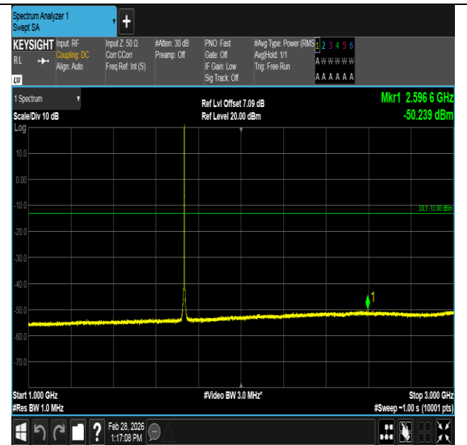
Band4-1.4MHz-16QAM-20175-1RB#5-1000~3000-PASS
