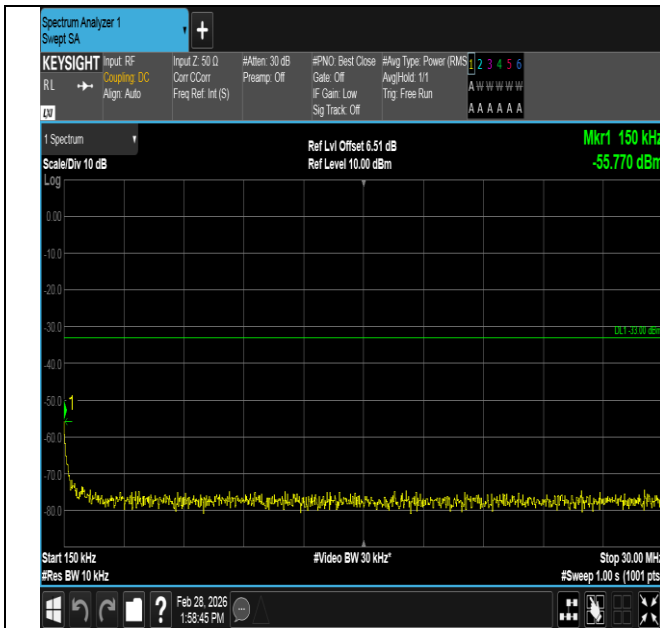
Band4-3MHz-16QAM-19965-15RB#0-0.15~30-PASS
