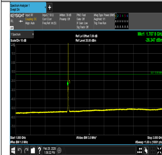
Band4-3MHz-QPSK-19965-1RB#14-1000~3000-PASS
