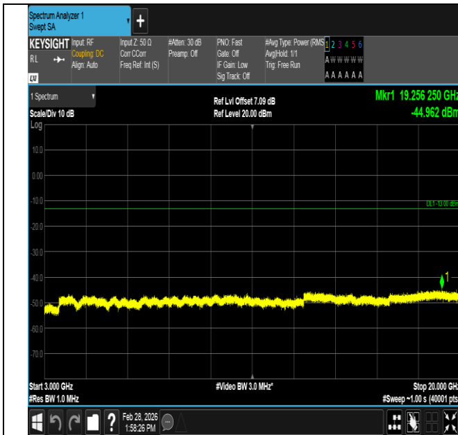
Band4-3MHz-QPSK-19965-15RB#0-3000~20000-PASS
