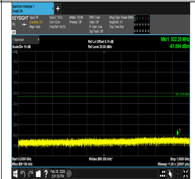
Band4-3MHz-QPSK-20175-1RB#14-30~1000-PASS
