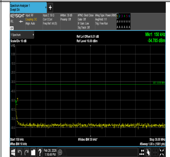
Band4-1.4MHz-16QAM-20175-1RB#5-0.15~30-PASS
