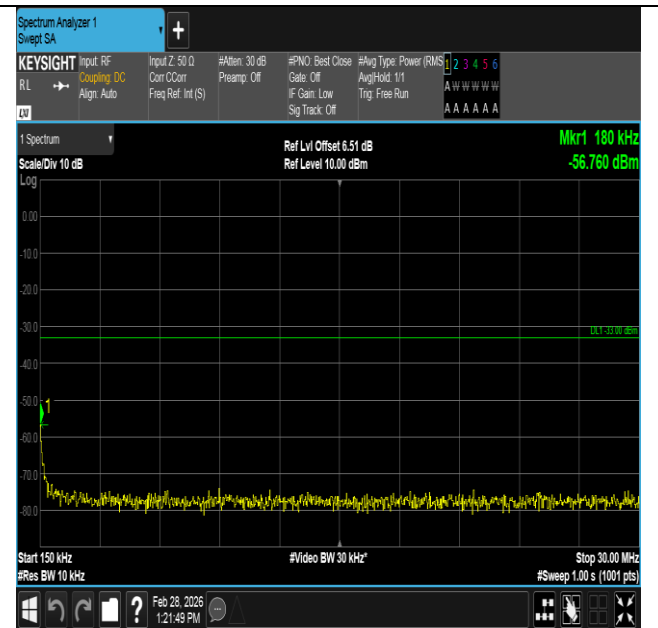
Band4-1.4MHz-16QAM-20393-1RB#5-0.15~30-PASS
