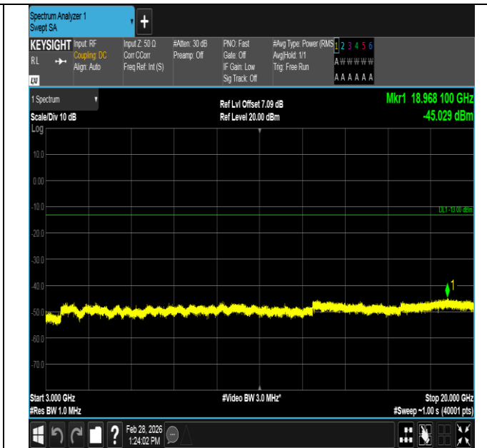
Band4-1.4MHz-16QAM-20393-6RB#0-3000~20000-PASS
