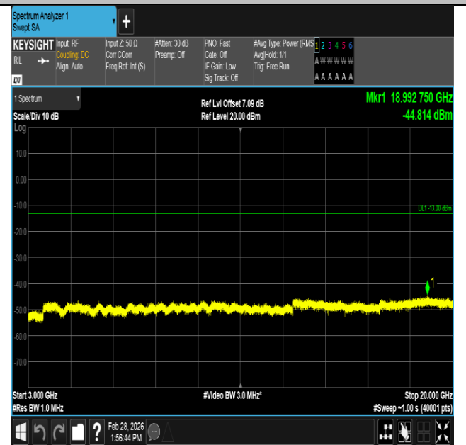
Band4-3MHz-QPSK-19965-1RB#14-3000~20000-PASS
