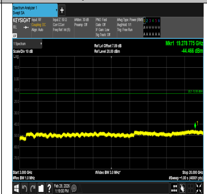
Band4-1.4MHz-16QAM-20175-6RB#0-3000~20000-PASS
