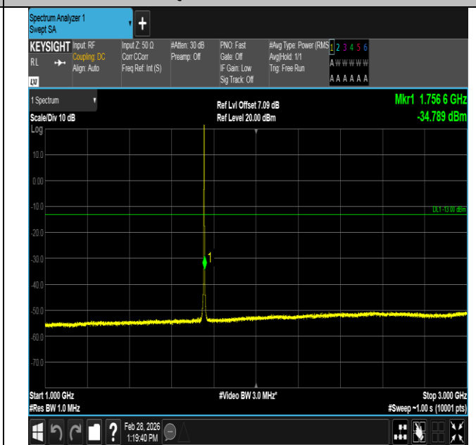
Band4-1.4MHz-QPSK-20393-1RB#0-1000~3000-PASS
