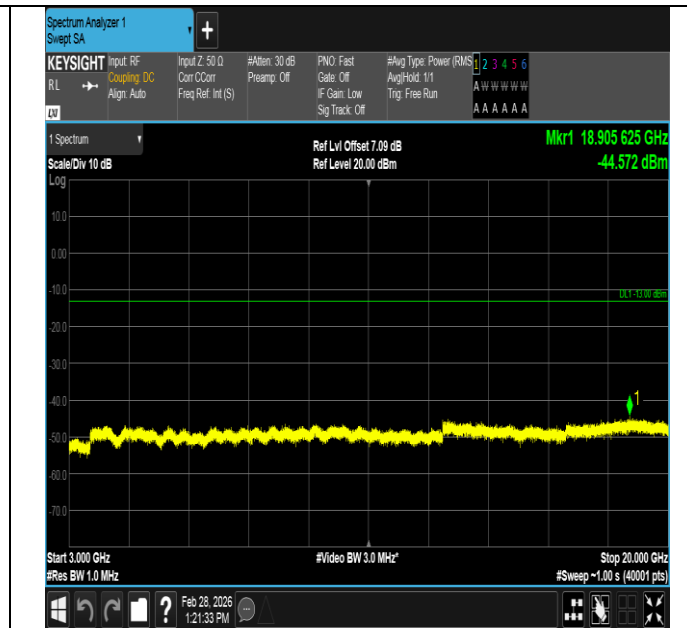
Band4-1.4MHz-QPSK-20393-1RB#5-3000~20000-PASS
