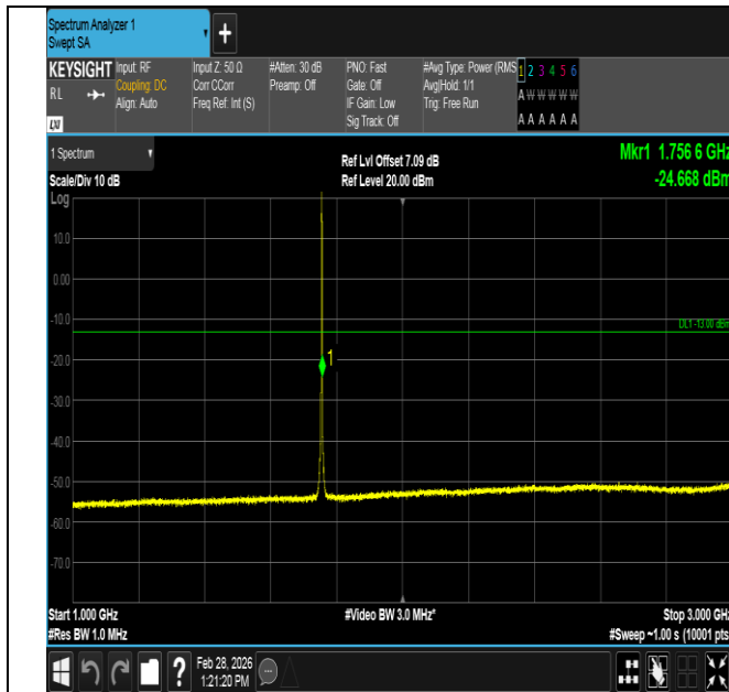
Band4-1.4MHz-QPSK-20393-1RB#5-1000~3000-PASS
