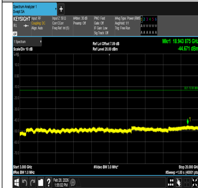
Band4-3MHz-QPSK-19965-1RB#0-3000~20000-PASS
