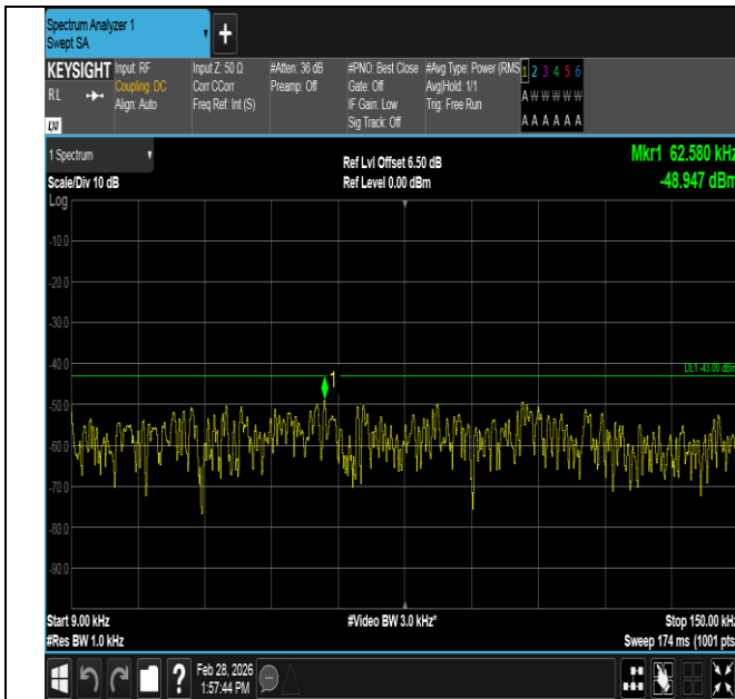
Band4-3MHz-QPSK-19965-15RB#0-0.009~0.15-PASS
