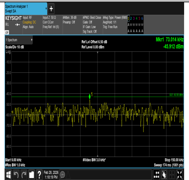
Band4-1.4MHz-16QAM-20175-6RB#0-0.009~0.15-PASS
