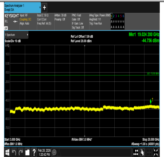
Band4-1.4MHz-16QAM-20393-1RB#0-3000~20000-PASS
