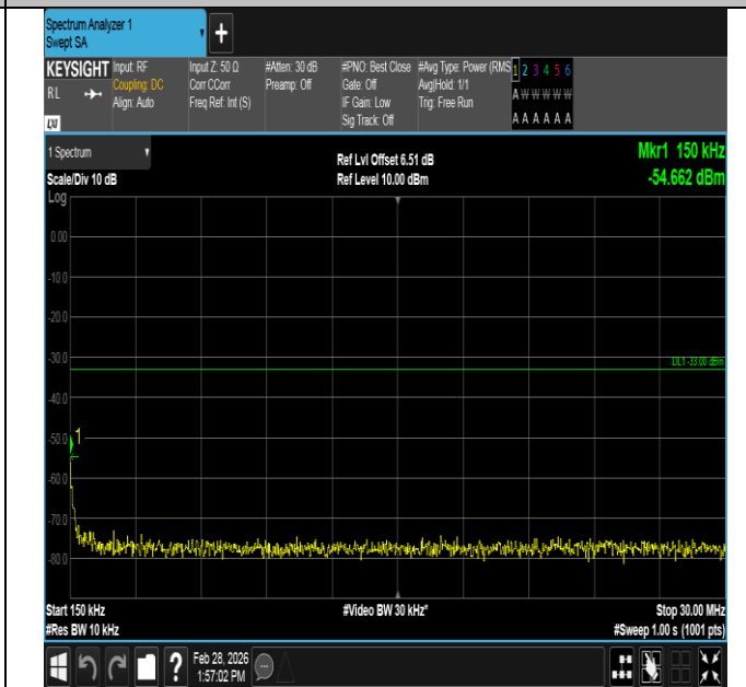
Band4-3MHz-16QAM-19965-1RB#14-0.15~30-PASS
