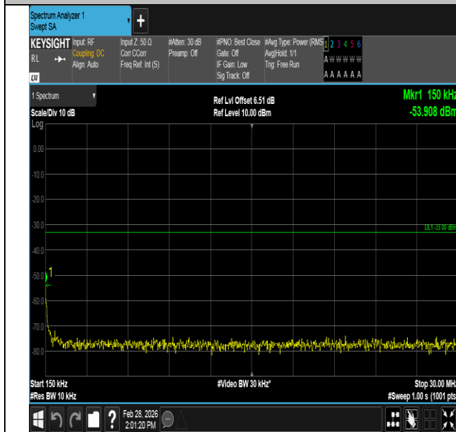
Band4-3MHz-QPSK-20175-1RB#14-0.15~30-PASS
