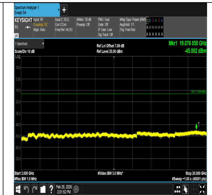
Band4-3MHz-QPSK-20175-1RB#14-3000~20000-PASS
