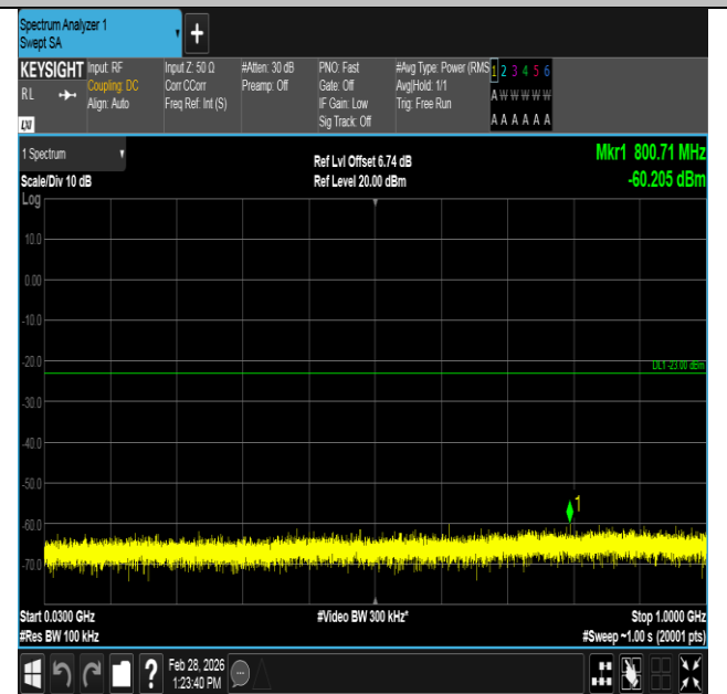
Band4-1.4MHz-16QAM-20393-6RB#0-30~1000-PASS
