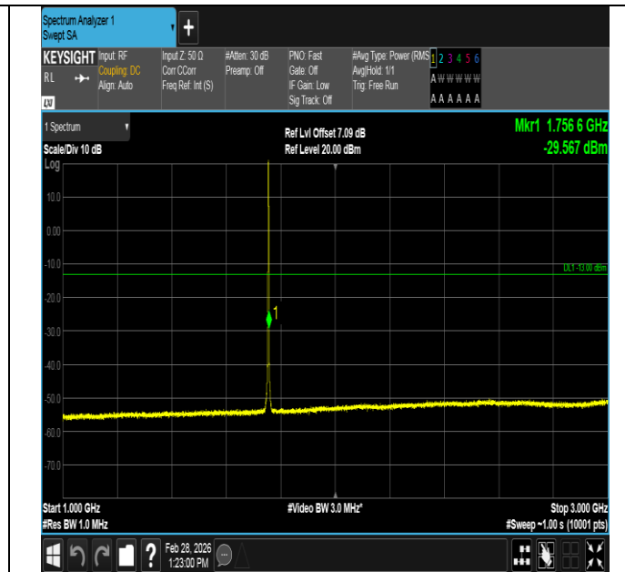
Band4-1.4MHz-QPSK-20393-6RB#0-1000~3000-PASS
