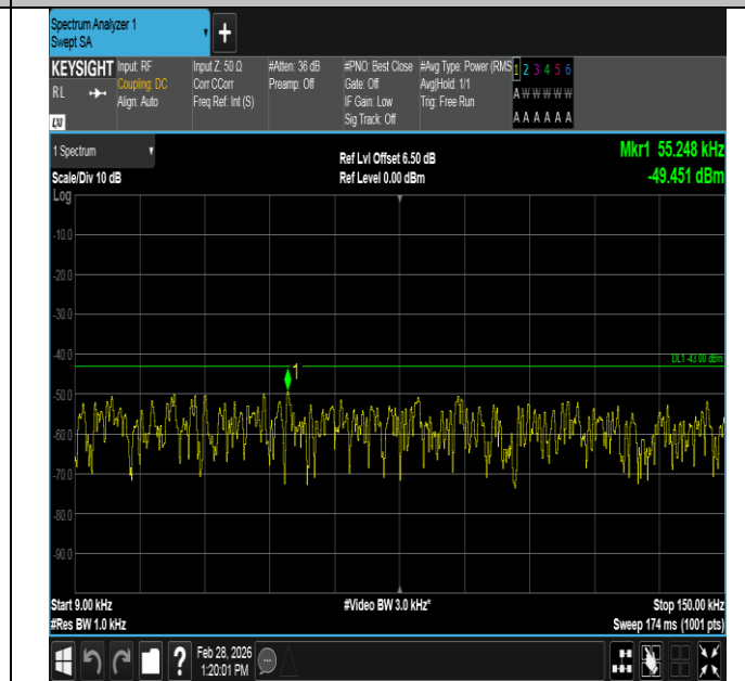
Band4-1.4MHz-16QAM-20393-1RB#0-0.009~0.15-PASS
