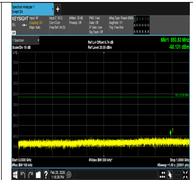
Band4-1.4MHz-16QAM-20175-6RB#0-30~1000-PASS
