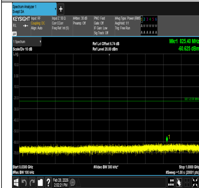
Band4-3MHz-16QAM-20175-1RB#14-30~1000-PASS
