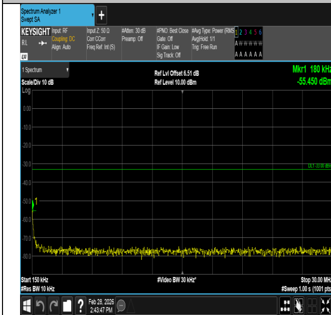
Band4-5MHz-16QAM-19975-25RB#0-0.15~30-PASS
