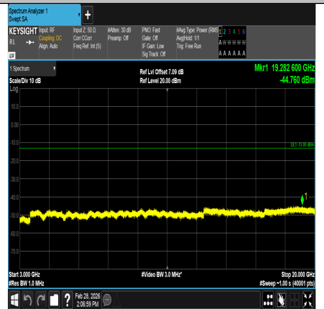
Band4-3MHz-QPSK-20385-1RB#14-3000~20000-PASS
