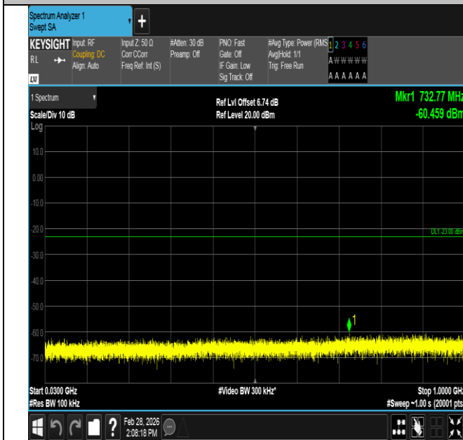
Band4-3MHz-QPSK-20385-15RB#0-30~1000-PASS
