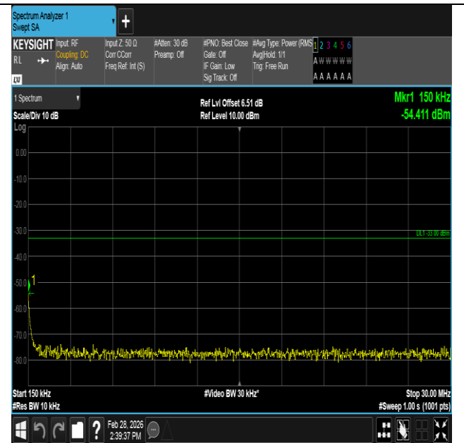
Band4-5MHz-QPSK-19975-1RB#0-0.15~30-PASS
