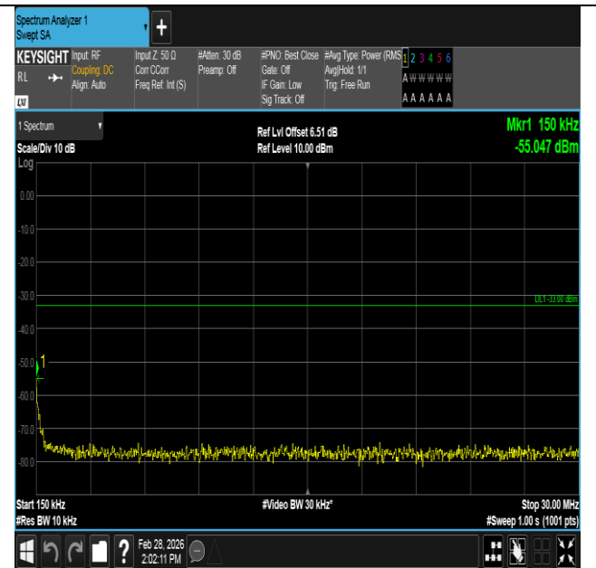
Band4-3MHz-16QAM-20175-1RB#14-0.15~30-PASS
