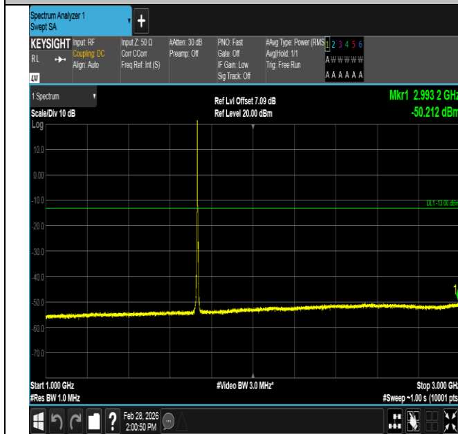
Band4-3MHz-16QAM-20175-1RB#0-1000~3000-PASS
