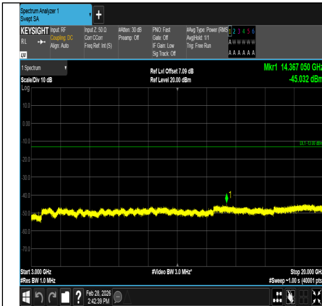
Band4-5MHz-16QAM-19975-1RB#24-3000~20000-PASS
