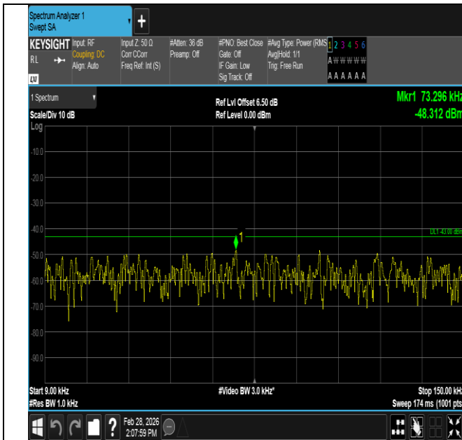
Band4-3MHz-QPSK-20385-15RB#0-0.009~0.15-PASS
