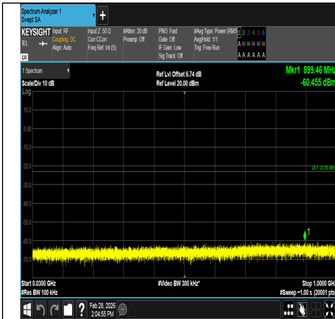
Band4-3MHz-QPSK-20385-1RB#0-30~1000-PASS
