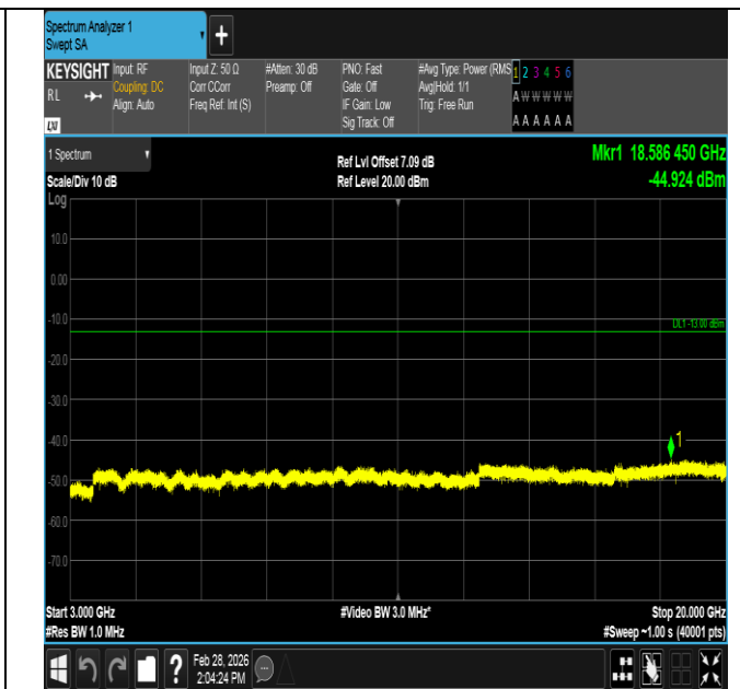
Band4-3MHz-16QAM-20175-15RB#0-3000~20000-PASS
