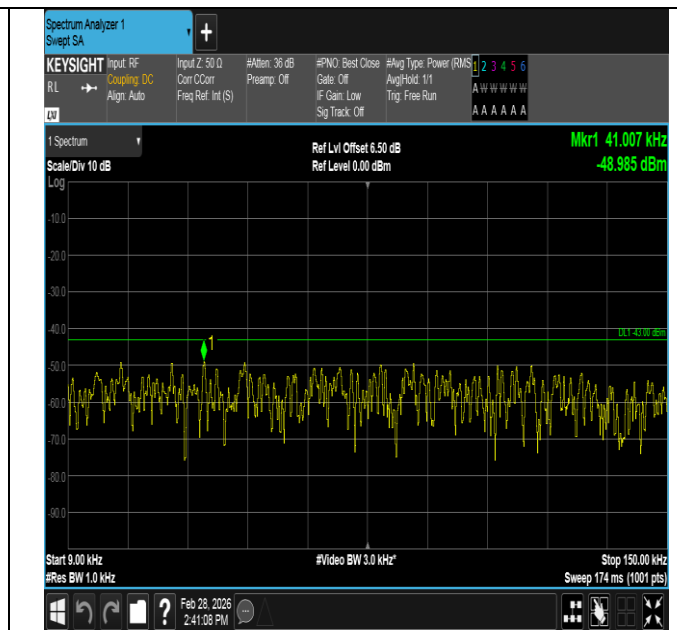
Band4-5MHz-QPSK-19975-1RB#24-0.009~0.15-PASS
