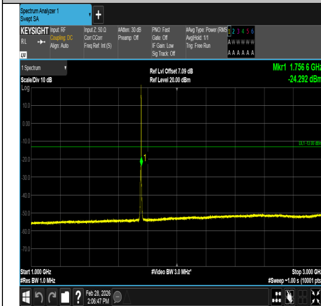
Band4-3MHz-QPSK-20385-1RB#14-1000~3000-PASS
