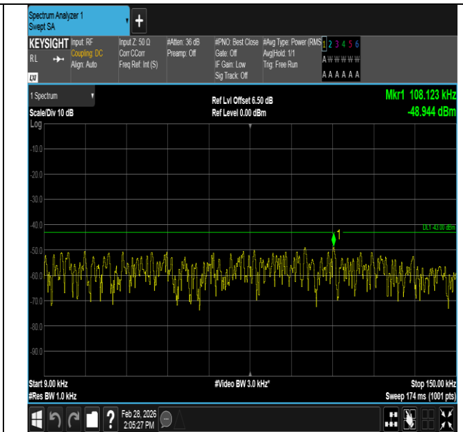
Band4-3MHz-16QAM-20385-1RB#0-0.009~0.15-PASS
