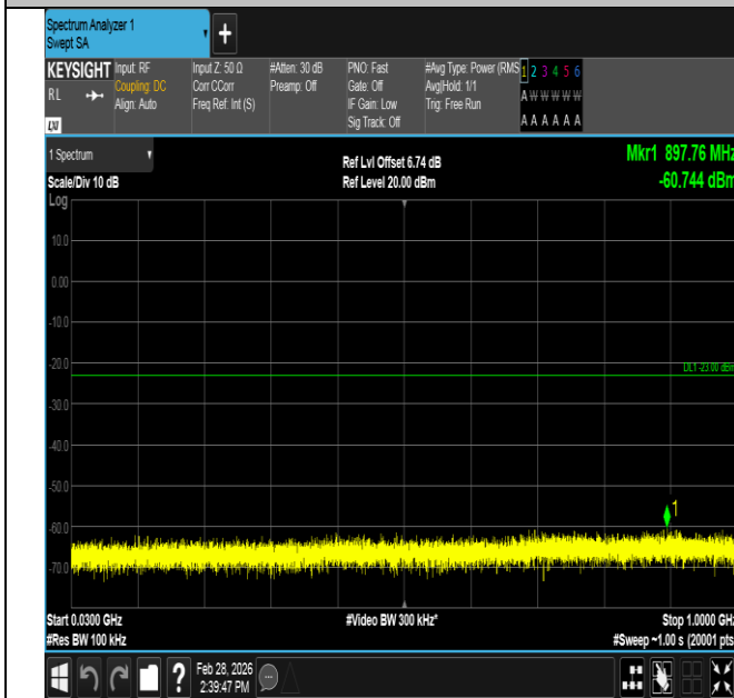
Band4-5MHz-QPSK-19975-1RB#0-30~1000-PASS
