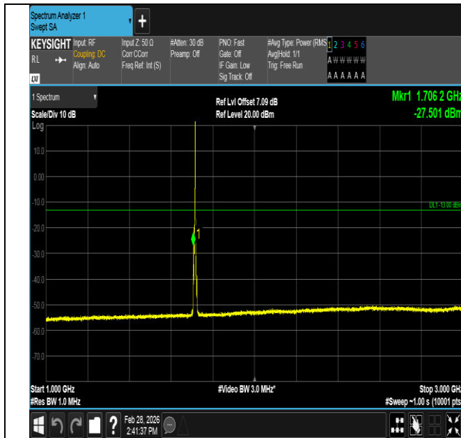
Band4-5MHz-QPSK-19975-1RB#24-1000~3000-PASS
