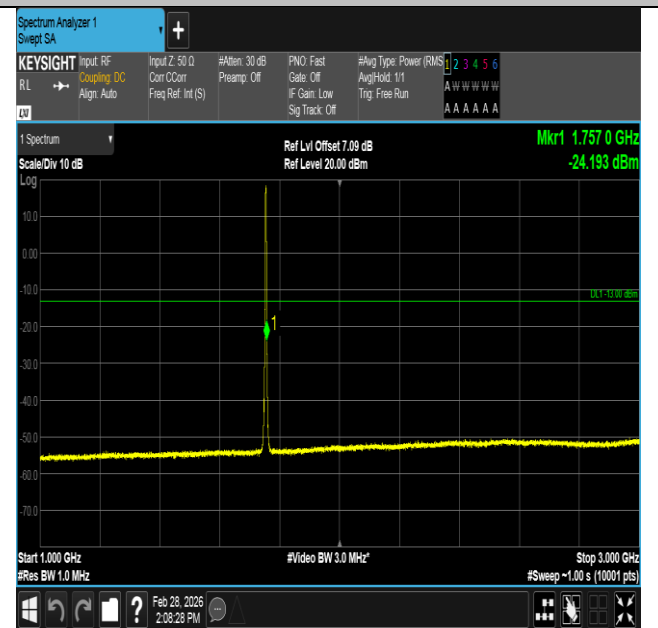
Band4-3MHz-QPSK-20385-15RB#0-1000~3000-PASS
