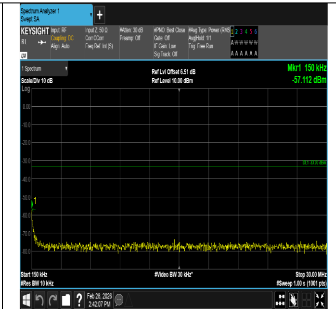
Band4-5MHz-16QAM-19975-1RB#24-0.15~30-PASS
