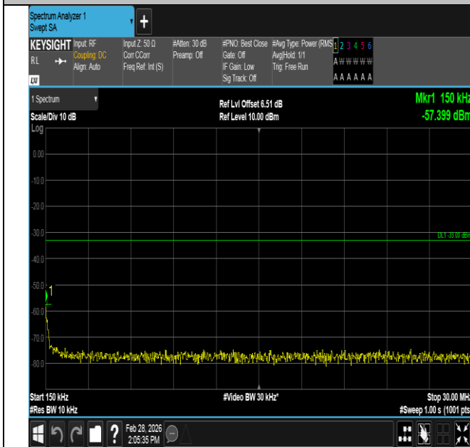
Band4-3MHz-16QAM-20385-1RB#0-0.15~30-PASS
