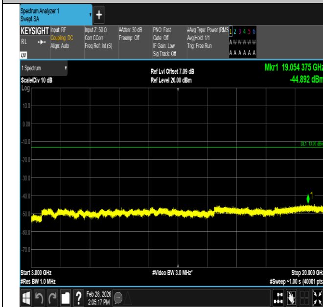
Band4-3MHz-QPSK-20385-1RB#0-3000~20000-PASS
