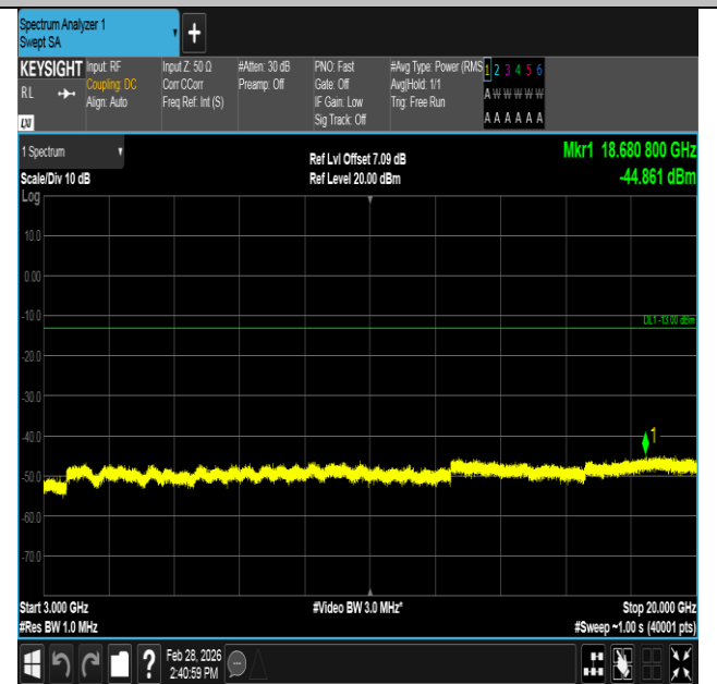
Band4-5MHz-16QAM-19975-1RB#0-3000~20000-PASS
