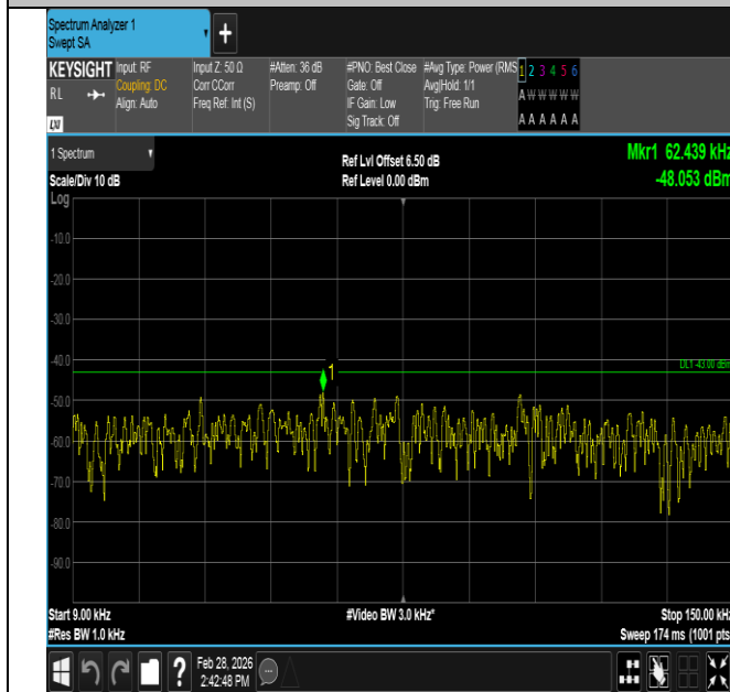
Band4-5MHz-QPSK-19975-25RB#0-0.009~0.15-PASS
