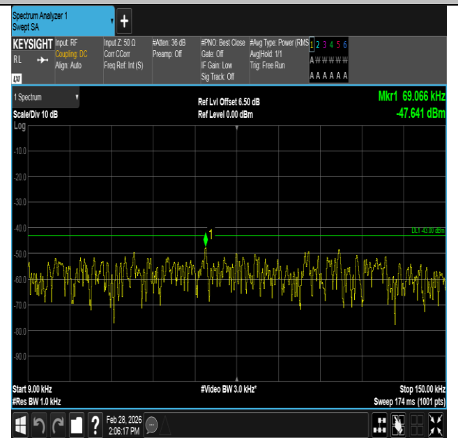
Band4-3MHz-QPSK-20385-1RB#14-0.009~0.15-PASS
