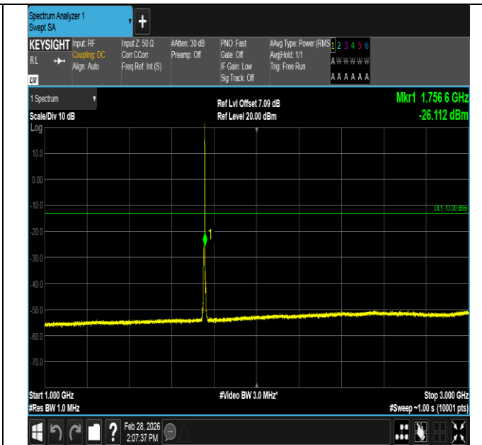
Band4-3MHz-16QAM-20385-1RB#14-1000~3000-PASS
