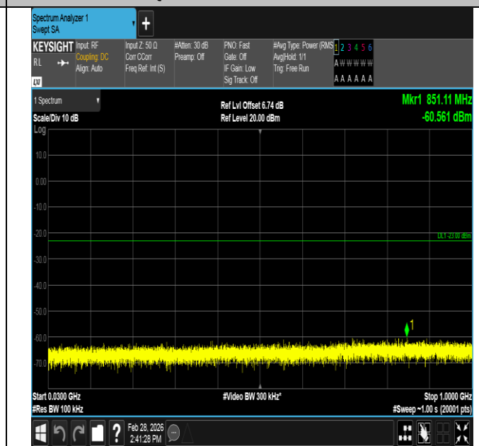
Band4-5MHz-QPSK-19975-1RB#24-30~1000-PASS
