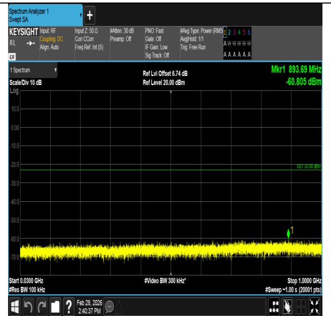
Band4-5MHz-16QAM-19975-1RB#0-30~1000-PASS
