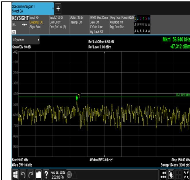
Band4-3MHz-16QAM-20175-1RB#14-0.009~0.15-PASS
