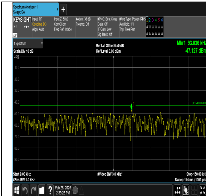
Band4-5MHz-QPSK-19975-1RB#0-0.009~0.15-PASS
