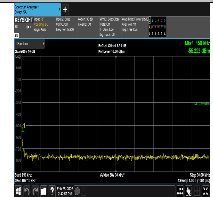
Band4-5MHz-QPSK-19975-25RB#0-0.15~30-PASS
