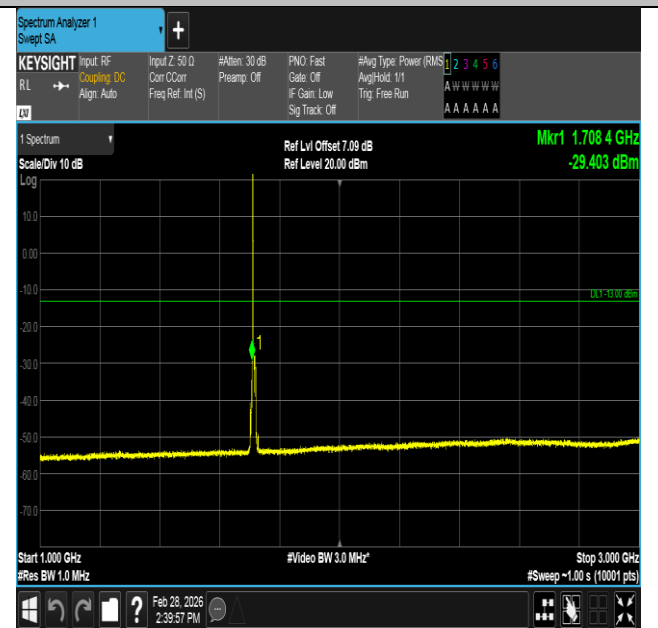
Band4-5MHz-QPSK-19975-1RB#0-1000~3000-PASS
