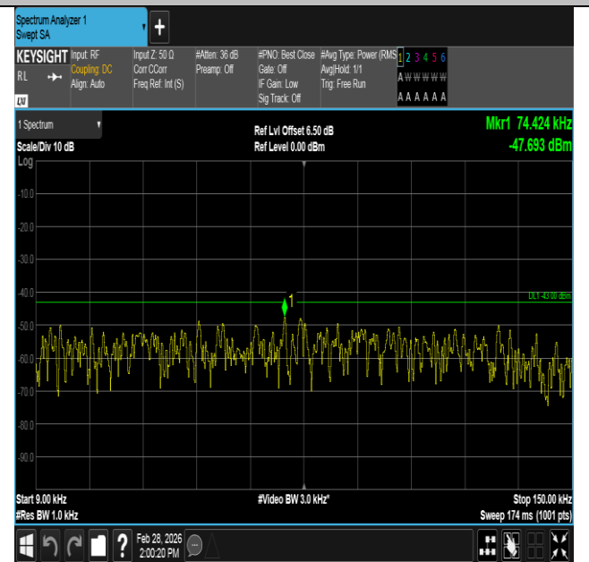
Band4-3MHz-16QAM-20175-1RB#0-0.009~0.15-PASS
