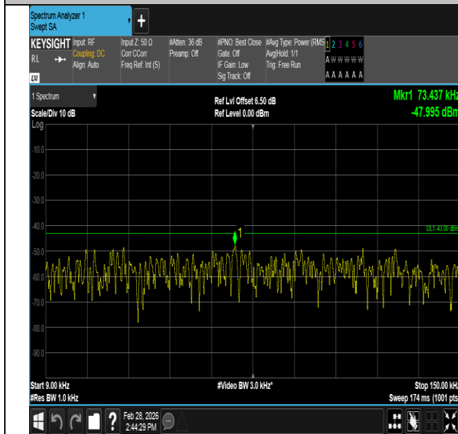
Band4-5MHz-QPSK-20175-1RB#0-0.009~0.15-PASS
