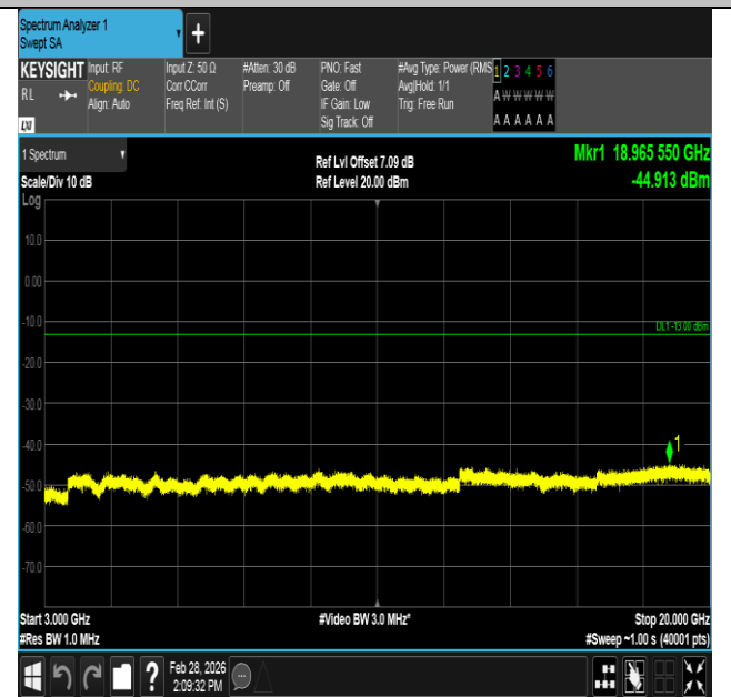
Band4-3MHz-16QAM-20385-15RB#0-3000~20000-PASS
