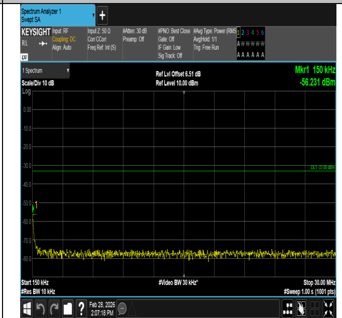
Band4-3MHz-16QAM-20385-1RB#14-0.15~30-PASS
