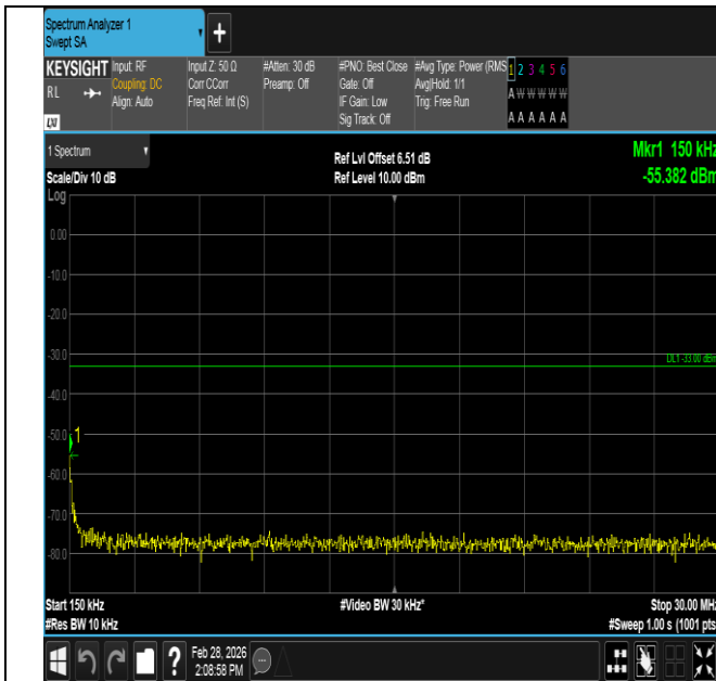
Band4-3MHz-16QAM-20385-15RB#0-0.15~30-PASS
