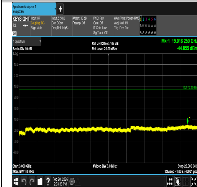
Band4-3MHz-QPSK-20175-15RB#0-3000~20000-PASS
