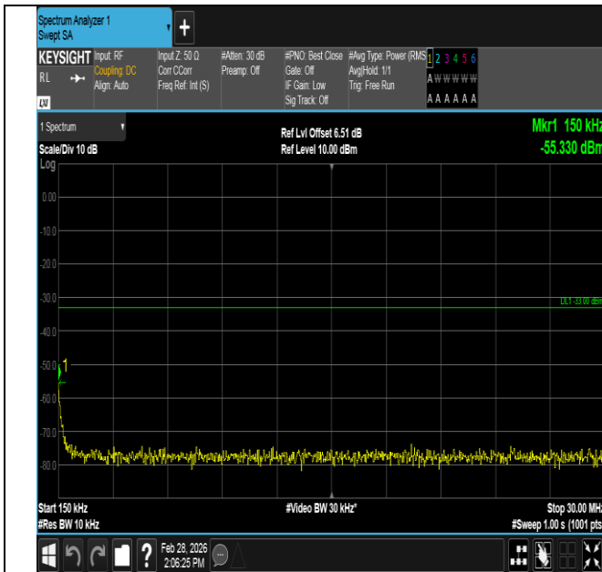
Band4-3MHz-QPSK-20385-1RB#14-0.15~30-PASS
