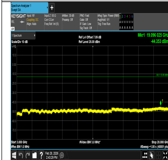
Band4-5MHz-QPSK-19975-25RB#0-3000~20000-PASS
