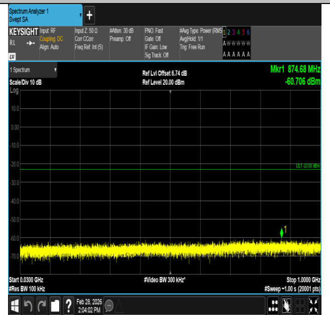
Band4-3MHz-16QAM-20175-15RB#0-30~1000-PASS
