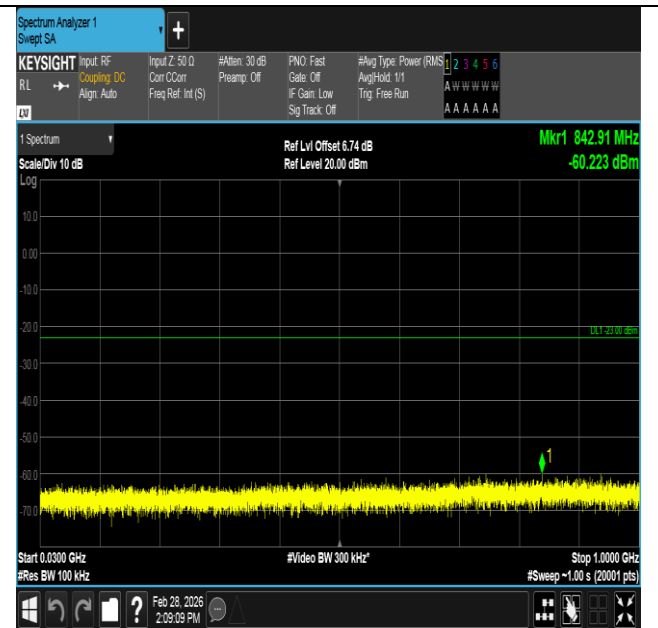
Band4-3MHz-16QAM-20385-15RB#0-30~1000-PASS
