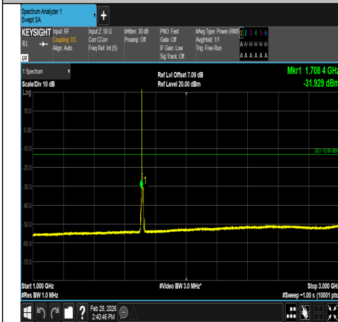
Band4-5MHz-16QAM-19975-1RB#0-1000~3000-PASS
