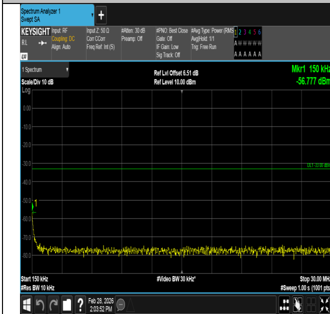
Band4-3MHz-16QAM-20175-15RB#0-0.15~30-PASS
