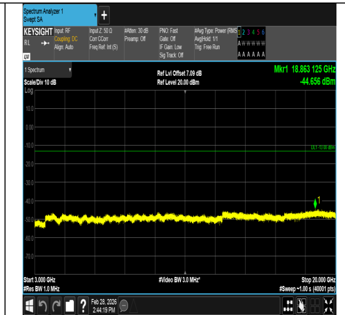
Band4-5MHz-16QAM-19975-25RB#0-3000~20000-PASS
