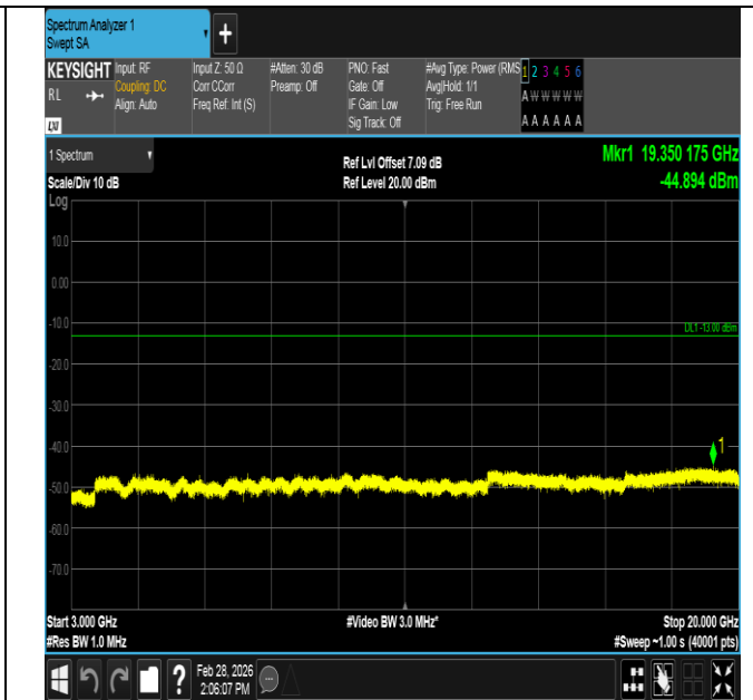
Band4-3MHz-16QAM-20385-1RB#0-3000~20000-PASS
