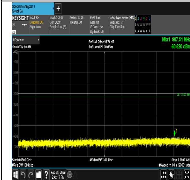
Band4-5MHz-16QAM-19975-1RB#24-30~1000-PASS
