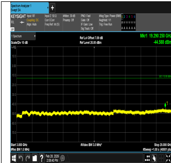
Band4-3MHz-QPSK-20385-15RB#0-3000~20000-PASS
