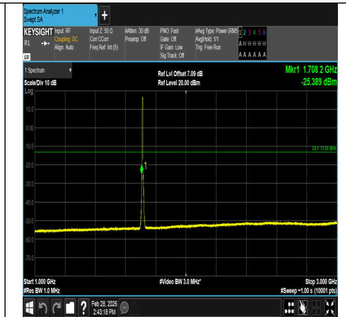
Band4-5MHz-QPSK-19975-25RB#0-1000~3000-PASS
