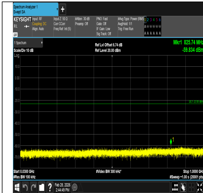
Band4-5MHz-QPSK-20175-1RB#0-30~1000-PASS
