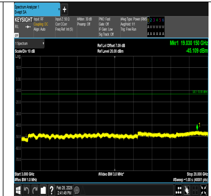
Band4-5MHz-QPSK-19975-1RB#24-3000~20000-PASS
