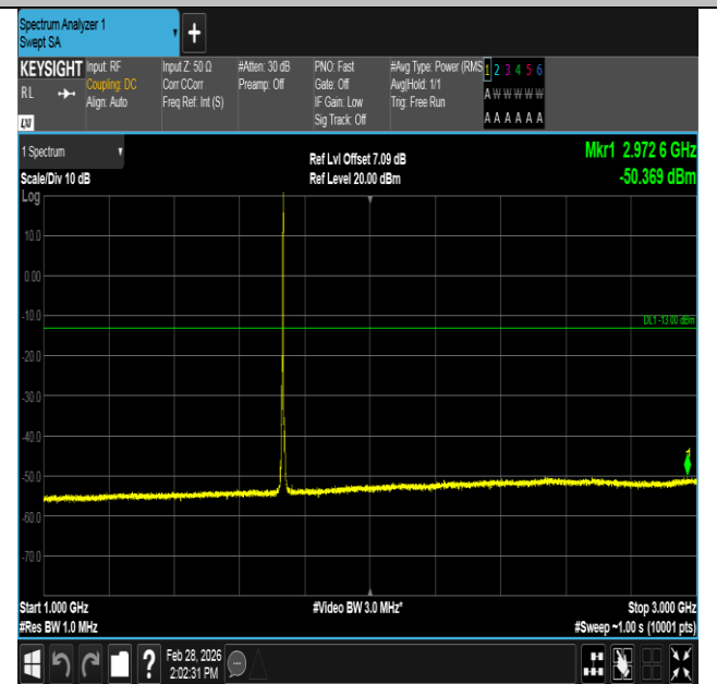
Band4-3MHz-16QAM-20175-1RB#14-1000~3000-PASS
