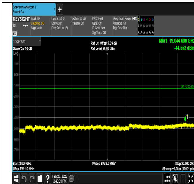
Band4-5MHz-QPSK-19975-1RB#0-3000~20000-PASS
