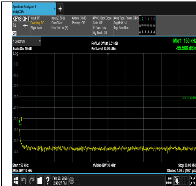
Band4-5MHz-16QAM-19975-1RB#0-0.15~30-PASS
