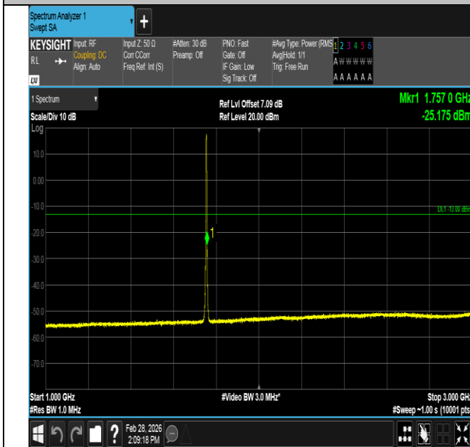
Band4-3MHz-16QAM-20385-15RB#0-1000~3000-PASS
