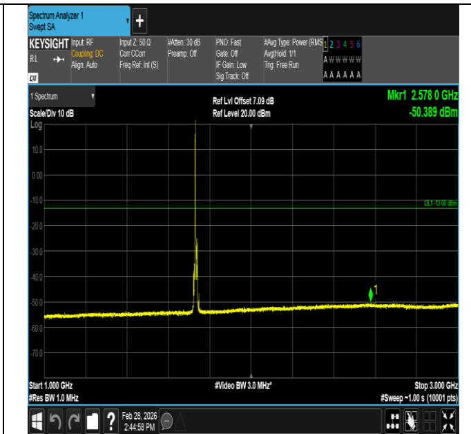
Band4-5MHz-QPSK-20175-1RB#0-1000~3000-PASS
