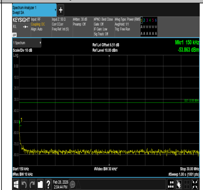
Band4-3MHz-QPSK-20385-1RB#0-0.15~30-PASS
