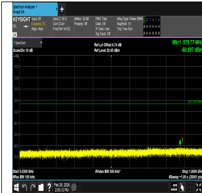
Band4-3MHz-QPSK-20175-15RB#0-30~1000-PASS
