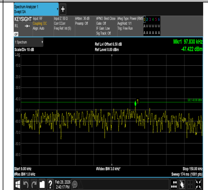
Band4-5MHz-16QAM-19975-1RB#0-0.009~0.15-PASS
