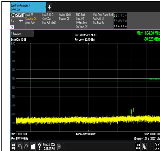
Band4-5MHz-QPSK-19975-25RB#0-30~1000-PASS
