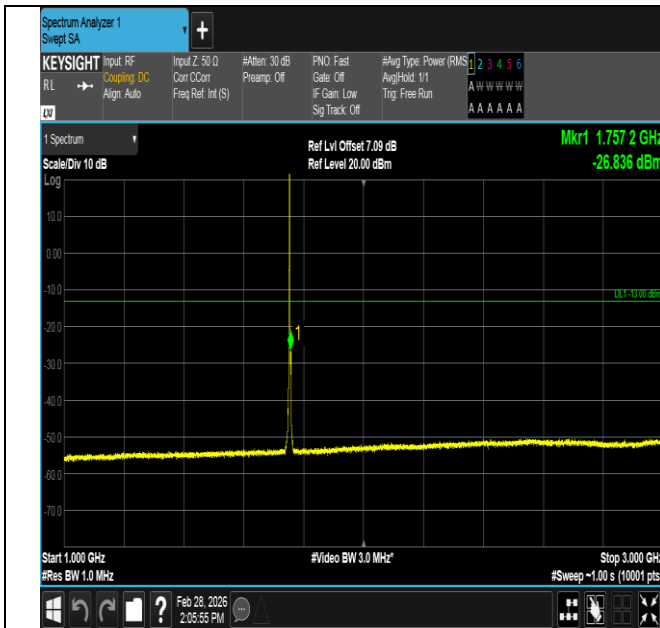
Band4-3MHz-16QAM-20385-1RB#0-1000~3000-PASS
