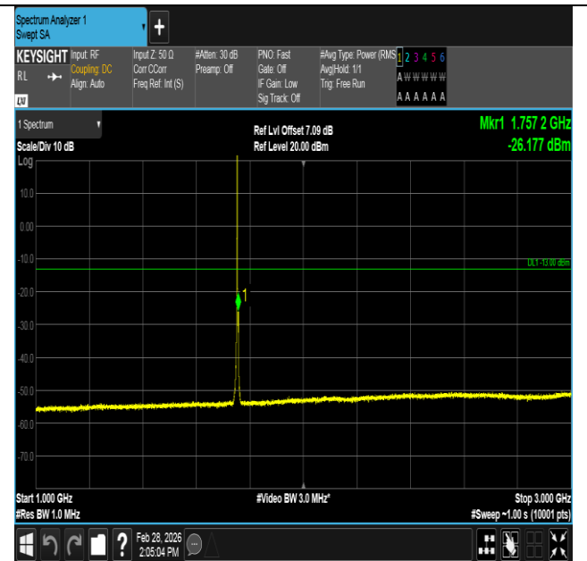
Band4-3MHz-QPSK-20385-1RB#0-1000~3000-PASS
