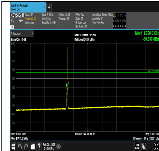
Band4-5MHz-16QAM-19975-25RB#0-1000~3000-PASS
