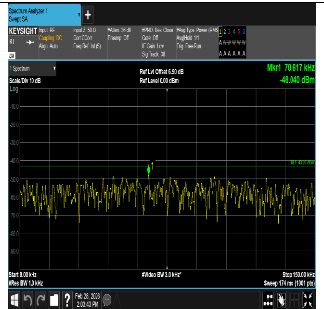
Band4-3MHz-16QAM-20175-15RB#0-0.009~0.15-PASS
