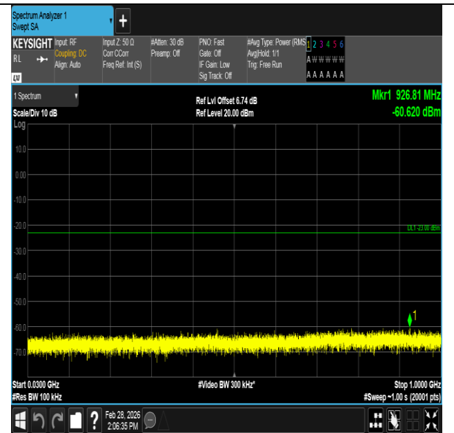
Band4-3MHz-QPSK-20385-1RB#14-30~1000-PASS
