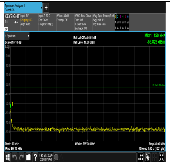
Band4-3MHz-QPSK-20385-15RB#0-0.15~30-PASS
