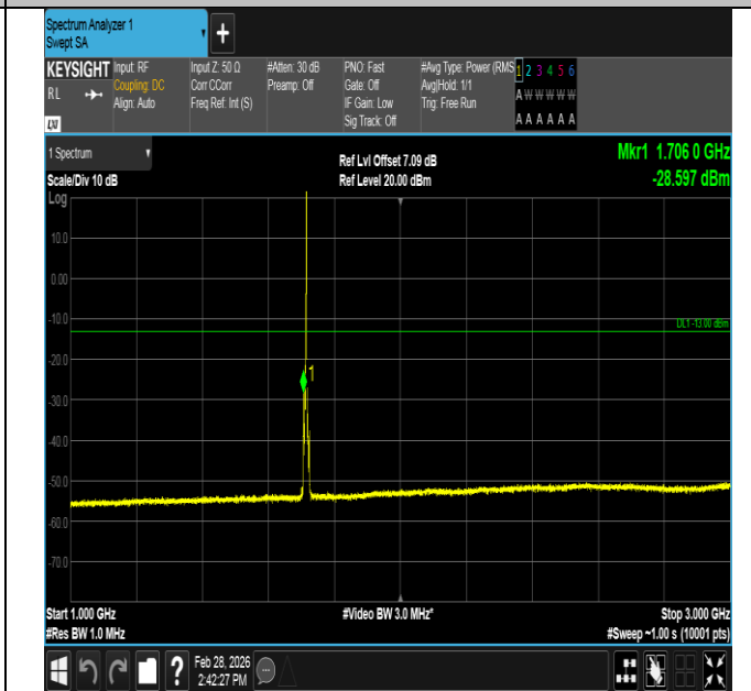
Band4-5MHz-16QAM-19975-1RB#24-1000~3000-PASS
