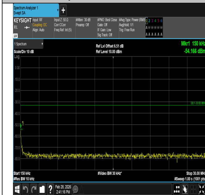
Band4-5MHz-QPSK-19975-1RB#24-0.15~30-PASS
