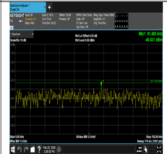
Band4-3MHz-16QAM-20385-15RB#0-0.009~0.15-PASS
