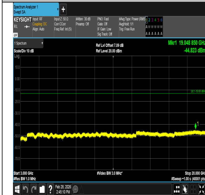
Band4-5MHz-QPSK-20175-1RB#0-3000~20000-PASS
