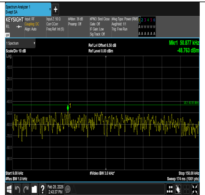
Band4-5MHz-16QAM-19975-25RB#0-0.009~0.15-PASS
