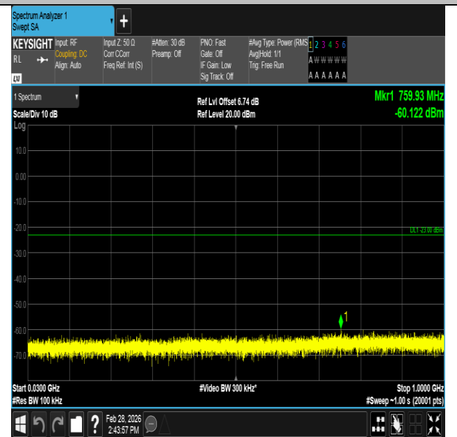
Band4-5MHz-16QAM-19975-25RB#0-30~1000-PASS
