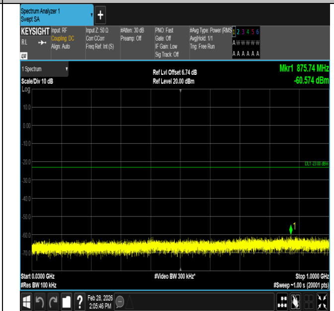
Band4-3MHz-16QAM-20385-1RB#0-30~1000-PASS
