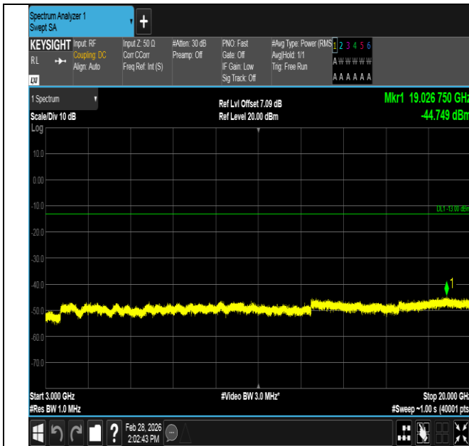
Band4-3MHz-16QAM-20175-1RB#14-3000~20000-PASS
