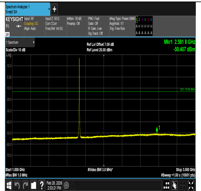
Band4-3MHz-QPSK-20175-15RB#0-1000~3000-PASS
