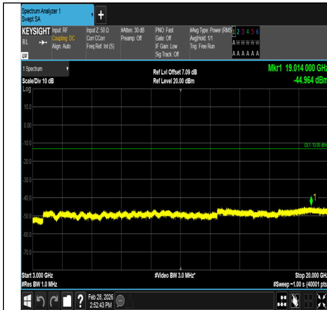
Band4-5MHz-16QAM-20375-1RB#24-3000~20000-PASS
