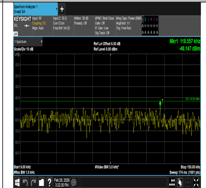
Band4-10MHz-QPSK-20000-1RB#49-0.009~0.15-PASS
