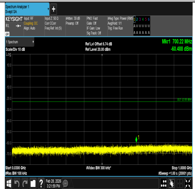
Band4-10MHz-16QAM-20000-1RB#0-30~1000-PASS
