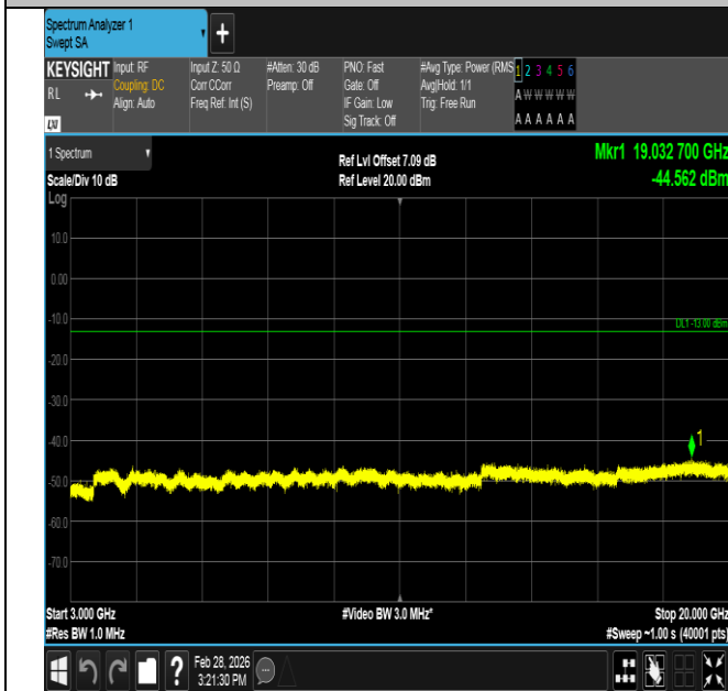
Band4-10MHz-QPSK-20000-1RB#0-3000~20000-PASS
