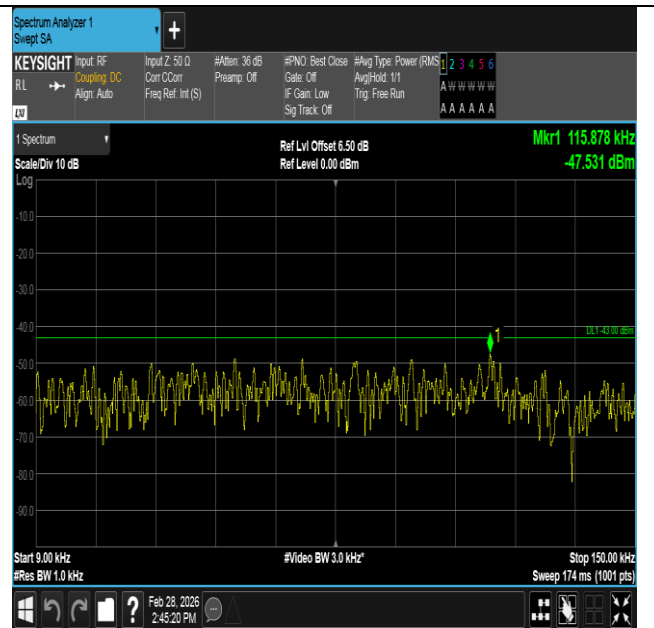
Band4-5MHz-16QAM-20175-1RB#0-0.009~0.15-PASS
