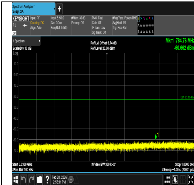
Band4-5MHz-QPSK-20375-25RB#0-30~1000-PASS
