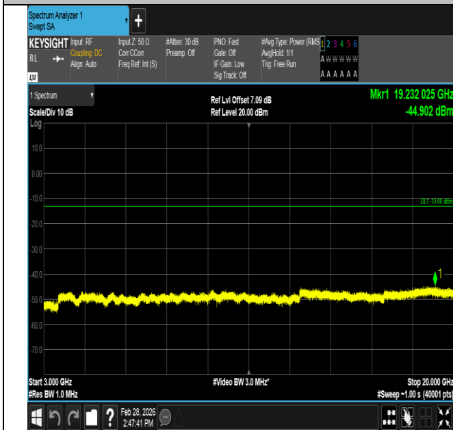
Band4-5MHz-16QAM-20175-1RB#24-3000~20000-PASS
