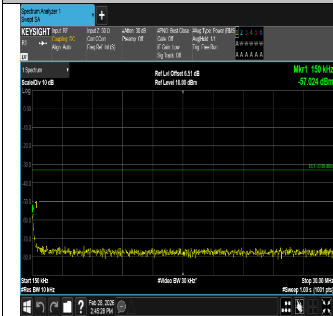
Band4-5MHz-16QAM-20175-1RB#0-0.15~30-PASS
