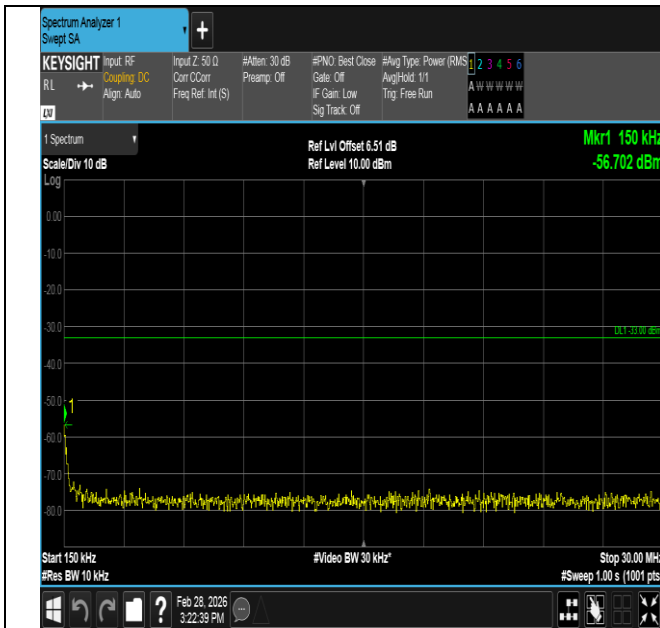
Band4-10MHz-QPSK-20000-1RB#49-0.15~30-PASS
