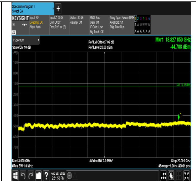
Band4-5MHz-QPSK-20375-1RB#24-3000~20000-PASS
