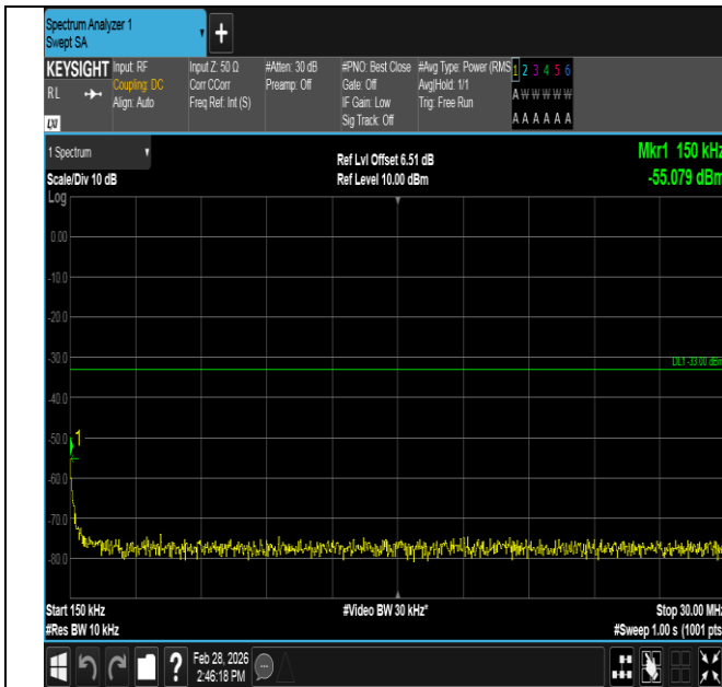
Band4-5MHz-QPSK-20175-1RB#24-0.15~30-PASS
