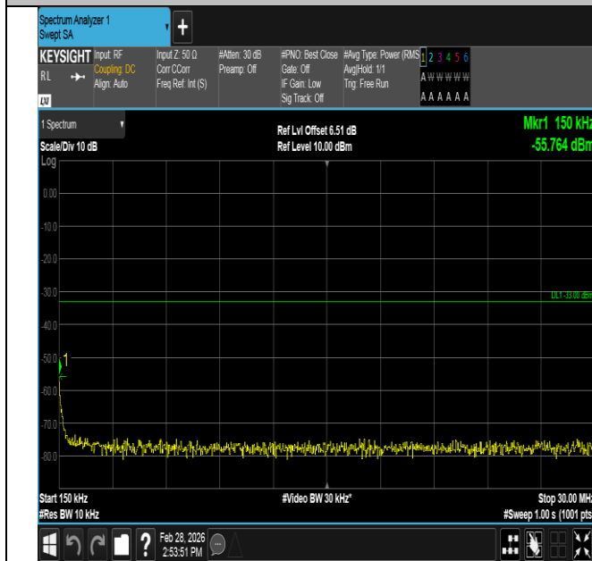
Band4-5MHz-16QAM-20375-25RB#0-0.15~30-PASS
