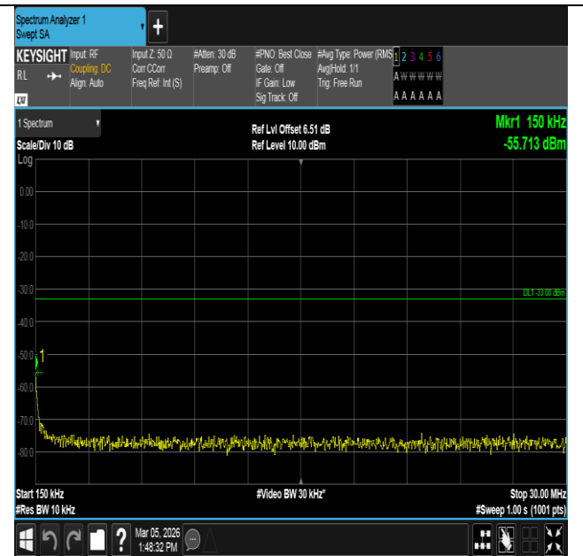
Band4-10MHz-QPSK-20000-50RB#0-0.15~30-PASS
