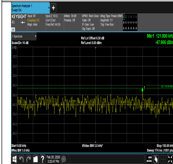
Band4-10MHz-QPSK-20000-1RB#0-0.009~0.15-PASS
