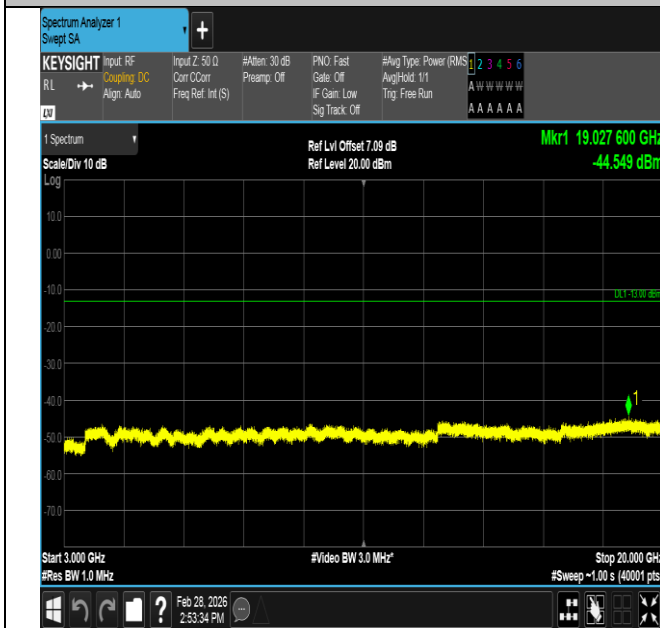
Band4-5MHz-QPSK-20375-25RB#0-3000~20000-PASS
