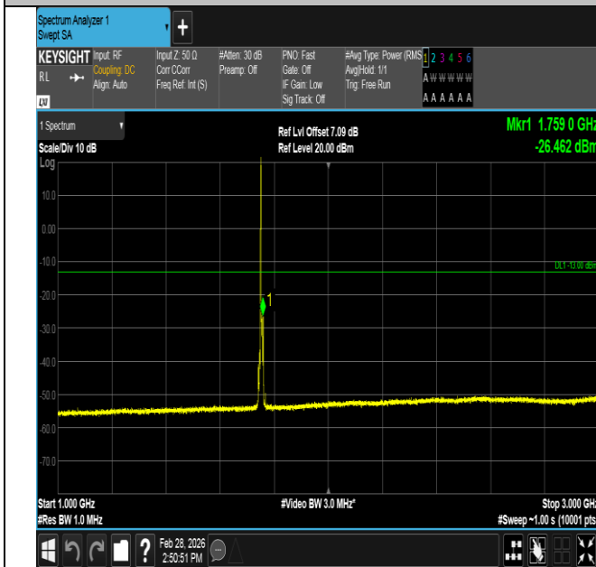
Band4-5MHz-16QAM-20375-1RB#0-1000~3000-PASS
