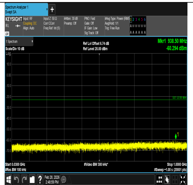
Band4-5MHz-16QAM-20175-25RB#0-30~1000-PASS
