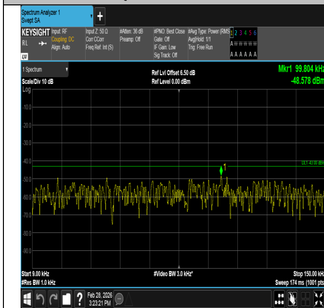
Band4-10MHz-16QAM-20000-1RB#49-0.009~0.15-PASS
