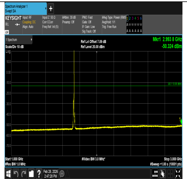
Band4-5MHz-16QAM-20175-1RB#24-1000~3000-PASS
