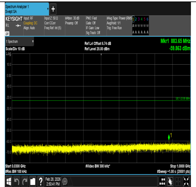
Band4-5MHz-16QAM-20375-1RB#0-30~1000-PASS
