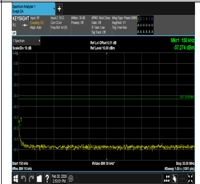
Band4-5MHz-QPSK-20375-25RB#0-0.15~30-PASS
