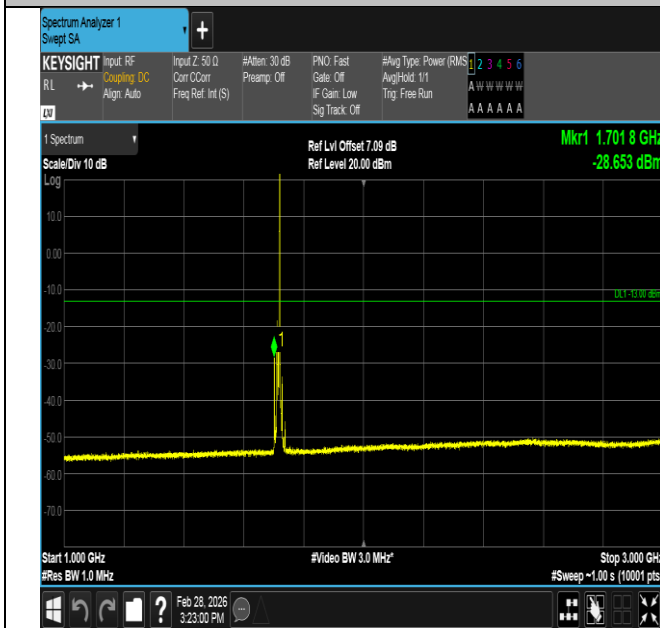
Band4-10MHz-QPSK-20000-1RB#49-1000~3000-PASS
