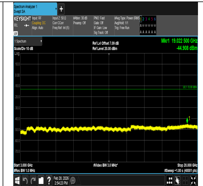
Band4-5MHz-16QAM-20375-25RB#0-3000~20000-PASS
