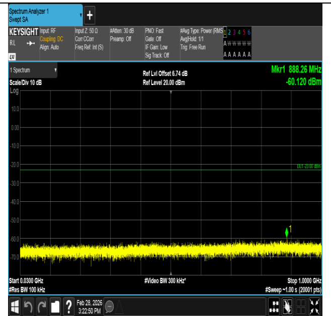
Band4-10MHz-QPSK-20000-1RB#49-30~1000-PASS
