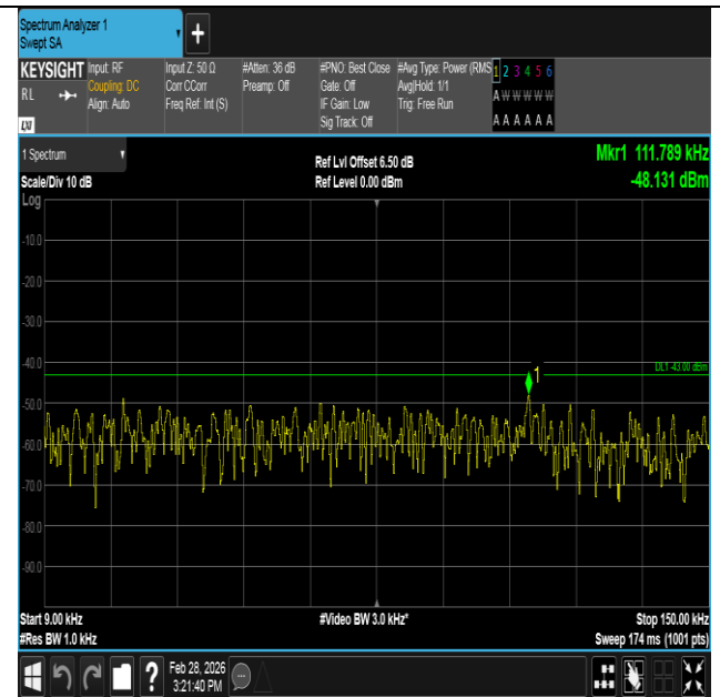
Band4-10MHz-16QAM-20000-1RB#0-0.009~0.15-PASS
