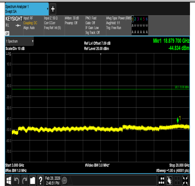
Band4-5MHz-QPSK-20175-1RB#24-3000~20000-PASS
