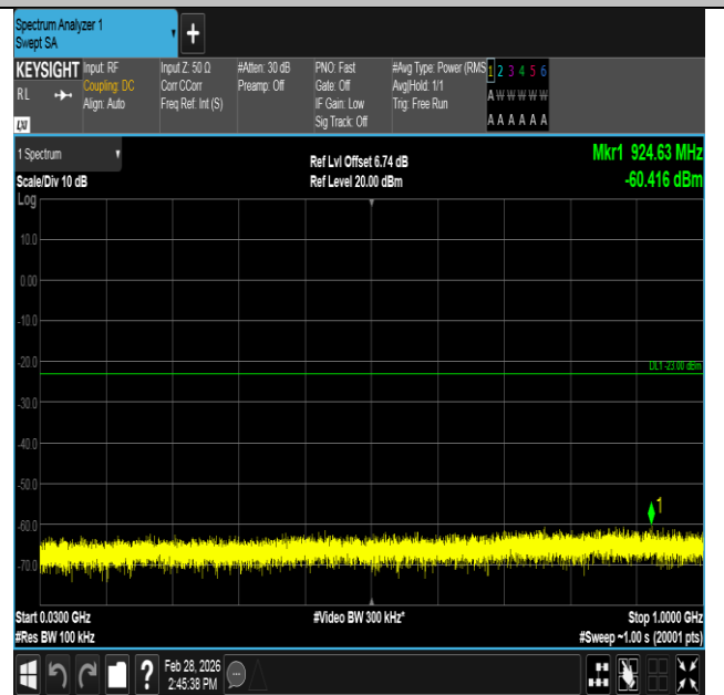
Band4-5MHz-16QAM-20175-1RB#0-30~1000-PASS
