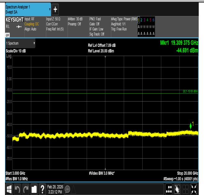
Band4-10MHz-QPSK-20000-1RB#49-3000~20000-PASS
