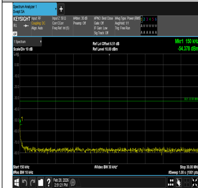
Band4-5MHz-QPSK-20375-1RB#24-0.15~30-PASS
