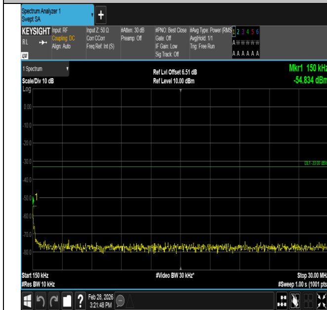
Band4-10MHz-16QAM-20000-1RB#0-0.15~30-PASS
