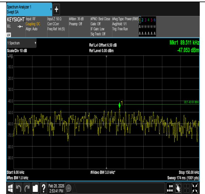
Band4-5MHz-16QAM-20375-25RB#0-0.009~0.15-PASS
