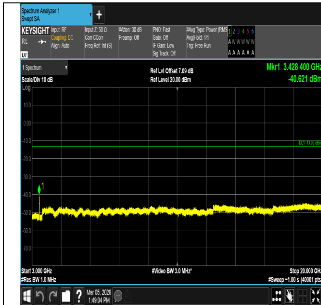
Band4-10MHz-QPSK-20000-50RB#0-3000~20000-PASS
