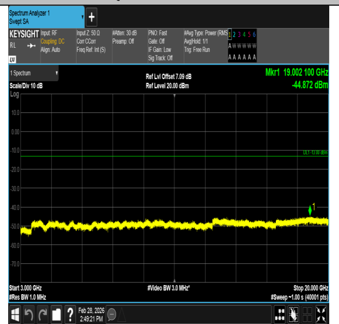
Band4-5MHz-16QAM-20175-25RB#0-3000~20000-PASS
