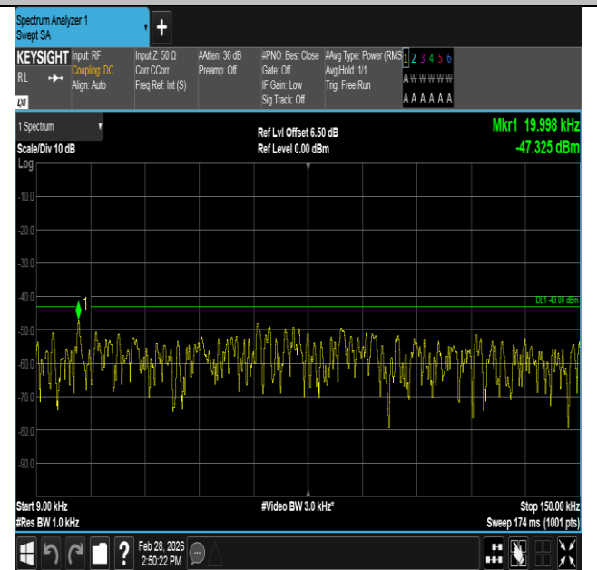
Band4-5MHz-16QAM-20375-1RB#0-0.009~0.15-PASS
