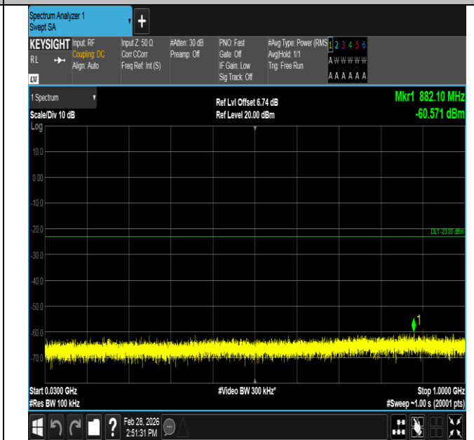
Band4-5MHz-QPSK-20375-1RB#24-30~1000-PASS
