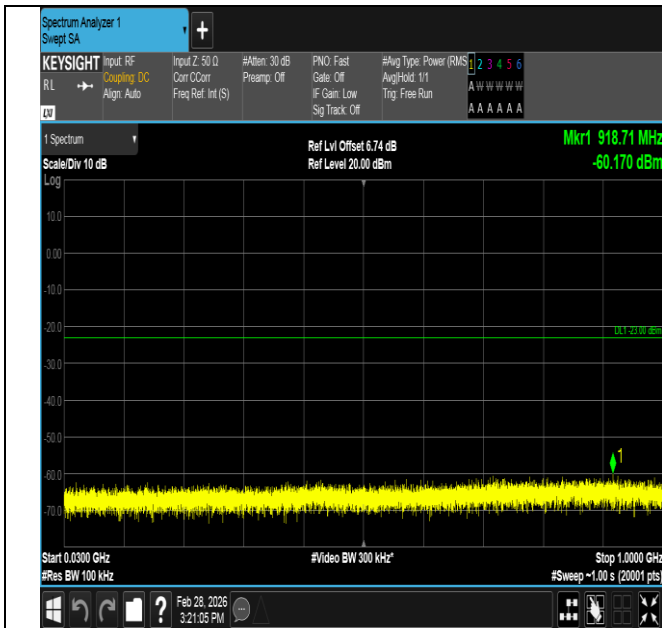
Band4-10MHz-QPSK-20000-1RB#0-30~1000-PASS
