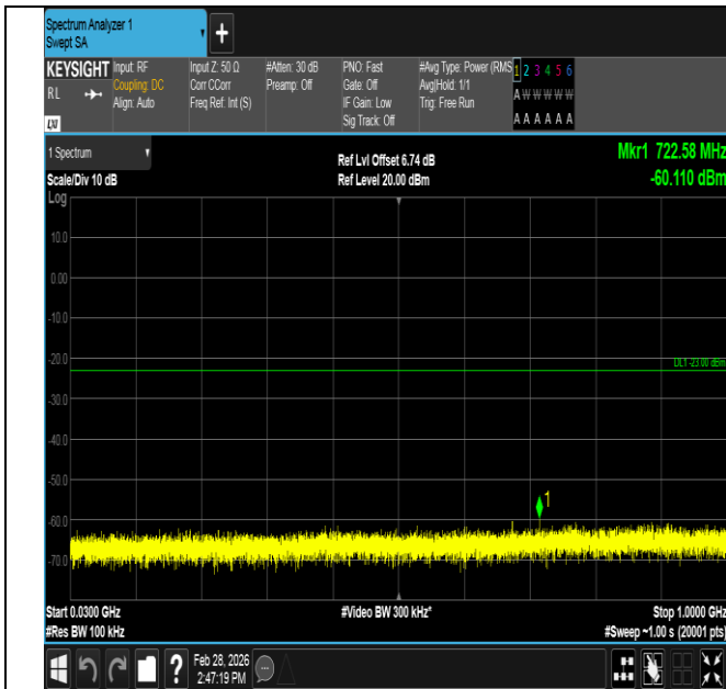
Band4-5MHz-16QAM-20175-1RB#24-30~1000-PASS
