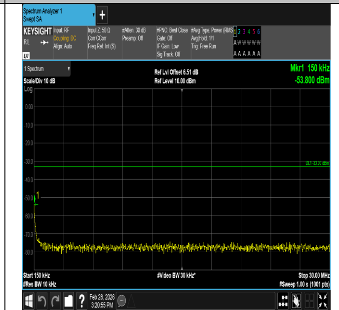
Band4-10MHz-QPSK-20000-1RB#0-0.15~30-PASS
