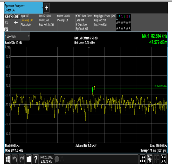
Band4-5MHz-16QAM-20175-25RB#0-0.009~0.15-PASS
