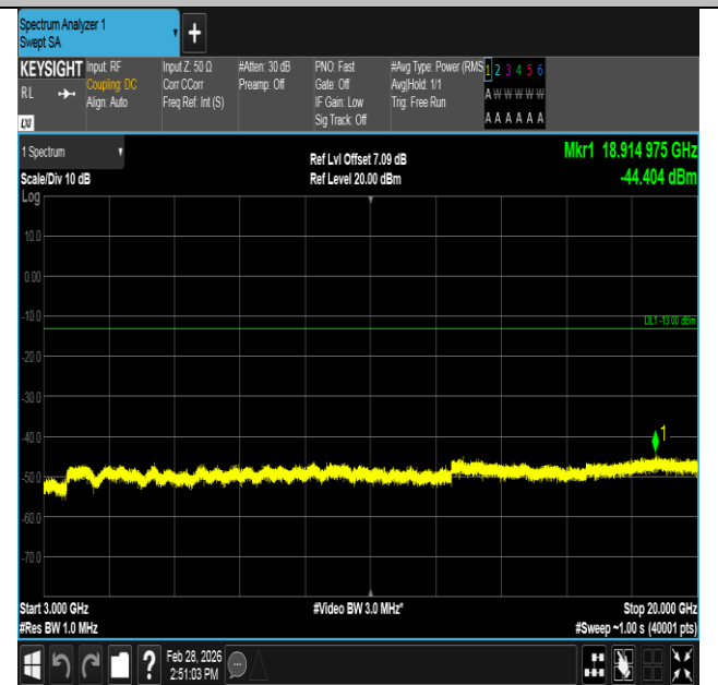
Band4-5MHz-16QAM-20375-1RB#0-3000~20000-PASS
