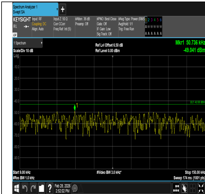
Band4-5MHz-16QAM-20375-1RB#24-0.009~0.15-PASS
