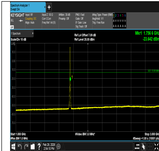
Band4-5MHz-16QAM-20375-25RB#0-1000~3000-PASS
