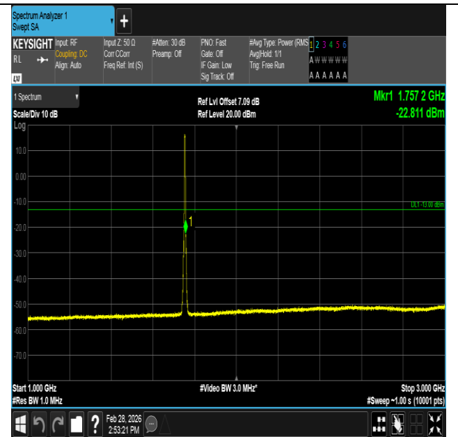
Band4-5MHz-QPSK-20375-25RB#0-1000~3000-PASS
