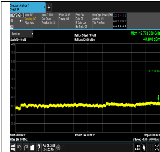
Band4-5MHz-QPSK-20175-25RB#0-3000~20000-PASS
