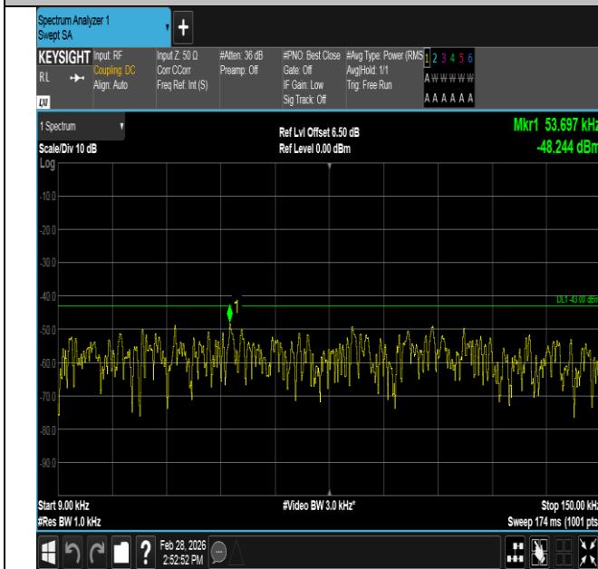
Band4-5MHz-QPSK-20375-25RB#0-0.009~0.15-PASS
