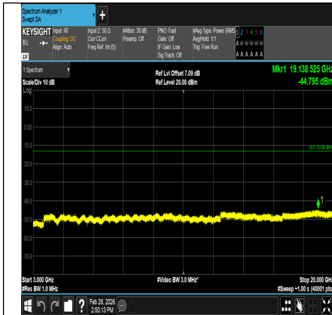
Band4-5MHz-QPSK-20375-1RB#0-3000~20000-PASS
