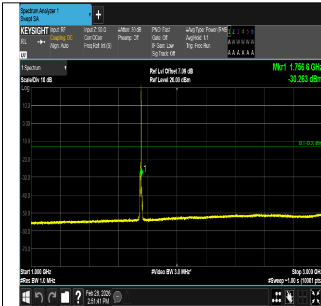
Band4-5MHz-QPSK-20375-1RB#24-1000~3000-PASS
