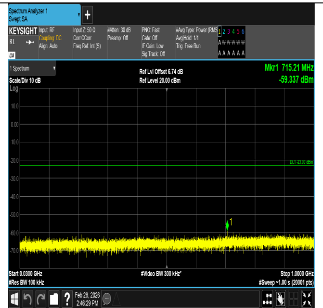
Band4-5MHz-QPSK-20175-1RB#24-30~1000-PASS
