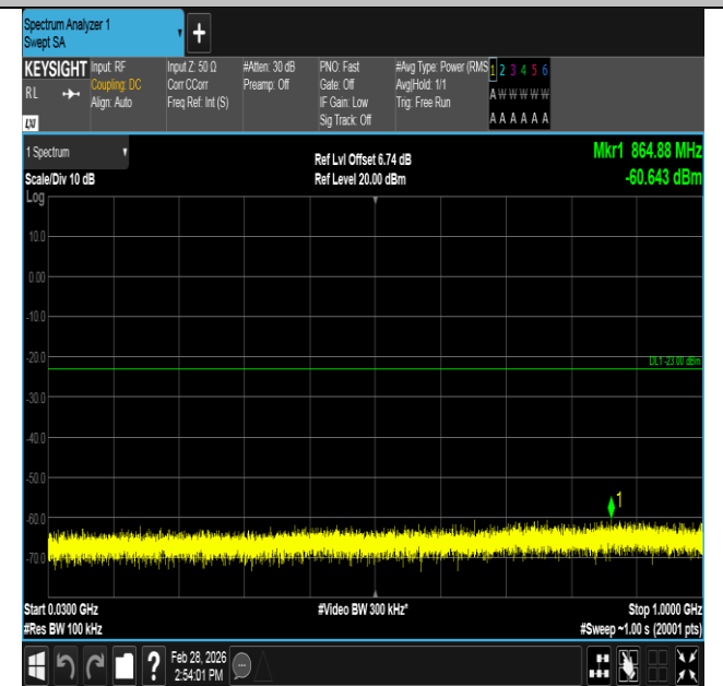
Band4-5MHz-16QAM-20375-25RB#0-30~1000-PASS
