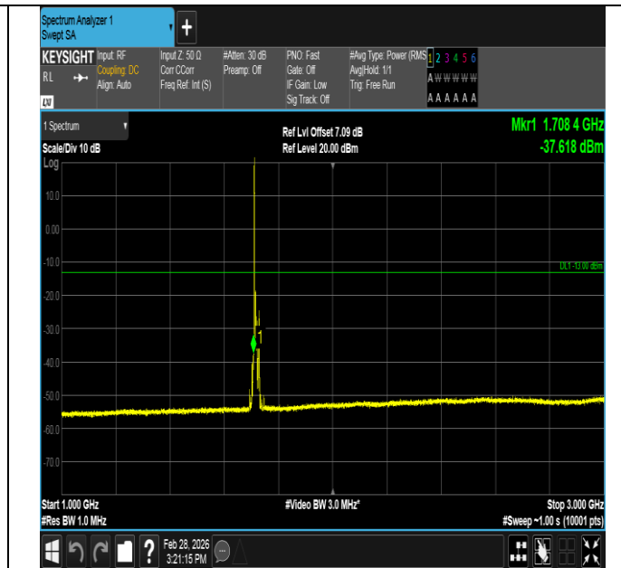
Band4-10MHz-QPSK-20000-1RB#0-1000~3000-PASS
