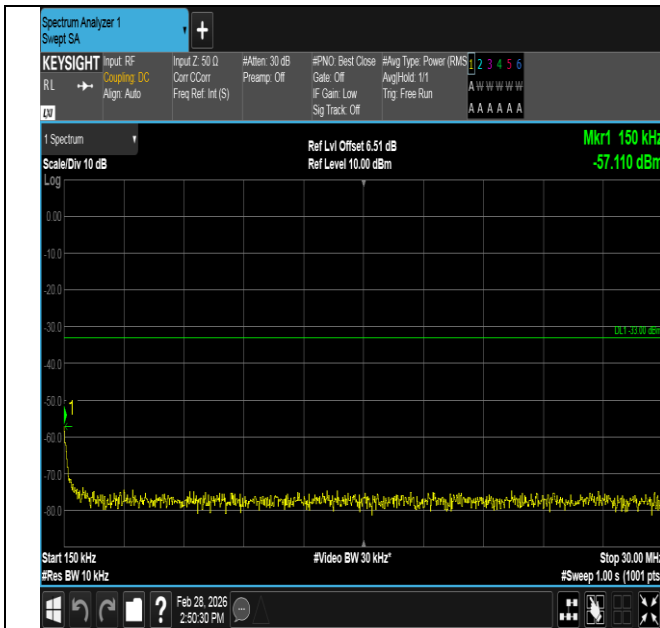
Band4-5MHz-16QAM-20375-1RB#0-0.15~30-PASS
