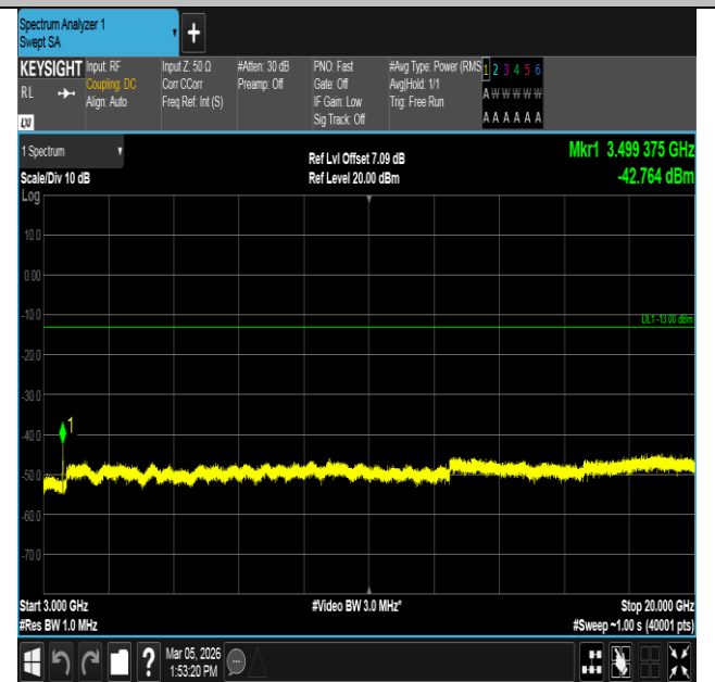
Band4-10MHz-16QAM-20350-50RB#0-3000~20000-PASS
