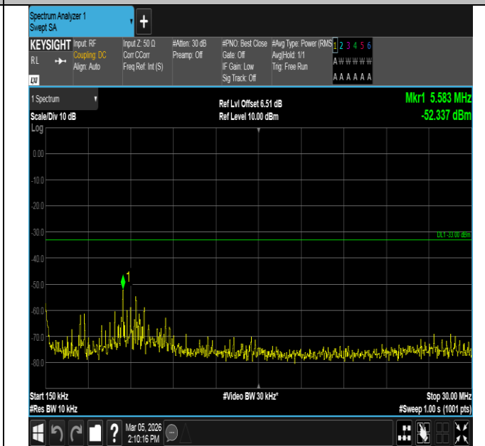
Band4-15MHz-QPSK-20025-75RB#0-0.15~30-PASS
