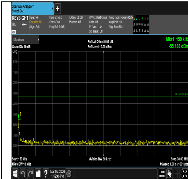
Band4-10MHz-16QAM-20350-50RB#0-0.15~30-PASS
