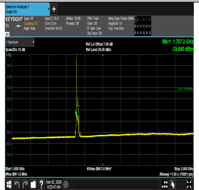
Band4-15MHz-QPSK-20025-1RB#0-1000~3000-PASS
