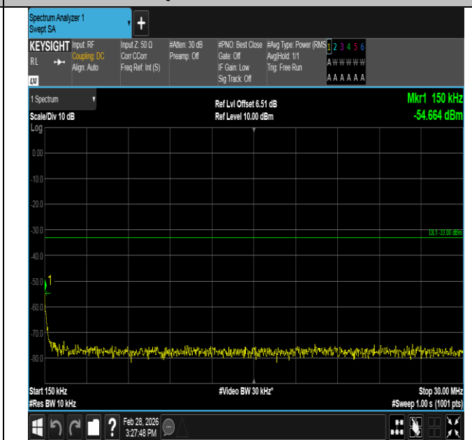
Band4-10MHz-QPSK-20350-1RB#0-0.15~30-PASS
