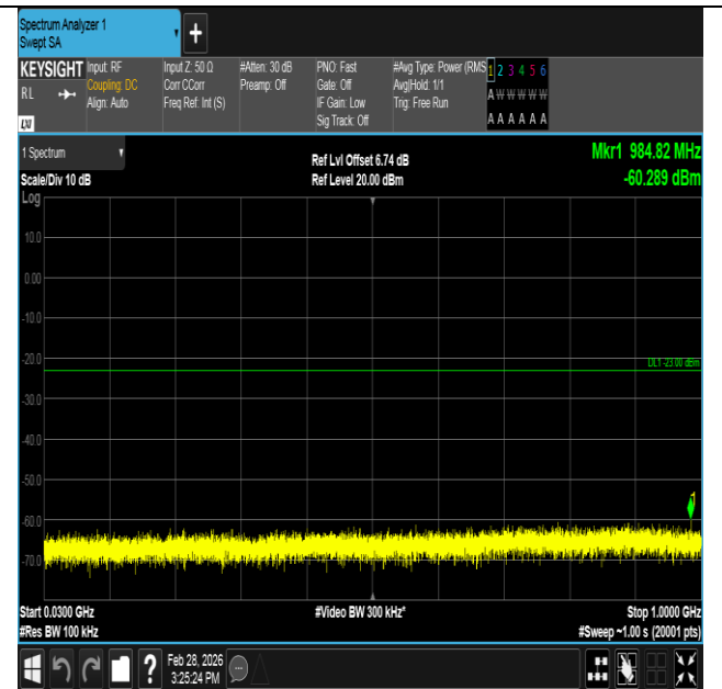
Band4-10MHz-16QAM-20175-1RB#0-30~1000-PASS
