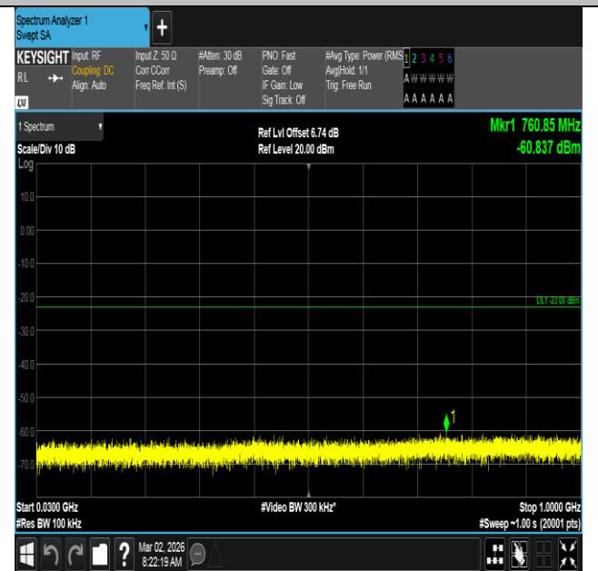
Band4-15MHz-QPSK-20025-1RB#74-30~1000-PASS
