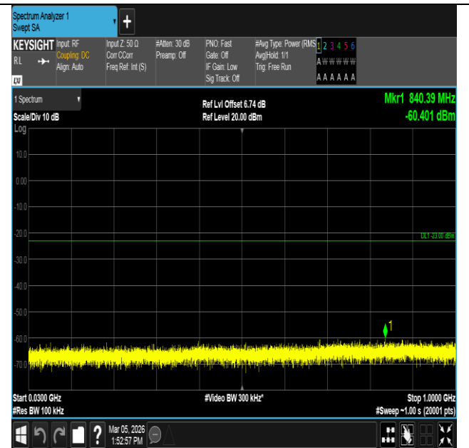
Band4-10MHz-16QAM-20350-50RB#0-30~1000-PASS
