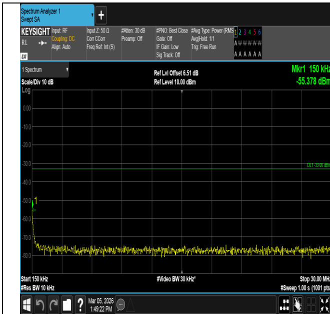
Band4-10MHz-16QAM-20000-50RB#0-0.15~30-PASS
