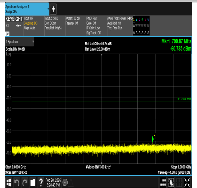
Band4-10MHz-16QAM-20350-1RB#0-30~1000-PASS
