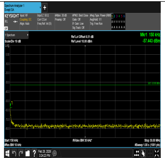
Band4-10MHz-QPSK-20175-1RB#0-0.15~30-PASS
