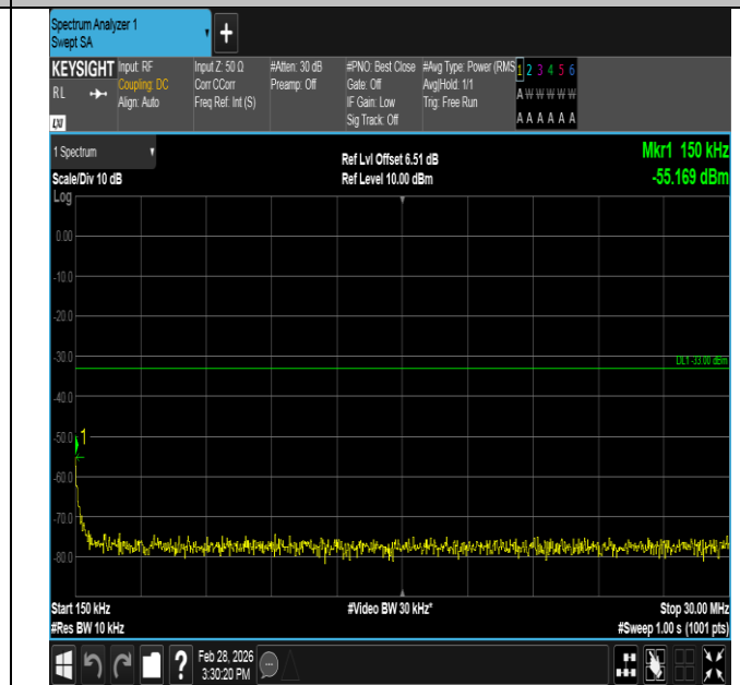
Band4-10MHz-16QAM-20350-1RB#49-0.15~30-PASS
