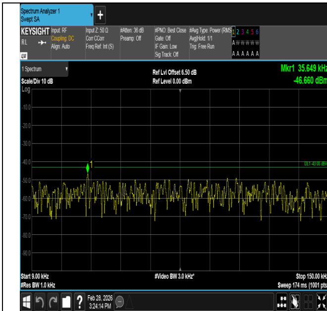
Band4-10MHz-QPSK-20175-1RB#0-0.009~0.15-PASS
