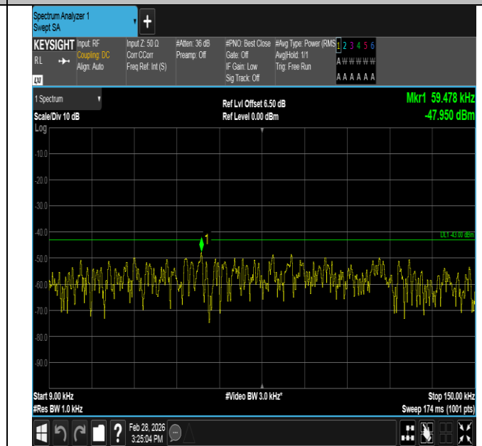
Band4-10MHz-16QAM-20175-1RB#0-0.009~0.15-PASS
