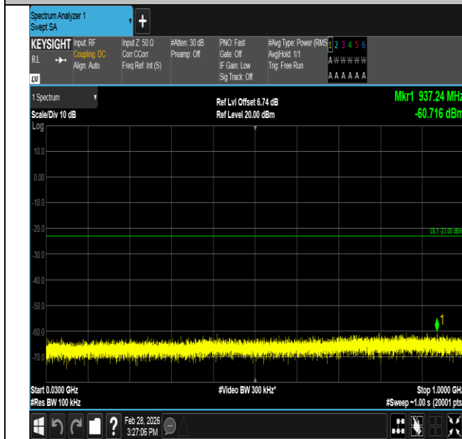
Band4-10MHz-16QAM-20175-1RB#49-30~1000-PASS
