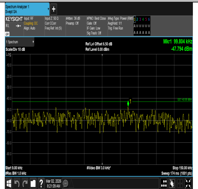
Band4-15MHz-16QAM-20025-1RB#0-0.009~0.15-PASS
