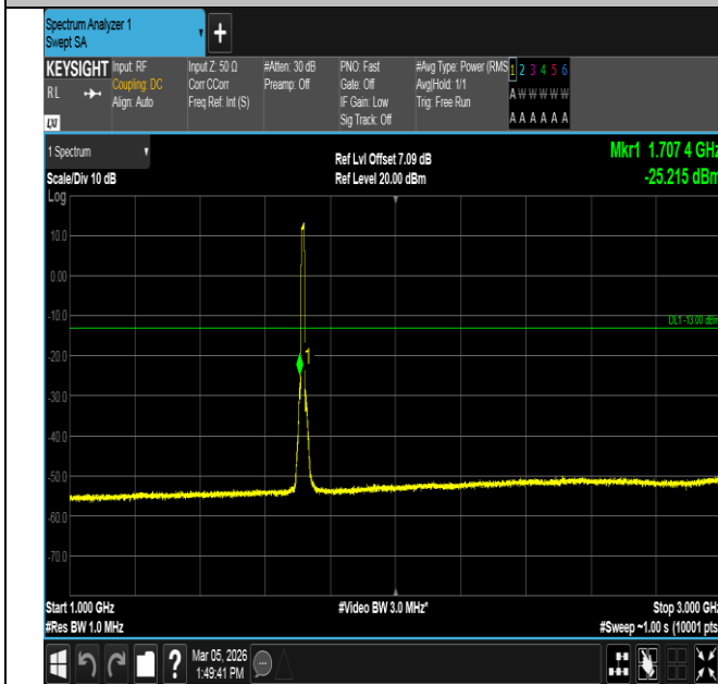
Band4-10MHz-16QAM-20000-50RB#0-1000~3000-PASS
