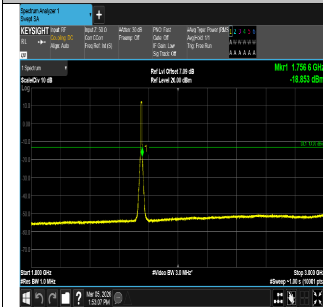
Band4-10MHz-16QAM-20350-50RB#0-1000~3000-PASS
