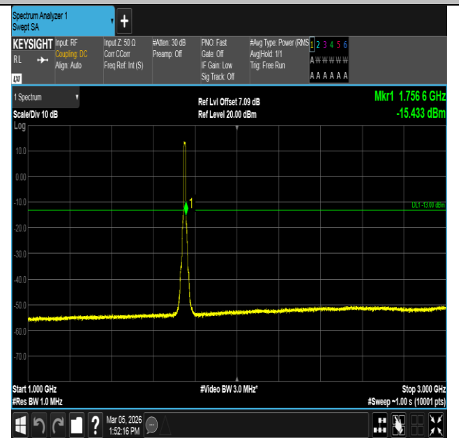
Band4-10MHz-QPSK-20350-50RB#0-1000~3000-PASS
