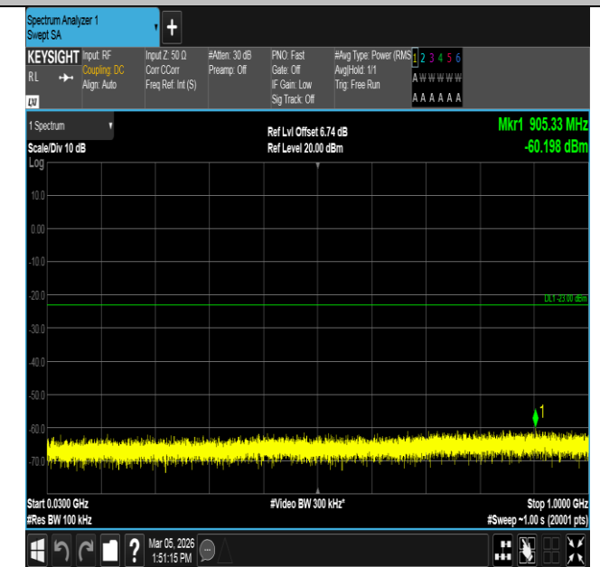
Band4-10MHz-16QAM-20175-50RB#0-30~1000-PASS
