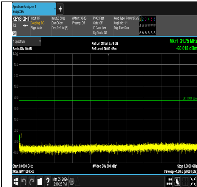
Band4-15MHz-QPSK-20025-75RB#0-30~1000-PASS
