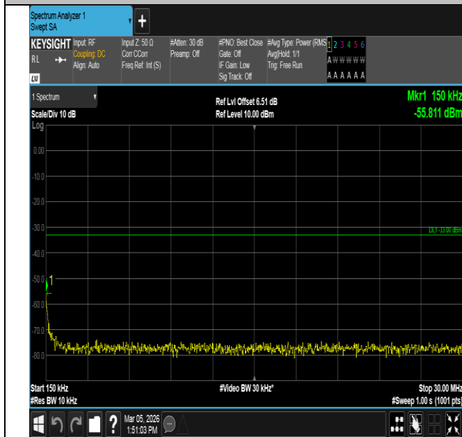
Band4-10MHz-16QAM-20175-50RB#0-0.15~30-PASS
