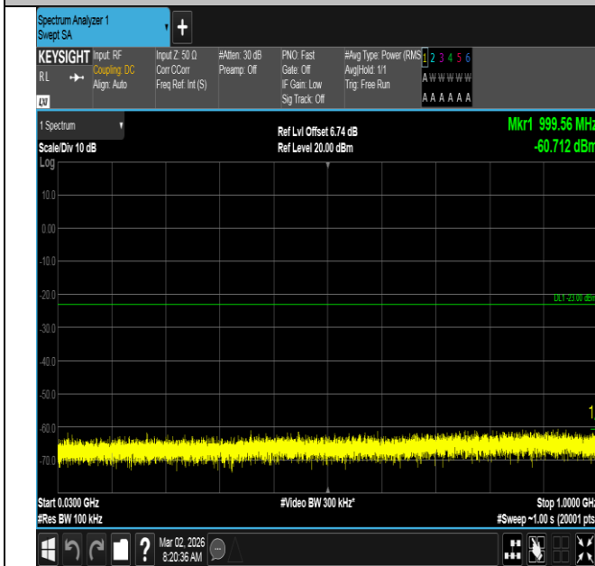
Band4-15MHz-QPSK-20025-1RB#0-30~1000-PASS
