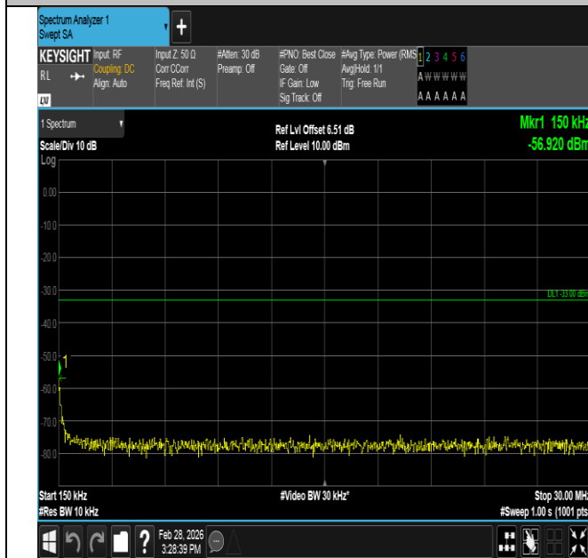
Band4-10MHz-16QAM-20350-1RB#0-0.15~30-PASS
