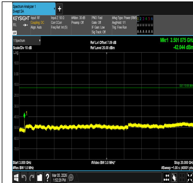
Band4-10MHz-QPSK-20350-50RB#0-3000~20000-PASS
