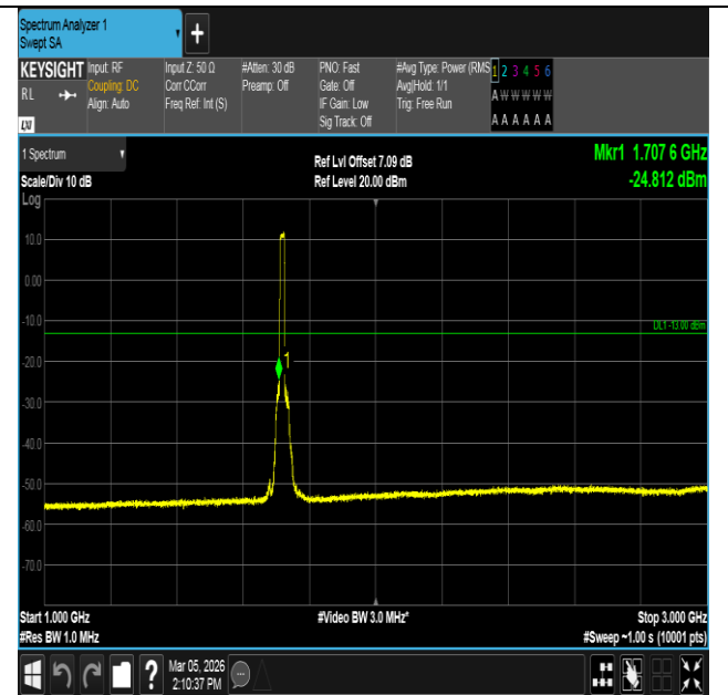
Band4-15MHz-QPSK-20025-75RB#0-1000~3000-PASS
