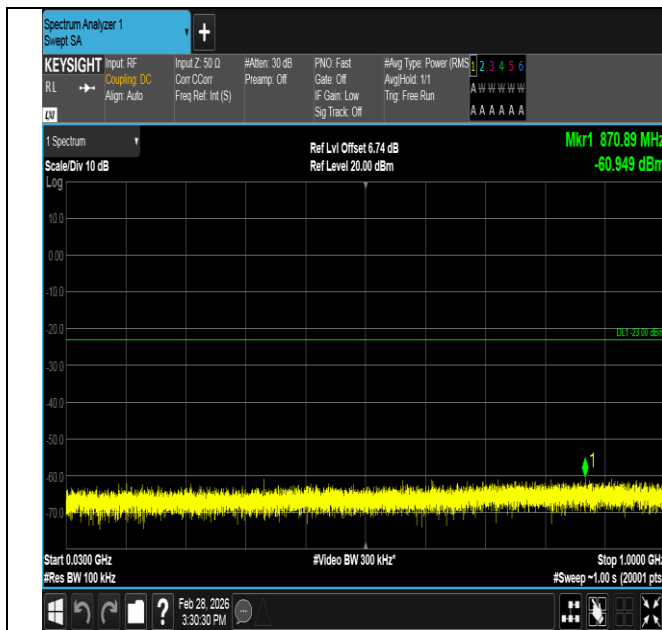
Band4-10MHz-16QAM-20350-1RB#49-30~1000-PASS
