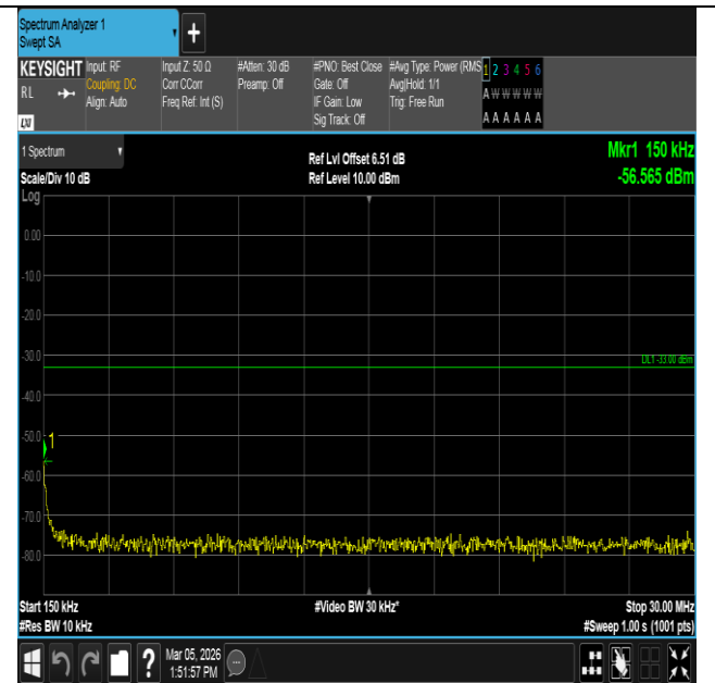
Band4-10MHz-QPSK-20350-50RB#0-0.15~30-PASS
