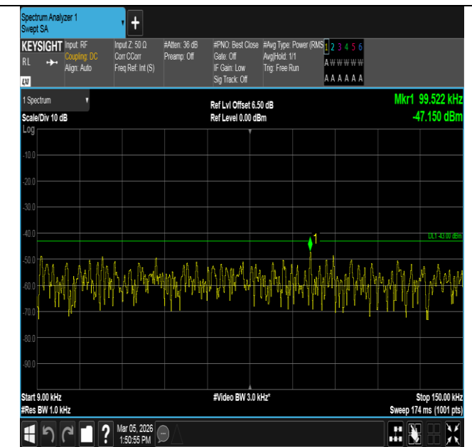
Band4-10MHz-16QAM-20175-50RB#0-0.009~0.15-PASS
