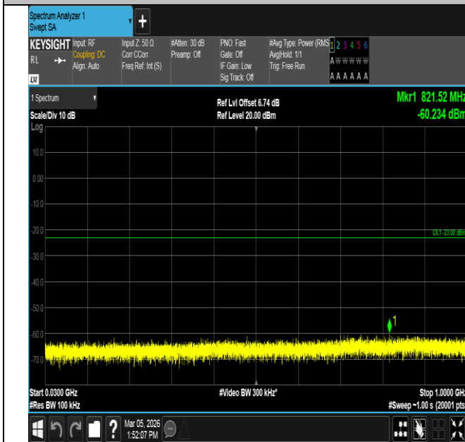
Band4-10MHz-QPSK-20350-50RB#0-30~1000-PASS
