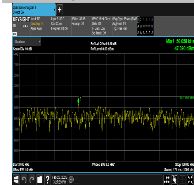
Band4-10MHz-QPSK-20350-1RB#0-0.009~0.15-PASS
