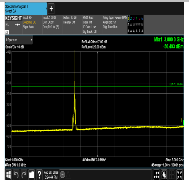
Band4-10MHz-QPSK-20175-1RB#0-1000~3000-PASS
