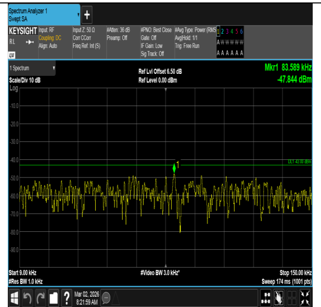
Band4-15MHz-QPSK-20025-1RB#74-0.009~0.15-PASS
