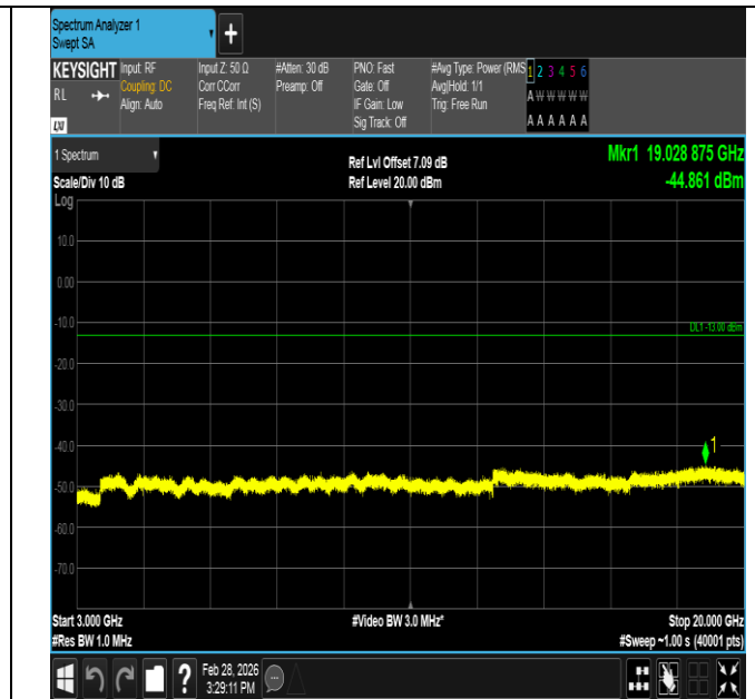
Band4-10MHz-16QAM-20350-1RB#0-3000~20000-PASS
