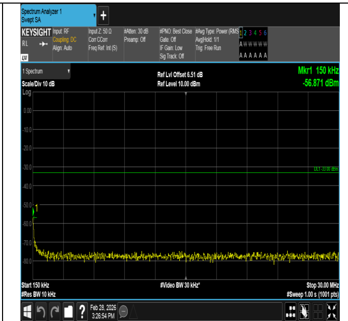
Band4-10MHz-16QAM-20175-1RB#49-0.15~30-PASS
