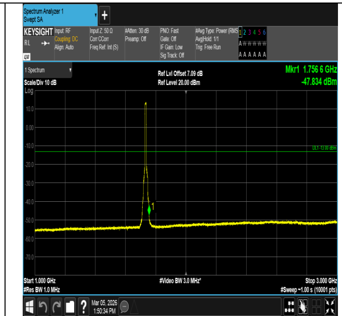
Band4-10MHz-QPSK-20175-50RB#0-1000~3000-PASS
