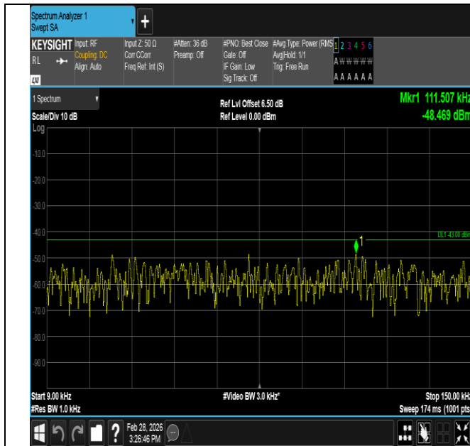
Band4-10MHz-16QAM-20175-1RB#49-0.009~0.15-PASS
