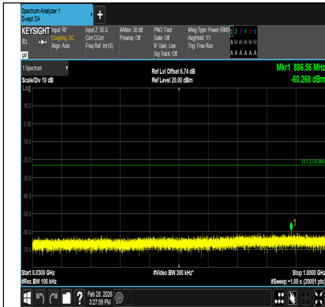
Band4-10MHz-QPSK-20350-1RB#0-30~1000-PASS
