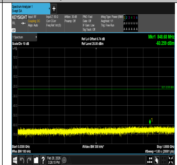
Band4-10MHz-QPSK-20175-1RB#49-30~1000-PASS
