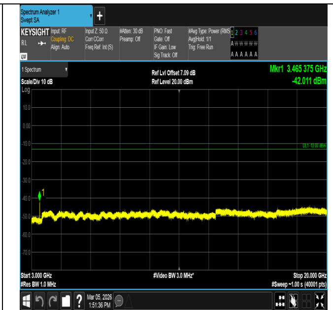
Band4-10MHz-16QAM-20175-50RB#0-3000~20000-PASS
