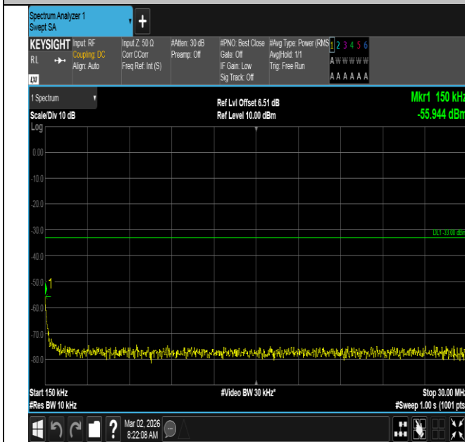
Band4-15MHz-QPSK-20025-1RB#74-0.15~30-PASS
