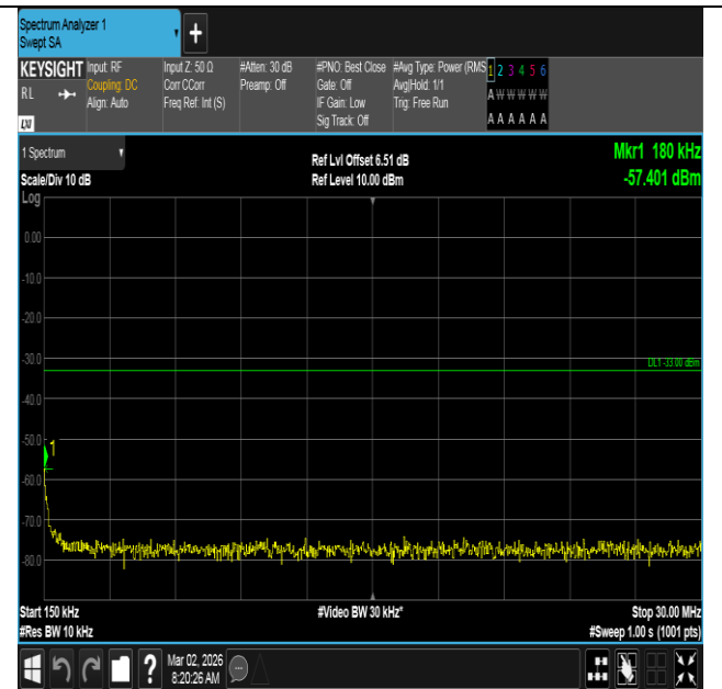
Band4-15MHz-QPSK-20025-1RB#0-0.15~30-PASS
