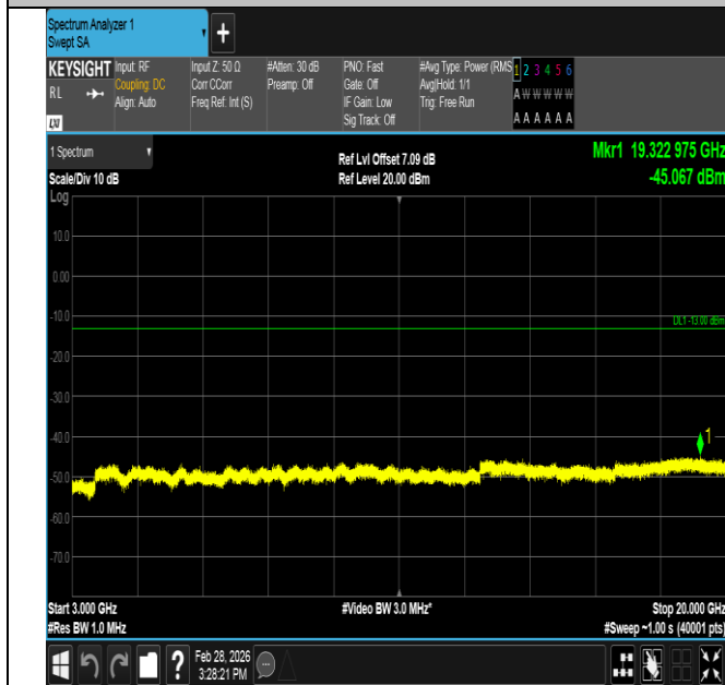
Band4-10MHz-QPSK-20350-1RB#0-3000~20000-PASS
