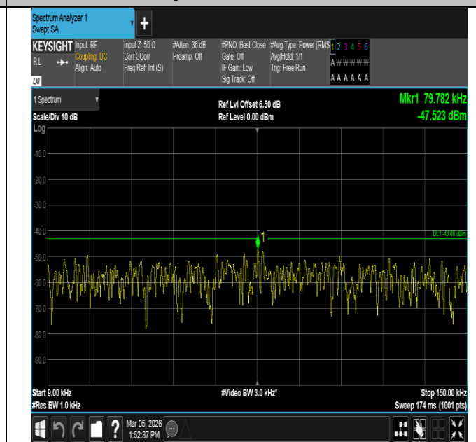
Band4-10MHz-16QAM-20350-50RB#0-0.009~0.15-PASS
