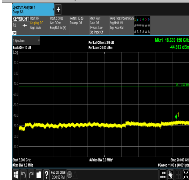
Band4-10MHz-16QAM-20350-1RB#49-3000~20000-PASS
