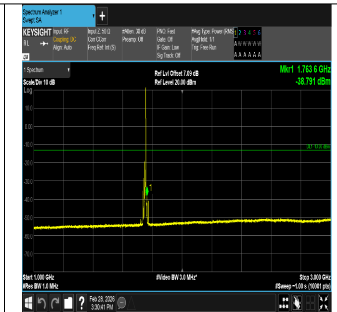
Band4-10MHz-16QAM-20350-1RB#49-1000~3000-PASS
