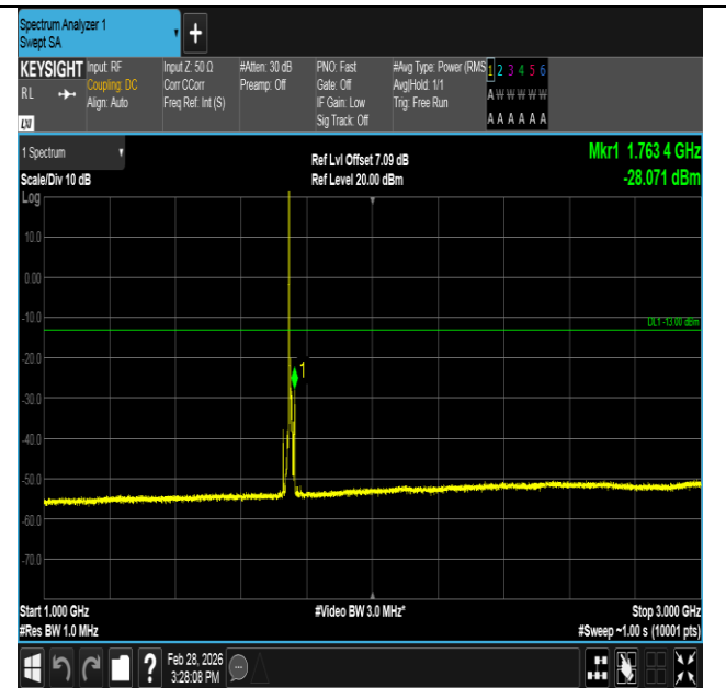
Band4-10MHz-QPSK-20350-1RB#0-1000~3000-PASS
