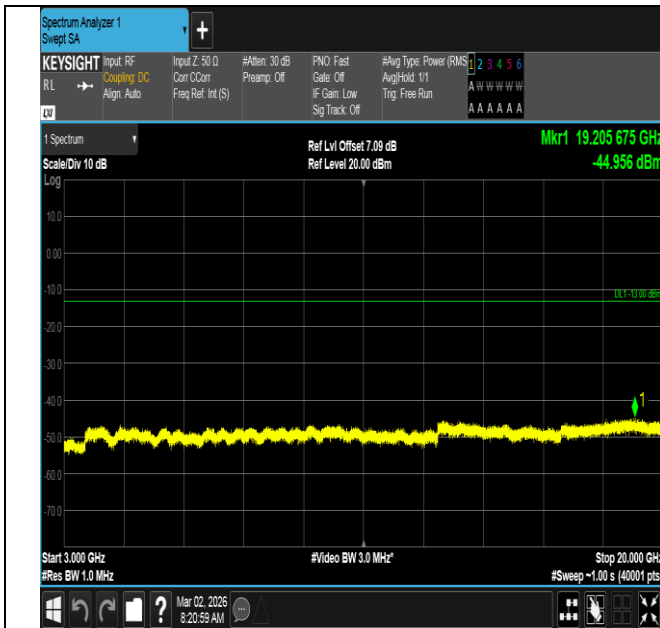
Band4-15MHz-QPSK-20025-1RB#0-3000~20000-PASS
