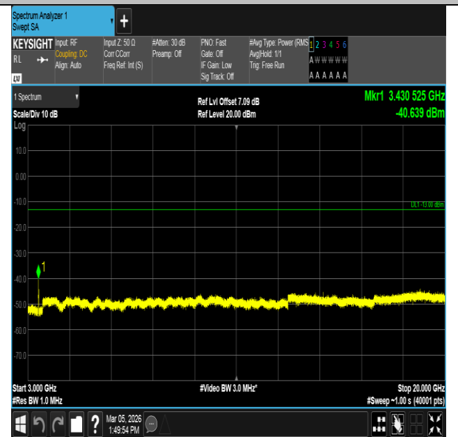
Band4-10MHz-16QAM-20000-50RB#0-3000~20000-PASS
