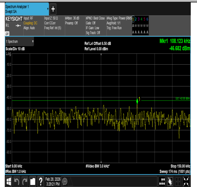
Band4-10MHz-QPSK-20350-1RB#49-0.009~0.15-PASS
