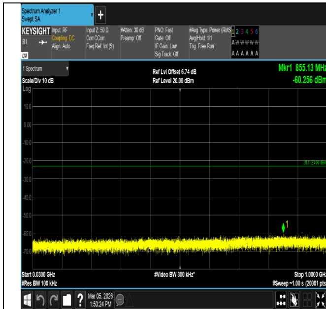
Band4-10MHz-QPSK-20175-50RB#0-30~1000-PASS
