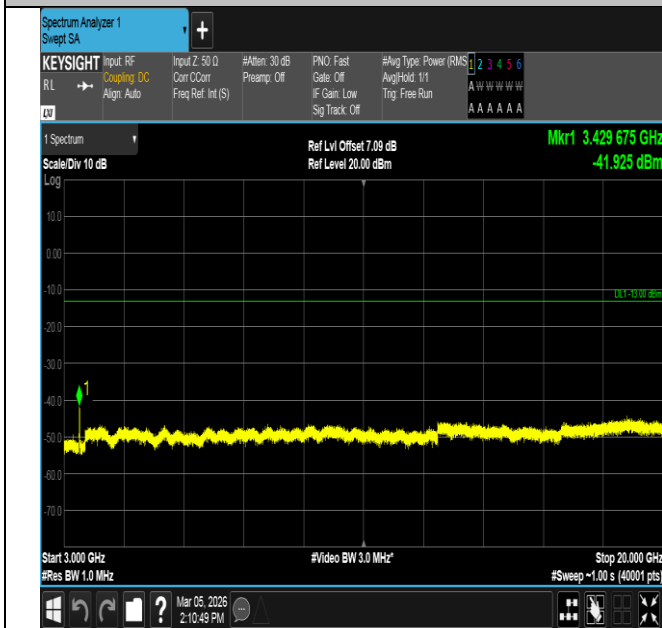
Band4-15MHz-QPSK-20025-75RB#0-3000~20000-PASS
