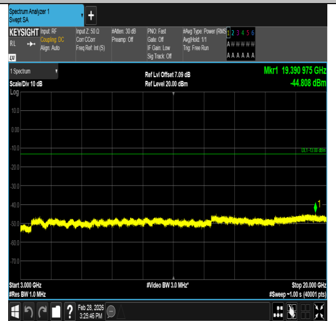
Band4-10MHz-16QAM-20175-1RB#0-3000~20000-PASS
