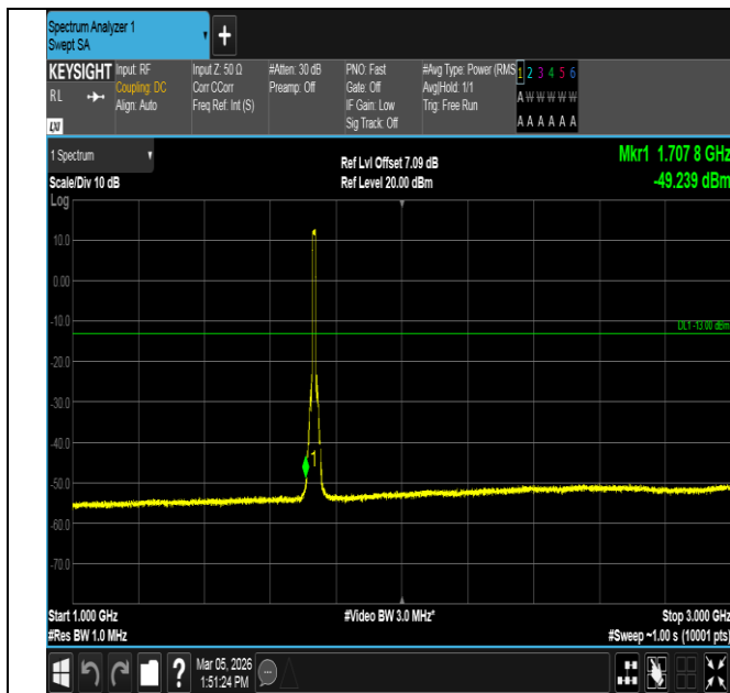
Band4-10MHz-16QAM-20175-50RB#0-1000~3000-PASS
