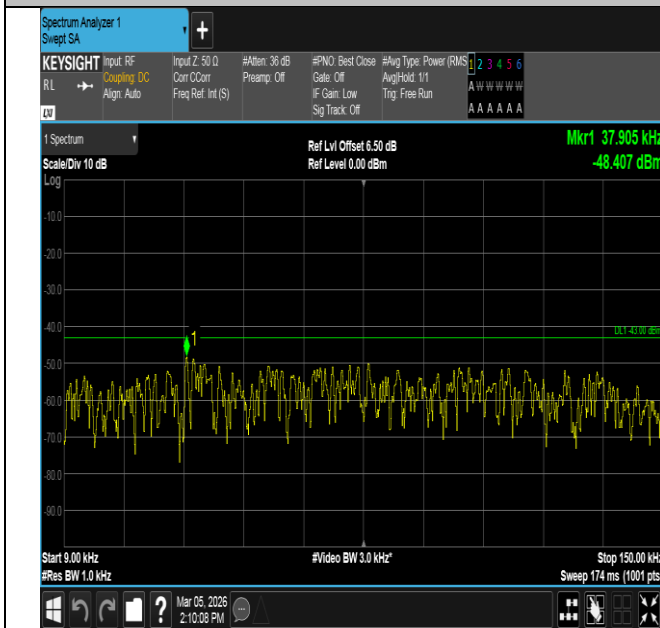
Band4-15MHz-QPSK-20025-75RB#0-0.009~0.15-PASS
