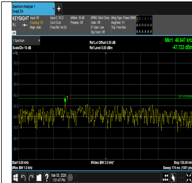
Band4-10MHz-QPSK-20350-50RB#0-0.009~0.15-PASS
