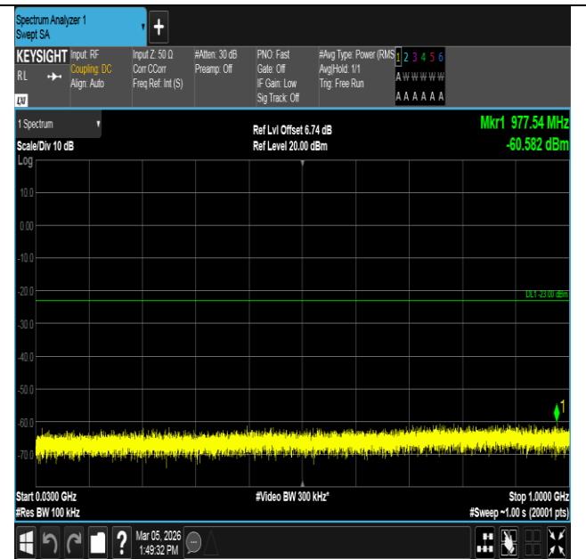
Band4-10MHz-16QAM-20000-50RB#0-30~1000-PASS
