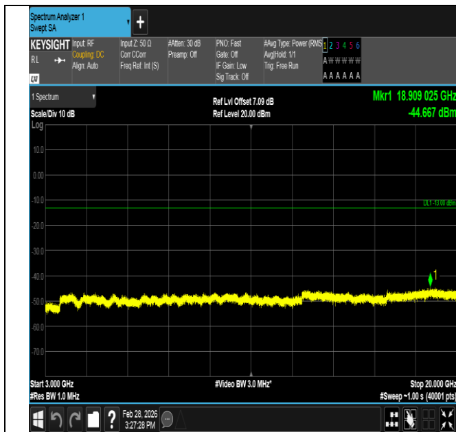
Band4-10MHz-16QAM-20175-1RB#49-3000~20000-PASS
