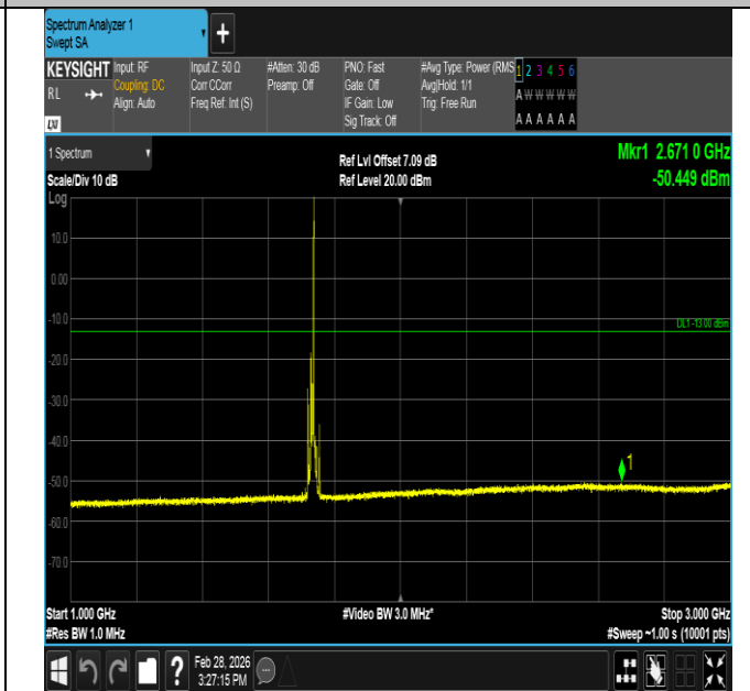
Band4-10MHz-16QAM-20175-1RB#49-1000~3000-PASS
