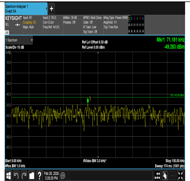
Band4-10MHz-16QAM-20350-1RB#0-0.009~0.15-PASS
