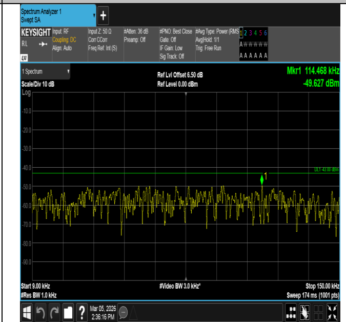
Band4-20MHz-16QAM-20300-100RB#0-0.009~0.15-PASS
