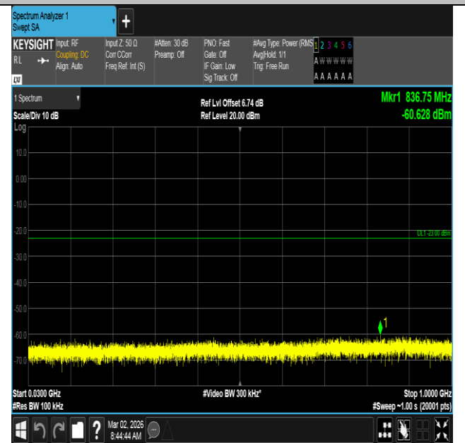
Band4-20MHz-16QAM-20050-1RB#0-30~1000-PASS
