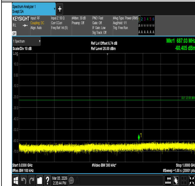
Band4-20MHz-QPSK-20300-100RB#0-30~1000-PASS
