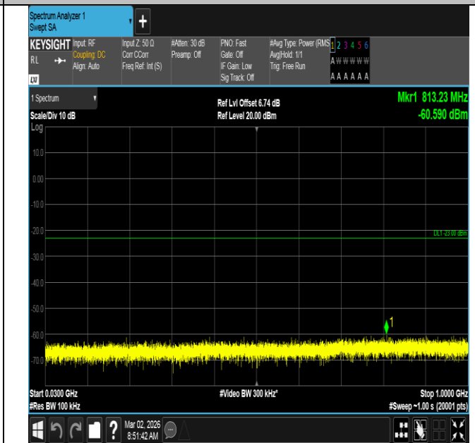
Band4-20MHz-16QAM-20300-1RB#0-30~1000-PASS
