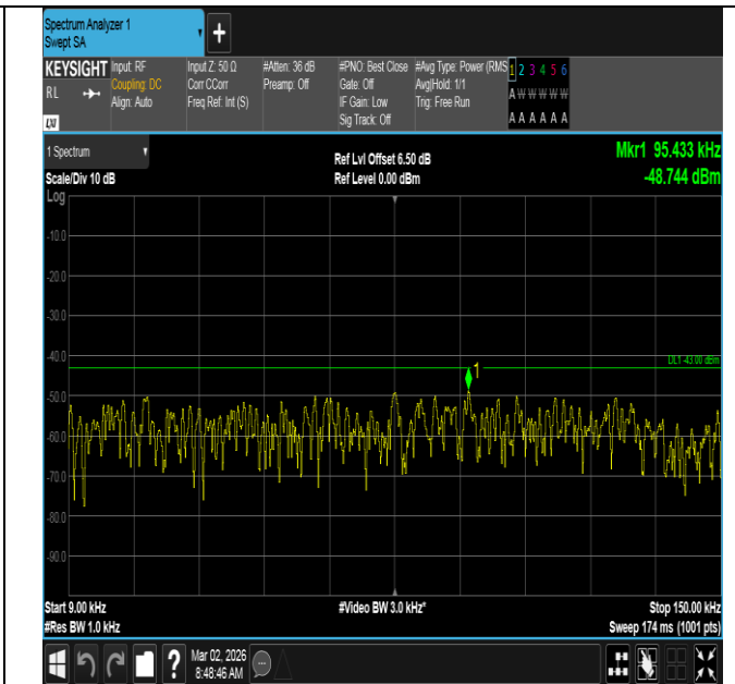
Band4-20MHz-QPSK-20175-1RB#99-0.009~0.15-PASS
