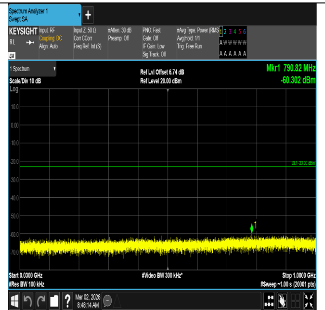
Band4-20MHz-16QAM-20175-1RB#0-30~1000-PASS
