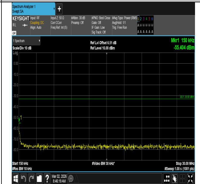
Band4-20MHz-16QAM-20050-1RB#99-0.15~30-PASS
