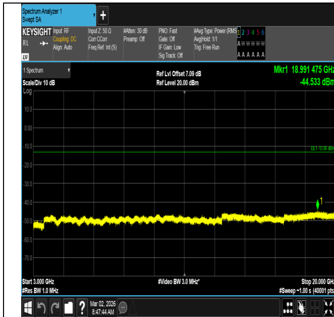
Band4-20MHz-QPSK-20175-1RB#0-3000~20000-PASS
