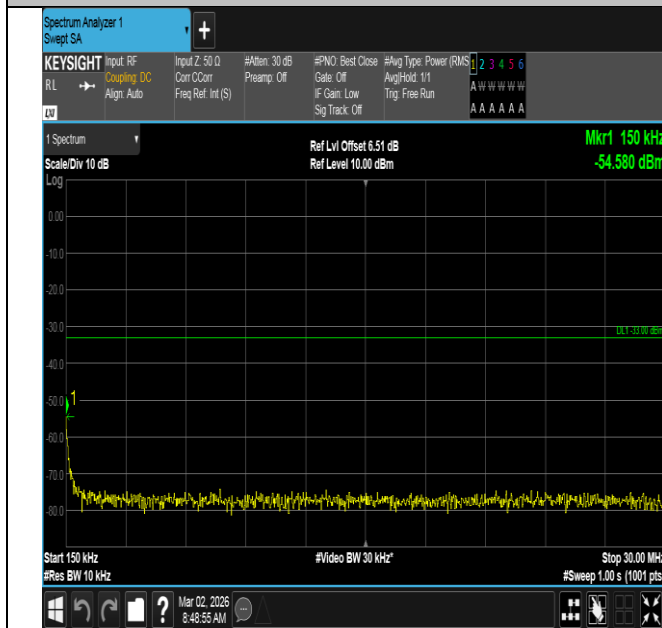
Band4-20MHz-QPSK-20175-1RB#99-0.15~30-PASS
