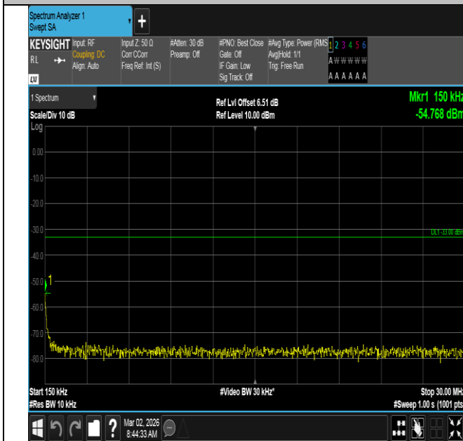
Band4-20MHz-16QAM-20050-1RB#0-0.15~30-PASS
