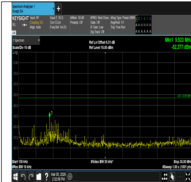
Band4-20MHz-16QAM-20050-100RB#0-0.15~30-PASS
