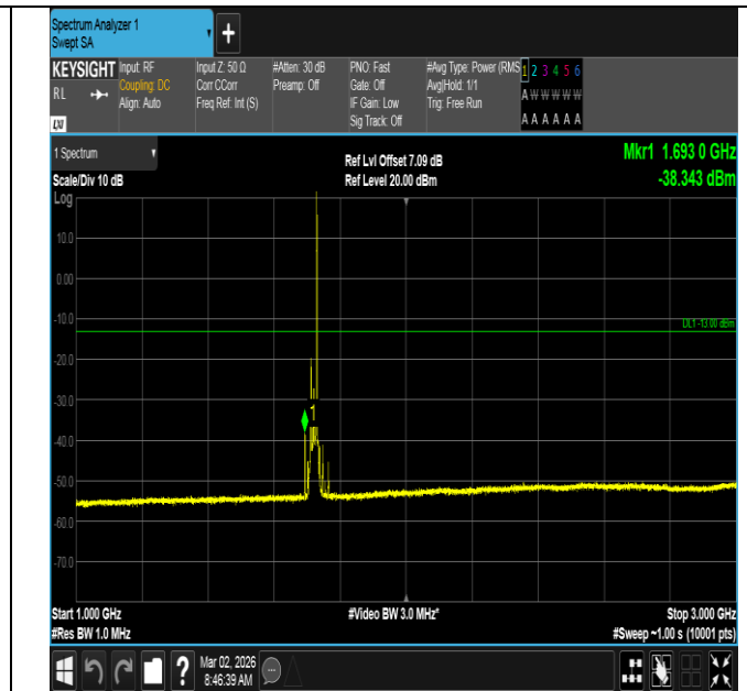
Band4-20MHz-16QAM-20050-1RB#99-1000~3000-PASS
