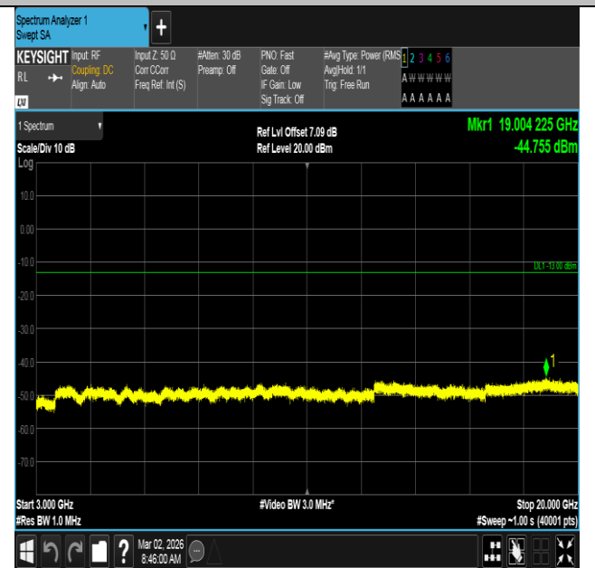
Band4-20MHz-QPSK-20050-1RB#99-3000~20000-PASS
