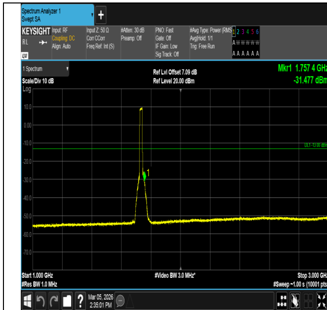
Band4-20MHz-16QAM-20175-100RB#0-1000~3000-PASS
