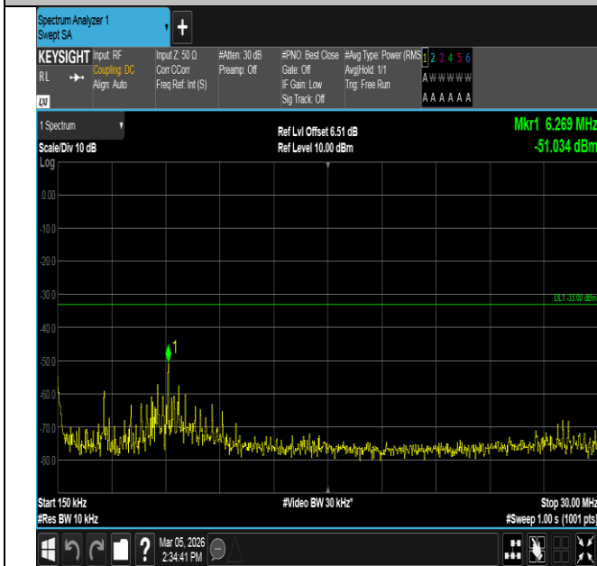
Band4-20MHz-16QAM-20175-100RB#0-0.15~30-PASS
