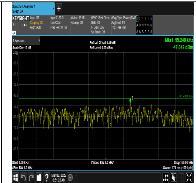
Band4-20MHz-16QAM-20300-1RB#0-0.009~0.15-PASS
