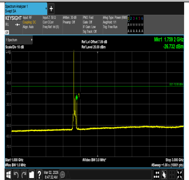
Band4-20MHz-QPSK-20175-1RB#0-1000~3000-PASS
