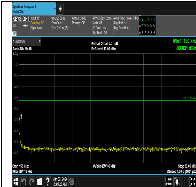
Band4-20MHz-QPSK-20050-1RB#99-0.15~30-PASS
