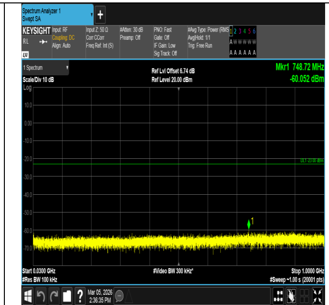
Band4-20MHz-16QAM-20300-100RB#0-30~1000-PASS
