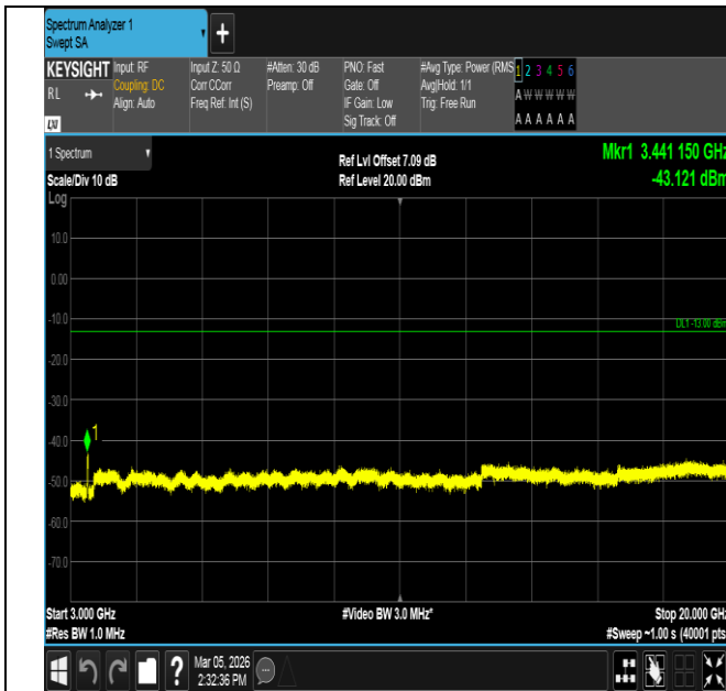
Band4-20MHz-QPSK-20050-100RB#0-3000~20000-PASS
