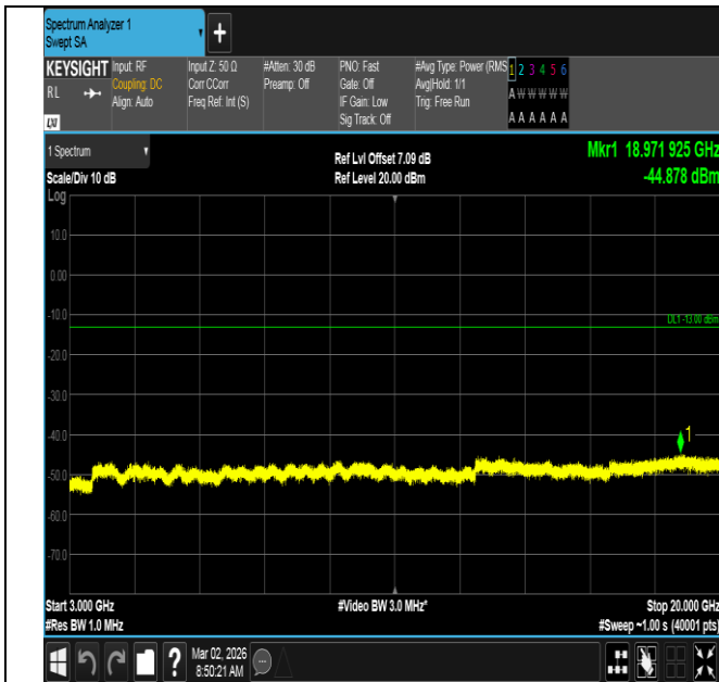
Band4-20MHz-16QAM-20175-1RB#99-3000~20000-PASS
