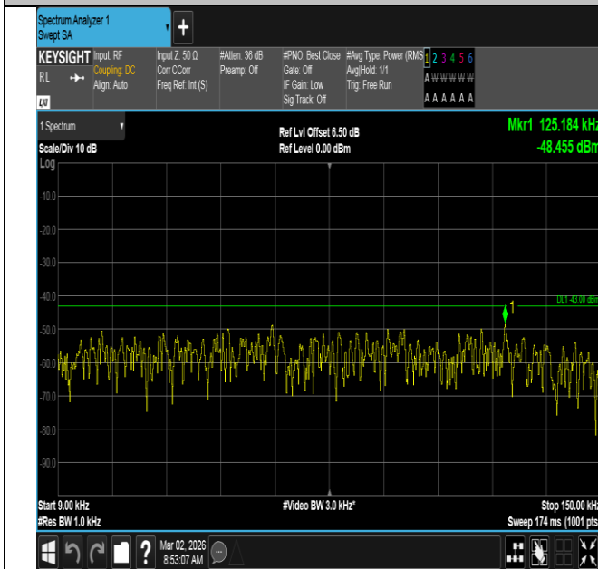
Band4-20MHz-16QAM-20300-1RB#99-0.009~0.15-PASS
