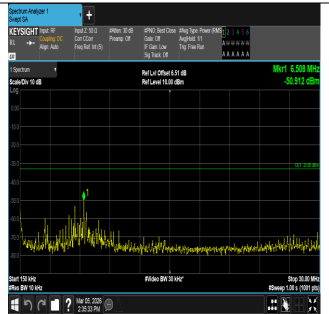
Band4-20MHz-QPSK-20300-100RB#0-0.15~30-PASS
