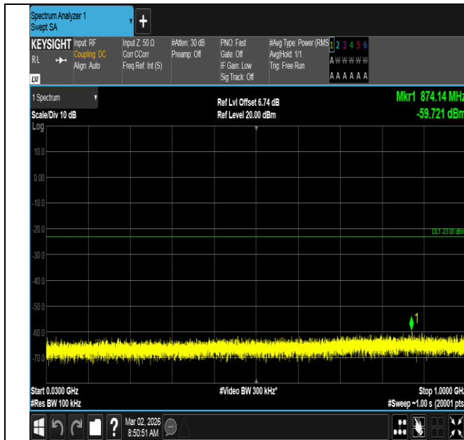
Band4-20MHz-QPSK-20300-1RB#0-30~1000-PASS
