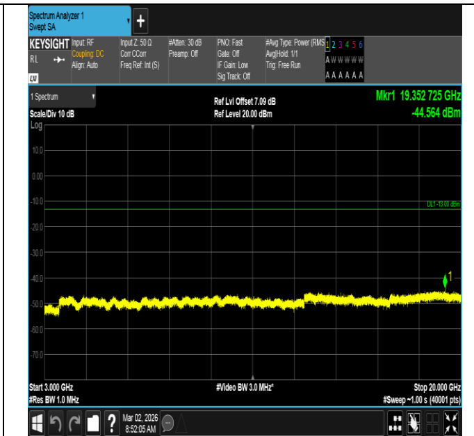
Band4-20MHz-16QAM-20300-1RB#0-3000~20000-PASS
