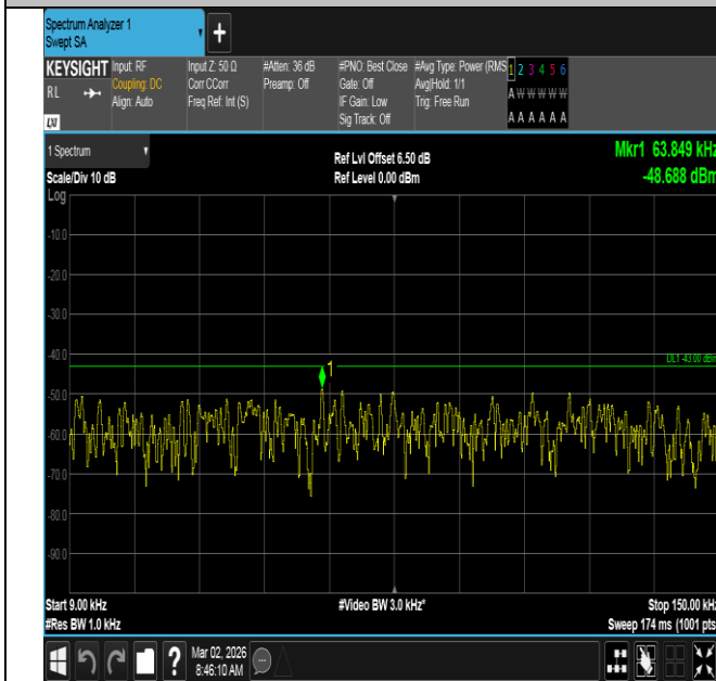
Band4-20MHz-16QAM-20050-1RB#99-0.009~0.15-PASS
