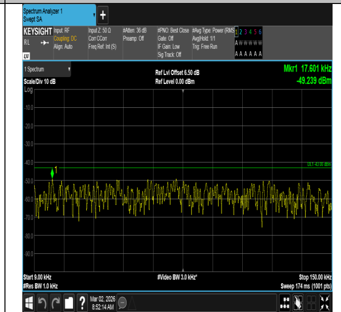
Band4-20MHz-QPSK-20300-1RB#99-0.009~0.15-PASS
