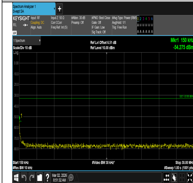
Band4-20MHz-16QAM-20300-1RB#0-0.15~30-PASS
