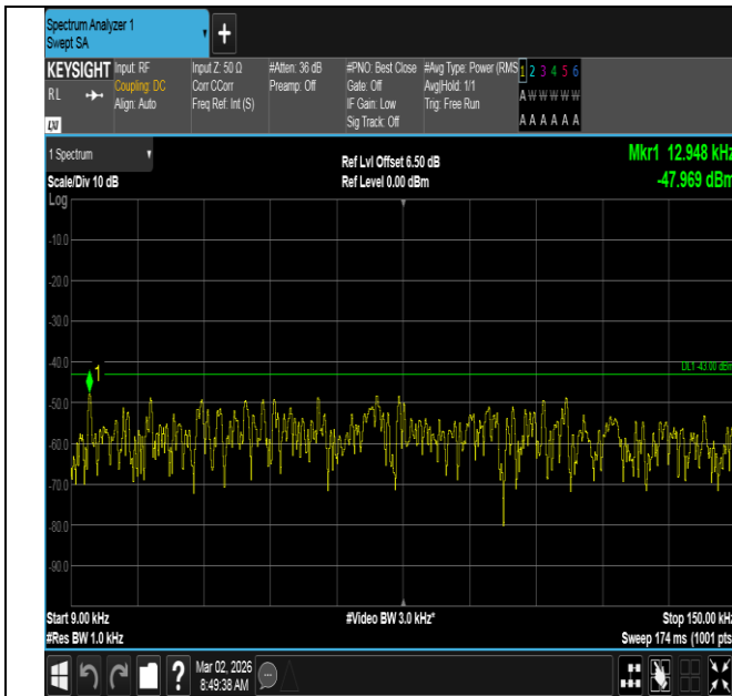
Band4-20MHz-16QAM-20175-1RB#99-0.009~0.15-PASS
