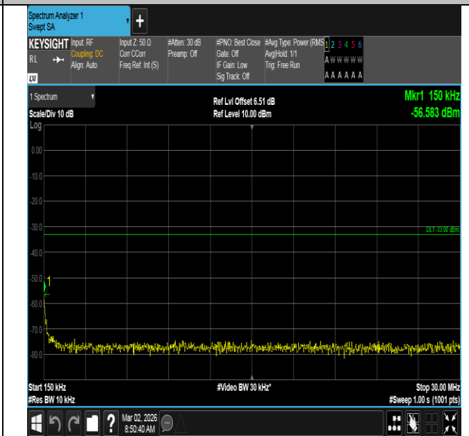
Band4-20MHz-QPSK-20300-1RB#0-0.15~30-PASS
