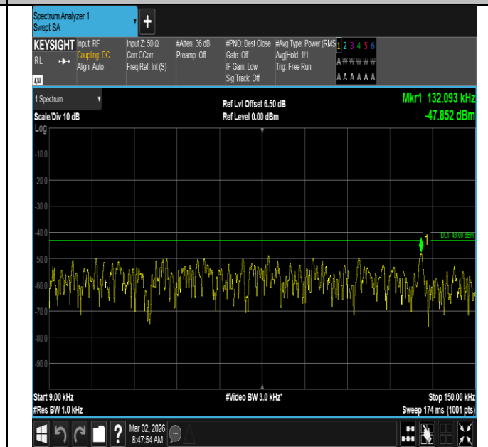
Band4-20MHz-16QAM-20175-1RB#0-0.009~0.15-PASS
