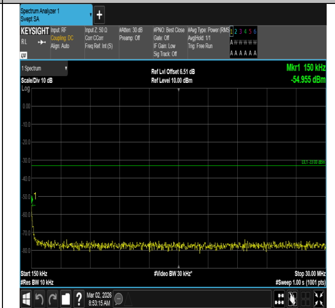
Band4-20MHz-16QAM-20300-1RB#99-0.15~30-PASS
