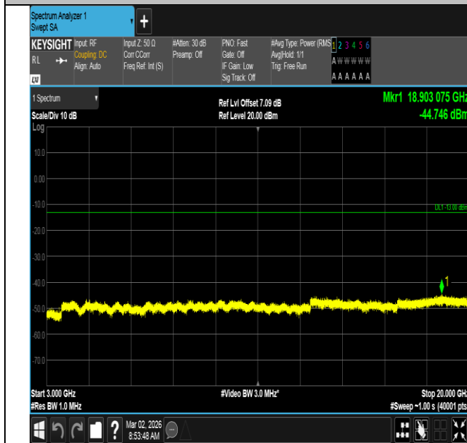
Band4-20MHz-16QAM-20300-1RB#99-3000~20000-PASS
