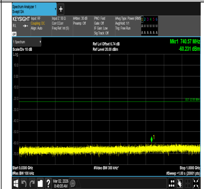
Band4-20MHz-QPSK-20175-1RB#99-30~1000-PASS
