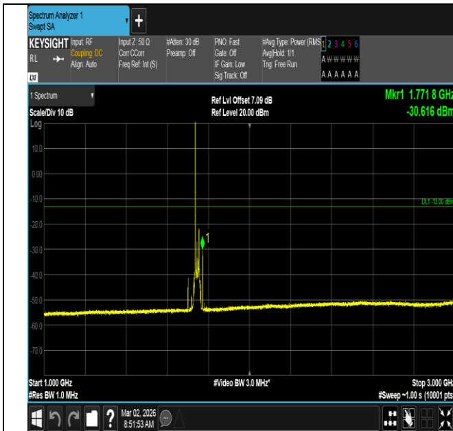
Band4-20MHz-16QAM-20300-1RB#0-1000~3000-PASS
