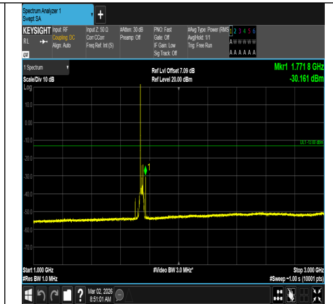
Band4-20MHz-QPSK-20300-1RB#0-1000~3000-PASS
