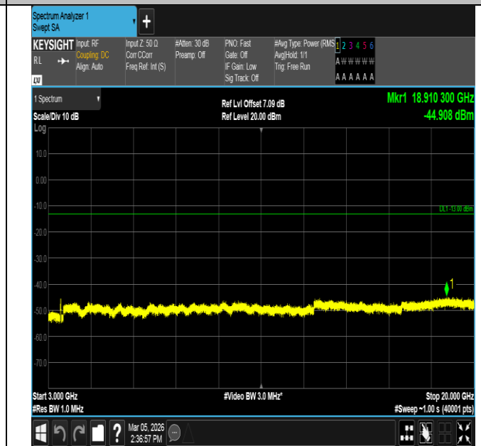
Band4-20MHz-16QAM-20300-100RB#0-3000~20000-PASS
