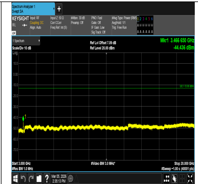
Band4-20MHz-16QAM-20175-100RB#0-3000~20000-PASS
