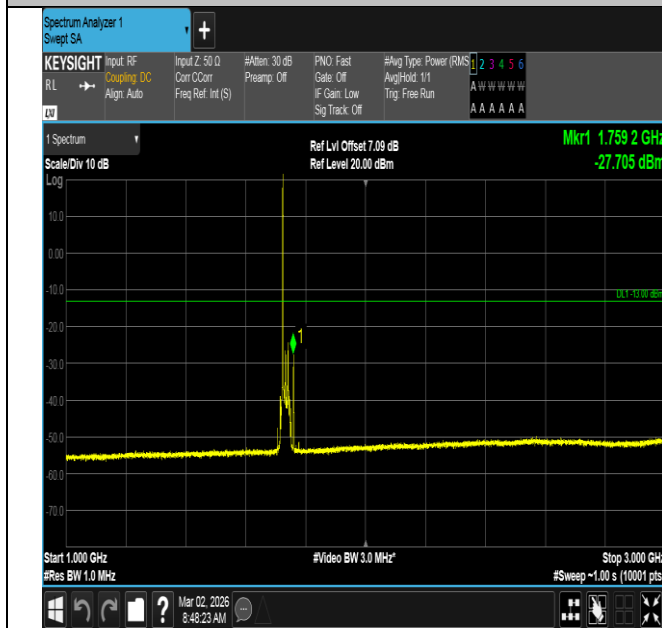
Band4-20MHz-16QAM-20175-1RB#0-1000~3000-PASS
