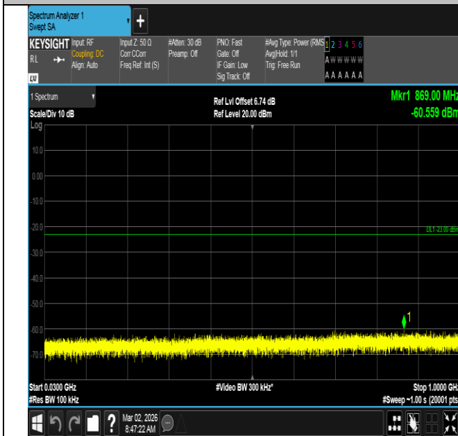
Band4-20MHz-QPSK-20175-1RB#0-30~1000-PASS
