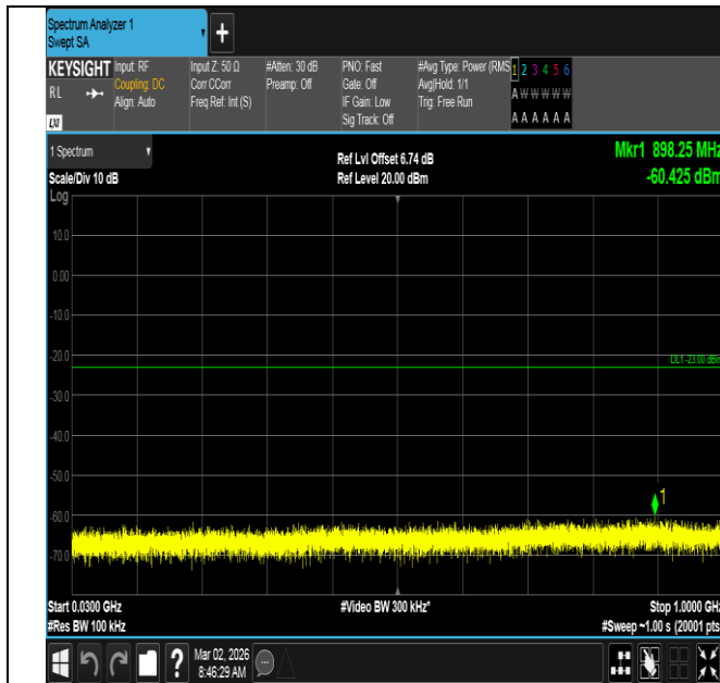
Band4-20MHz-16QAM-20050-1RB#99-30~1000-PASS
