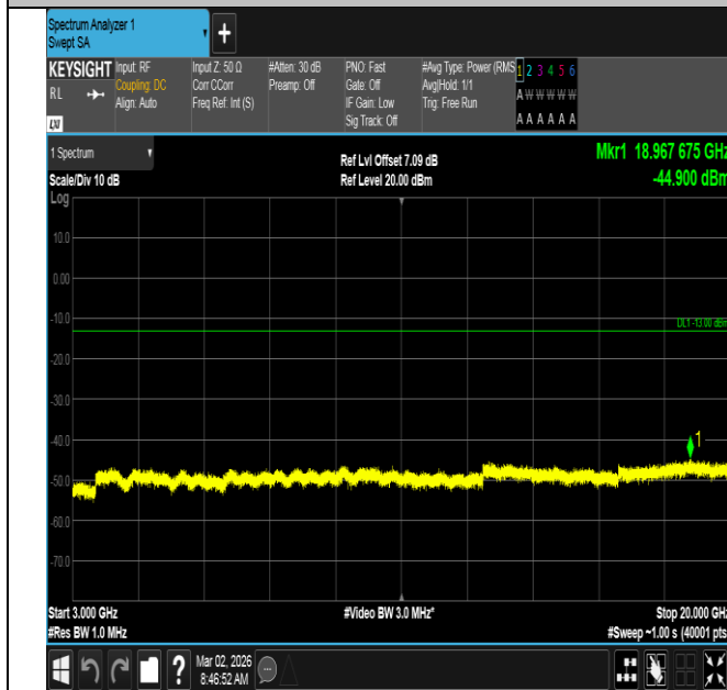
Band4-20MHz-16QAM-20050-1RB#99-3000~20000-PASS
