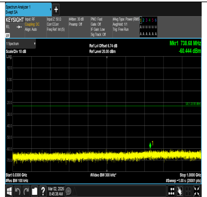
Band4-20MHz-QPSK-20050-1RB#99-30~1000-PASS
