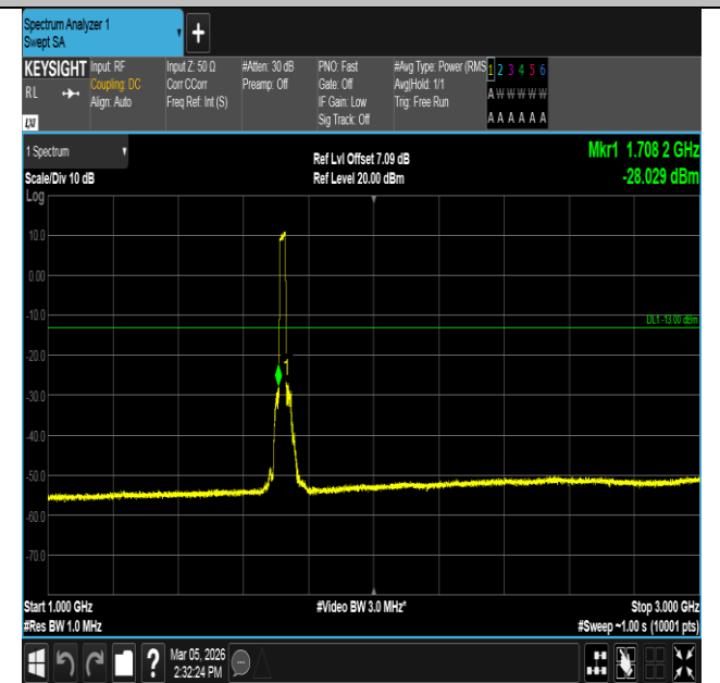
Band4-20MHz-QPSK-20050-100RB#0-1000~3000-PASS
