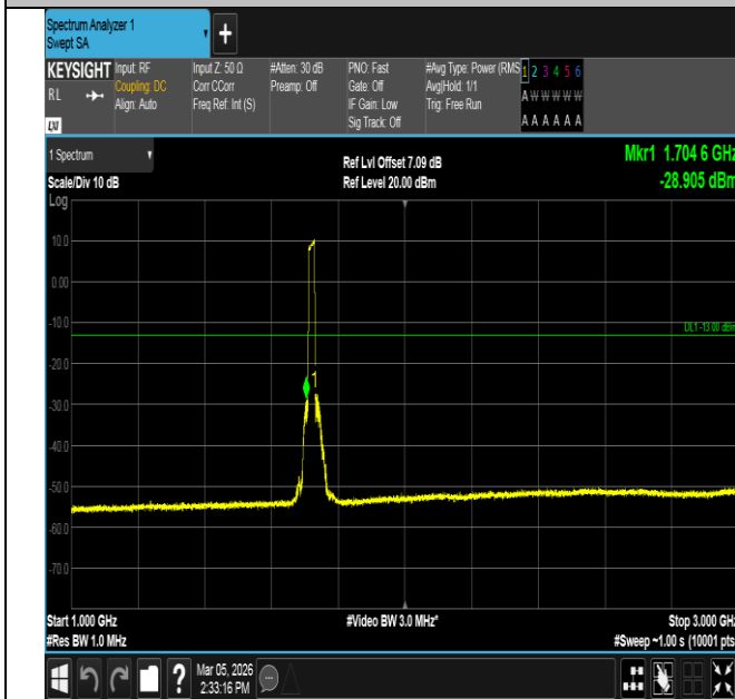
Band4-20MHz-16QAM-20050-100RB#0-1000~3000-PASS
