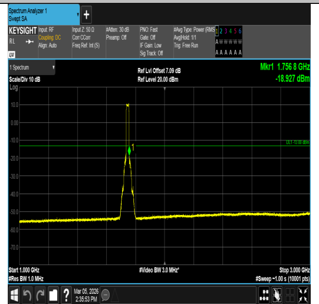
Band4-20MHz-QPSK-20300-100RB#0-1000~3000-PASS
