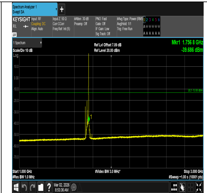
Band4-20MHz-16QAM-20300-1RB#99-1000~3000-PASS
