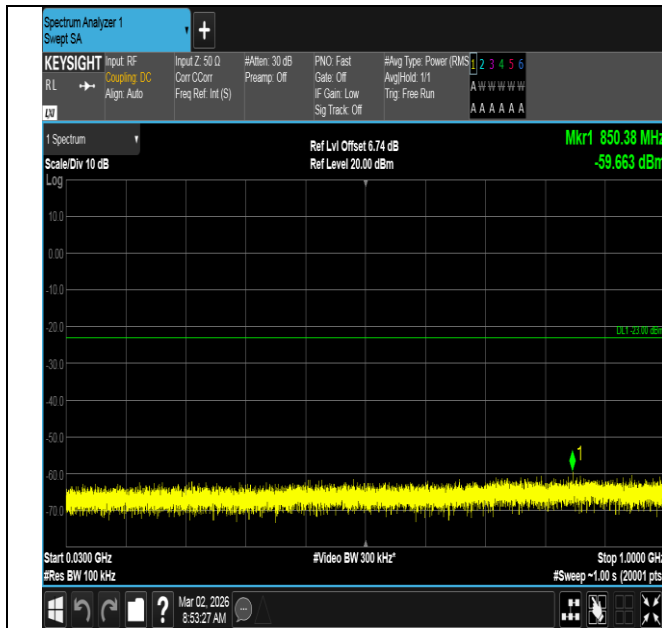
Band4-20MHz-16QAM-20300-1RB#99-30~1000-PASS
