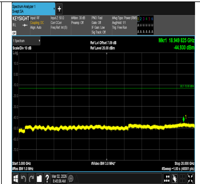
Band4-20MHz-16QAM-20050-1RB#0-3000~20000-PASS
