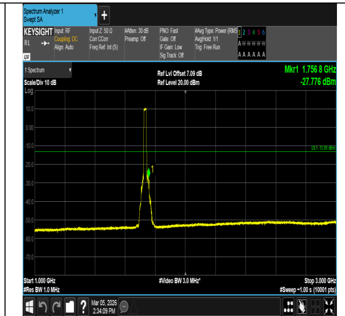
Band4-20MHz-QPSK-20175-100RB#0-1000~3000-PASS
