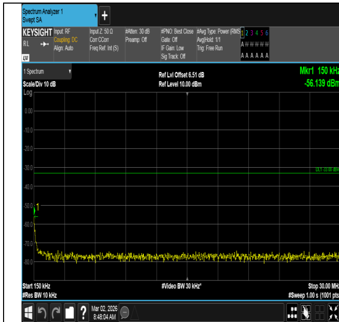
Band4-20MHz-16QAM-20175-1RB#0-0.15~30-PASS
