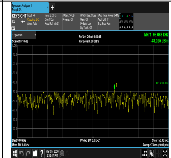
Band4-20MHz-16QAM-20050-100RB#0-0.009~0.15-PASS
