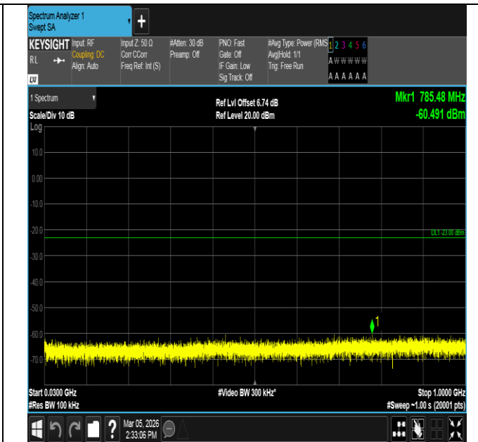
Band4-20MHz-16QAM-20050-100RB#0-30~1000-PASS
