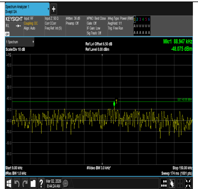
Band4-20MHz-16QAM-20050-1RB#0-0.009~0.15-PASS
