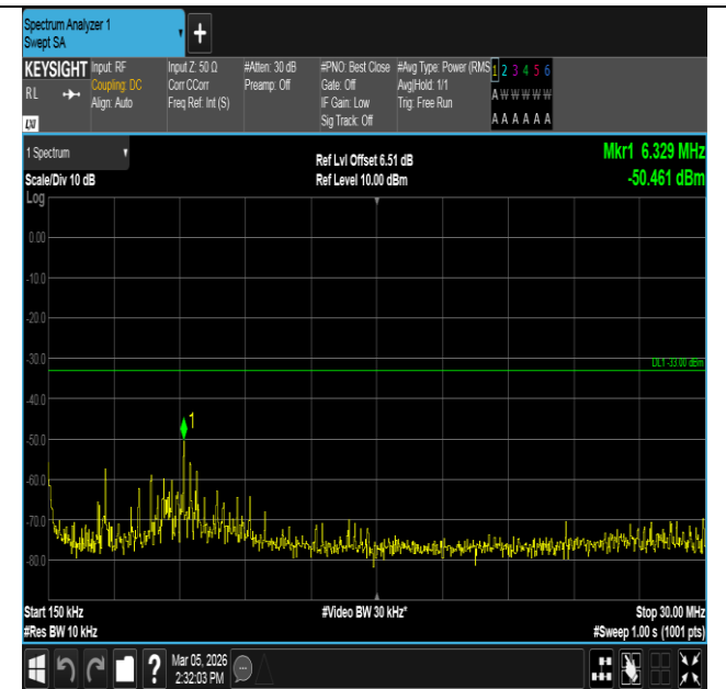
Band4-20MHz-QPSK-20050-100RB#0-0.15~30-PASS
