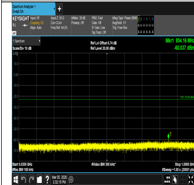
Band4-20MHz-QPSK-20050-100RB#0-30~1000-PASS
