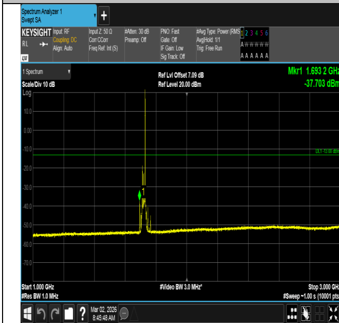
Band4-20MHz-QPSK-20050-1RB#99-1000~3000-PASS
