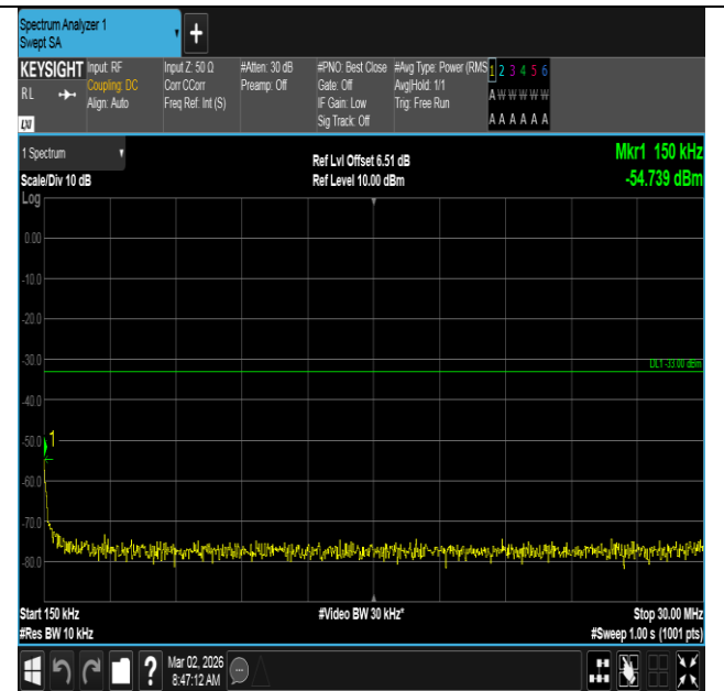
Band4-20MHz-QPSK-20175-1RB#0-0.15~30-PASS
