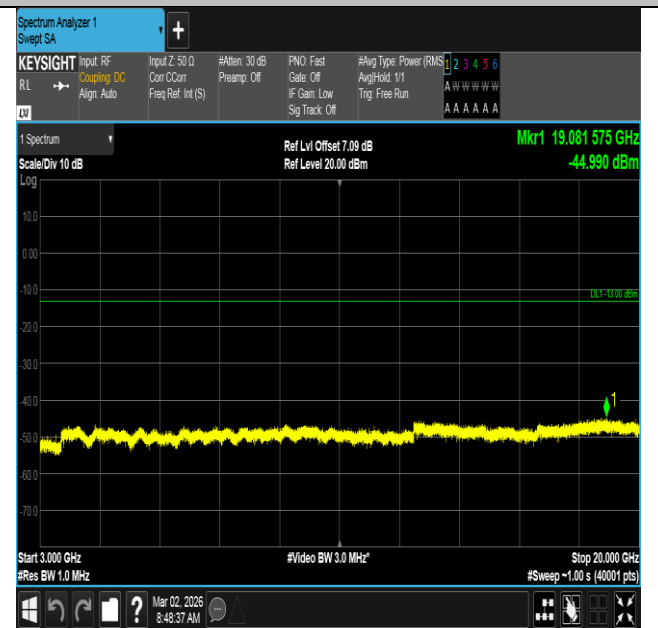
Band4-20MHz-16QAM-20175-1RB#0-3000~20000-PASS
