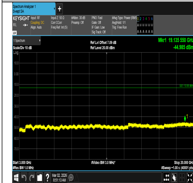
Band4-20MHz-QPSK-20300-1RB#0-3000~20000-PASS
