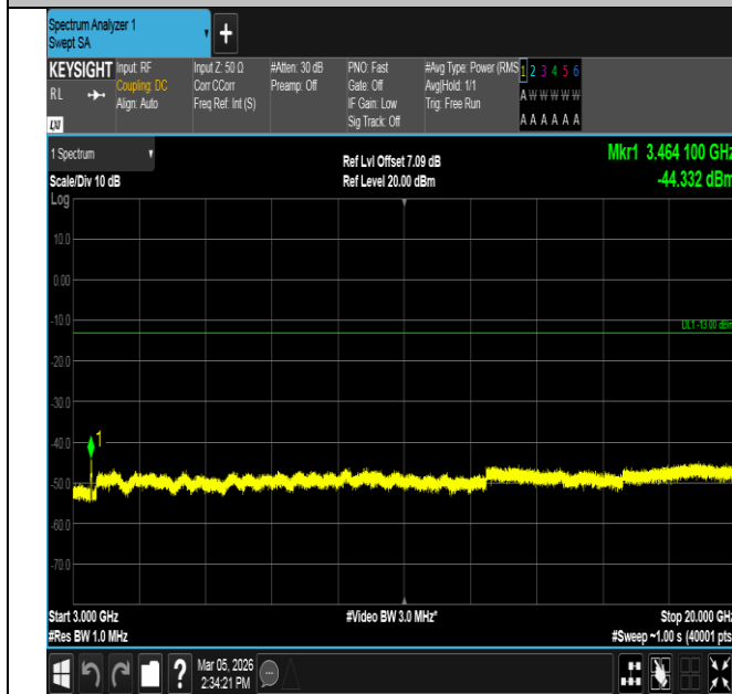
Band4-20MHz-QPSK-20175-100RB#0-3000~20000-PASS
