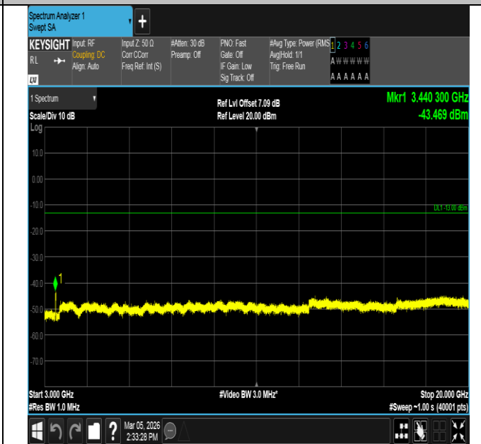
Band4-20MHz-16QAM-20050-100RB#0-3000~20000-PASS
