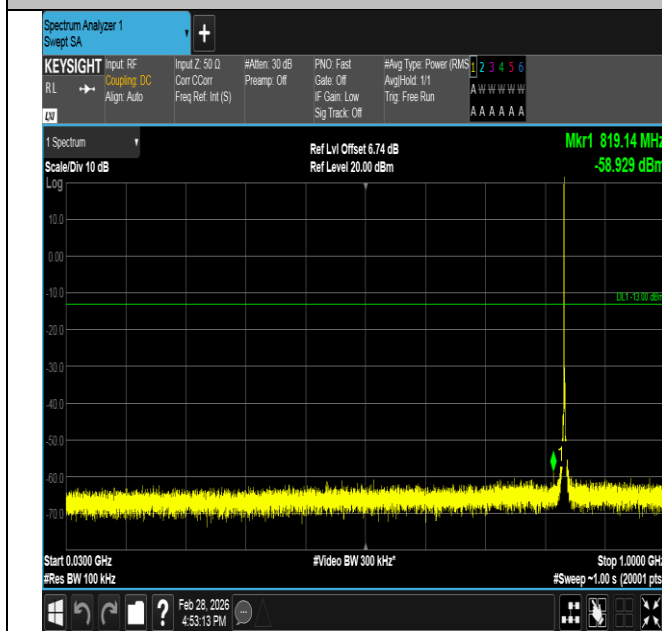
Band5-1.4MHz-QPSK-20525-1RB#0-30~1000-PASS
