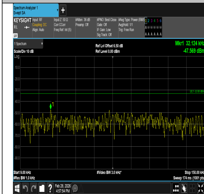
Band5-1.4MHz-QPSK-20643-1RB#0-0.009~0.15-PASS
