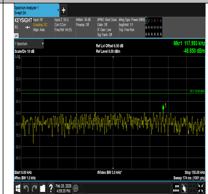
Band5-1.4MHz-QPSK-20643-1RB#5-0.009~0.15-PASS
