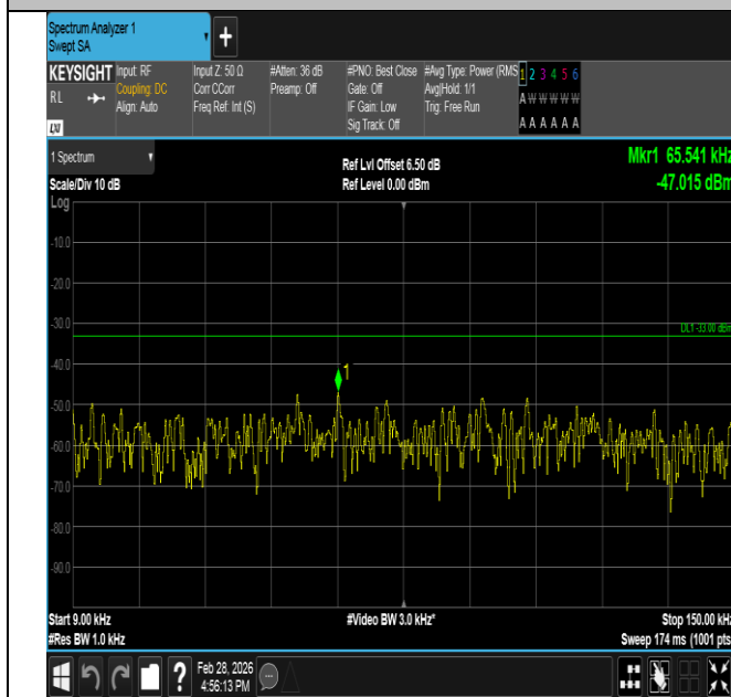
Band5-1.4MHz-QPSK-20525-6RB#0-0.009~0.15-PASS
