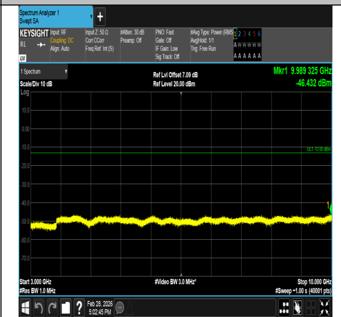
Band5-1.4MHz-16QAM-20643-6RB#0-3000~10000-PASS
