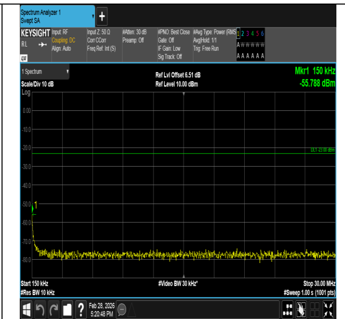
Band5-3MHz-QPSK-20415-1RB#0-0.15~30-PASS
