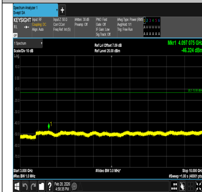
Band5-1.4MHz-QPSK-20643-1RB#0-3000~10000-PASS
