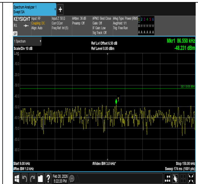
Band5-3MHz-QPSK-20415-1RB#14-0.009~0.15-PASS
