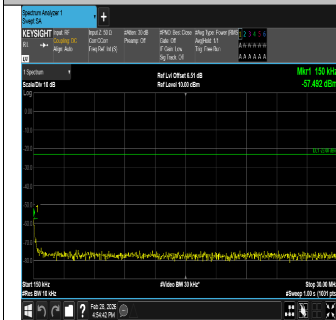
Band5-1.4MHz-QPSK-20525-1RB#5-0.15~30-PASS
