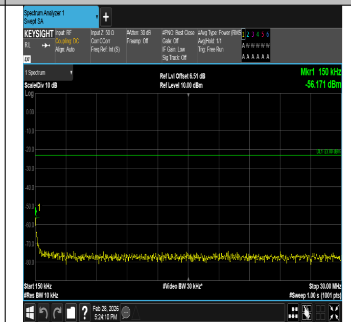
Band5-3MHz-QPSK-20415-15RB#0-0.15~30-PASS
