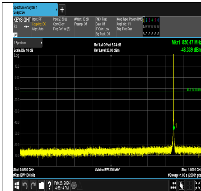
Band5-1.4MHz-QPSK-20643-1RB#0-30~1000-PASS
