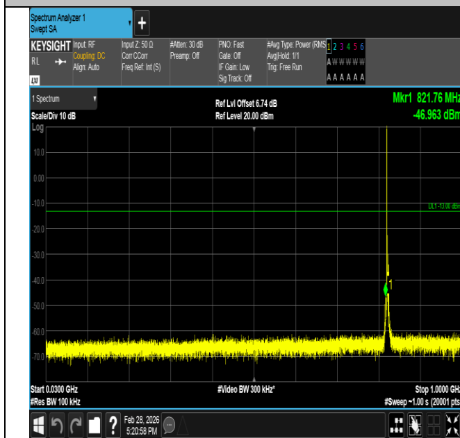
Band5-3MHz-QPSK-20415-1RB#0-30~1000-PASS
