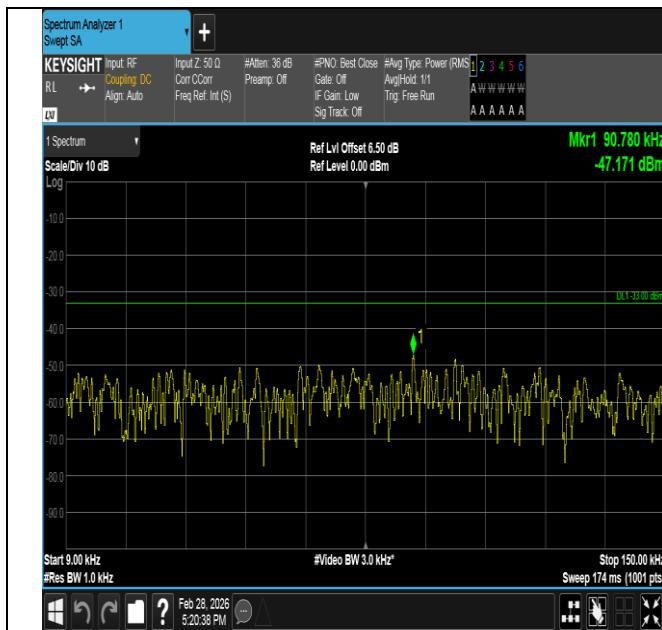
Band5-3MHz-QPSK-20415-1RB#0-0.009~0.15-PASS
