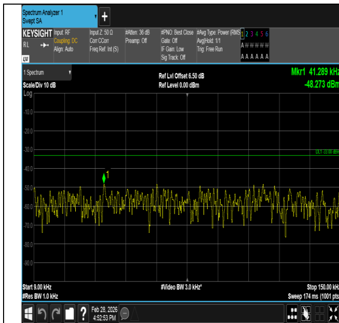
Band5-1.4MHz-QPSK-20525-1RB#0-0.009~0.15-PASS
