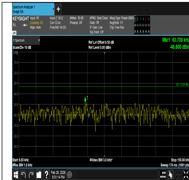
Band5-1.4MHz-QPSK-20643-6RB#0-0.009~0.15-PASS
