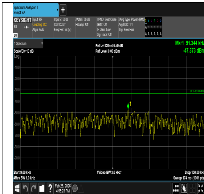
Band5-1.4MHz-16QAM-20525-1RB#5-0.009~0.15-PASS
