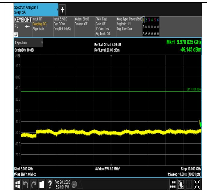
Band5-3MHz-QPSK-20415-1RB#14-3000~10000-PASS
