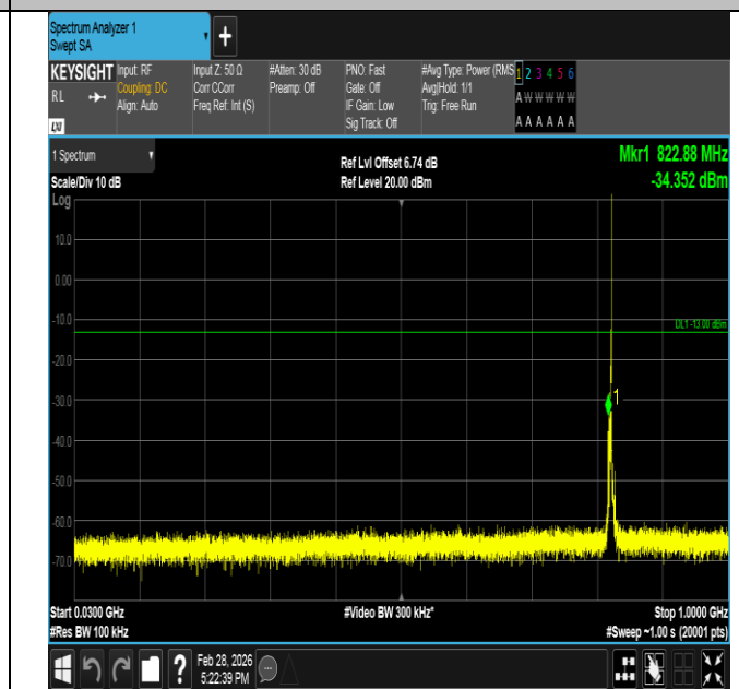
Band5-3MHz-QPSK-20415-1RB#14-30~1000-PASS
