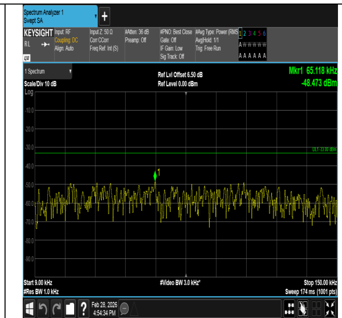
Band5-1.4MHz-QPSK-20525-1RB#5-0.009~0.15-PASS
