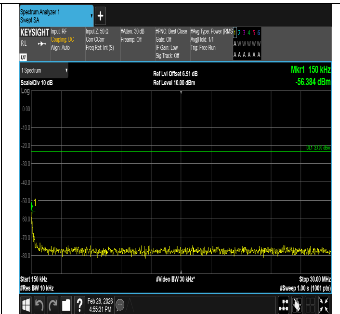
Band5-1.4MHz-16QAM-20525-1RB#5-0.15~30-PASS
