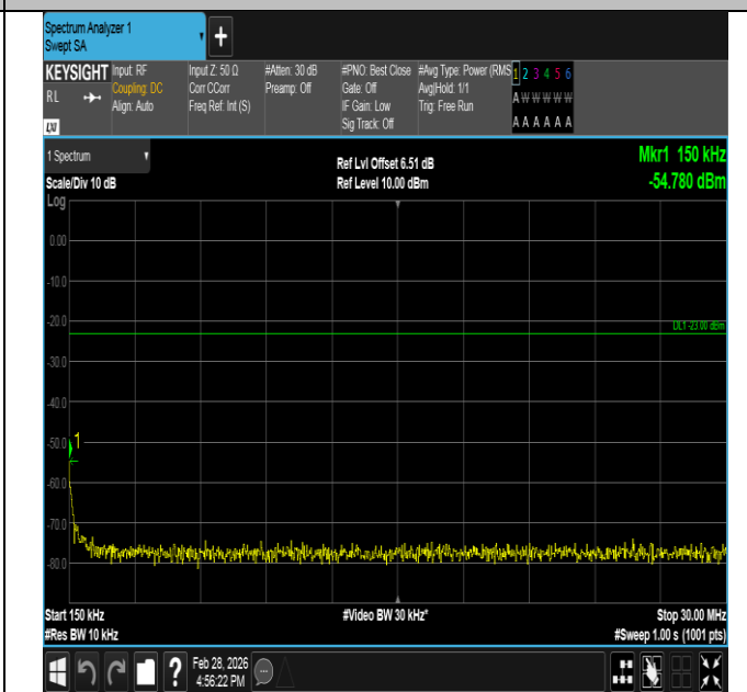
Band5-1.4MHz-QPSK-20525-6RB#0-0.15~30-PASS
