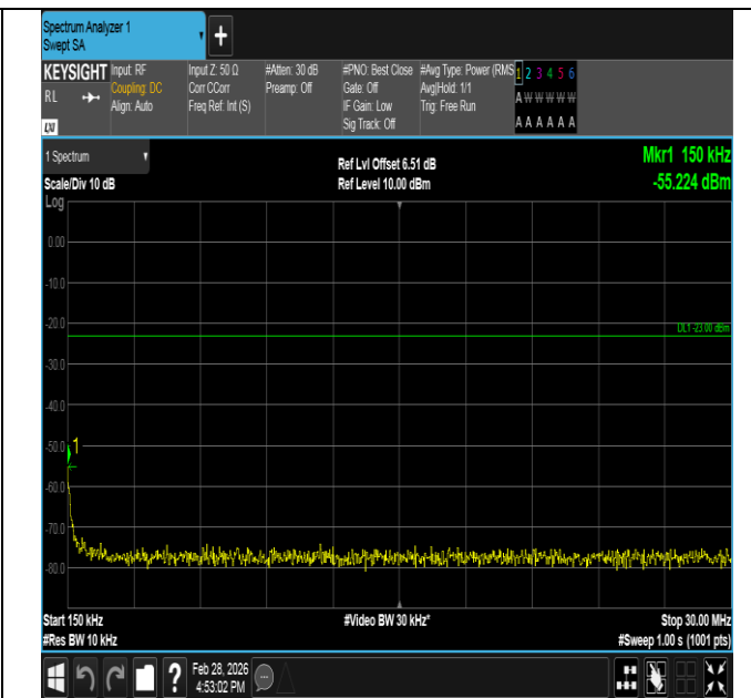
Band5-1.4MHz-QPSK-20525-1RB#0-0.15~30-PASS
