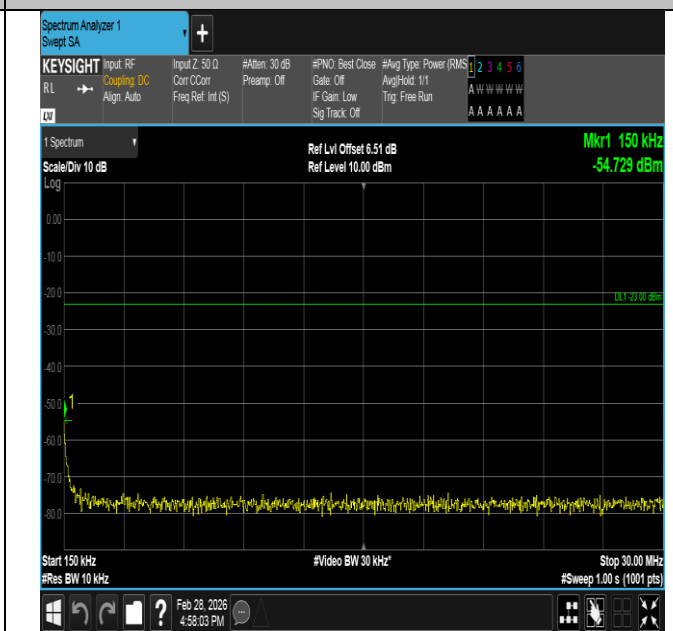
Band5-1.4MHz-QPSK-20643-1RB#0-0.15~30-PASS
