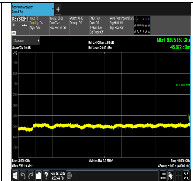
Band5-1.4MHz-16QAM-20525-6RB#0-3000~10000-PASS
