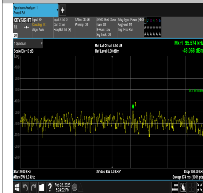
Band5-3MHz-QPSK-20415-15RB#0-0.009~0.15-PASS
