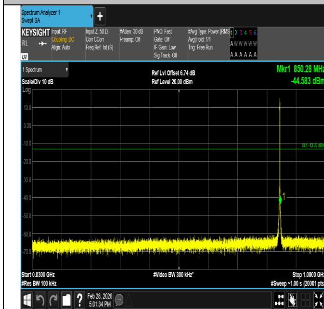
Band5-1.4MHz-QPSK-20643-6RB#0-30~1000-PASS
