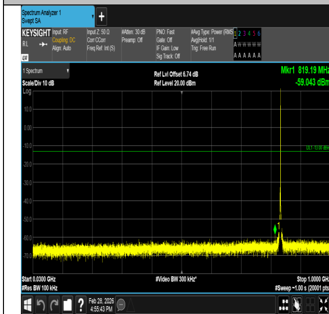
Band5-1.4MHz-16QAM-20525-1RB#5-30~1000-PASS
