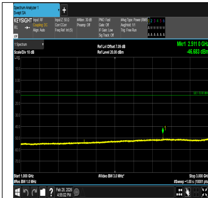
Band5-1.4MHz-QPSK-20525-1RB#5-1000~3000-PASS
