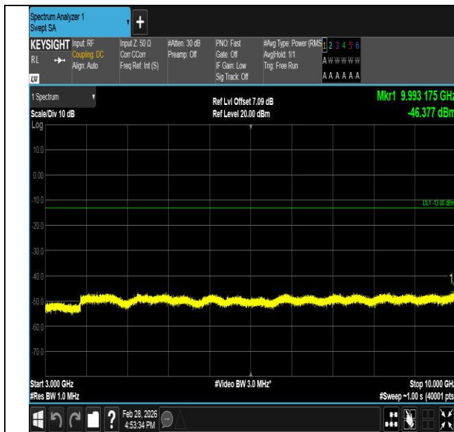
Band5-1.4MHz-QPSK-20525-1RB#0-3000~10000-PASS
