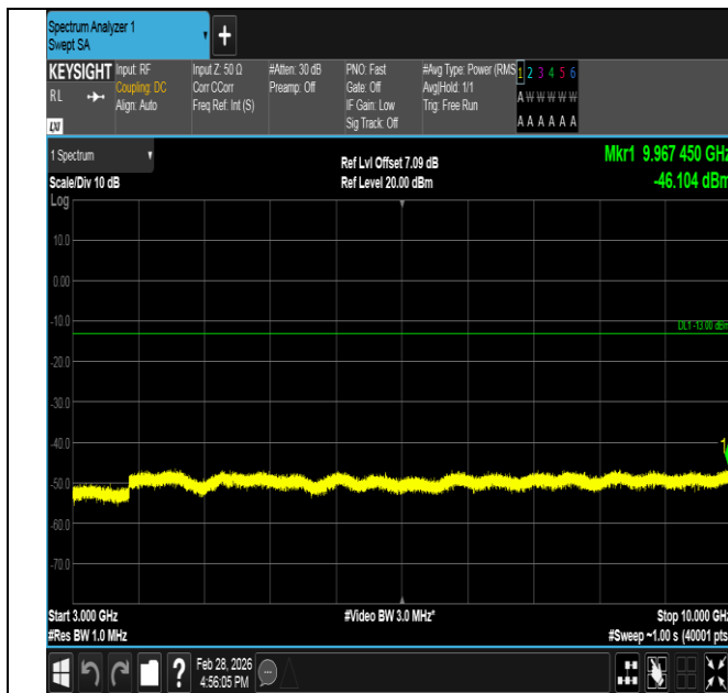
Band5-1.4MHz-16QAM-20525-1RB#5-3000~10000-PASS
