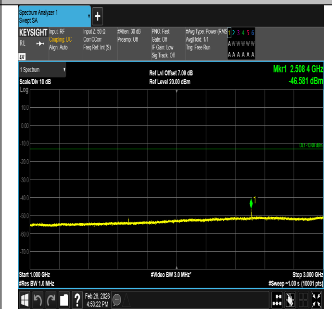
Band5-1.4MHz-QPSK-20525-1RB#0-1000~3000-PASS
