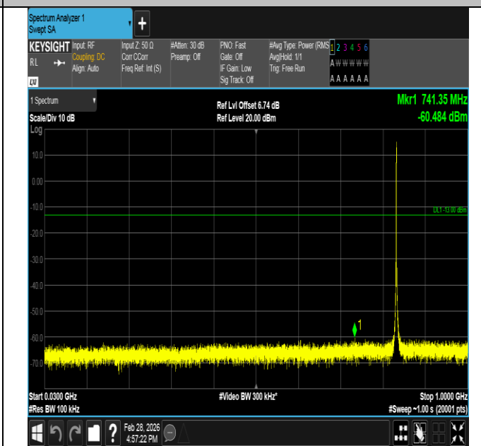
Band5-1.4MHz-16QAM-20525-6RB#0-30~1000-PASS
