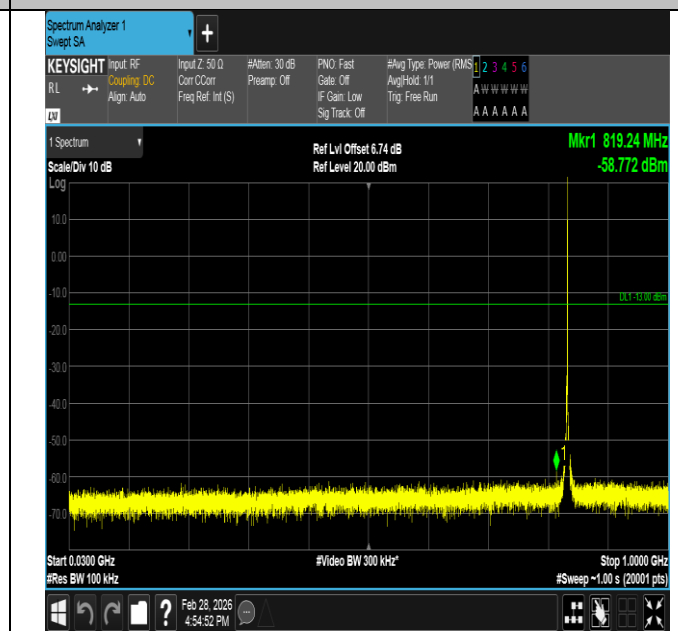
Band5-1.4MHz-QPSK-20525-1RB#5-30~1000-PASS
