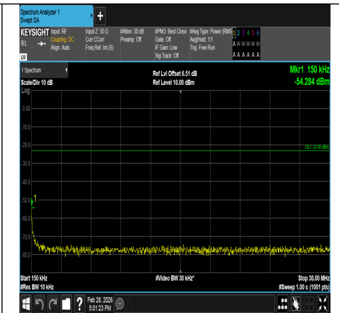
Band5-1.4MHz-QPSK-20643-6RB#0-0.15~30-PASS
