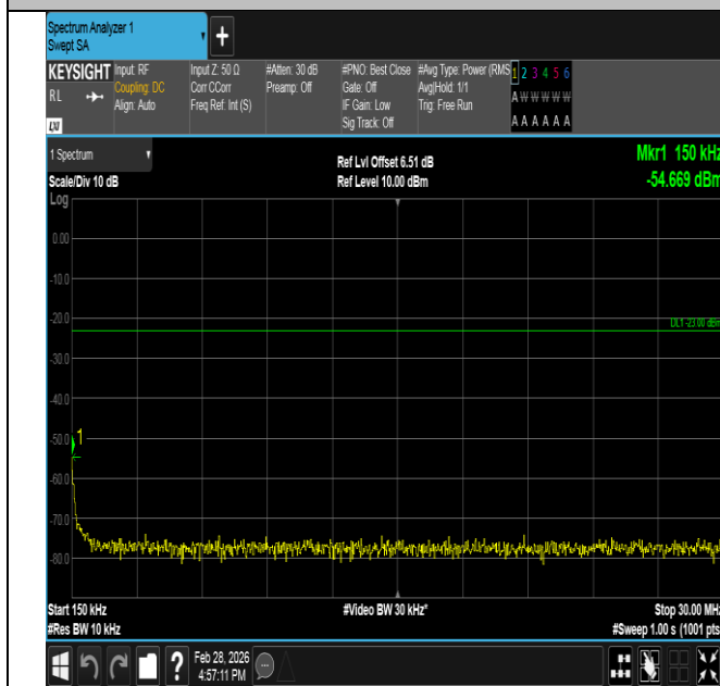
Band5-1.4MHz-16QAM-20525-6RB#0-0.15~30-PASS
