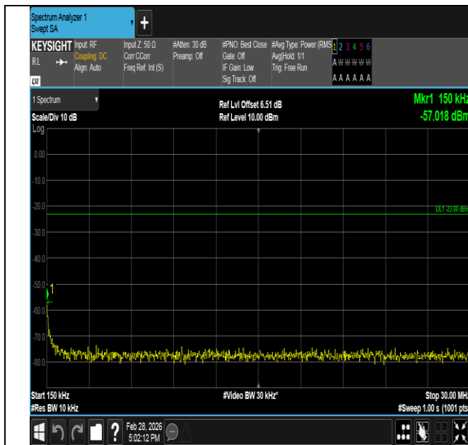
Band5-1.4MHz-16QAM-20643-6RB#0-0.15~30-PASS
