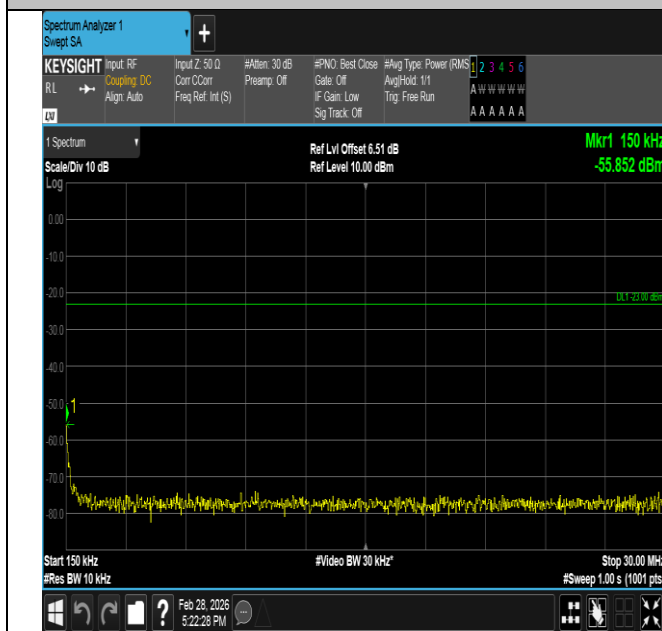
Band5-3MHz-QPSK-20415-1RB#14-0.15~30-PASS
