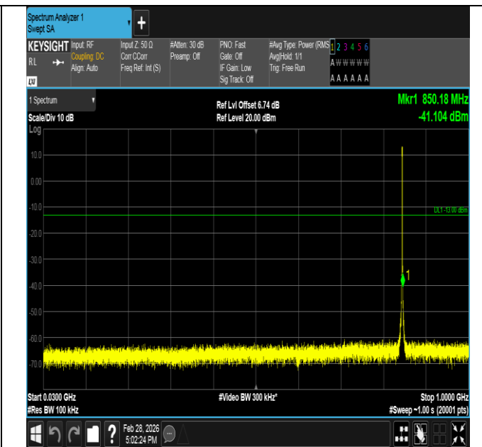
Band5-1.4MHz-16QAM-20643-6RB#0-30~1000-PASS
