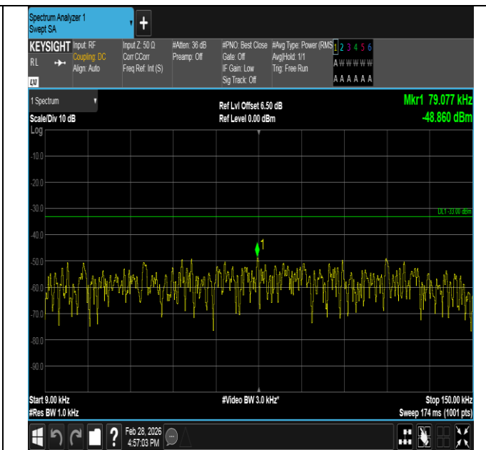
Band5-1.4MHz-16QAM-20525-6RB#0-0.009~0.15-PASS
