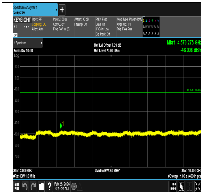
Band5-3MHz-QPSK-20415-1RB#0-3000~10000-PASS
