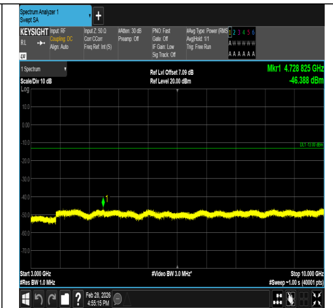
Band5-1.4MHz-QPSK-20525-1RB#5-3000~10000-PASS
