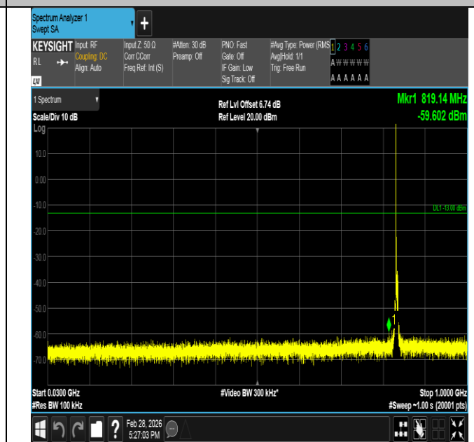
Band5-3MHz-16QAM-20525-1RB#0-30~1000-PASS
