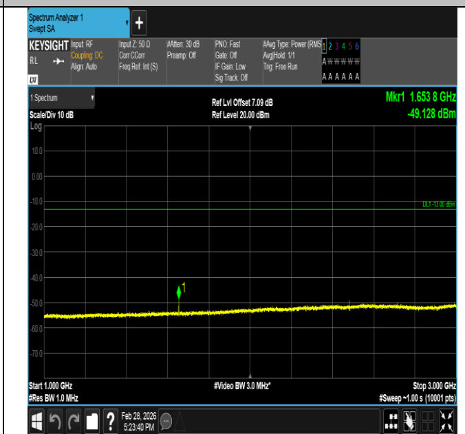
Band5-3MHz-16QAM-20415-1RB#14-1000~3000-PASS
