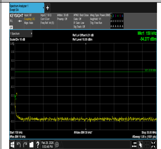
Band5-5MHz-QPSK-20425-1RB#0-0.15~30-PASS
