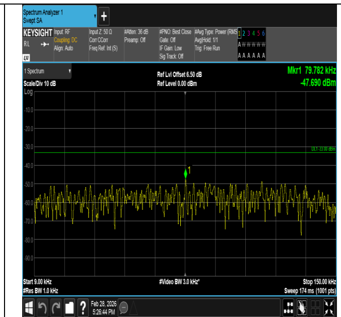
Band5-3MHz-16QAM-20525-1RB#0-0.009~0.15-PASS
