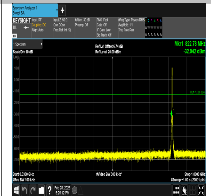
Band5-3MHz-16QAM-20415-15RB#0-30~1000-PASS
