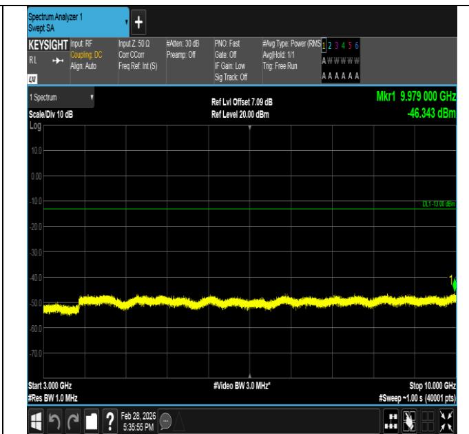
Band5-3MHz-16QAM-20635-15RB#0-3000~10000-PASS
