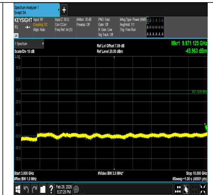
Band5-3MHz-16QAM-20525-1RB#0-3000~10000-PASS
