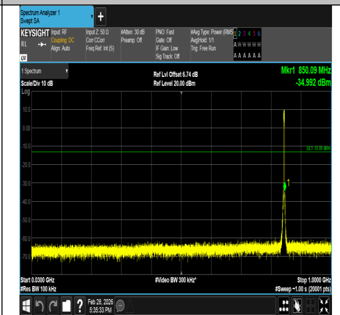
Band5-3MHz-16QAM-20635-15RB#0-30~1000-PASS
