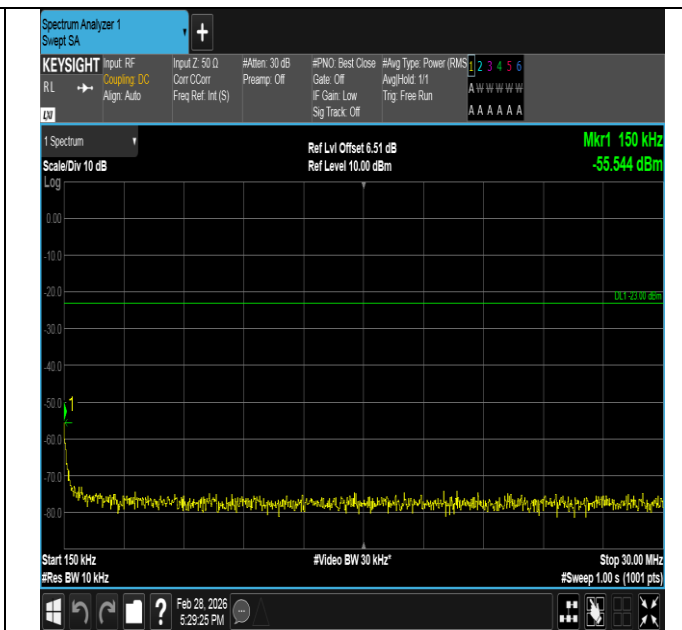
Band5-3MHz-QPSK-20525-15RB#0-0.15~30-PASS
