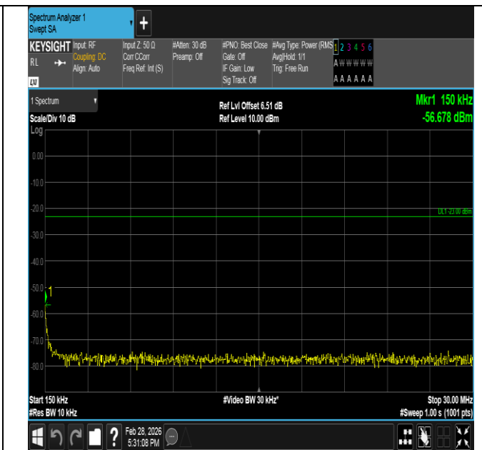
Band5-3MHz-QPSK-20635-1RB#0-0.15~30-PASS
