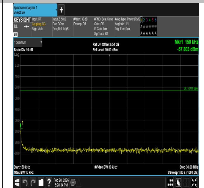
Band5-3MHz-16QAM-20525-1RB#14-0.15~30-PASS
