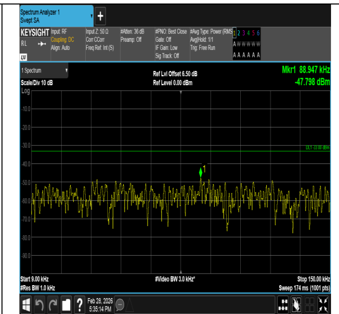
Band5-3MHz-16QAM-20635-15RB#0-0.009~0.15-PASS
