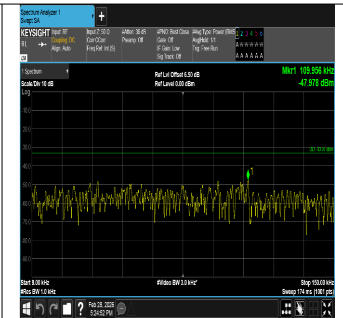
Band5-3MHz-16QAM-20415-15RB#0-0.009~0.15-PASS
