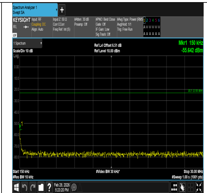
Band5-3MHz-16QAM-20415-1RB#14-0.15~30-PASS
