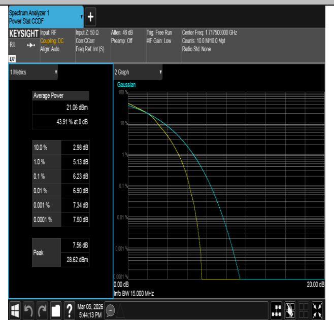
Band66-15MHz-16QAM-132047-75RB#0-PASS
