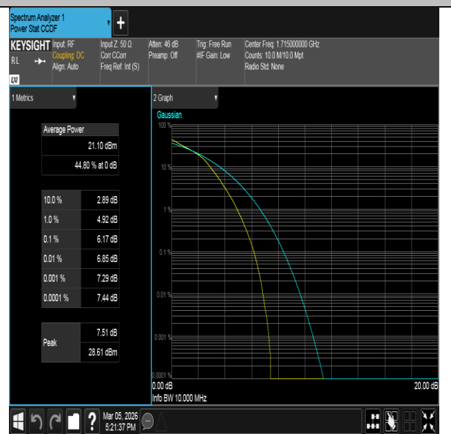
Band66-10MHz-16QAM-132022-50RB#0-PASS
