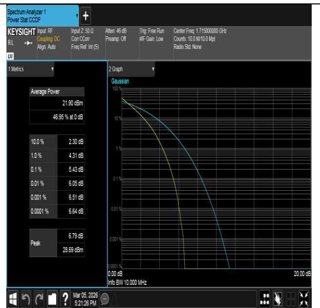
Band66-10MHz-QPSK-132022-50RB#0-PASS
