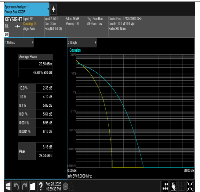
Band66-5MHz-QPSK-131997-25RB#0-PASS
