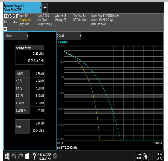
Band66-5MHz-16QAM-131997-25RB#0-PASS
