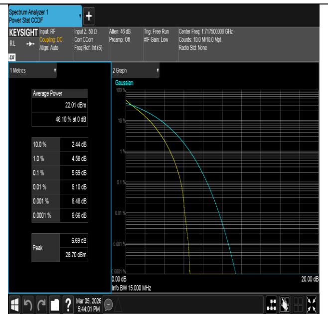
Band66-15MHz-QPSK-132047-75RB#0-PASS
