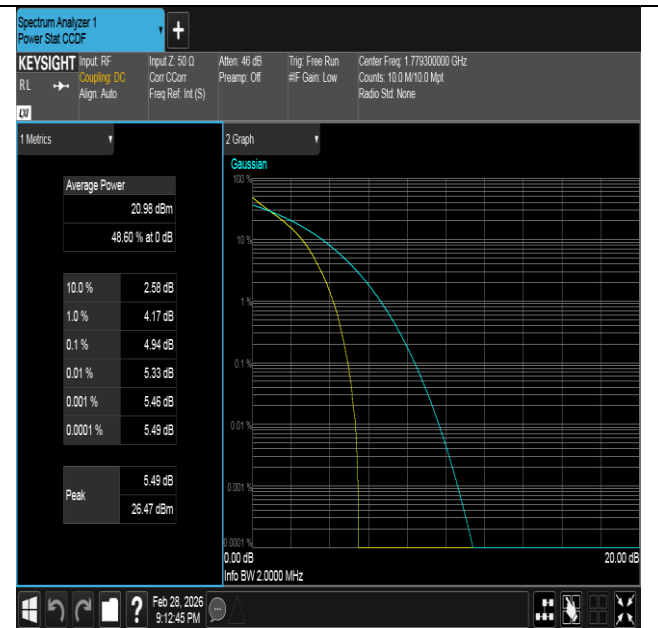
Band66-1.4MHz-QPSK-132665-6RB#0-PASS
