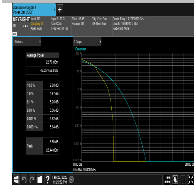
Band66-15MHz-16QAM-132047-1RB#0-PASS
