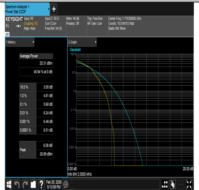
Band66-1.4MHz-16QAM-132665-6RB#0-PASS
