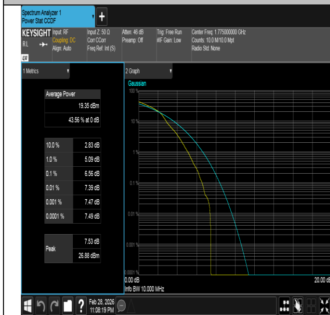
Band66-10MHz-16QAM-132622-1RB#0-PASS
