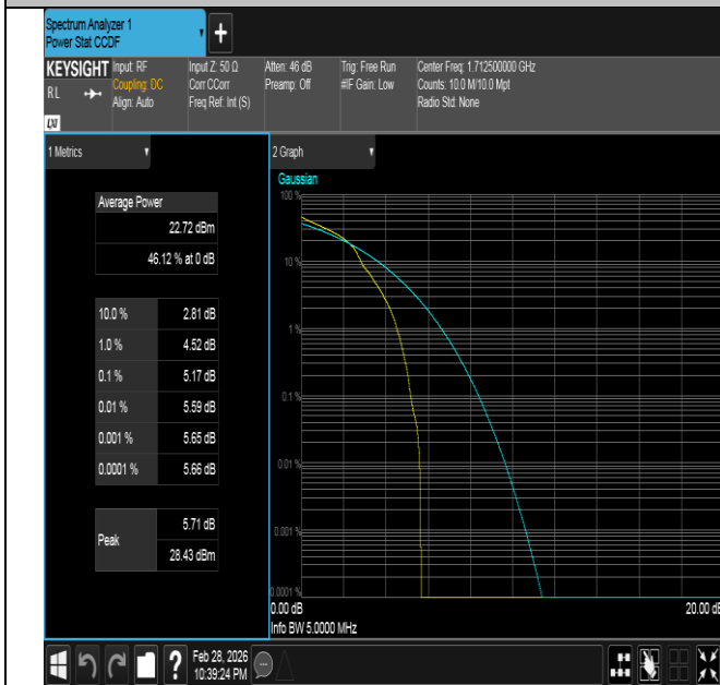
Band66-5MHz-16QAM-131997-1RB#0-PASS
