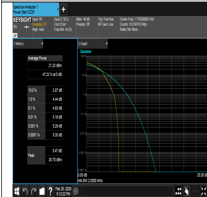
Band66-1.4MHz-16QAM-132665-1RB#0-PASS
