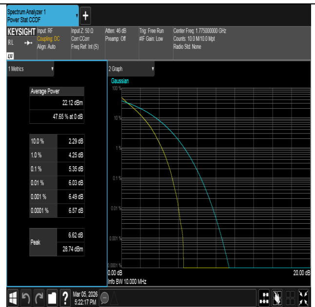
Band66-10MHz-QPSK-132622-50RB#0-PASS
