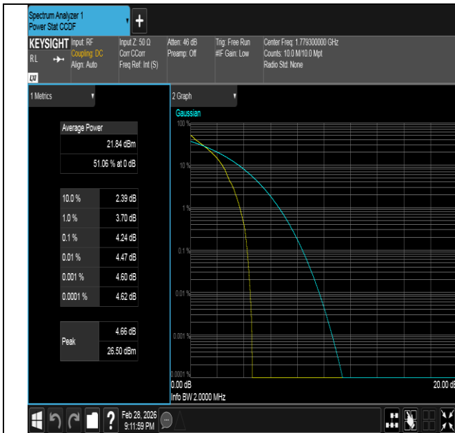
Band66-1.4MHz-QPSK-132665-1RB#0-PASS
