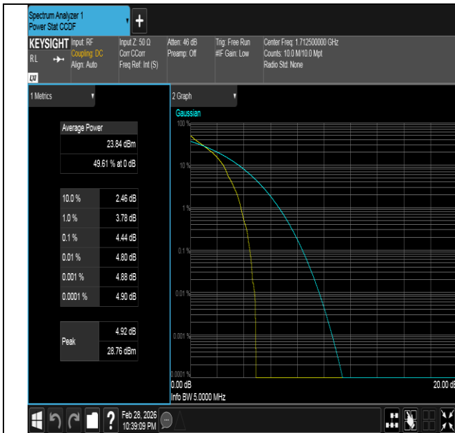
Band66-5MHz-QPSK-131997-1RB#0-PASS
