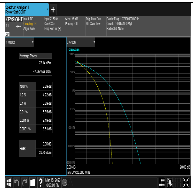
Band66-20MHz-QPSK-132572-100RB#0-PASS
