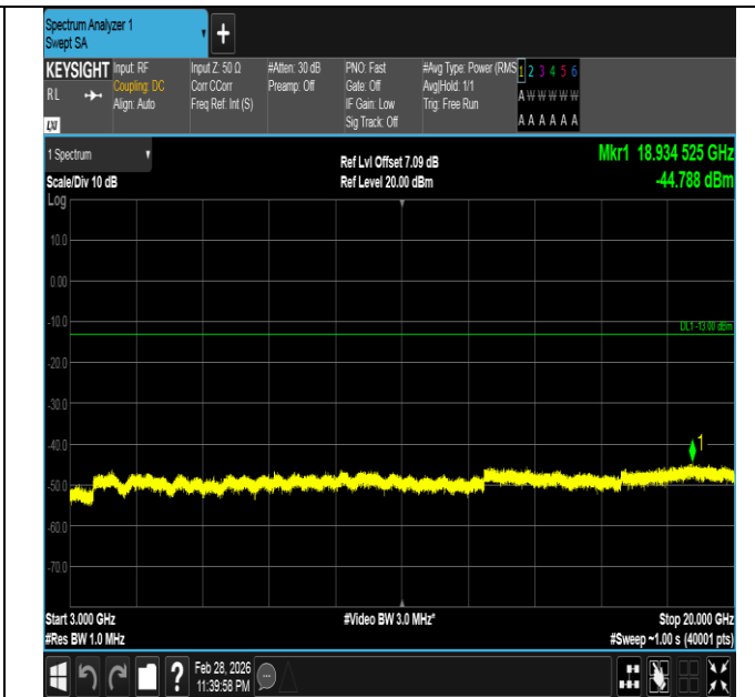
Band66-20MHz-QPSK-132322-1RB#99-3000~20000-PASS
