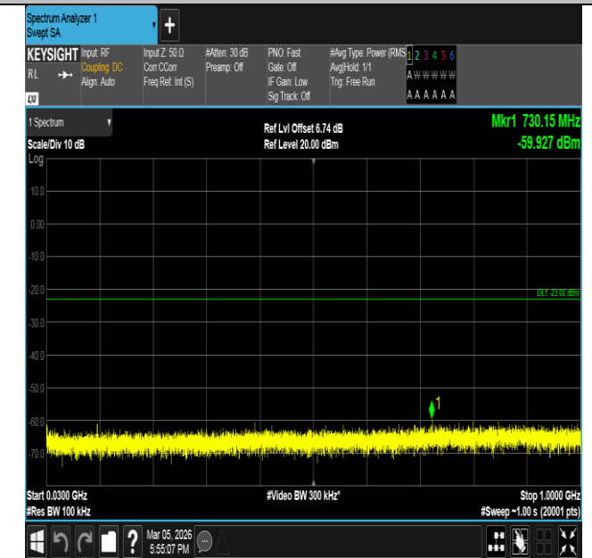
Band66-20MHz-16QAM-132322-100RB#0-30~1000-PASS
