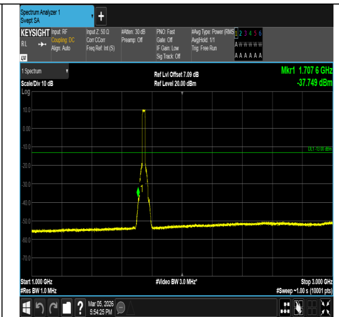
Band66-20MHz-QPSK-132322-100RB#0-1000~3000-PASS
