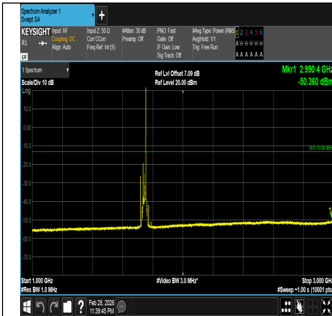
Band66-20MHz-QPSK-132322-1RB#99-1000~3000-PASS
