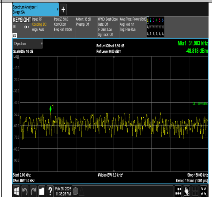
Band66-20MHz-16QAM-132322-1RB#0-0.009~0.15-PASS
