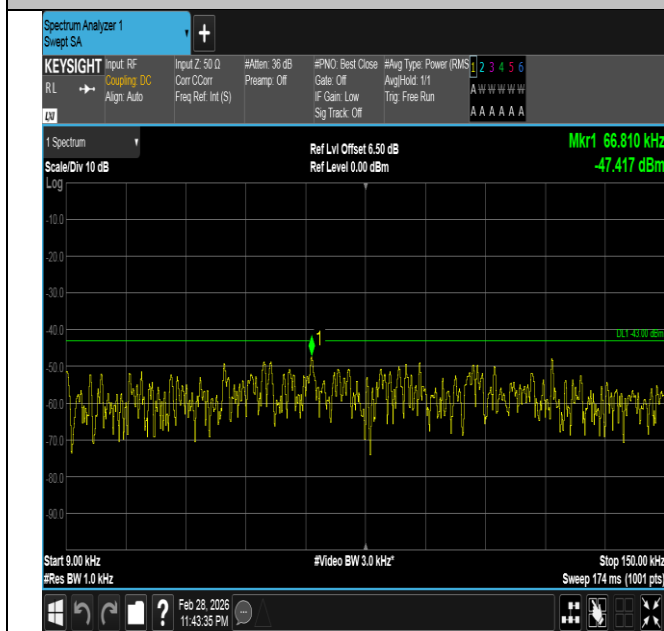
Band66-20MHz-16QAM-132572-1RB#99-0.009~0.15-PASS
