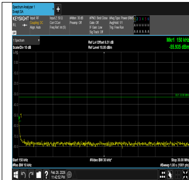
Band66-20MHz-QPSK-132572-1RB#99-0.15~30-PASS
