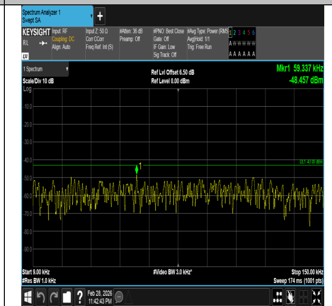
Band66-20MHz-QPSK-132572-1RB#99-0.009~0.15-PASS
