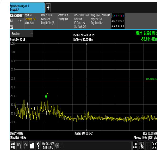
Band66-20MHz-16QAM-132572-100RB#0-0.15~30-PASS
