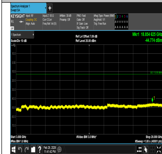
Band66-20MHz-QPSK-132572-1RB#0-3000~20000-PASS
