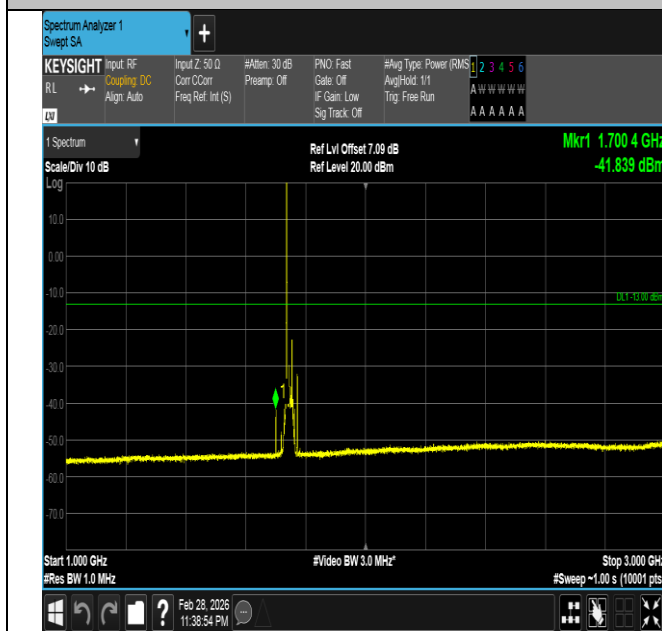
Band66-20MHz-16QAM-132322-1RB#0-1000~3000-PASS
