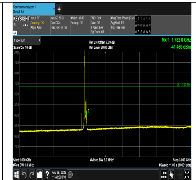
Band66-20MHz-QPSK-132572-1RB#0-1000~3000-PASS
