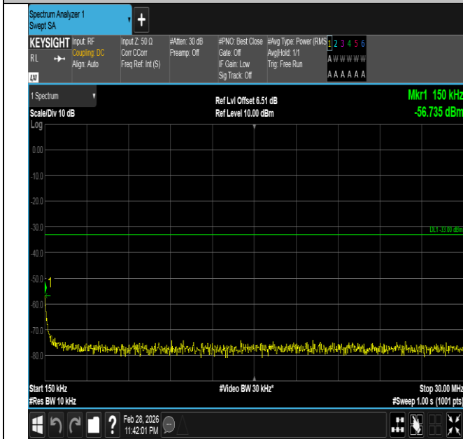
Band66-20MHz-16QAM-132572-1RB#0-0.15~30-PASS
