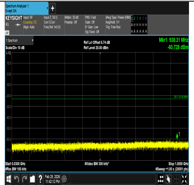
Band66-20MHz-16QAM-132572-1RB#0-30~1000-PASS
