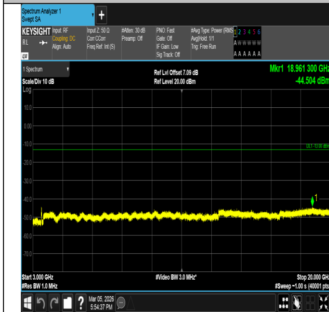
Band66-20MHz-QPSK-132322-100RB#0-3000~20000-PASS
