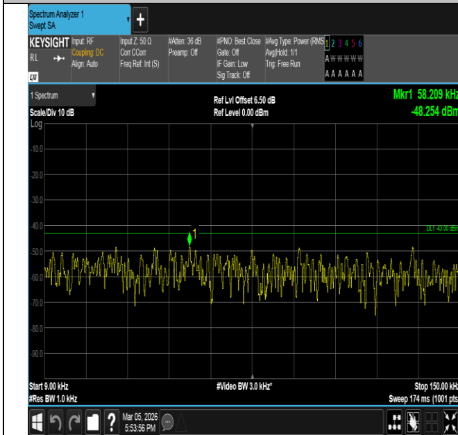
Band66-20MHz-QPSK-132322-100RB#0-0.009~0.15-PASS
