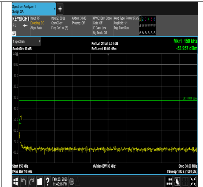
Band66-20MHz-16QAM-132322-1RB#99-0.15~30-PASS
