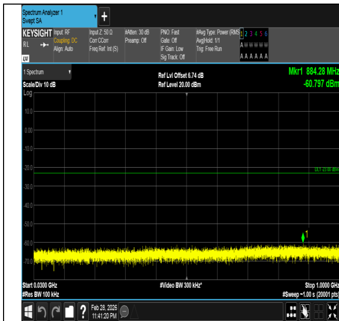
Band66-20MHz-QPSK-132572-1RB#0-30~1000-PASS
