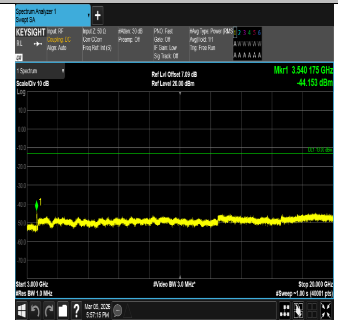
Band66-20MHz-16QAM-132572-100RB#0-3000~20000-PASS
