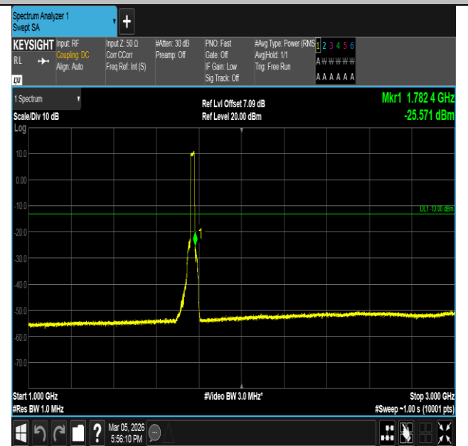
Band66-20MHz-QPSK-132572-100RB#0-1000~3000-PASS
