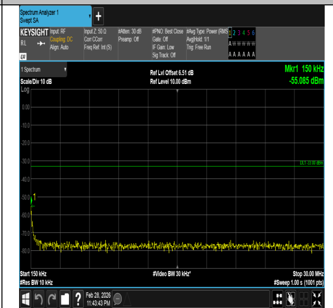
Band66-20MHz-16QAM-132572-1RB#99-0.15~30-PASS
