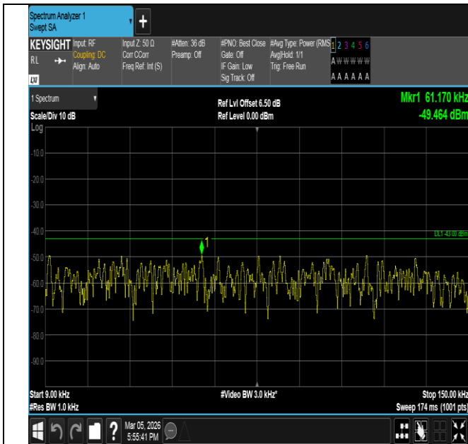
Band66-20MHz-QPSK-132572-100RB#0-0.009~0.15-PASS
