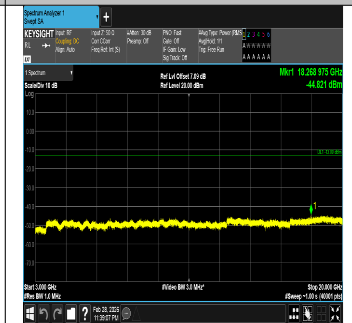
Band66-20MHz-16QAM-132322-1RB#0-3000~20000-PASS
