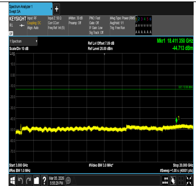
Band66-20MHz-16QAM-132322-100RB#0-3000~20000-PASS
