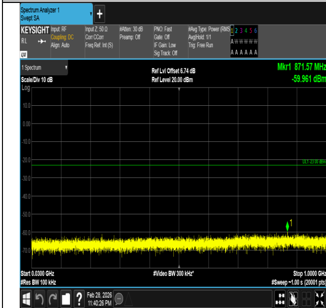
Band66-20MHz-16QAM-132322-1RB#99-30~1000-PASS
