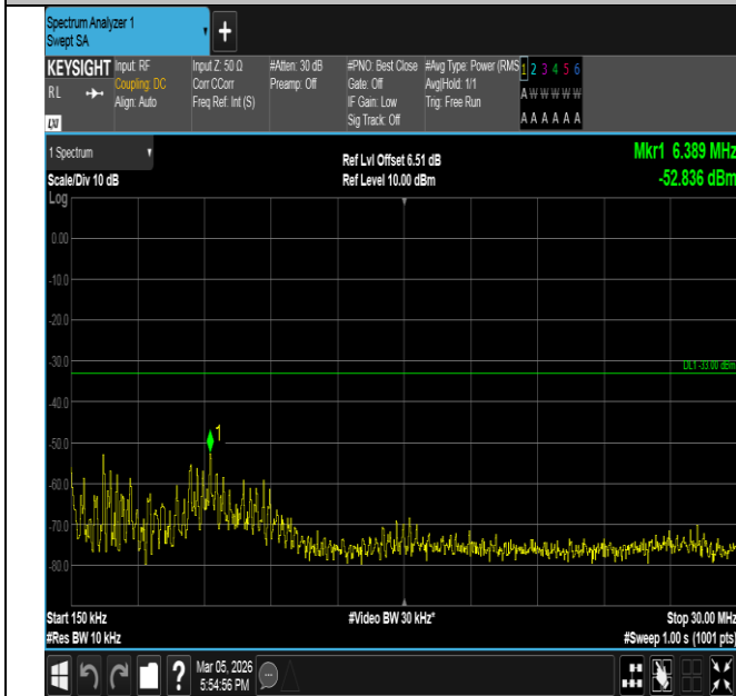
Band66-20MHz-16QAM-132322-100RB#0-0.15~30-PASS
