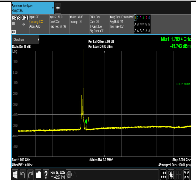
Band66-20MHz-16QAM-132322-1RB#99-1000~3000-PASS
