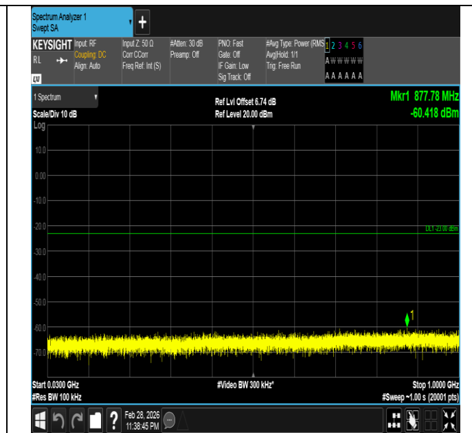
Band66-20MHz-16QAM-132322-1RB#0-30~1000-PASS
