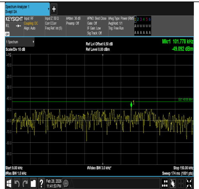
Band66-20MHz-16QAM-132572-1RB#0-0.009~0.15-PASS
