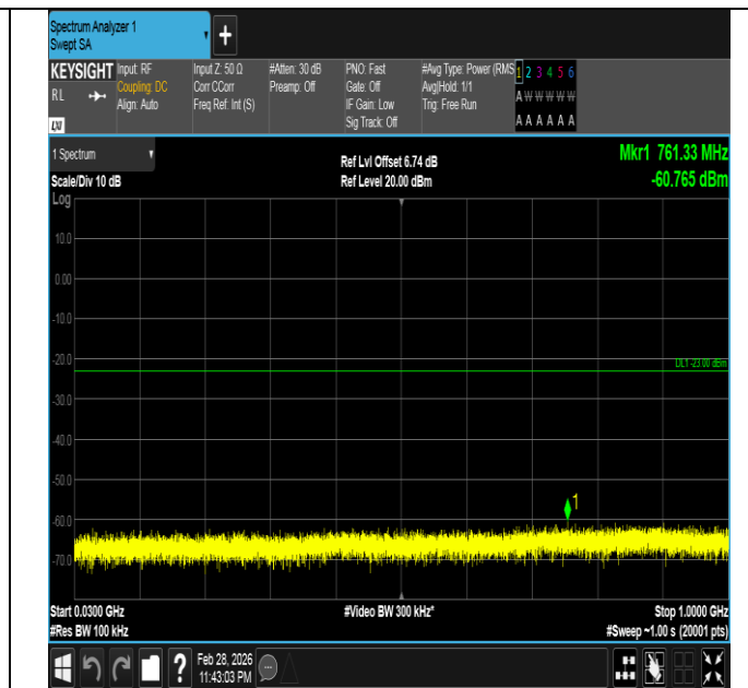
Band66-20MHz-QPSK-132572-1RB#99-30~1000-PASS
