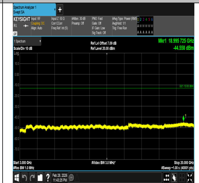
Band66-20MHz-QPSK-132572-1RB#99-3000~20000-PASS
