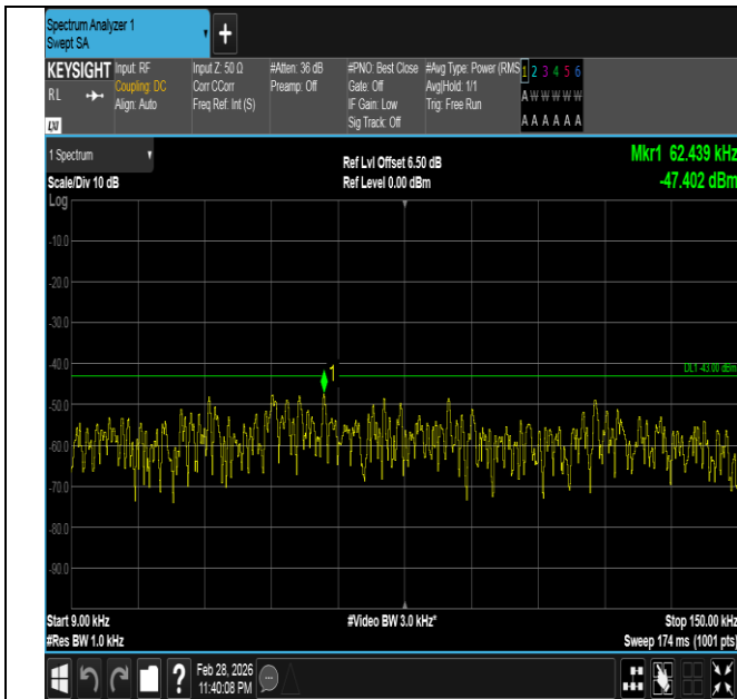
Band66-20MHz-16QAM-132322-1RB#99-0.009~0.15-PASS
