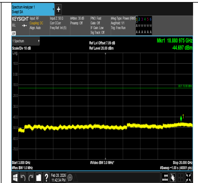
Band66-20MHz-16QAM-132572-1RB#0-3000~20000-PASS
