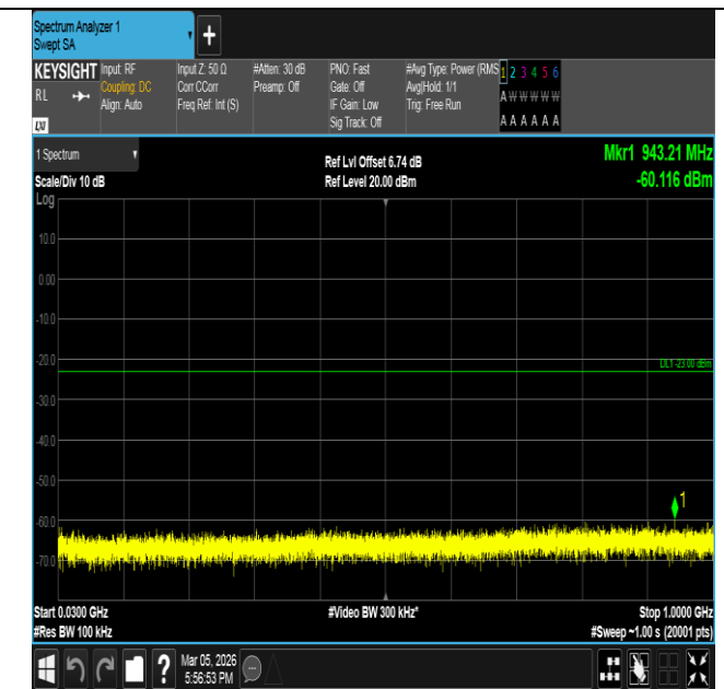
Band66-20MHz-16QAM-132572-100RB#0-30~1000-PASS
