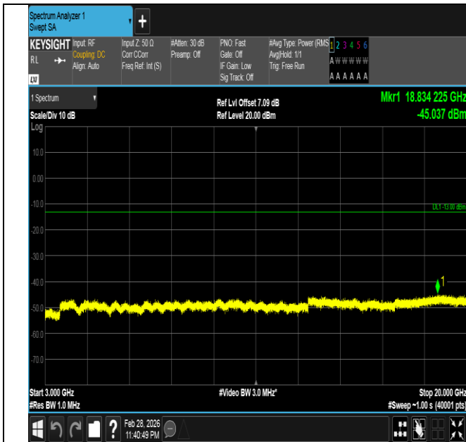
Band66-20MHz-16QAM-132322-1RB#99-3000~20000-PASS
