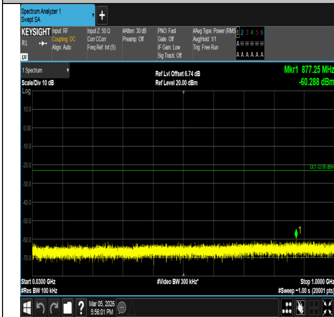
Band66-20MHz-QPSK-132572-100RB#0-30~1000-PASS
