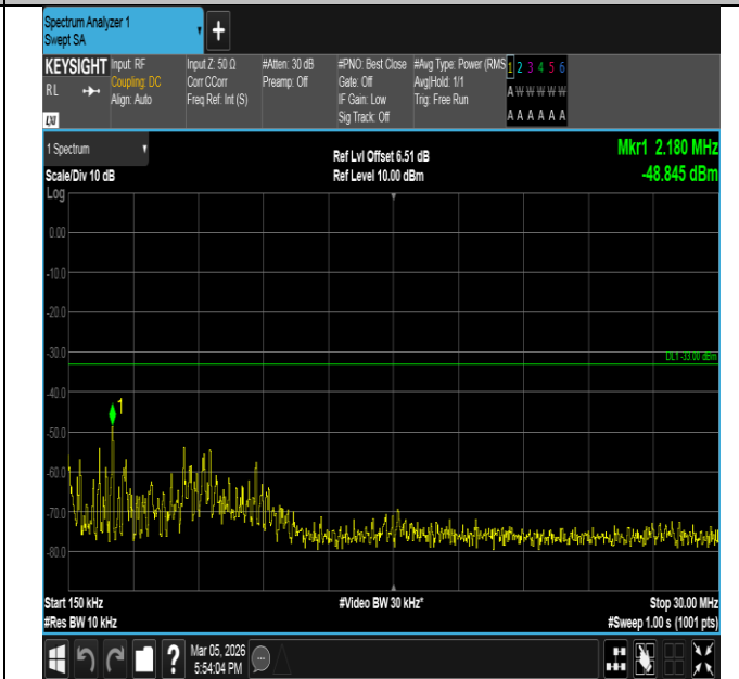
Band66-20MHz-QPSK-132322-100RB#0-0.15~30-PASS
