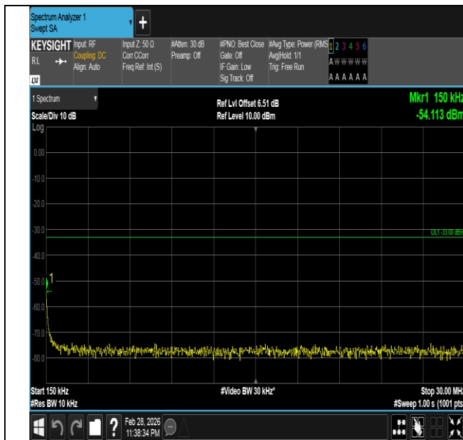
Band66-20MHz-16QAM-132322-1RB#0-0.15~30-PASS
