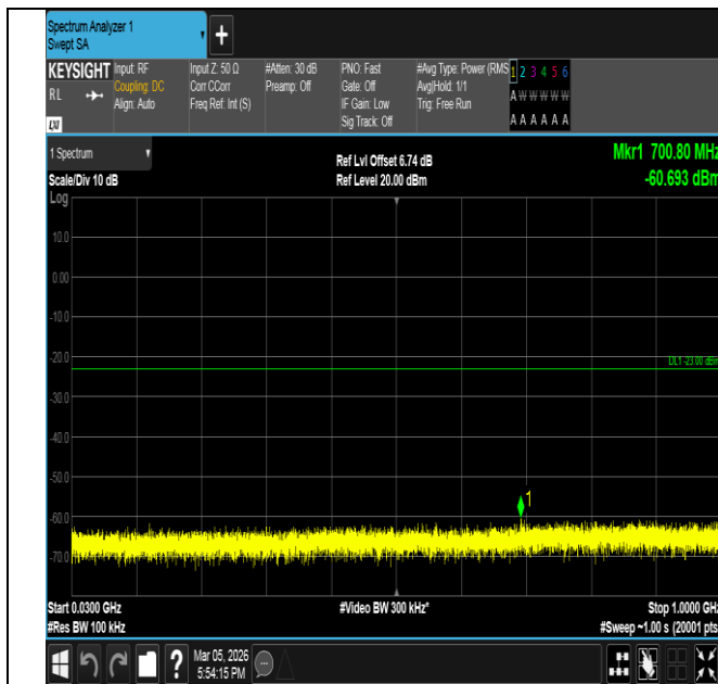
Band66-20MHz-QPSK-132322-100RB#0-30~1000-PASS
