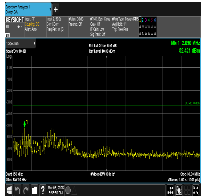
Band66-20MHz-QPSK-132572-100RB#0-0.15~30-PASS
