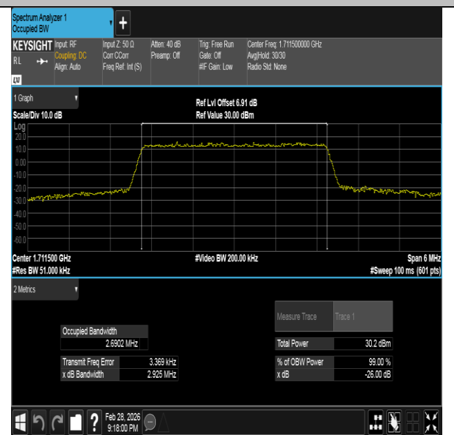
Band66-3MHz-16QAM-131987-15RB#0-PASS
