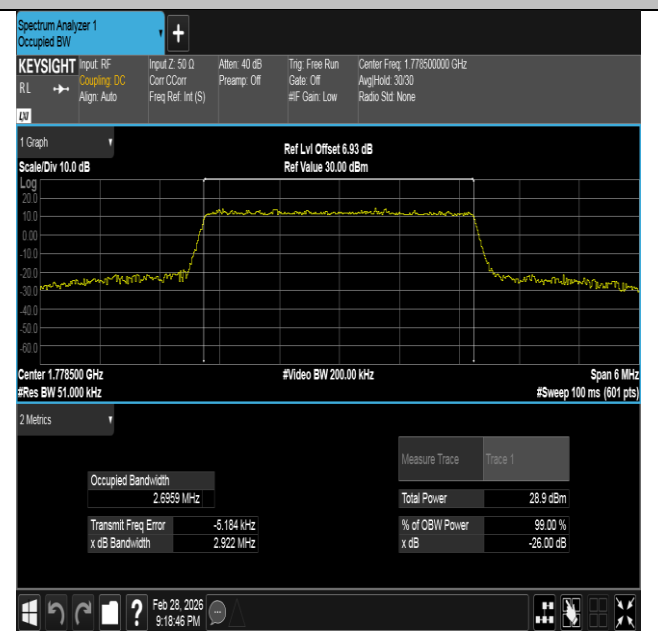
Band66-3MHz-16QAM-132657-15RB#0-PASS
