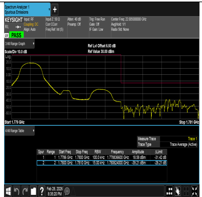
Band66-1.4MHz-16QAM-132665-1RB#0-PASS
