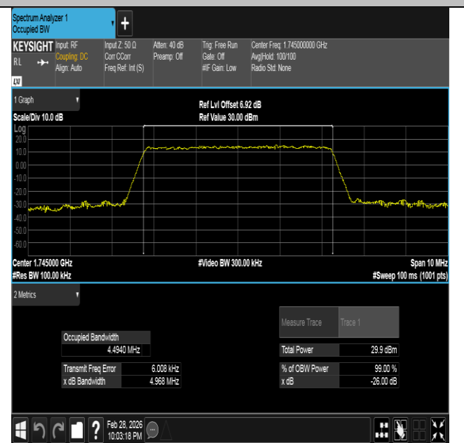
Band66-5MHz-16QAM-132322-25RB#0-PASS
