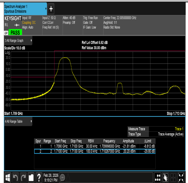
Band66-3MHz-16QAM-131987-1RB#0-PASS
