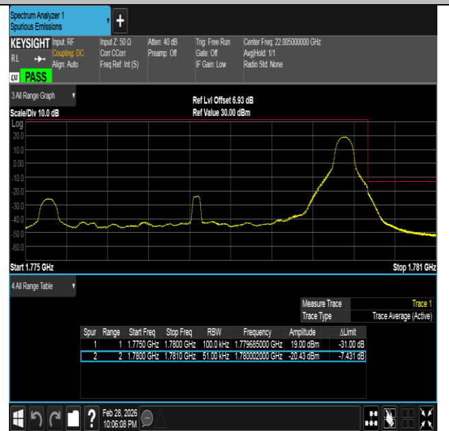
Band66-5MHz-QPSK-132647-1RB#24-PASS
