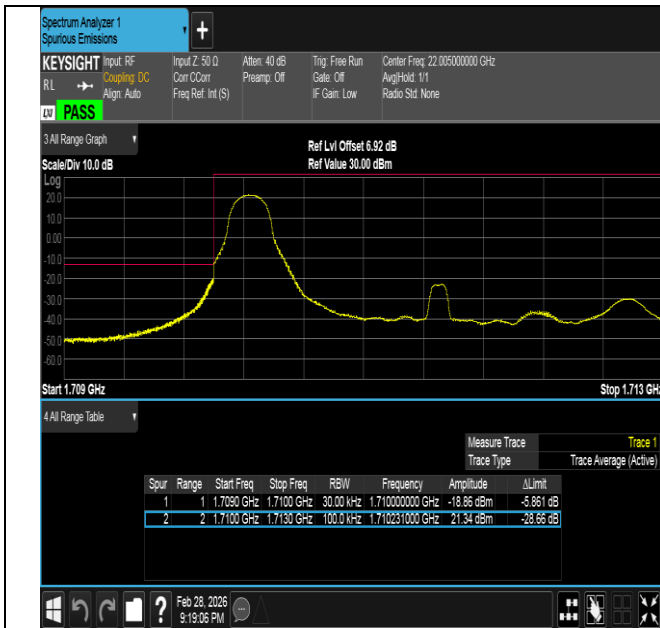
Band66-3MHz-QPSK-131987-1RB#0-PASS
