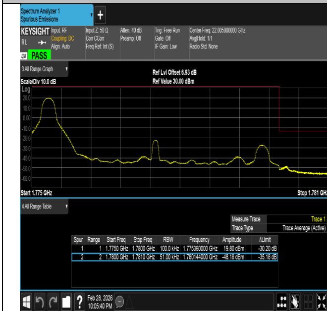
Band66-5MHz-QPSK-132647-1RB#0-PASS
