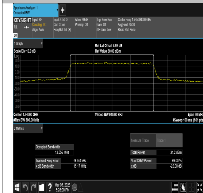
Band66-15MHz-QPSK-132322-75RB#0-PASS
