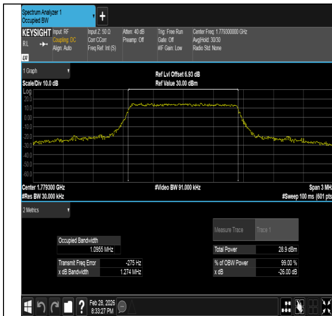
Band66-1.4MHz-QPSK-132665-6RB#0-PASS
