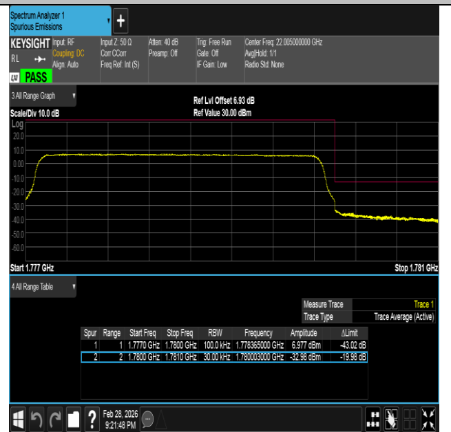
Band66-3MHz-16QAM-132657-15RB#0-PASS
