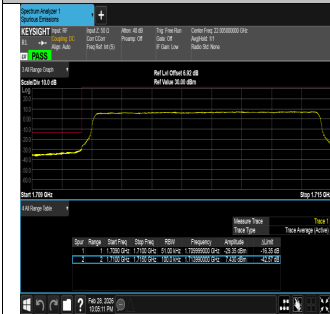
Band66-5MHz-QPSK-131997-25RB#0-PASS
