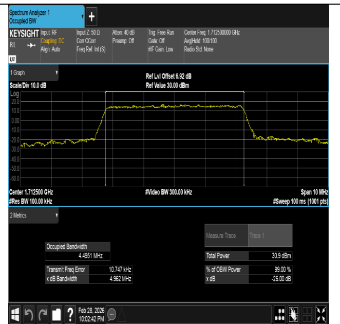
Band66-5MHz-16QAM-131997-25RB#0-PASS
