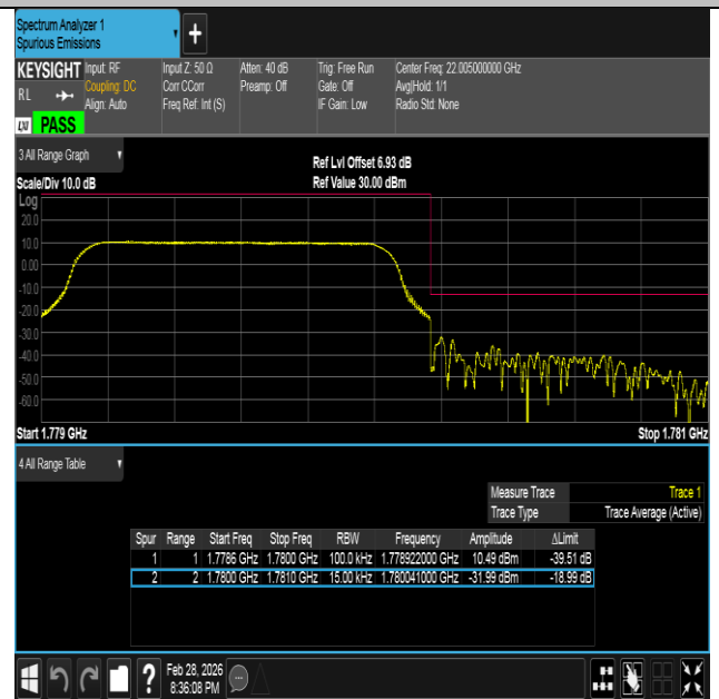
Band66-1.4MHz-16QAM-132665-6RB#0-PASS
