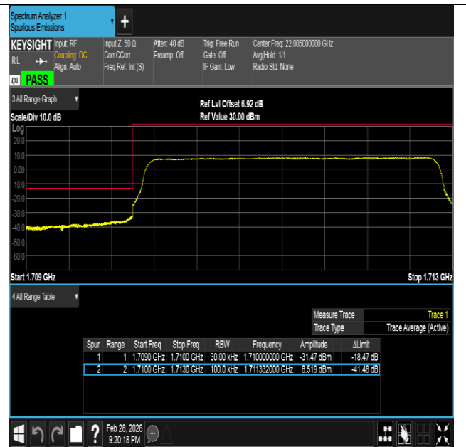
Band66-3MHz-16QAM-131987-15RB#0-PASS
