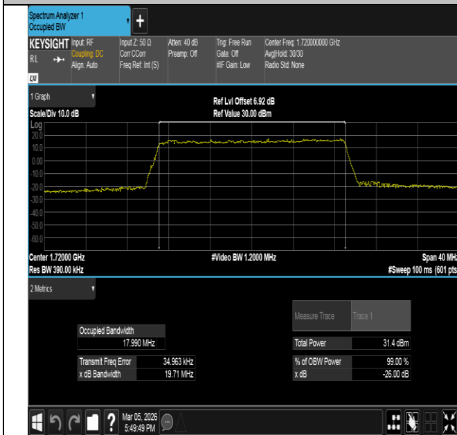
Band66-20MHz-QPSK-132072-100RB#0-PASS
