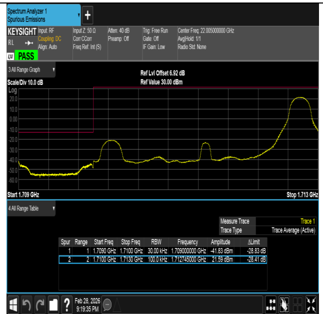
Band66-3MHz-QPSK-131987-1RB#14-PASS
