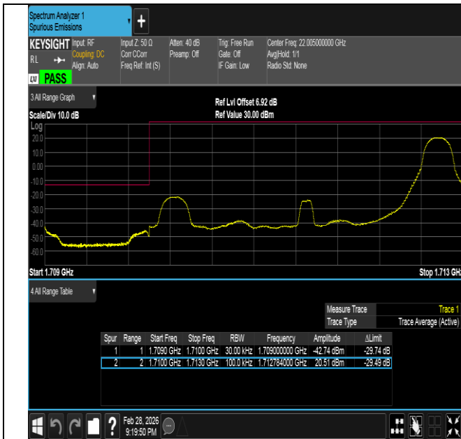
Band66-3MHz-16QAM-131987-1RB#14-PASS
