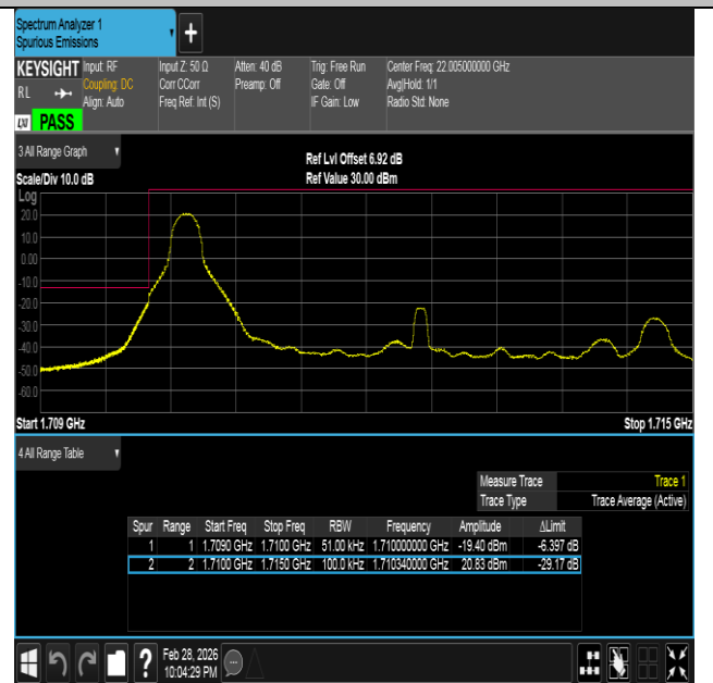
Band66-5MHz-16QAM-131997-1RB#0-PASS
