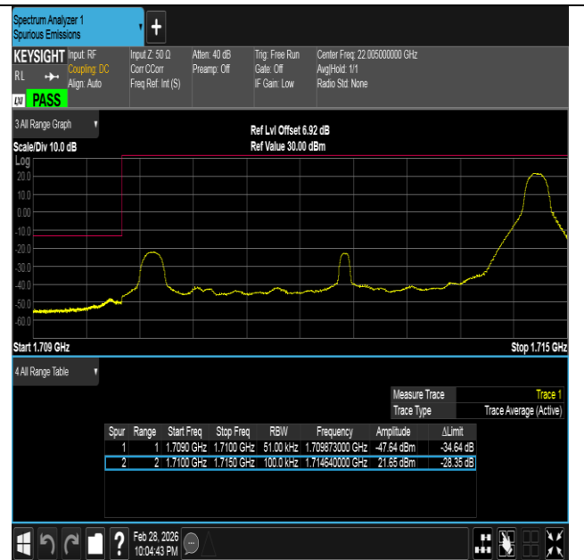
Band66-5MHz-QPSK-131997-1RB#24-PASS
