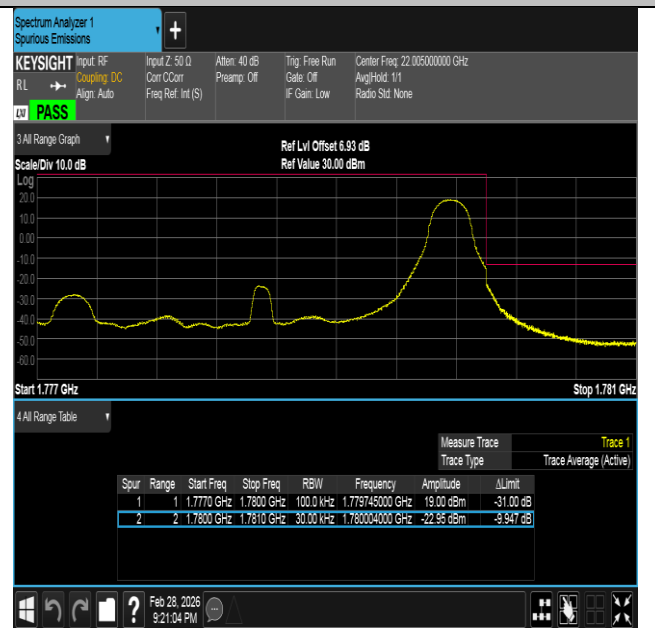
Band66-3MHz-QPSK-132657-1RB#14-PASS
