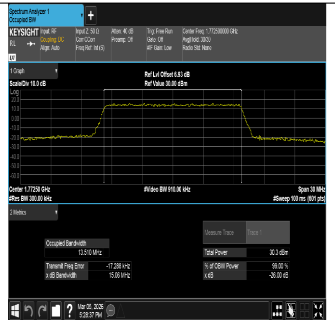
Band66-15MHz-16QAM-132597-75RB#0-PASS
