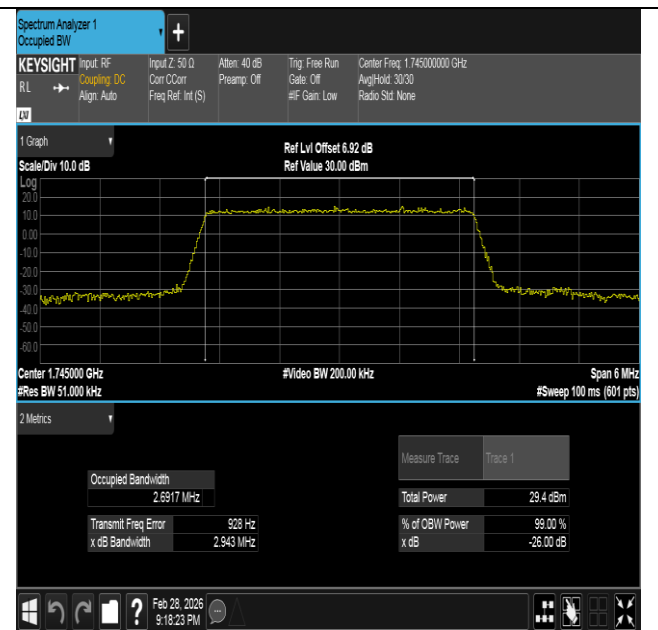
Band66-3MHz-16QAM-132322-15RB#0-PASS
