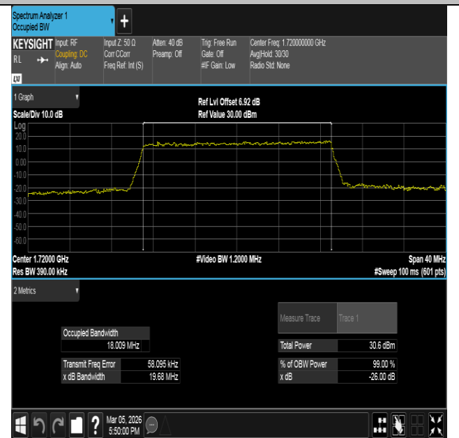
Band66-20MHz-16QAM-132072-100RB#0-PASS
