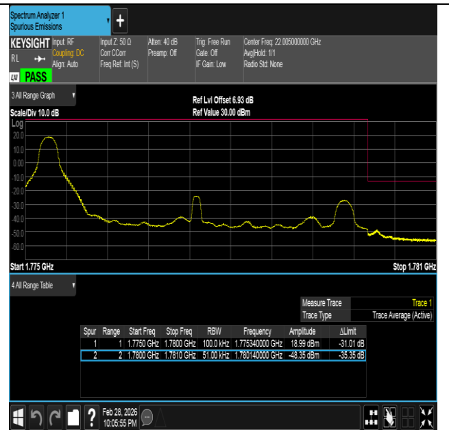
Band66-5MHz-16QAM-132647-1RB#0-PASS
