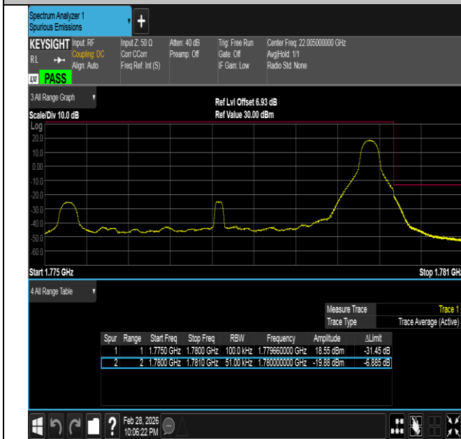
Band66-5MHz-16QAM-132647-1RB#24-PASS
