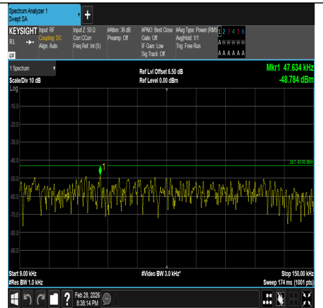
Band66-1.4MHz-QPSK-131979-1RB#5-0.009~0.15-PASS
