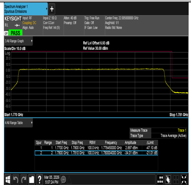
Band66-10MHz-16QAM-132622-50RB#0-PASS
