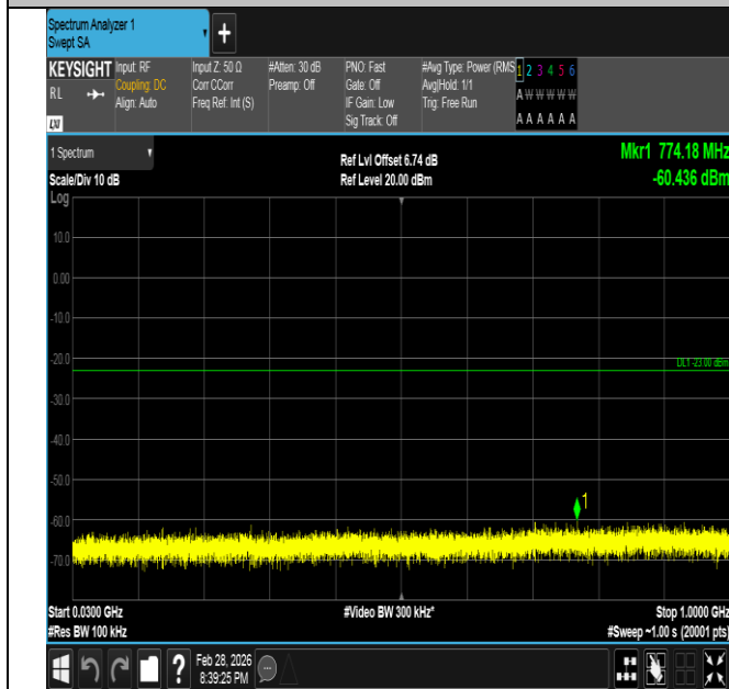
Band66-1.4MHz-16QAM-131979-1RB#5-30~1000-PASS
