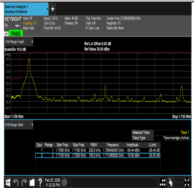
Band66-20MHz-16QAM-132072-1RB#0-PASS
