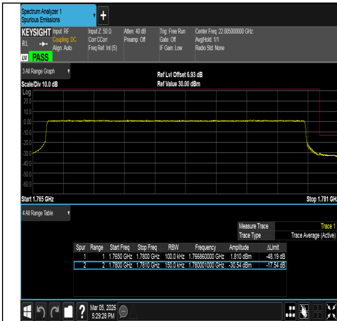
Band66-15MHz-QPSK-132597-75RB#0-PASS
