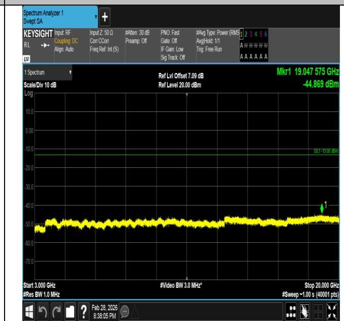
Band66-1.4MHz-16QAM-131979-1RB#0-3000~20000-PASS
