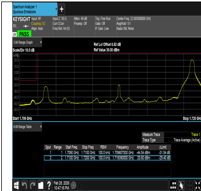
Band66-10MHz-16QAM-132022-1RB#49-PASS
