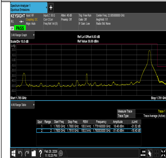
Band66-15MHz-16QAM-132597-1RB#74-PASS
