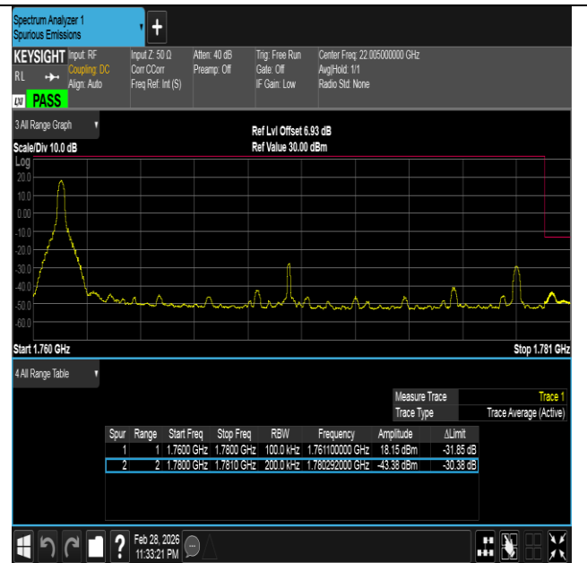
Band66-20MHz-16QAM-132572-1RB#0-PASS
