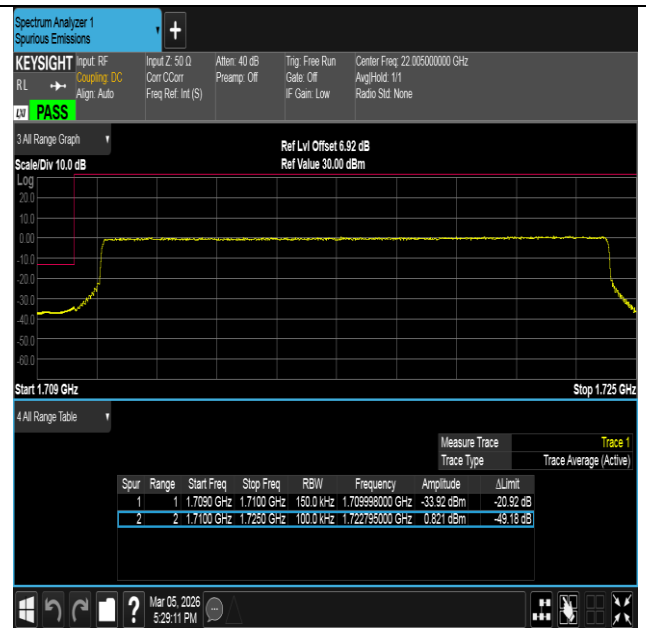
Band66-15MHz-16QAM-132047-75RB#0-PASS
