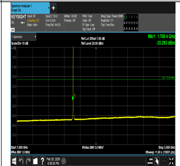
Band66-1.4MHz-16QAM-131979-1RB#5-1000~3000-PASS
