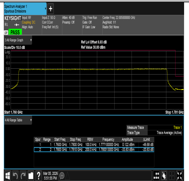
Band66-20MHz-16QAM-132572-100RB#0-PASS
