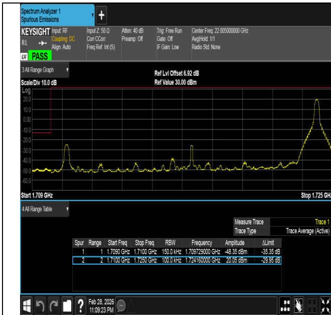
Band66-15MHz-16QAM-132047-1RB#74-PASS
