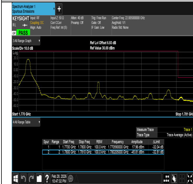
Band66-10MHz-QPSK-132622-1RB#0-PASS
