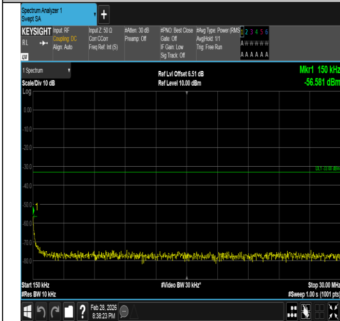
Band66-1.4MHz-QPSK-131979-1RB#5-0.15~30-PASS
