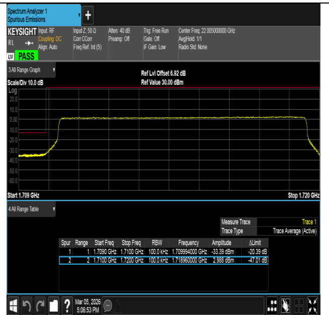
Band66-10MHz-16QAM-132022-50RB#0-PASS
