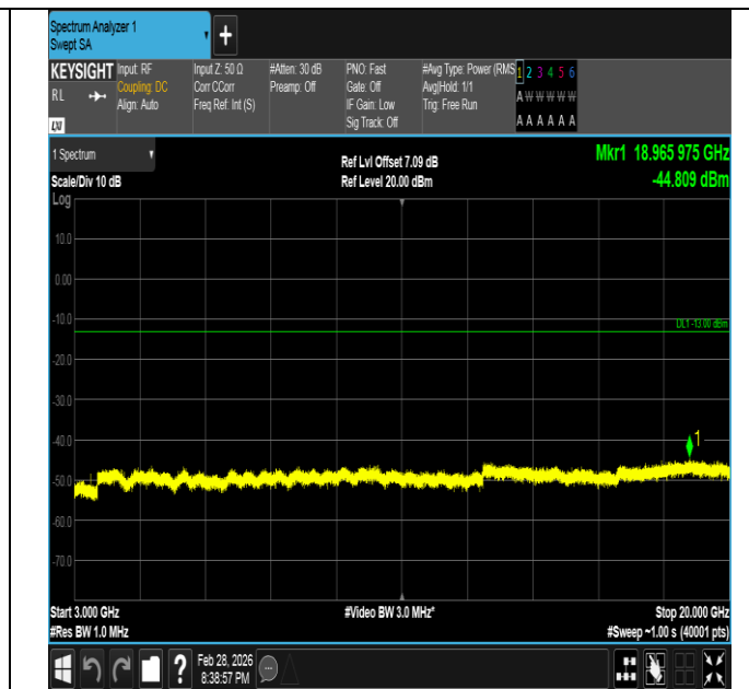
Band66-1.4MHz-QPSK-131979-1RB#5-3000~20000-PASS
