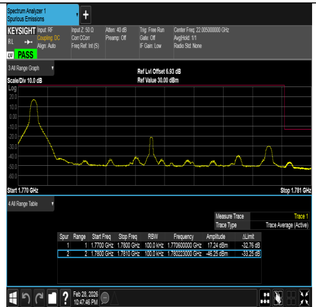
Band66-10MHz-16QAM-132622-1RB#0-PASS
