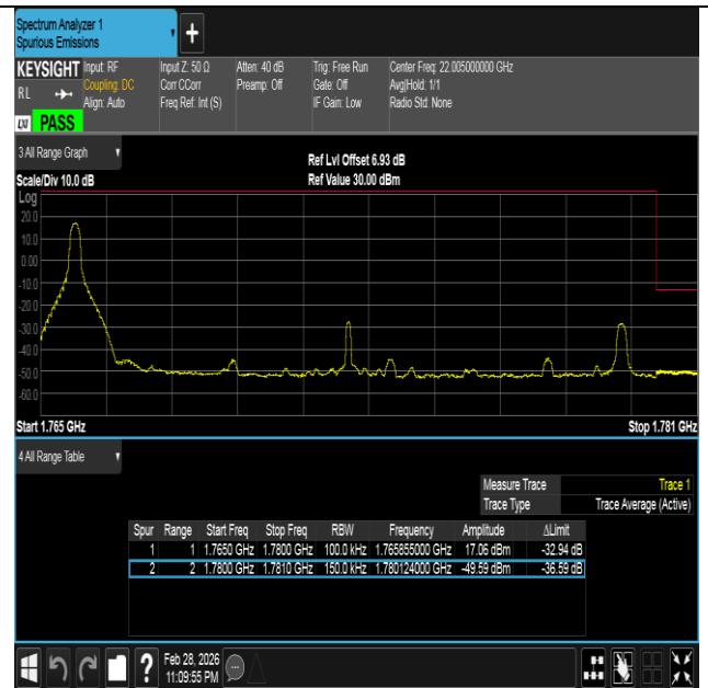
Band66-15MHz-16QAM-132597-1RB#0-PASS
