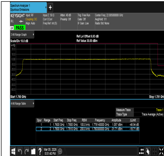
Band66-20MHz-QPSK-132572-100RB#0-PASS
