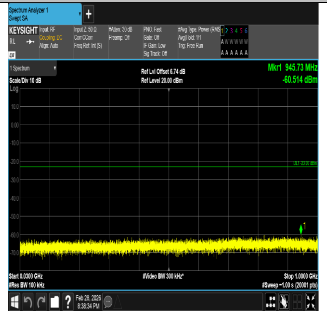
Band66-1.4MHz-QPSK-131979-1RB#5-30~1000-PASS
