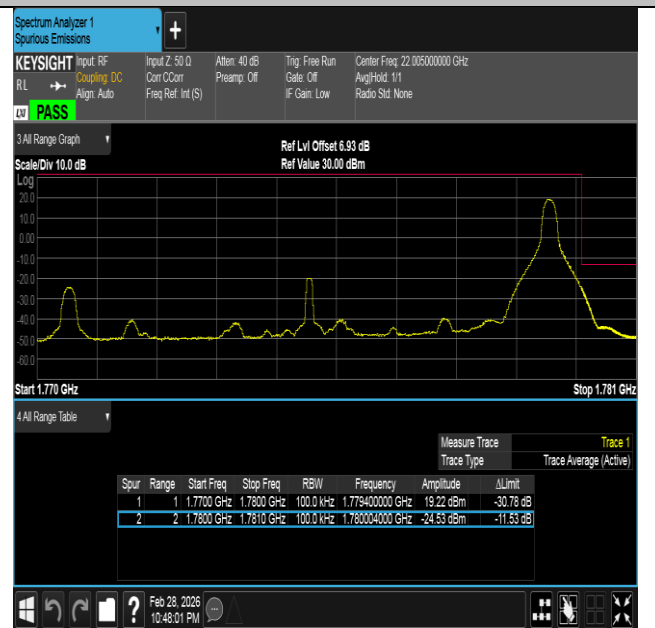
Band66-10MHz-QPSK-132622-1RB#49-PASS
