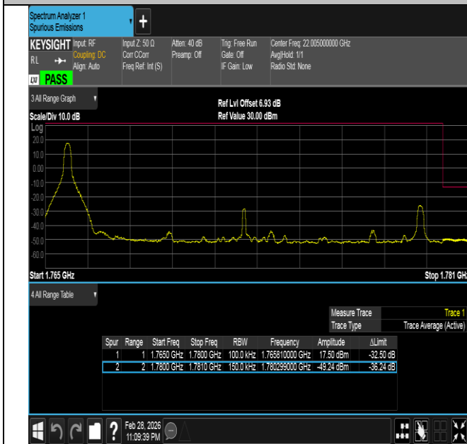
Band66-15MHz-QPSK-132597-1RB#0-PASS
