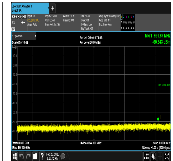
Band66-1.4MHz-16QAM-131979-1RB#0-30~1000-PASS
