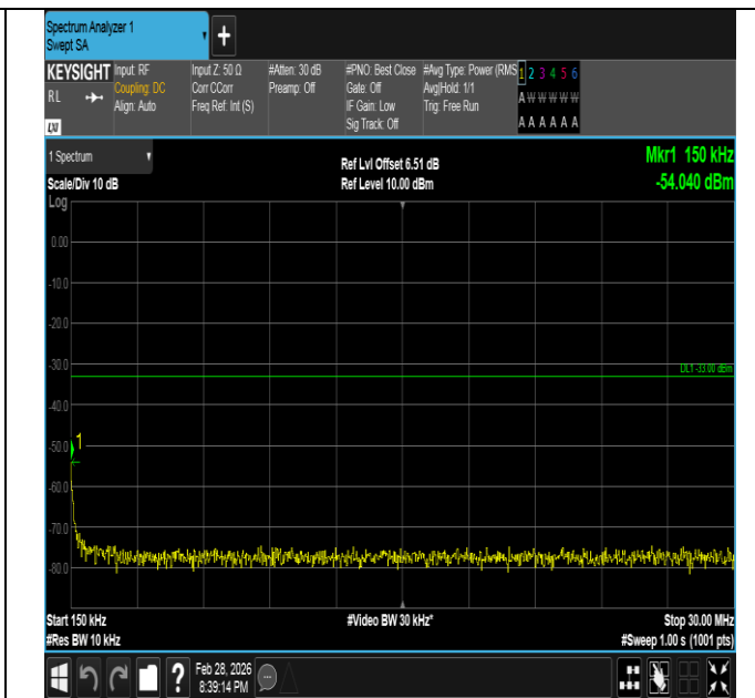
Band66-1.4MHz-16QAM-131979-1RB#5-0.15~30-PASS
