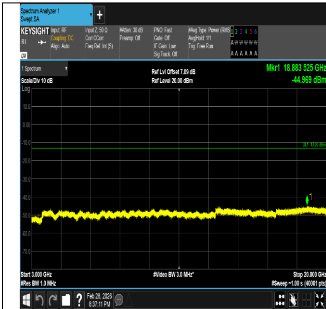
Band66-1.4MHz-QPSK-131979-1RB#0-3000~20000-PASS
