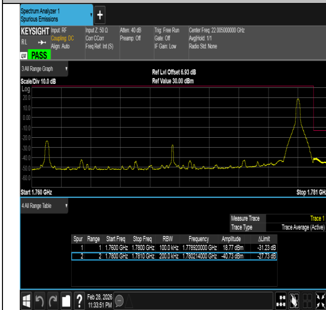
Band66-20MHz-16QAM-132572-1RB#99-PASS
