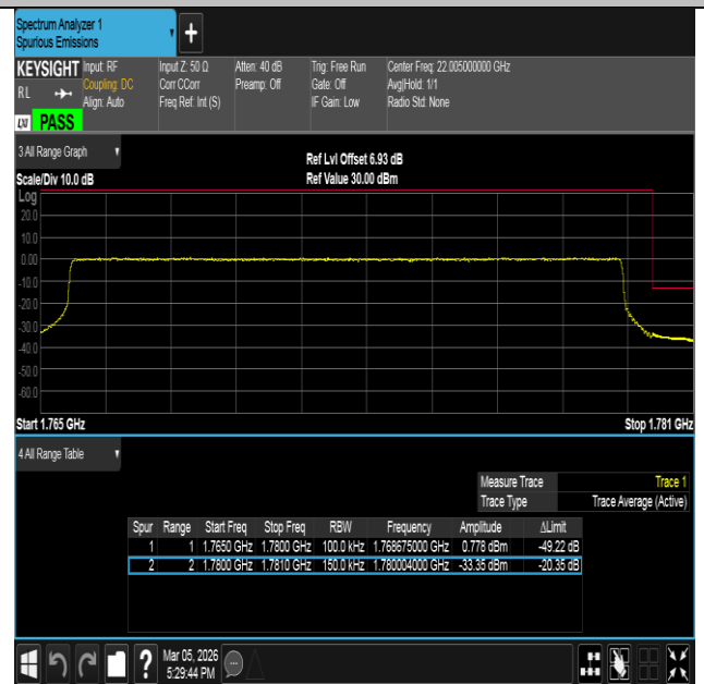
Band66-15MHz-16QAM-132597-75RB#0-PASS
