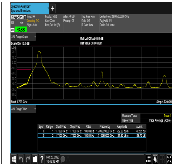
Band66-10MHz-QPSK-132022-1RB#0-PASS
