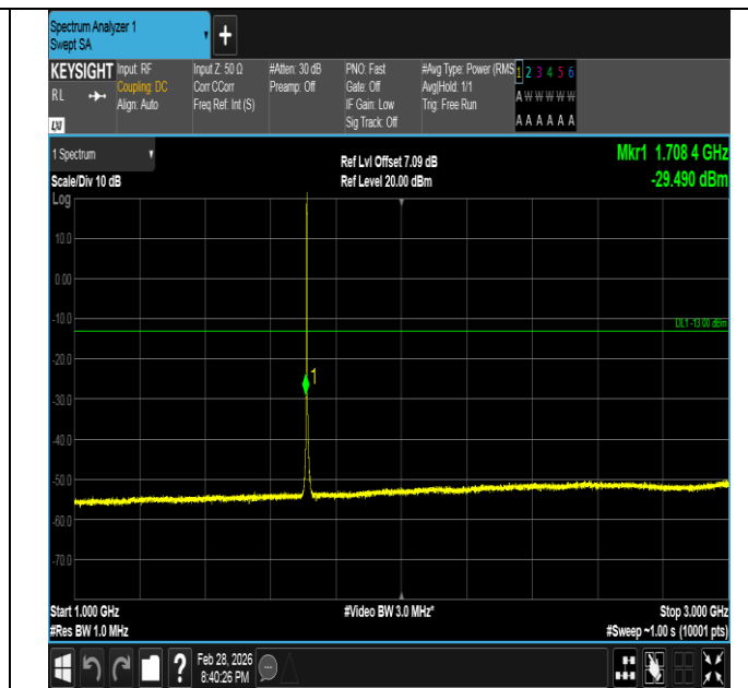
Band66-1.4MHz-QPSK-131979-6RB#0-1000~3000-PASS
