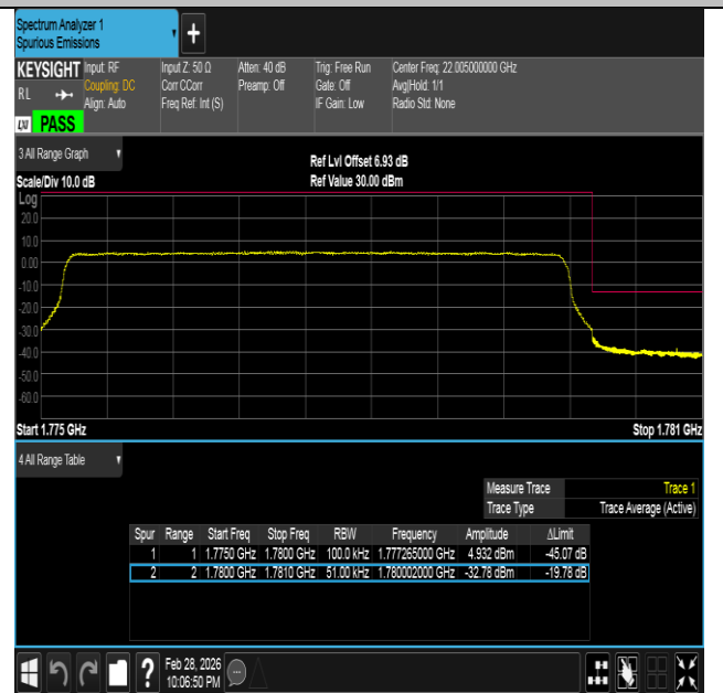
Band66-5MHz-16QAM-132647-25RB#0-PASS
