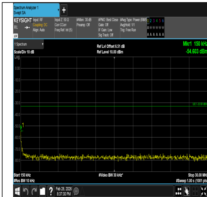
Band66-1.4MHz-16QAM-131979-1RB#0-0.15~30-PASS
