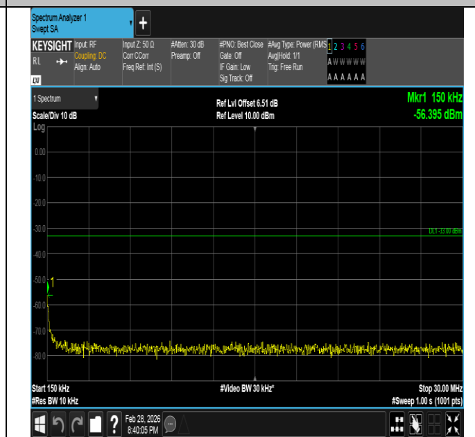
Band66-1.4MHz-QPSK-131979-6RB#0-0.15~30-PASS
