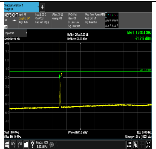
Band66-3MHz-QPSK-131987-1RB#0-1000~3000-PASS
