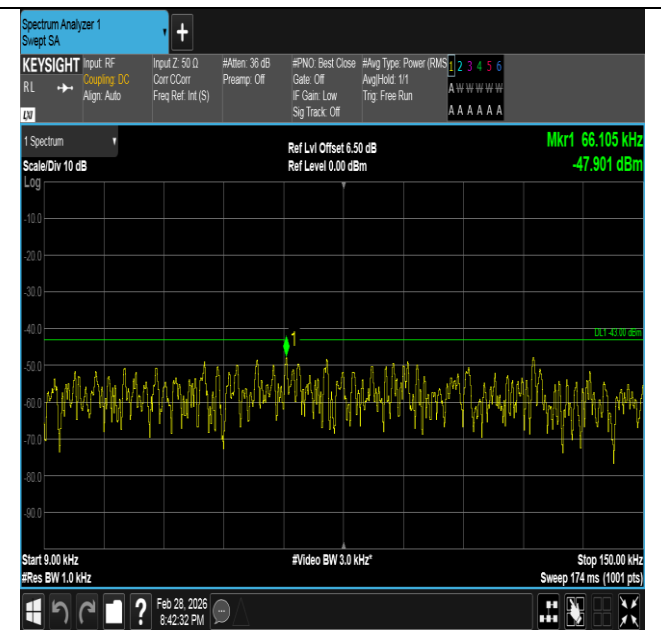
Band66-1.4MHz-16QAM-132322-1RB#0-0.009~0.15-PASS
