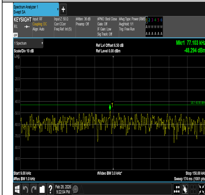
Band66-3MHz-QPSK-131987-1RB#0-0.009~0.15-PASS
