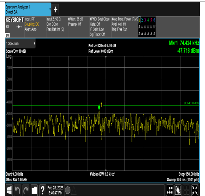
Band66-1.4MHz-16QAM-131979-6RB#0-0.009~0.15-PASS
