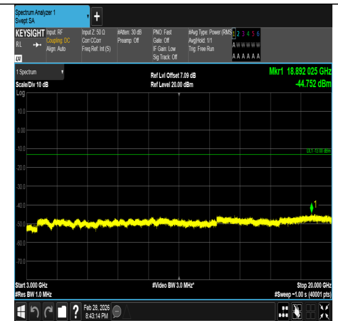
Band66-1.4MHz-16QAM-132322-1RB#0-3000~20000-PASS
