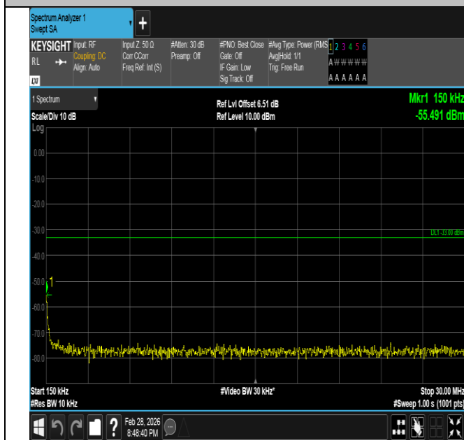
Band66-1.4MHz-QPSK-132665-1RB#5-0.15~30-PASS
