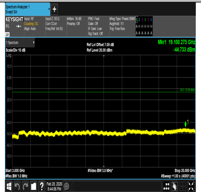
Band66-1.4MHz-QPSK-132322-1RB#5-3000~20000-PASS
