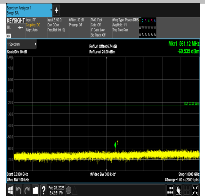
Band66-1.4MHz-16QAM-132322-1RB#0-30~1000-PASS
