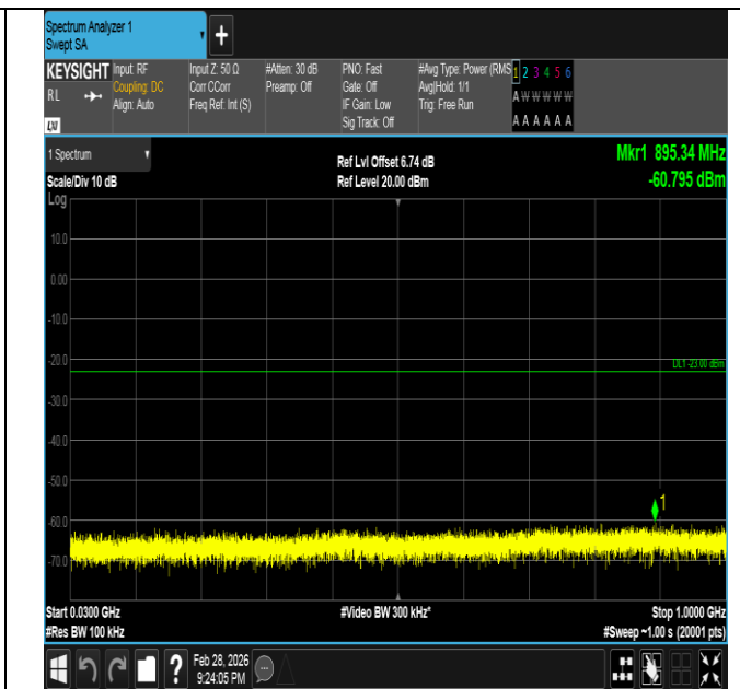
Band66-3MHz-QPSK-131987-1RB#14-30~1000-PASS
