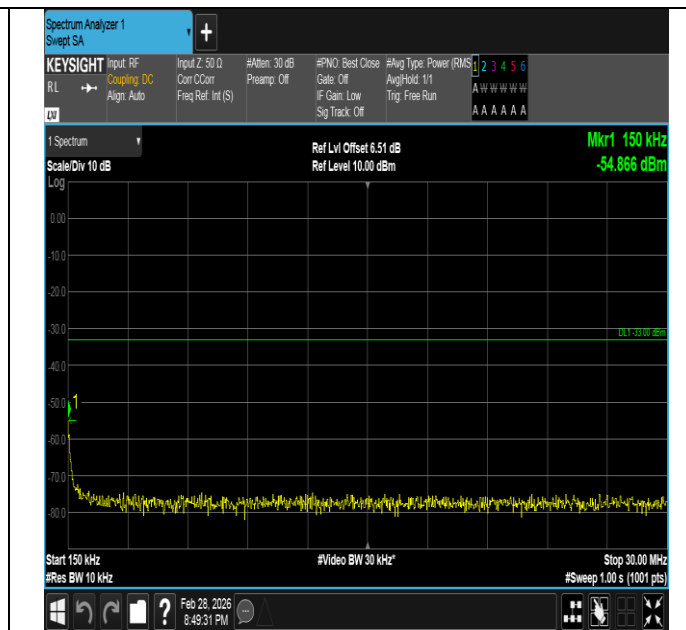
Band66-1.4MHz-16QAM-132665-1RB#5-0.15~30-PASS
