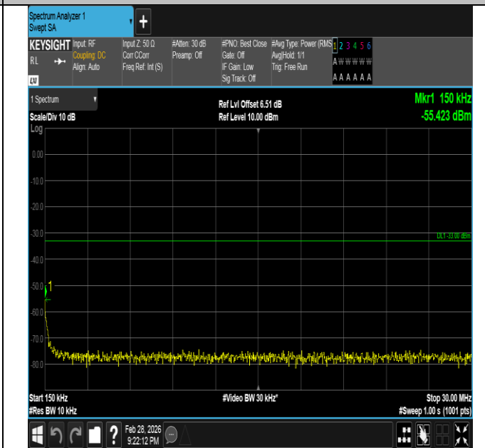
Band66-3MHz-QPSK-131987-1RB#0-0.15~30-PASS
