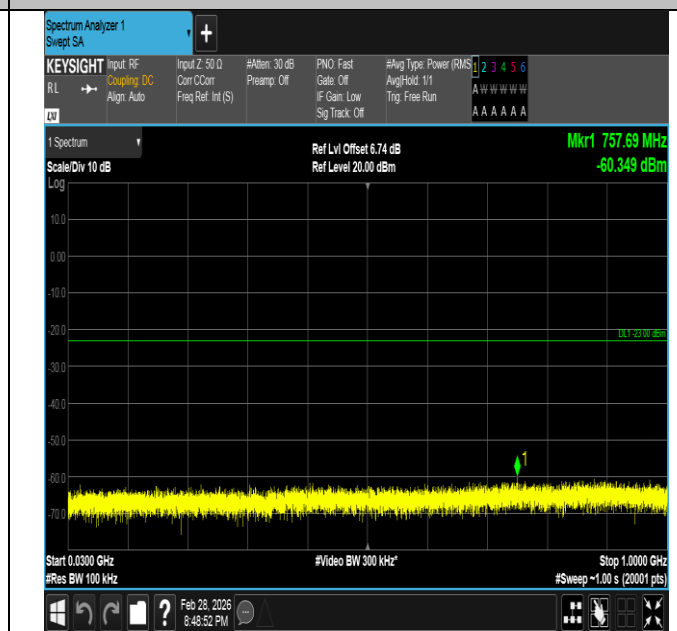
Band66-1.4MHz-QPSK-132665-1RB#5-30~1000-PASS
