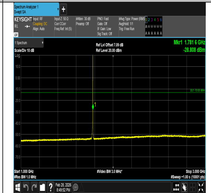
Band66-1.4MHz-16QAM-132665-1RB#5-1000~3000-PASS
