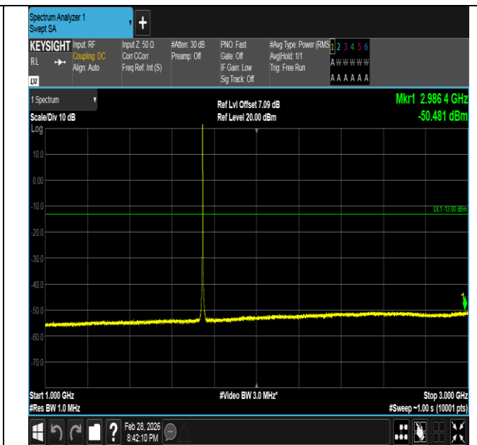
Band66-1.4MHz-QPSK-132322-1RB#0-1000~3000-PASS
