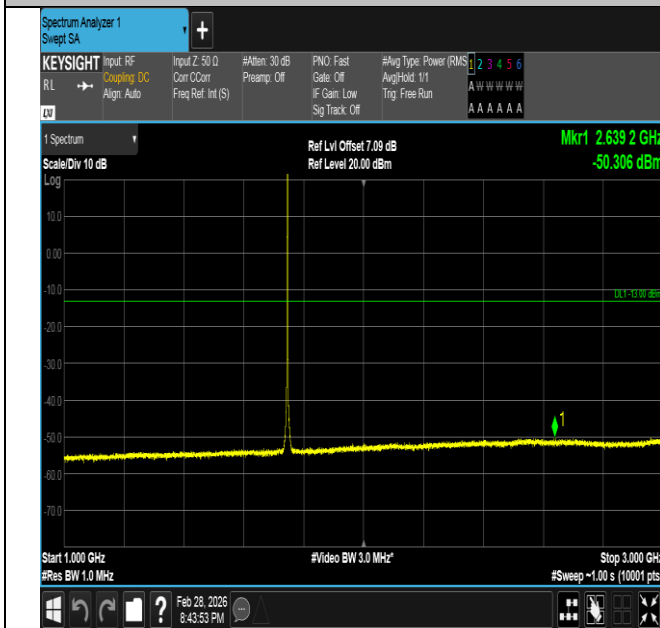
Band66-1.4MHz-QPSK-132322-1RB#5-1000~3000-PASS
