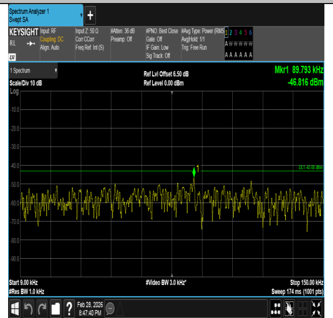
Band66-1.4MHz-16QAM-132665-1RB#0-0.009~0.15-PASS
