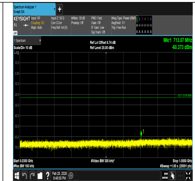
Band66-1.4MHz-16QAM-132665-1RB#0-30~1000-PASS
