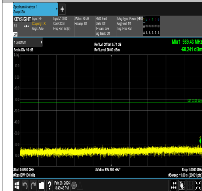
Band66-1.4MHz-16QAM-132665-1RB#5-30~1000-PASS
