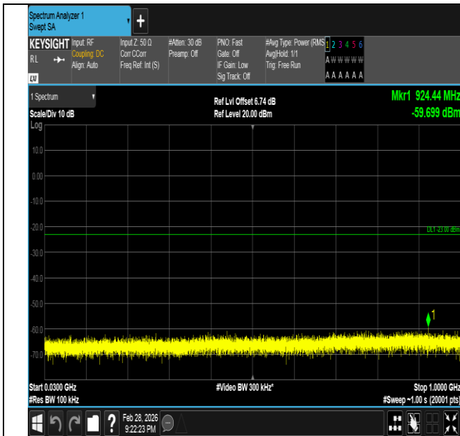
Band66-3MHz-QPSK-131987-1RB#0-30~1000-PASS
