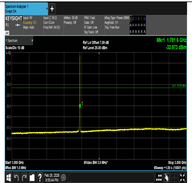
Band66-1.4MHz-QPSK-132665-6RB#0-1000~3000-PASS
