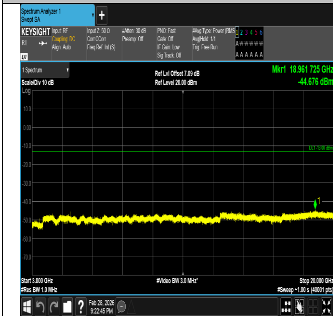
Band66-3MHz-QPSK-131987-1RB#0-3000~20000-PASS
