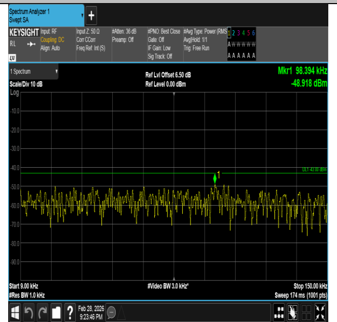
Band66-3MHz-QPSK-131987-1RB#14-0.009~0.15-PASS
