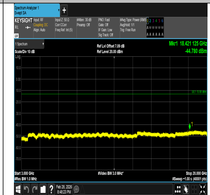
Band66-1.4MHz-16QAM-132665-1RB#0-3000~20000-PASS
