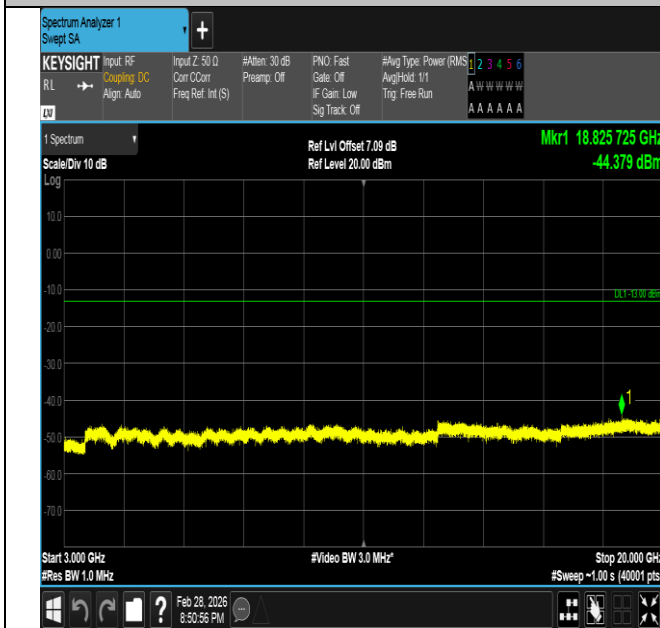
Band66-1.4MHz-QPSK-132665-6RB#0-3000~20000-PASS
