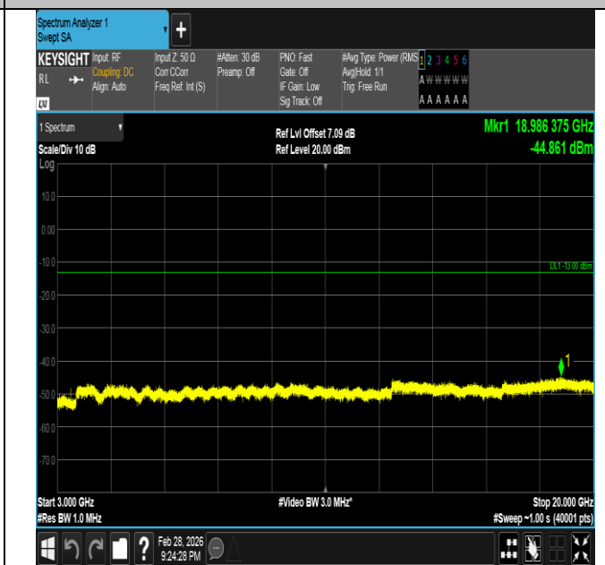
Band66-3MHz-QPSK-131987-1RB#14-3000~20000-PASS
