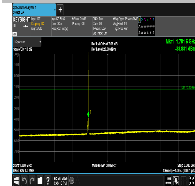
Band66-1.4MHz-16QAM-132665-1RB#0-1000~3000-PASS
