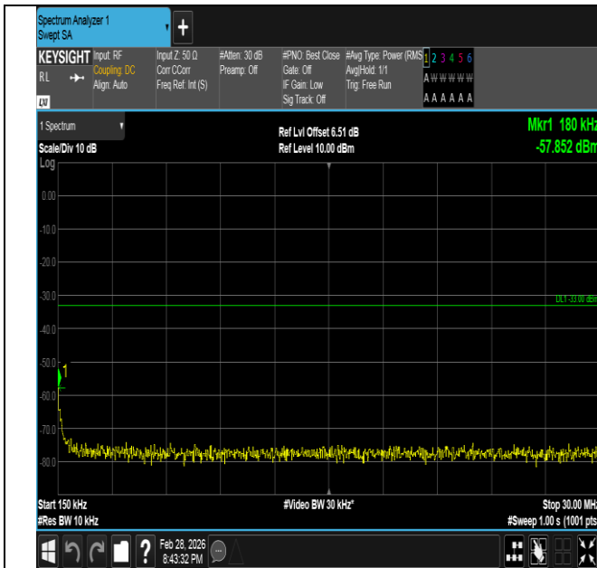
Band66-1.4MHz-QPSK-132322-1RB#5-0.15~30-PASS
