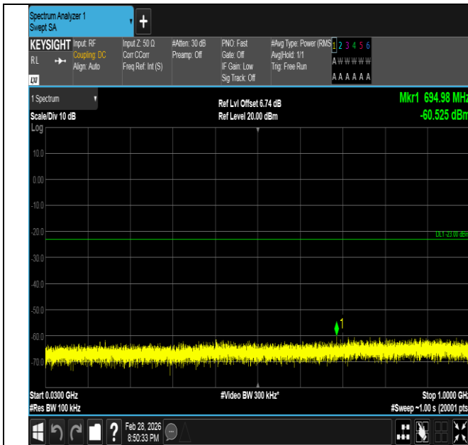
Band66-1.4MHz-QPSK-132665-6RB#0-30~1000-PASS
