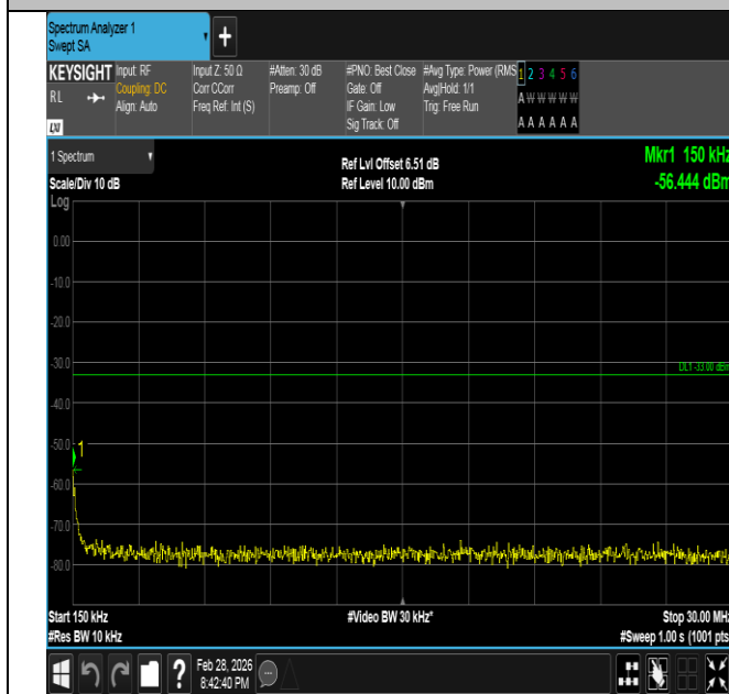
Band66-1.4MHz-16QAM-132322-1RB#0-0.15~30-PASS
