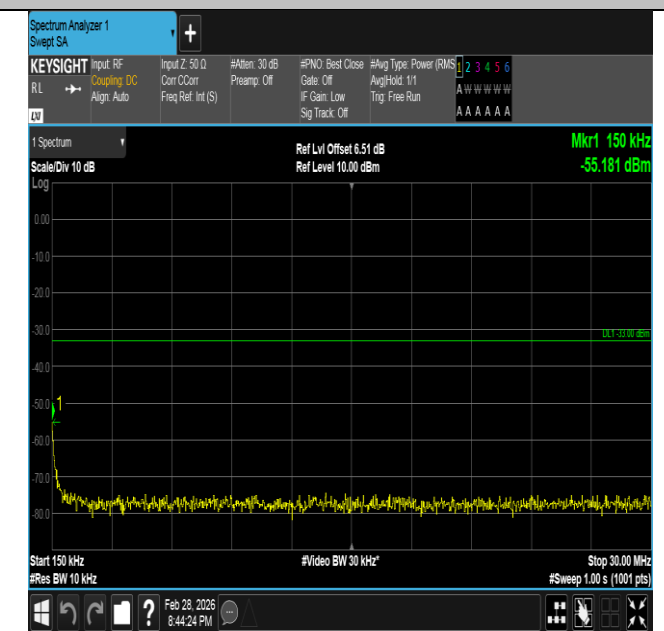
Band66-1.4MHz-16QAM-132322-1RB#5-0.15~30-PASS
