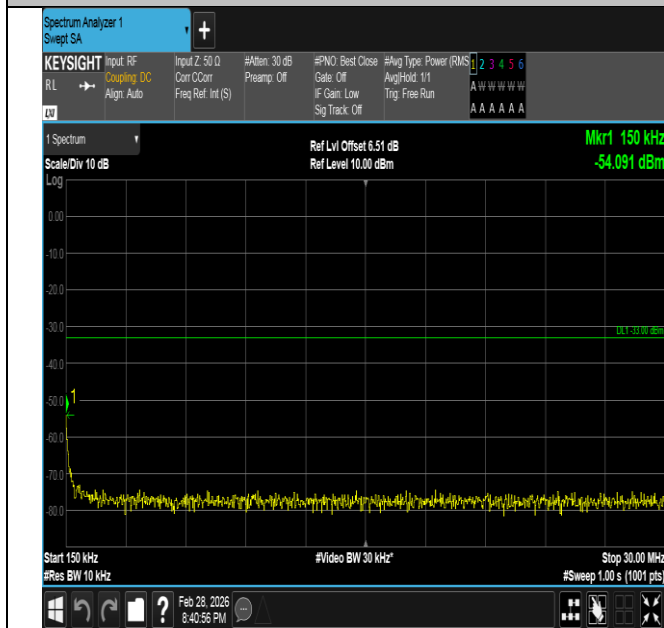
Band66-1.4MHz-16QAM-131979-6RB#0-0.15~30-PASS
