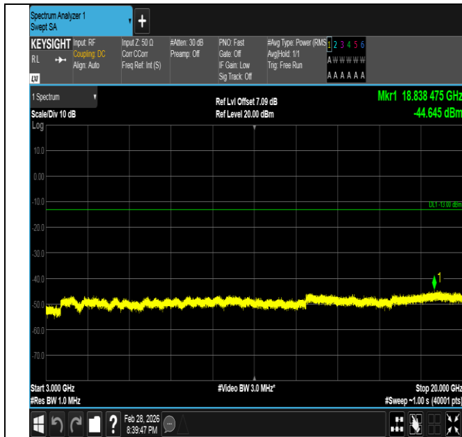
Band66-1.4MHz-16QAM-131979-1RB#5-3000~20000-PASS
