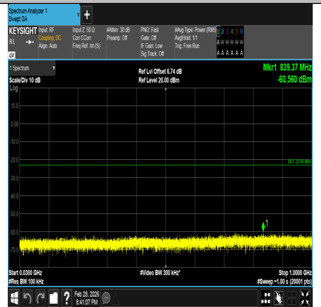
Band66-1.4MHz-16QAM-131979-6RB#0-30~1000-PASS
