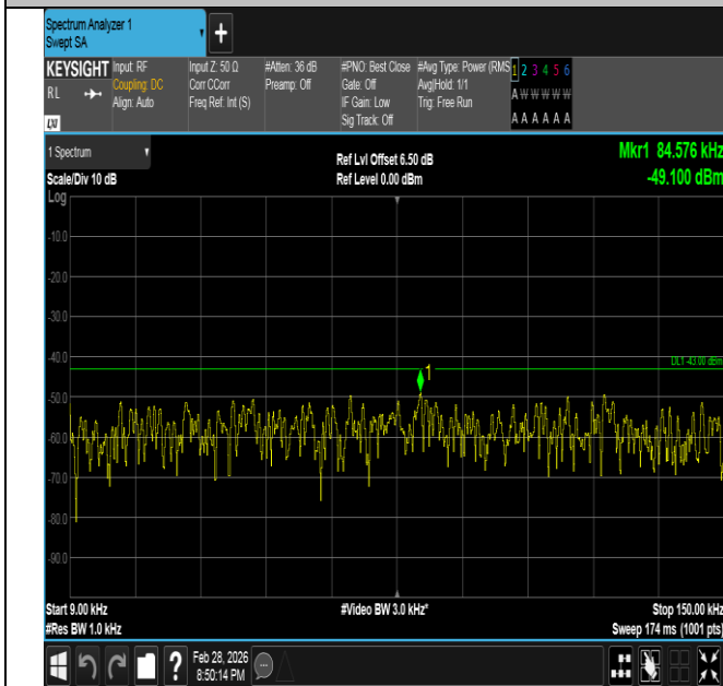
Band66-1.4MHz-QPSK-132665-6RB#0-0.009~0.15-PASS
